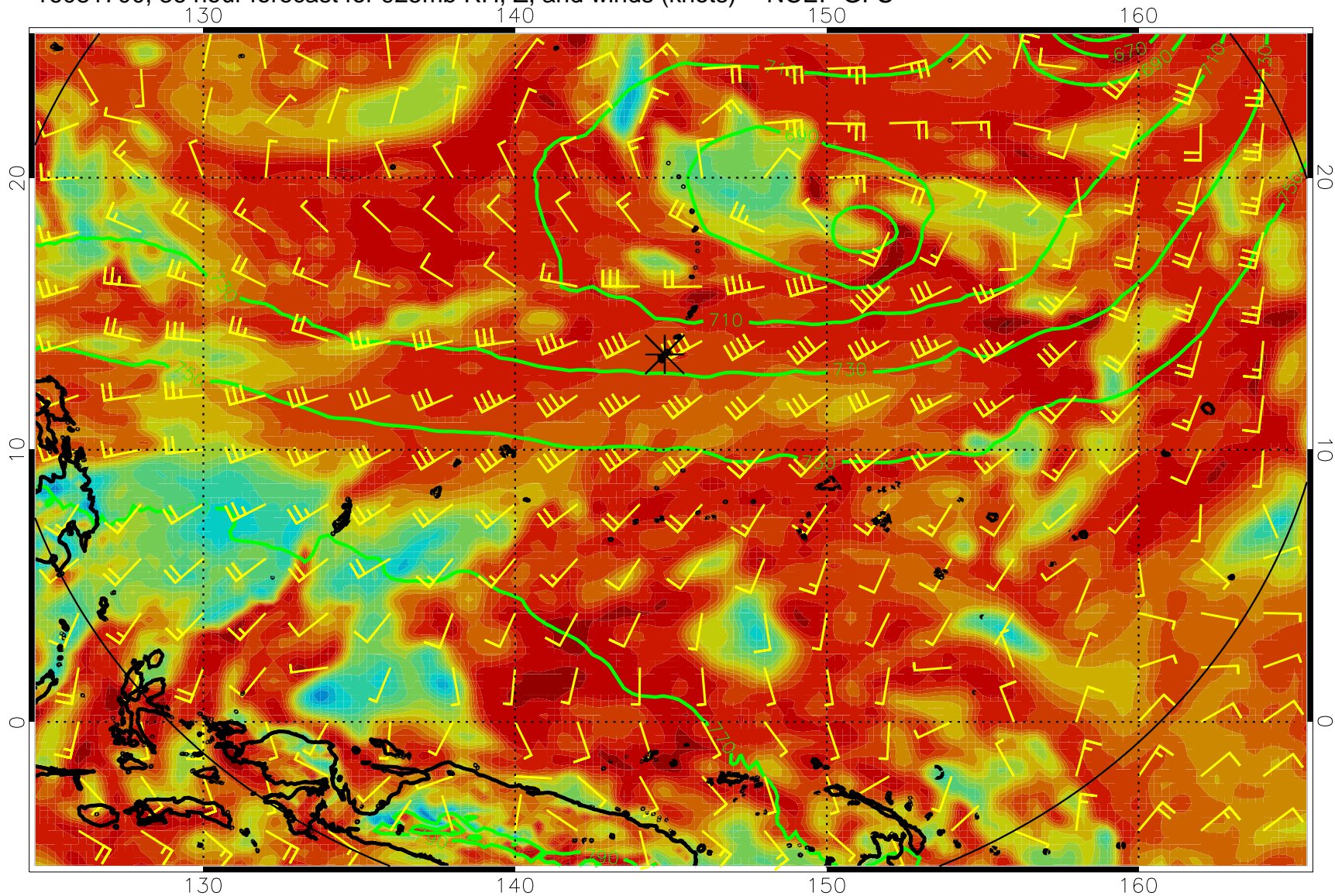
16081700, 36 hour forecast for 925mb RH, Z, and winds (knots) -- NCEP GFS
