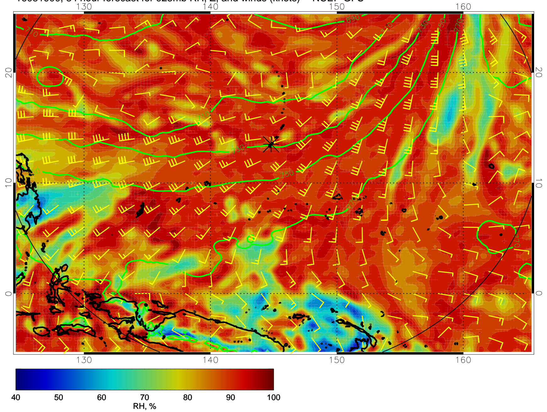
16081900, 84 hour forecast for 925mb RH, Z, and winds (knots) -- NCEP GFS
