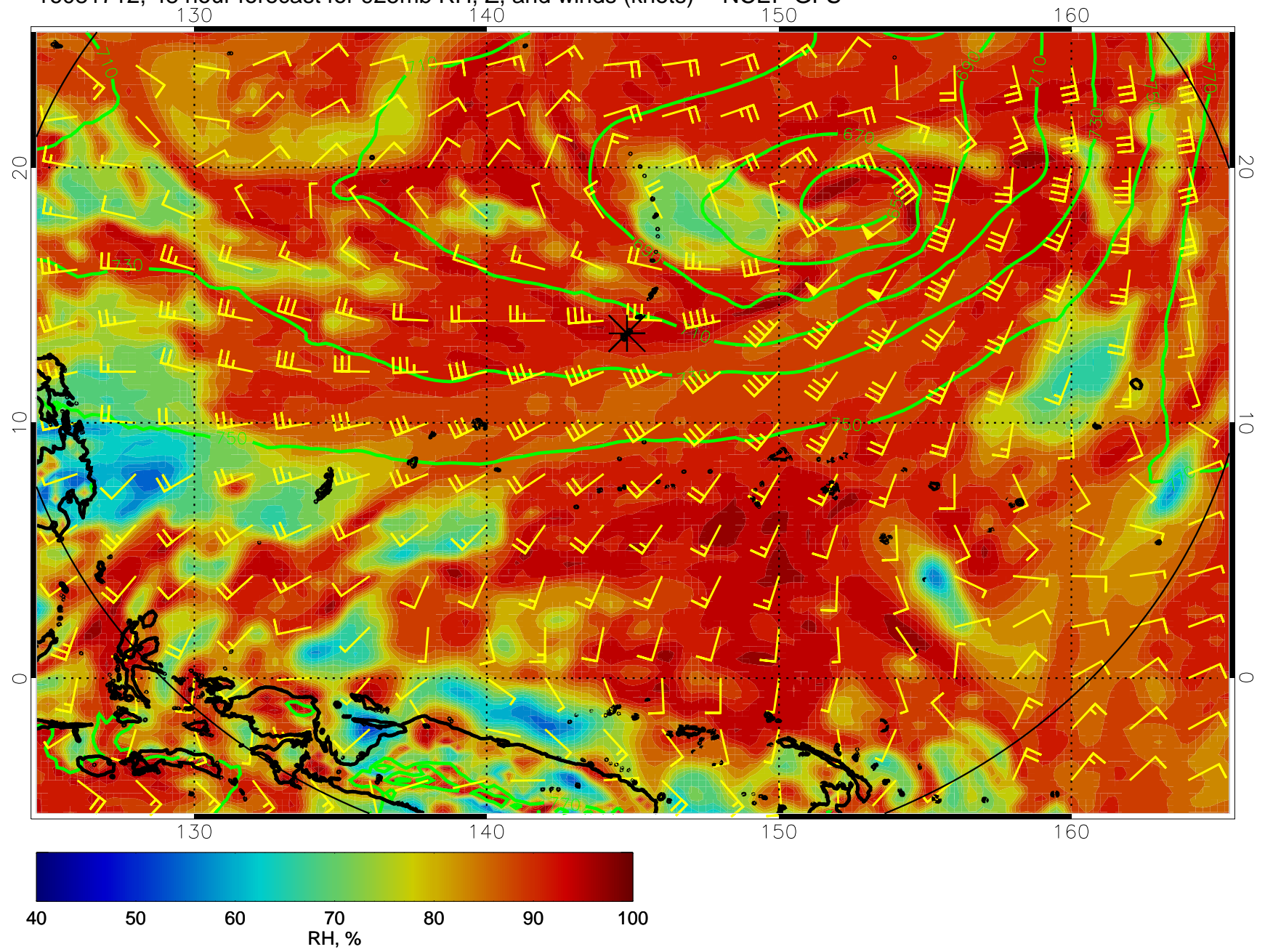
16081712, 48 hour forecast for 925mb RH, Z, and winds (knots) -- NCEP GFS
