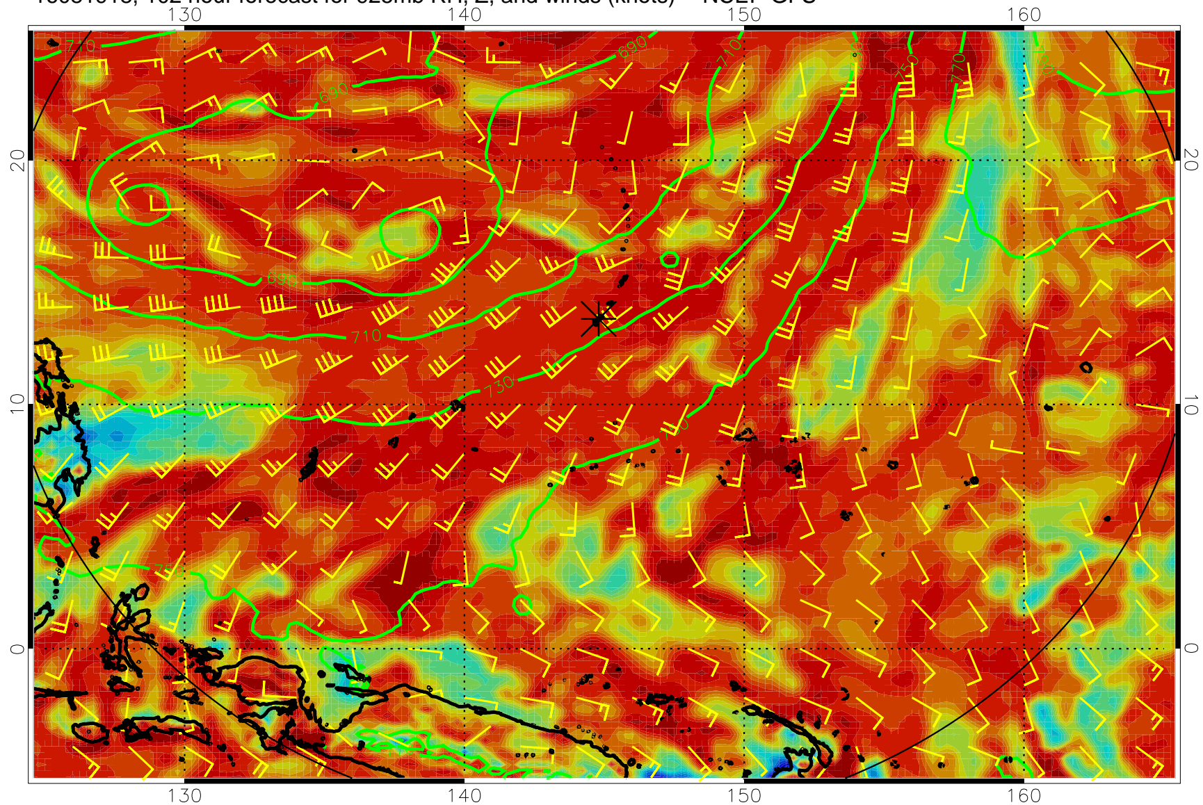
16081918, 102 hour forecast for 925mb RH, Z, and winds (knots) -- NCEP GFS
