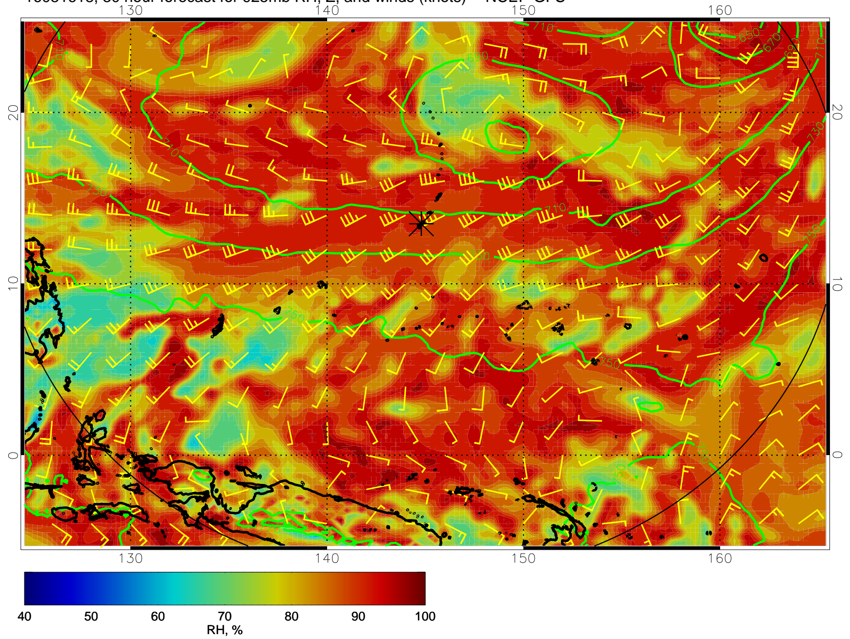
16081618, 30 hour forecast for 925mb RH, Z, and winds (knots) -- NCEP GFS
