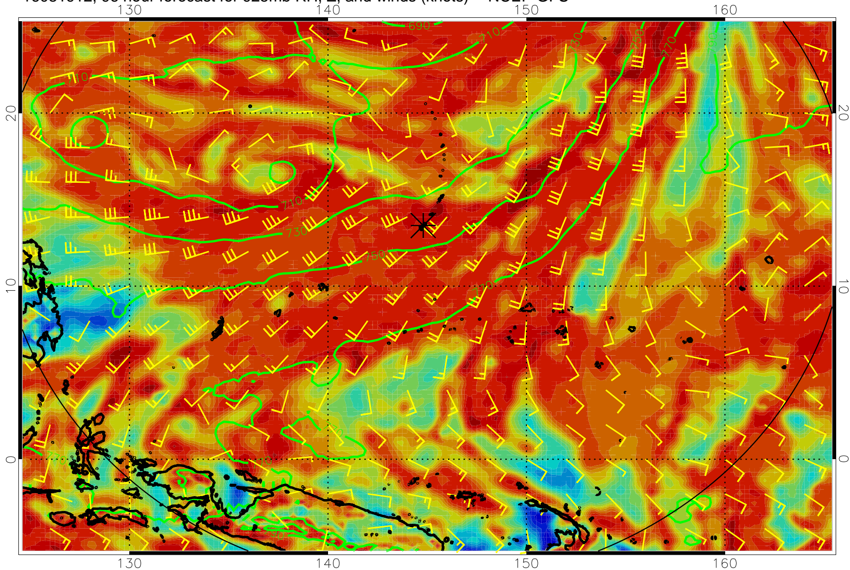
16081912, 96 hour forecast for 925mb RH, Z, and winds (knots) -- NCEP GFS
