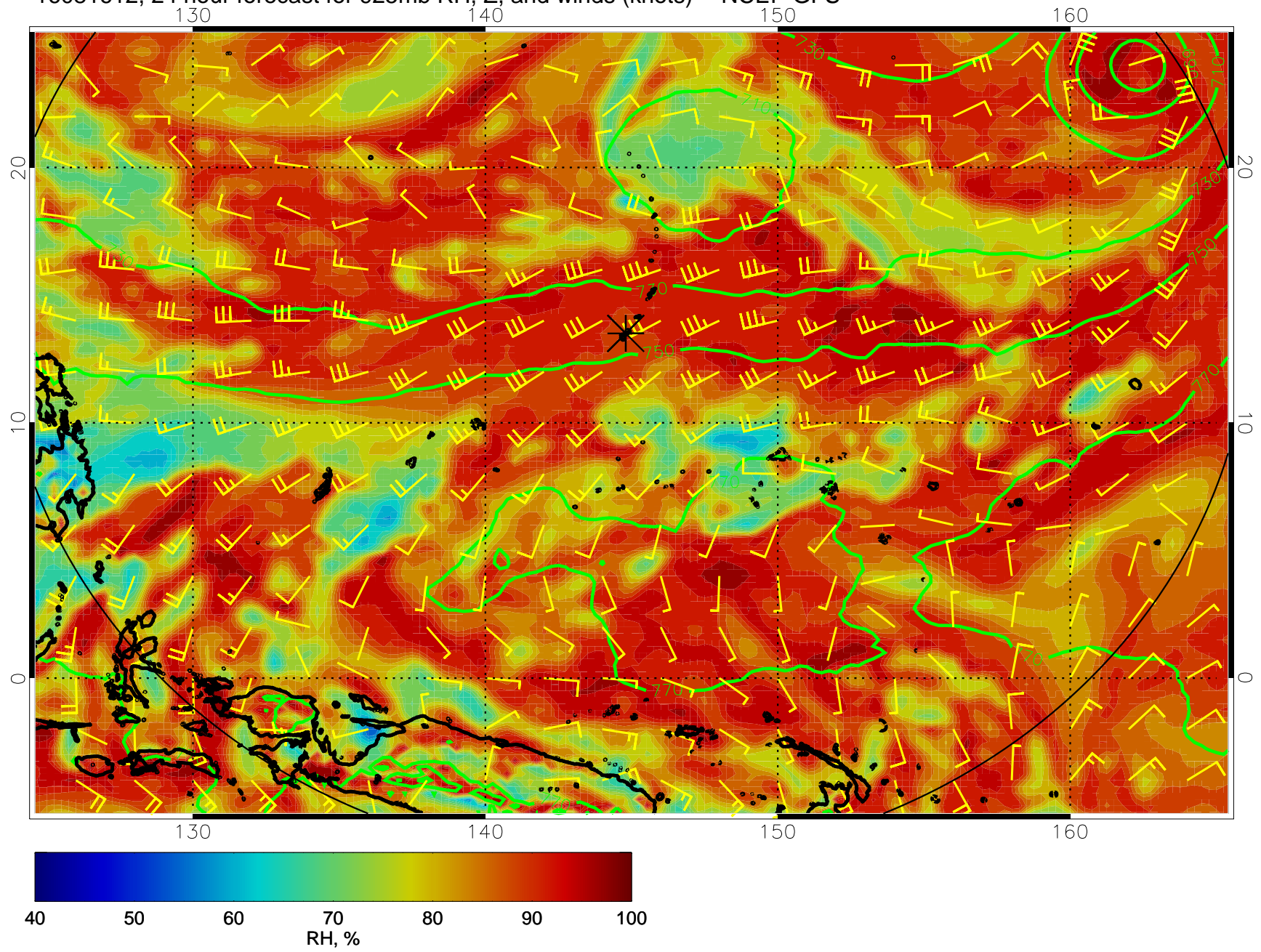
16081612, 24 hour forecast for 925mb RH, Z, and winds (knots) -- NCEP GFS
