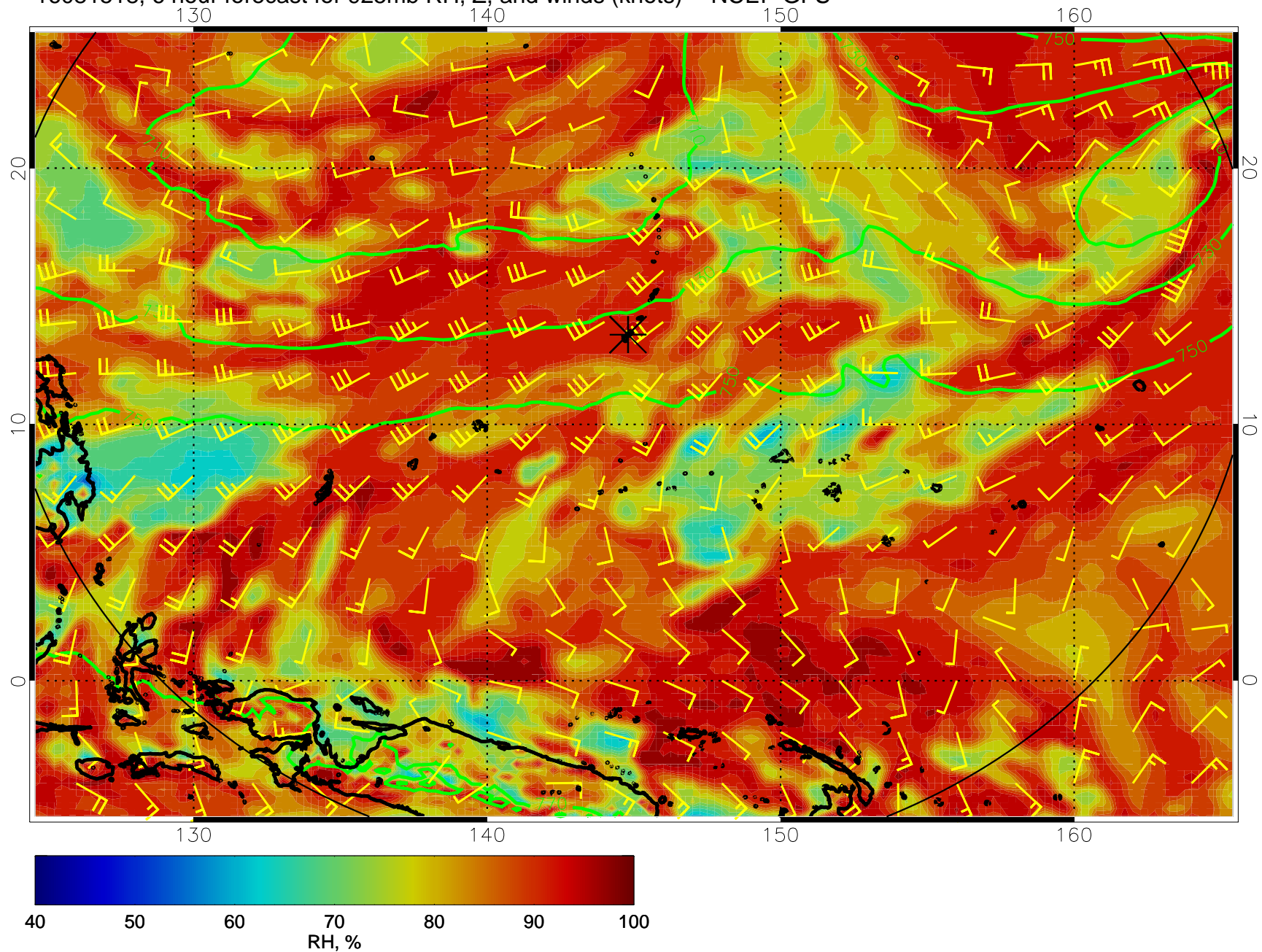
16081518, 6 hour forecast for 925mb RH, Z, and winds (knots) -- NCEP GFS
