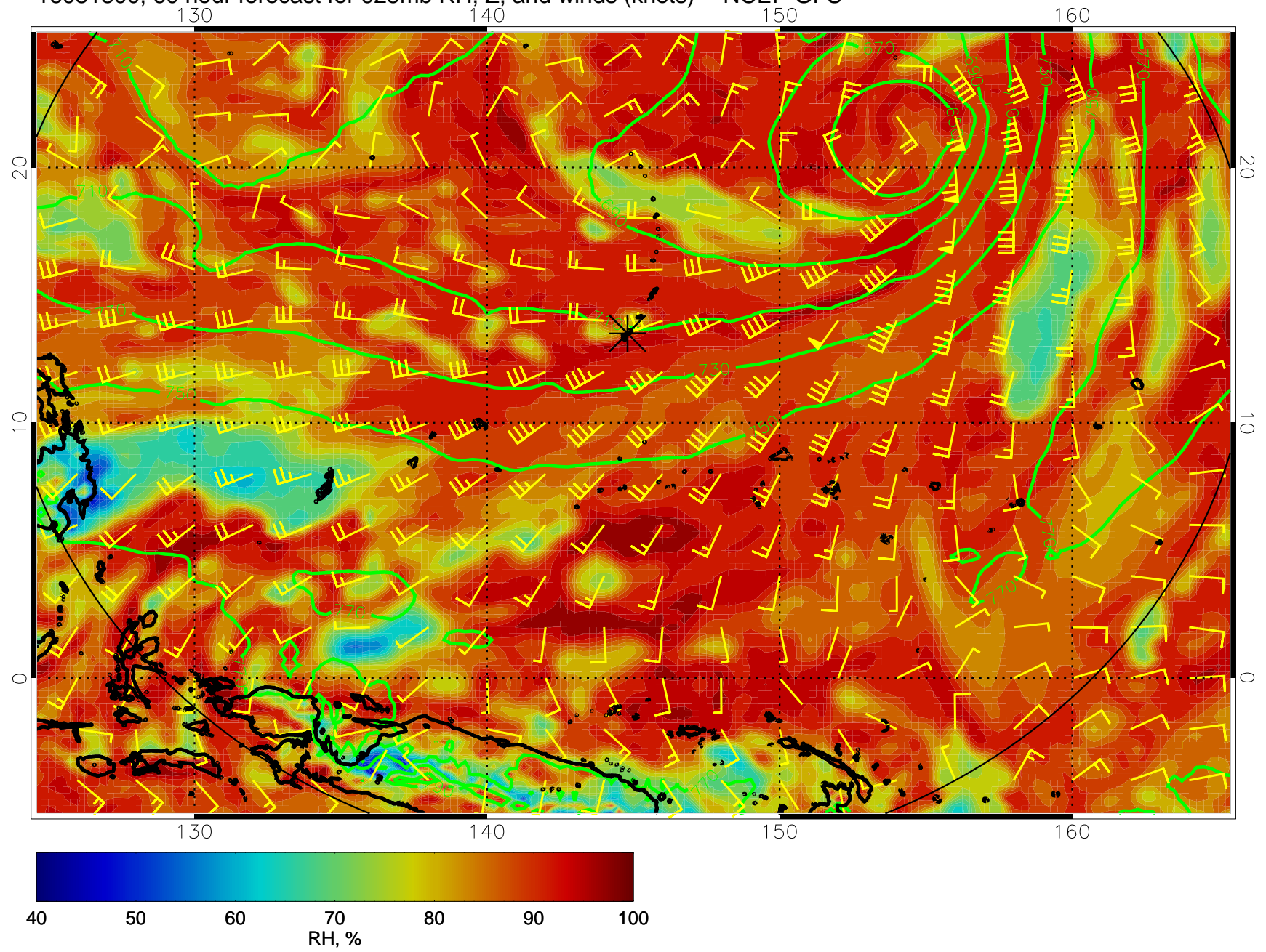
16081800, 60 hour forecast for 925mb RH, Z, and winds (knots) -- NCEP GFS
