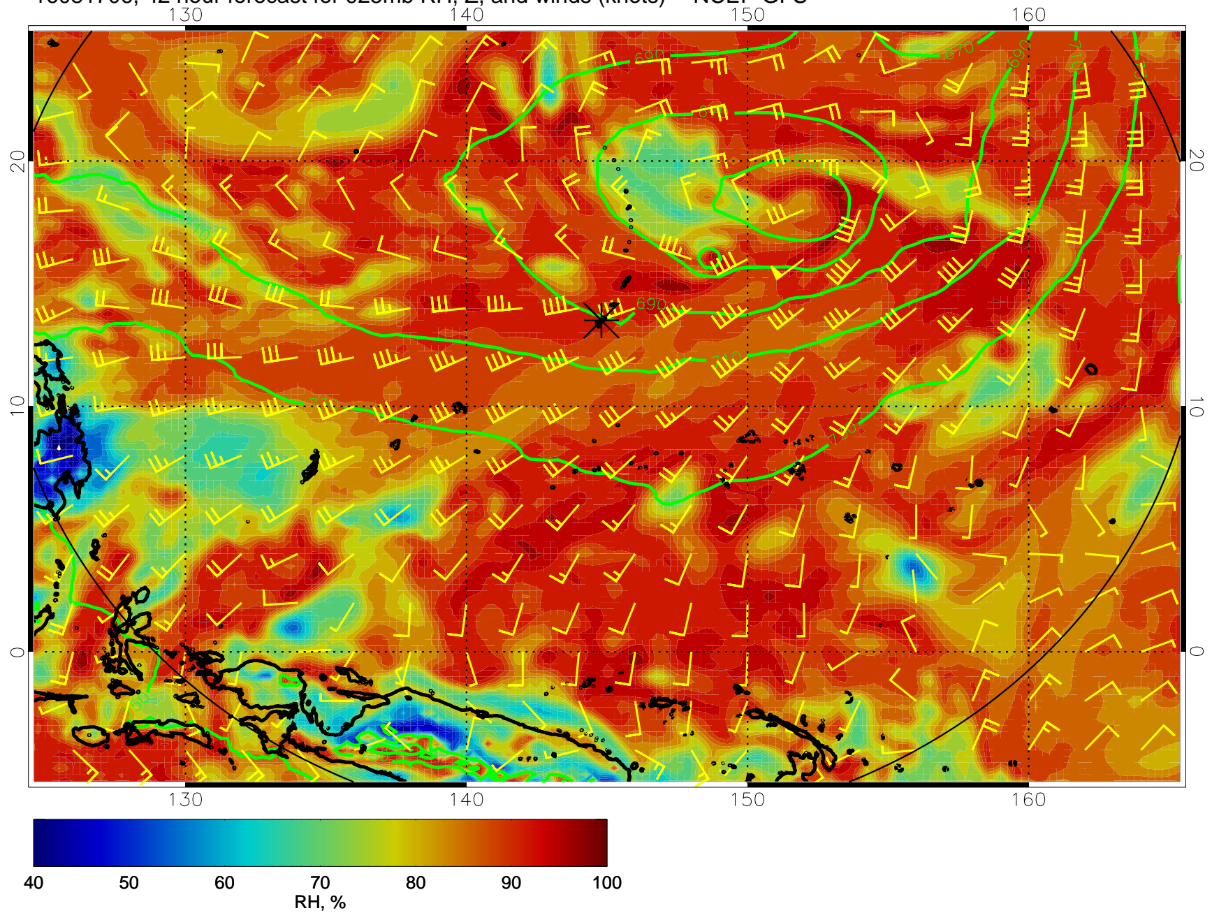
16081706, 42 hour forecast for 925mb RH, Z, and winds (knots) -- NCEP GFS
