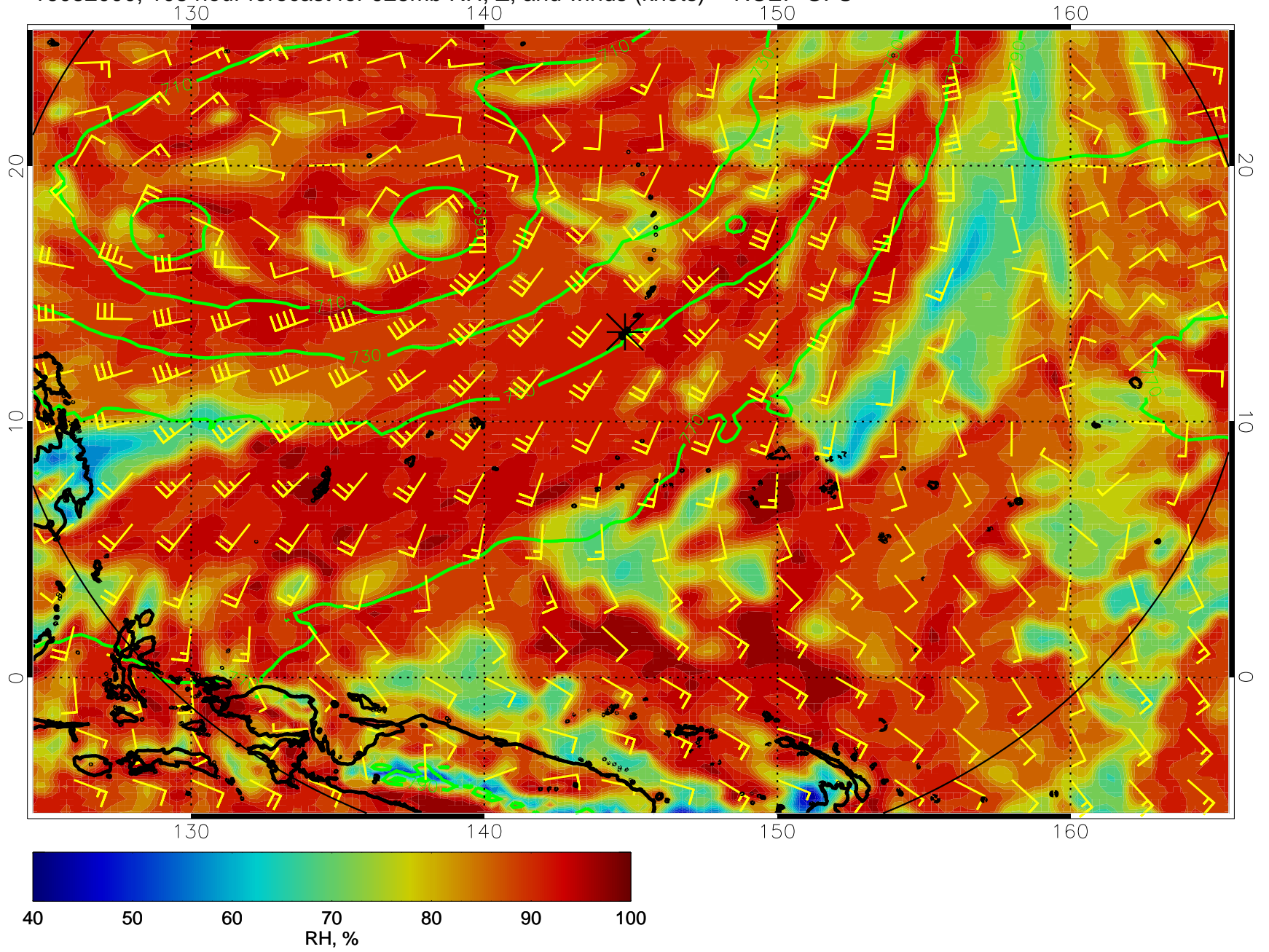
16082000, 108 hour forecast for 925mb RH, Z, and winds (knots) -- NCEP GFS
