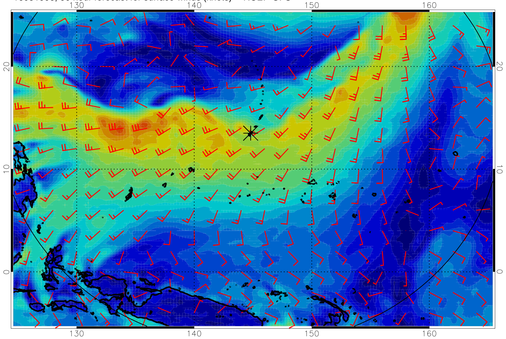
16081906, 90 hour forecast for surface winds (knots) -- NCEP GFS
