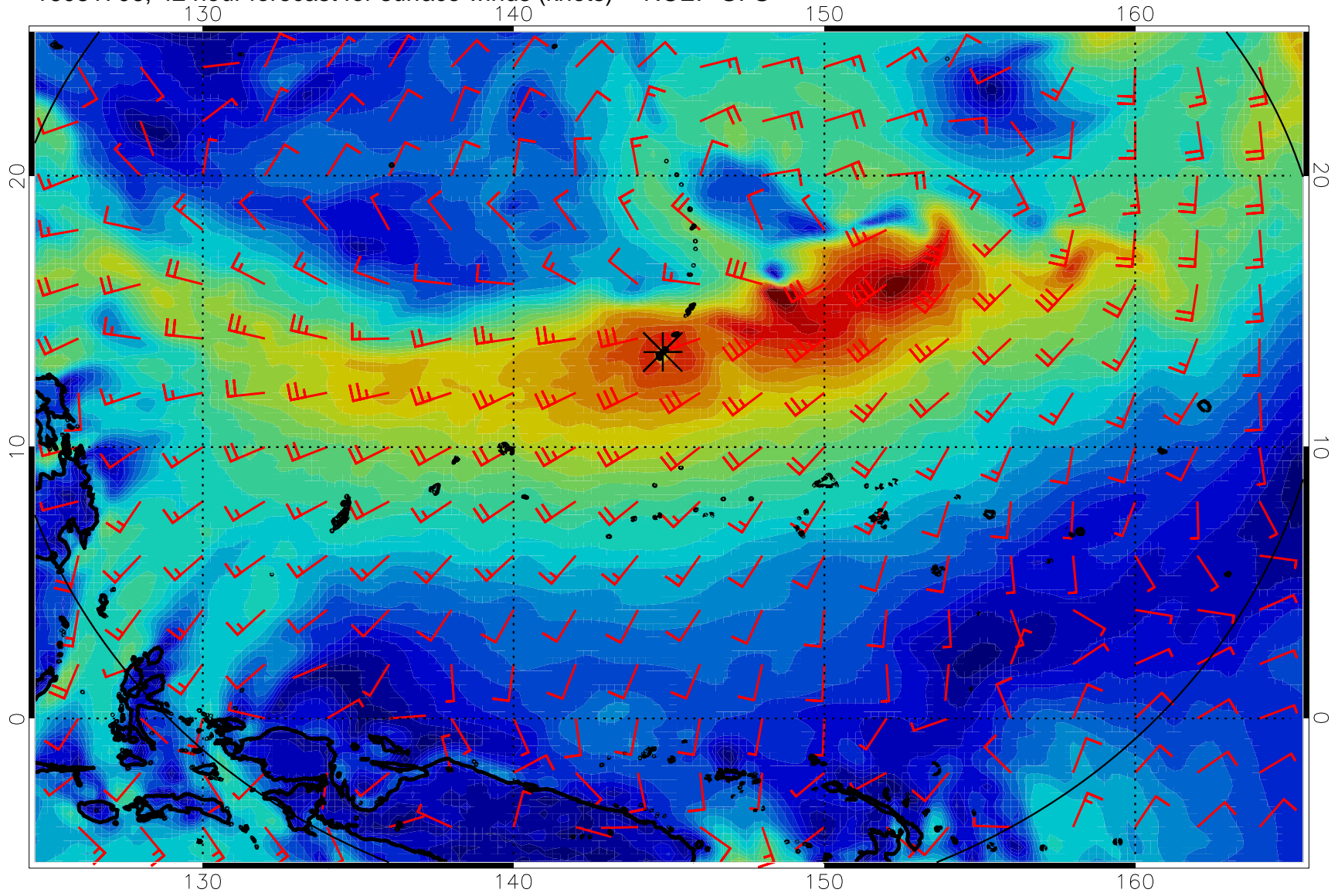
16081706, 42 hour forecast for surface winds (knots) -- NCEP GFS
