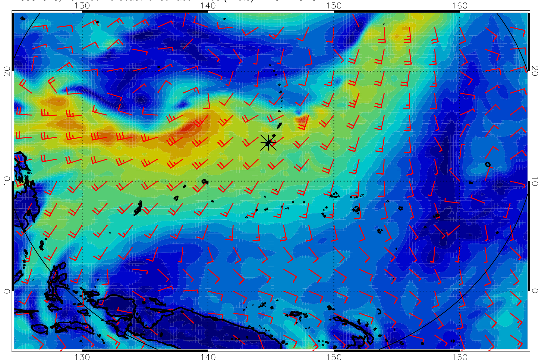
16081918, 102 hour forecast for surface winds (knots) -- NCEP GFS
