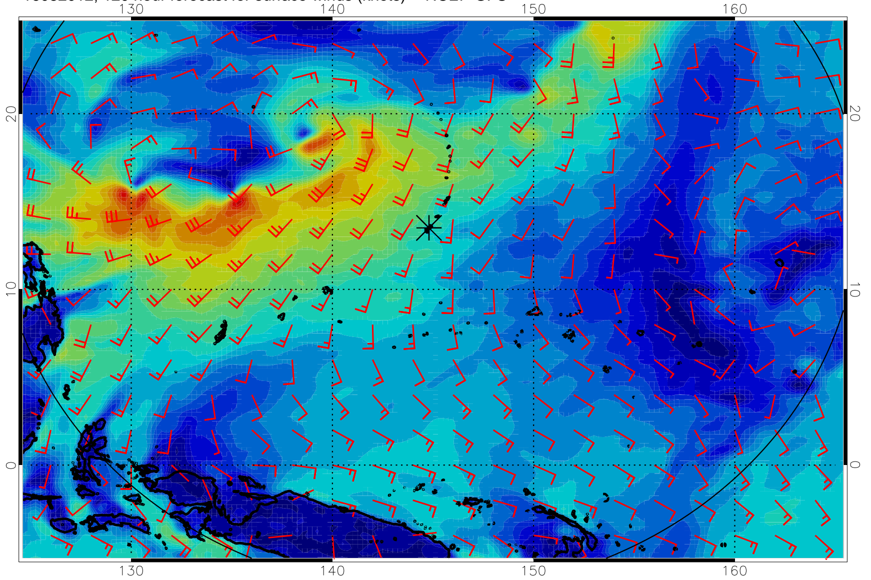
16082012, 120 hour forecast for surface winds (knots) -- NCEP GFS
