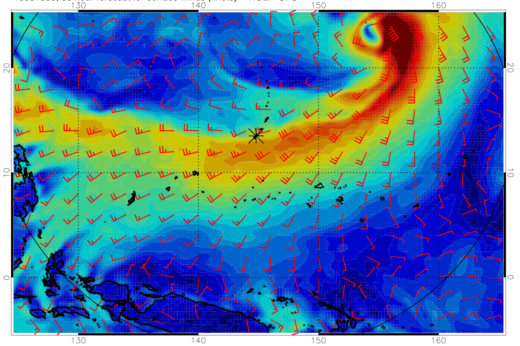
16081806, 66 hour forecast for surface winds (knots) -- NCEP GFS
