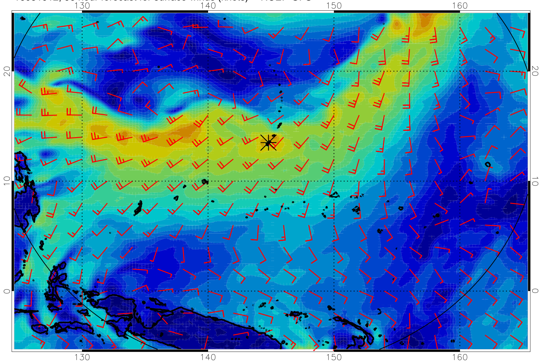
16081912, 96 hour forecast for surface winds (knots) -- NCEP GFS
