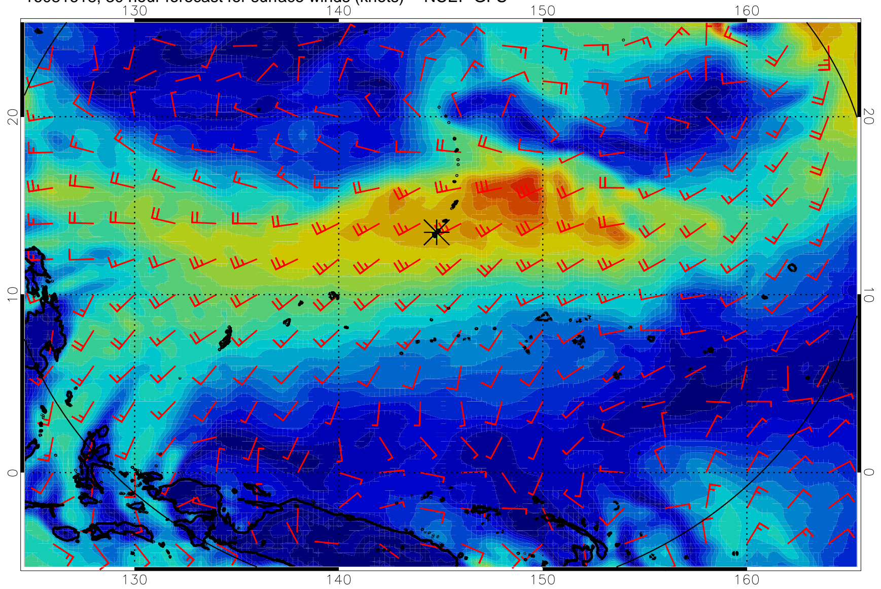
16081618, 30 hour forecast for surface winds (knots) -- NCEP GFS
