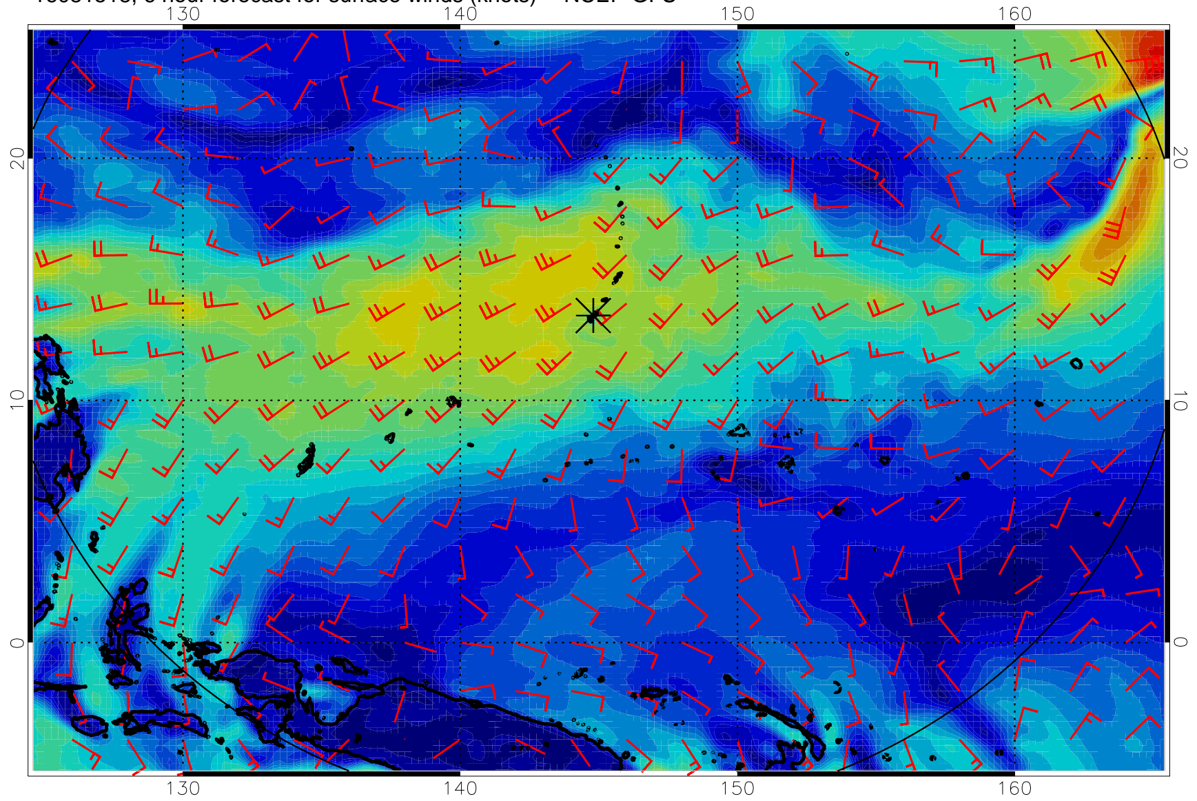
16081518, 6 hour forecast for surface winds (knots) -- NCEP GFS
