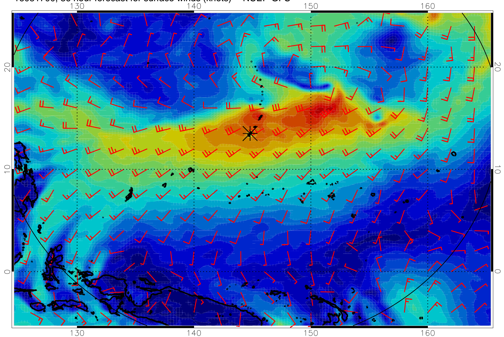
16081700, 36 hour forecast for surface winds (knots) -- NCEP GFS
