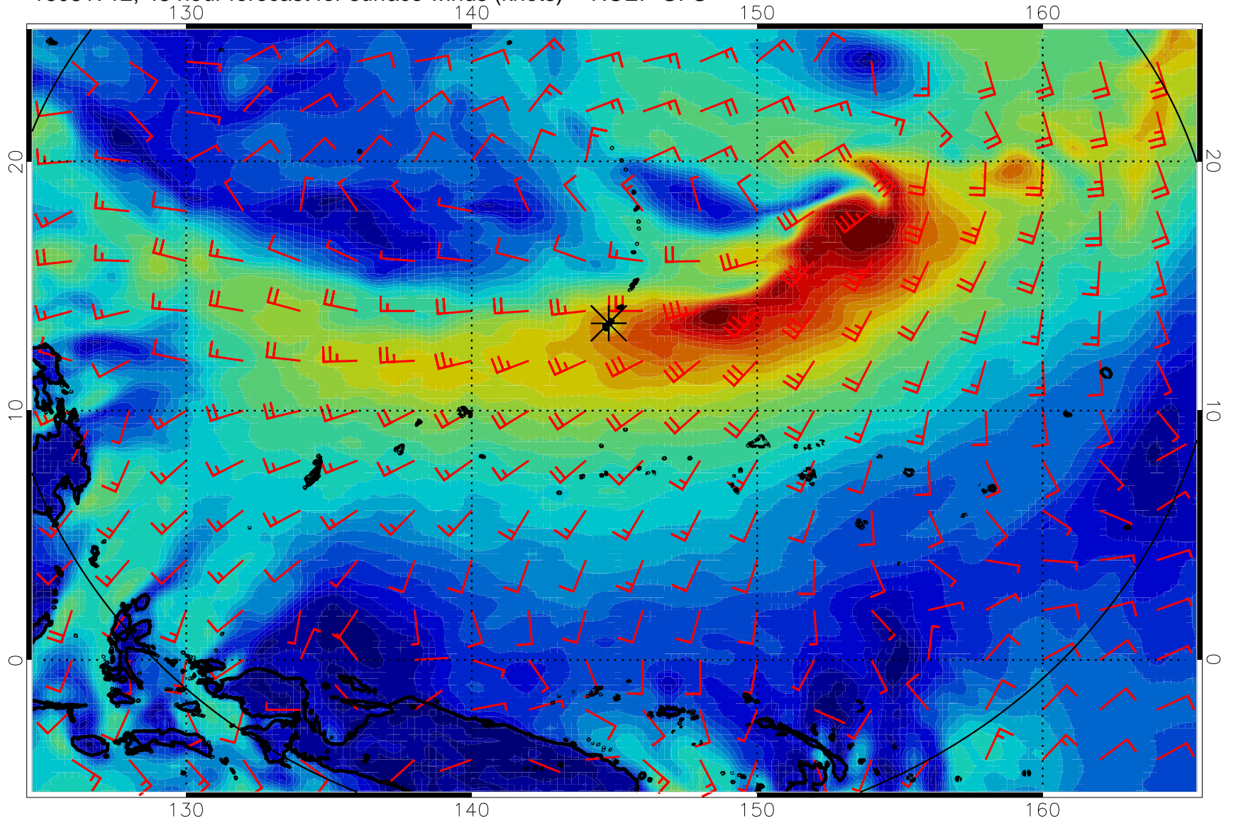
16081712, 48 hour forecast for surface winds (knots) -- NCEP GFS
