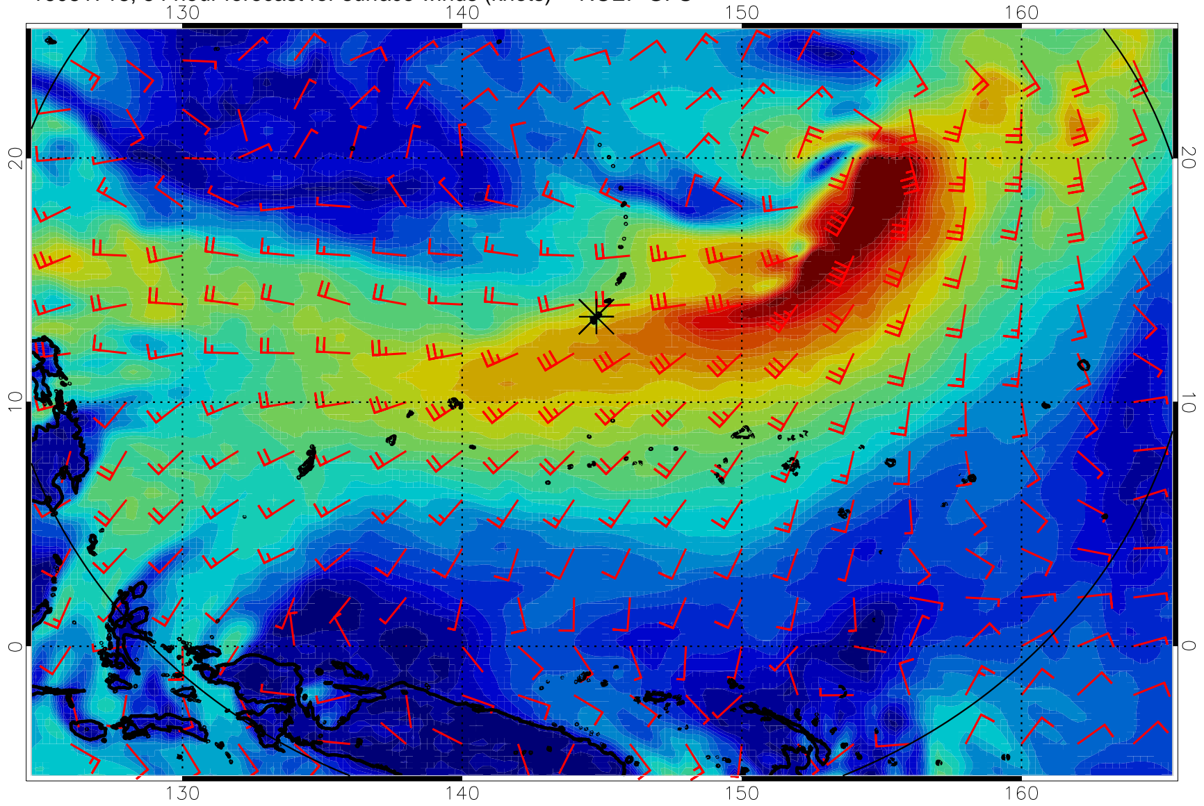
16081718, 54 hour forecast for surface winds (knots) -- NCEP GFS
