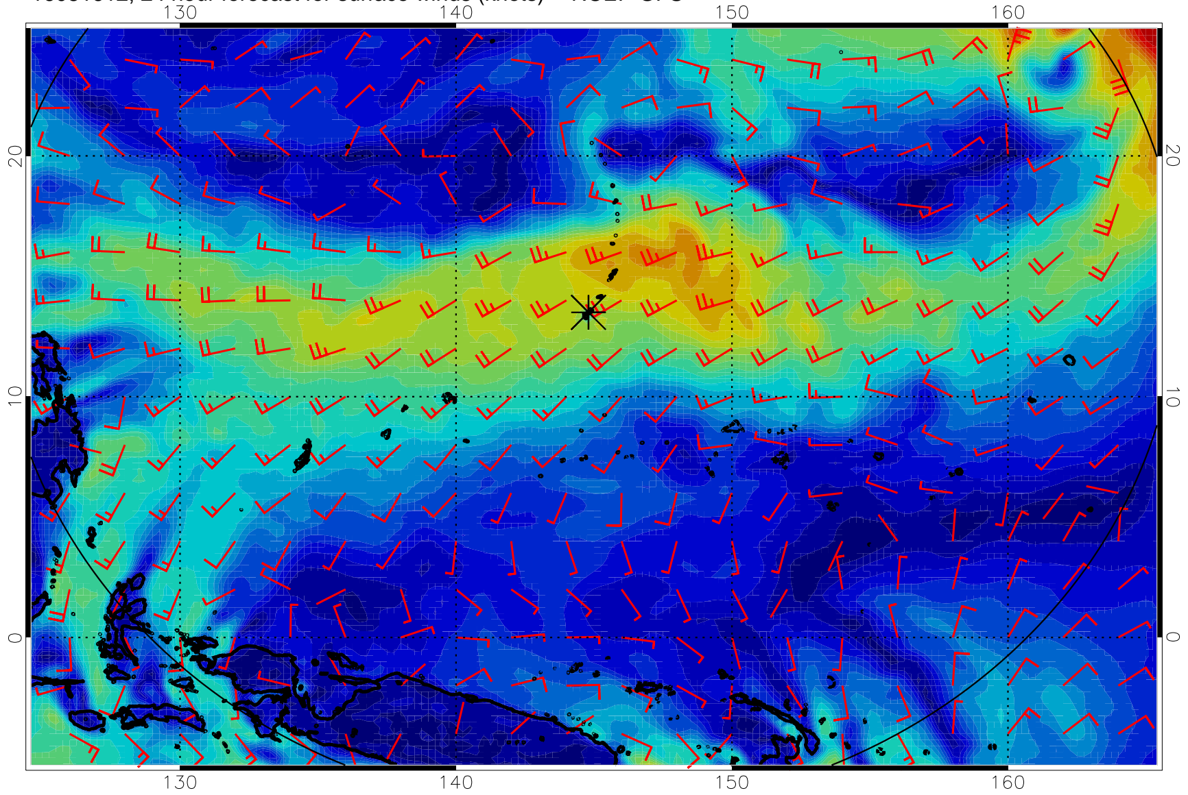
16081612, 24 hour forecast for surface winds (knots) -- NCEP GFS
