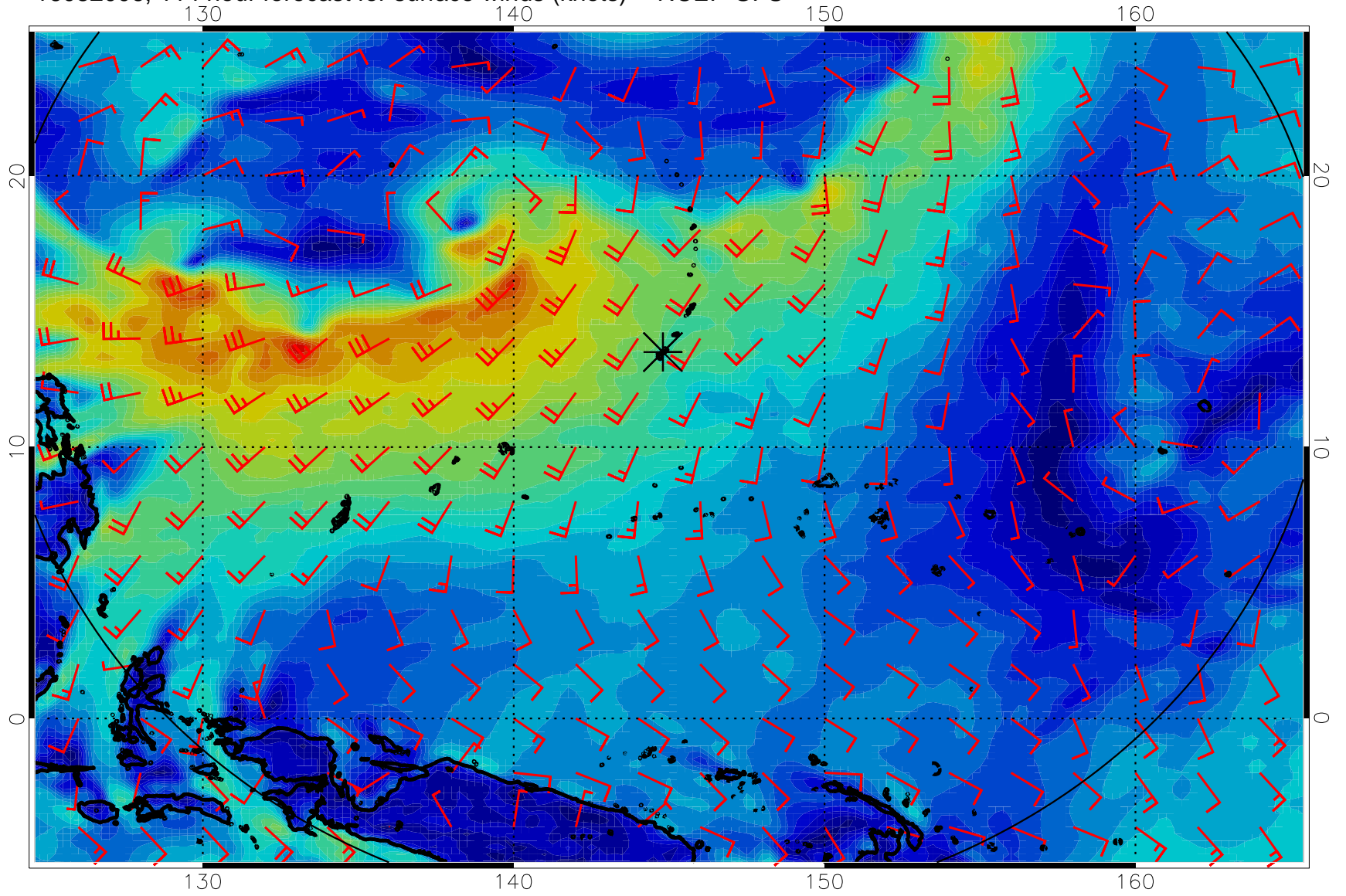
16082006, 114 hour forecast for surface winds (knots) -- NCEP GFS
