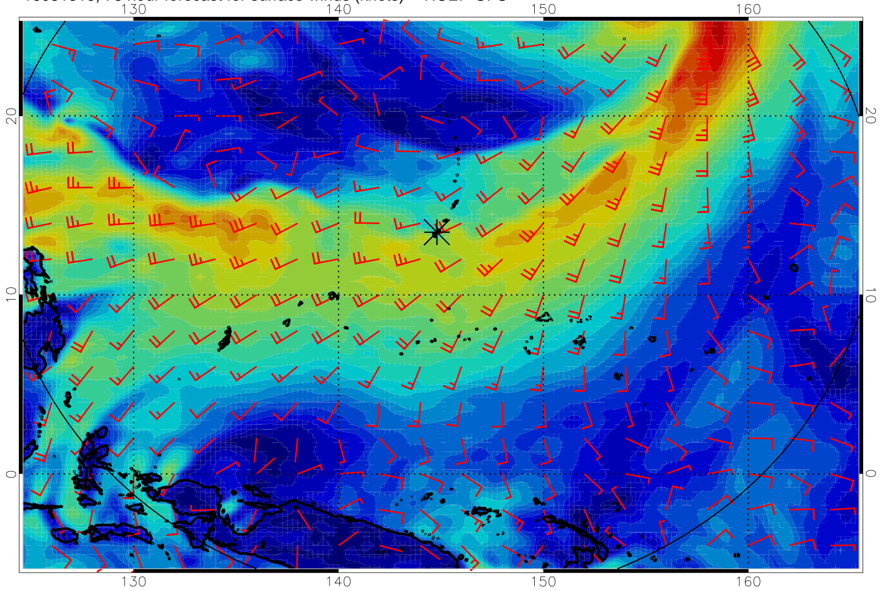
16081818, 78 hour forecast for surface winds (knots) -- NCEP GFS
