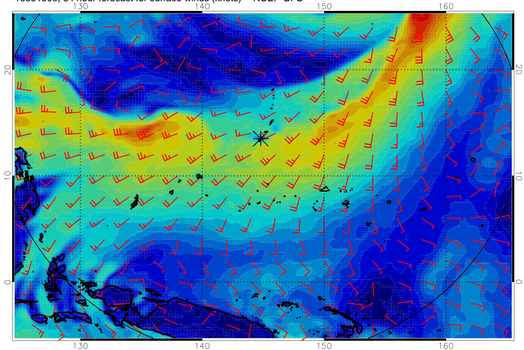
16081900, 84 hour forecast for surface winds (knots) -- NCEP GFS
