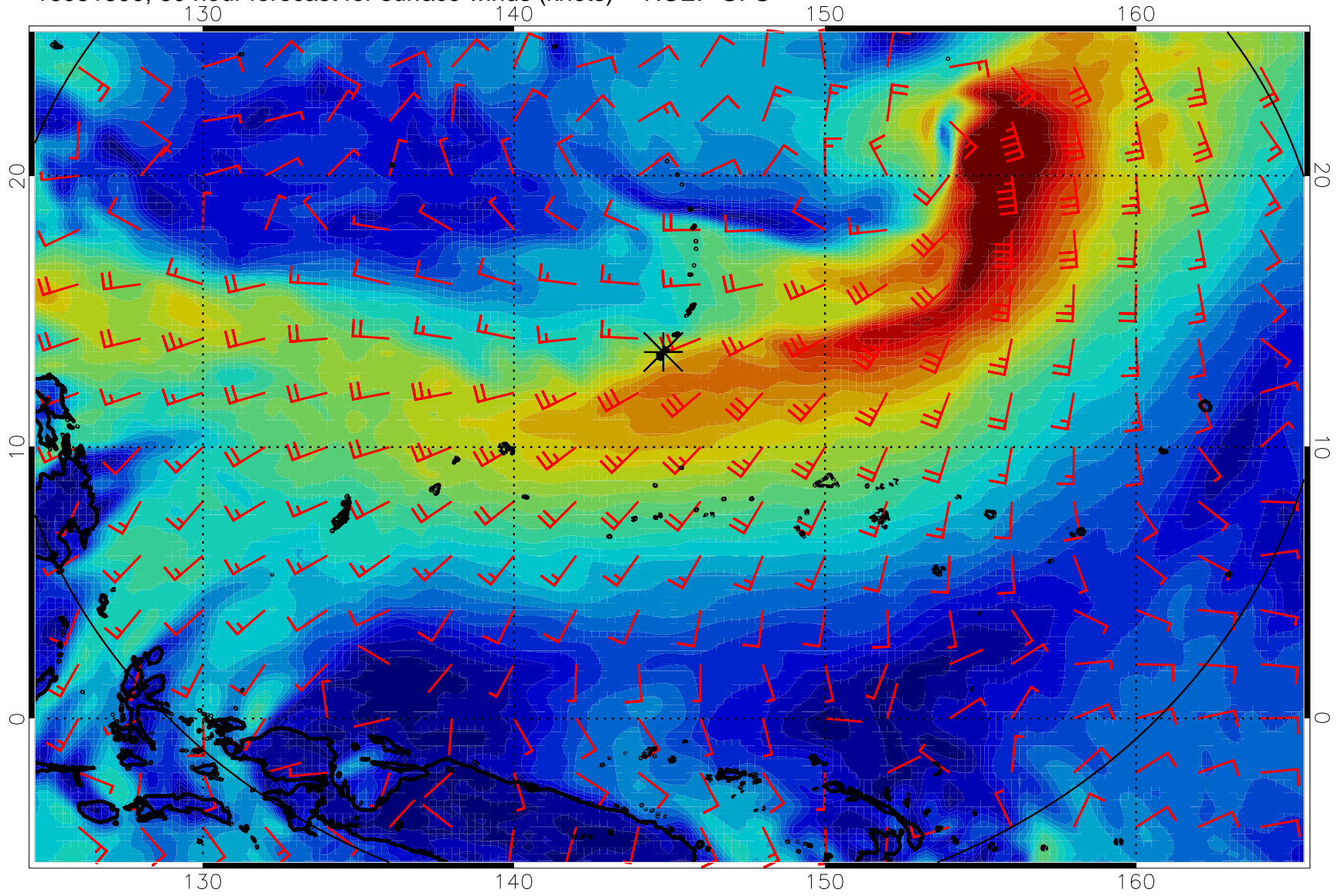
16081800, 60 hour forecast for surface winds (knots) -- NCEP GFS
