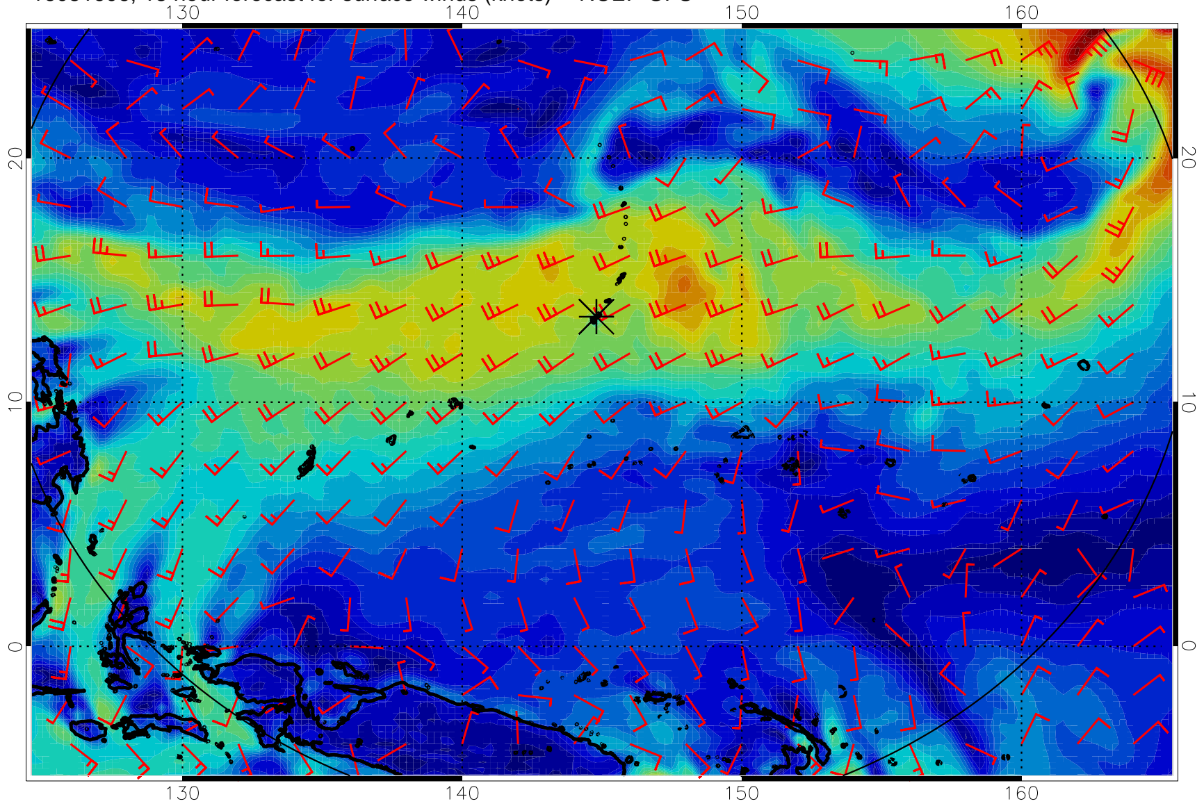
16081606, 18 hour forecast for surface winds (knots) -- NCEP GFS
