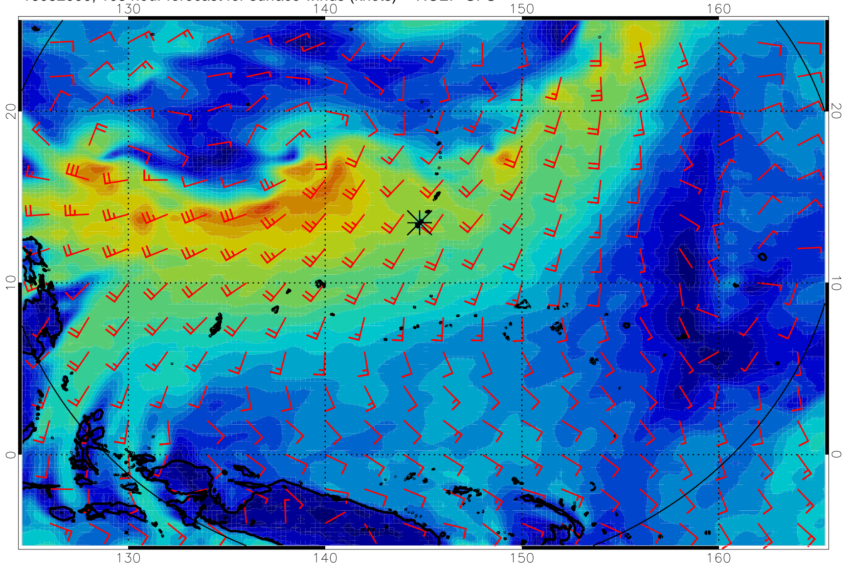
16082000, 108 hour forecast for surface winds (knots) -- NCEP GFS
