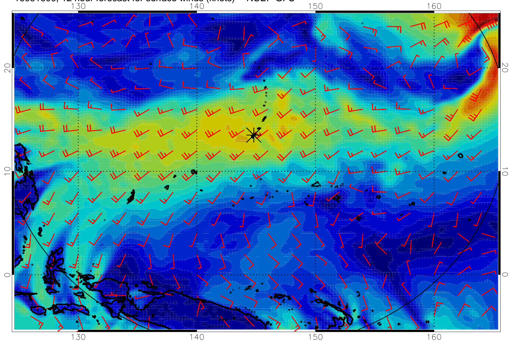
16081600, 12 hour forecast for surface winds (knots) -- NCEP GFS
