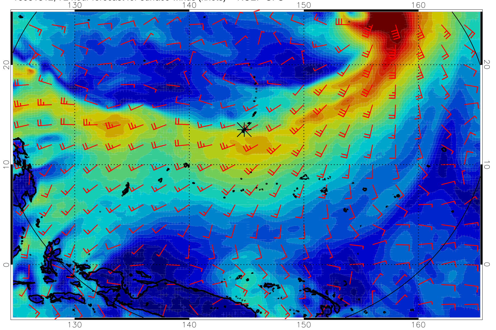
16081812, 72 hour forecast for surface winds (knots) -- NCEP GFS
