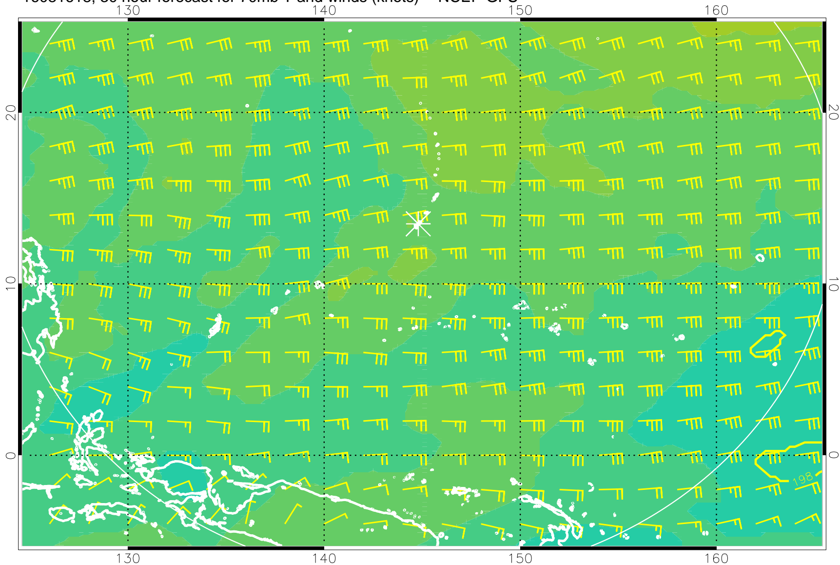
16081618, 30 hour forecast for 70mb T and winds (knots) -- NCEP GFS
