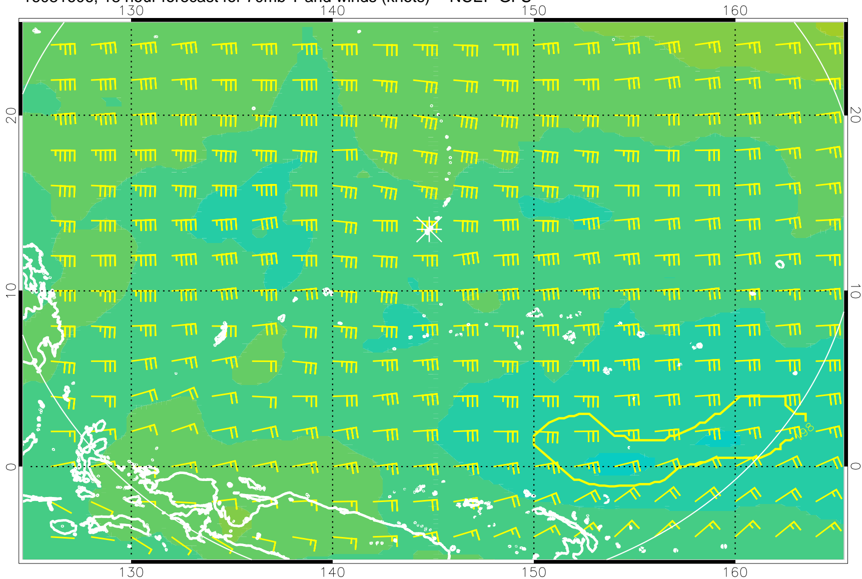
16081606, 18 hour forecast for 70mb T and winds (knots) -- NCEP GFS
