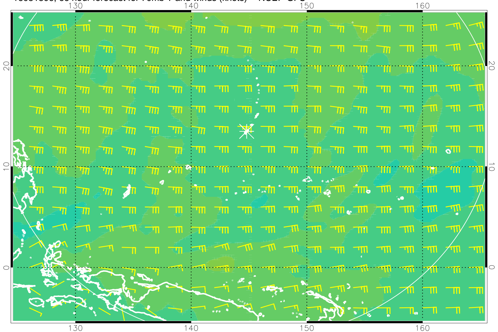
16081806, 66 hour forecast for 70mb T and winds (knots) -- NCEP GFS
