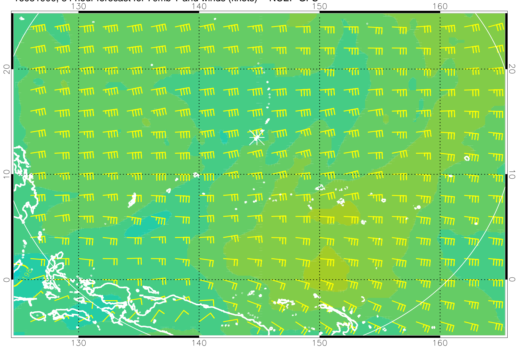
16081900, 84 hour forecast for 70mb T and winds (knots) -- NCEP GFS
