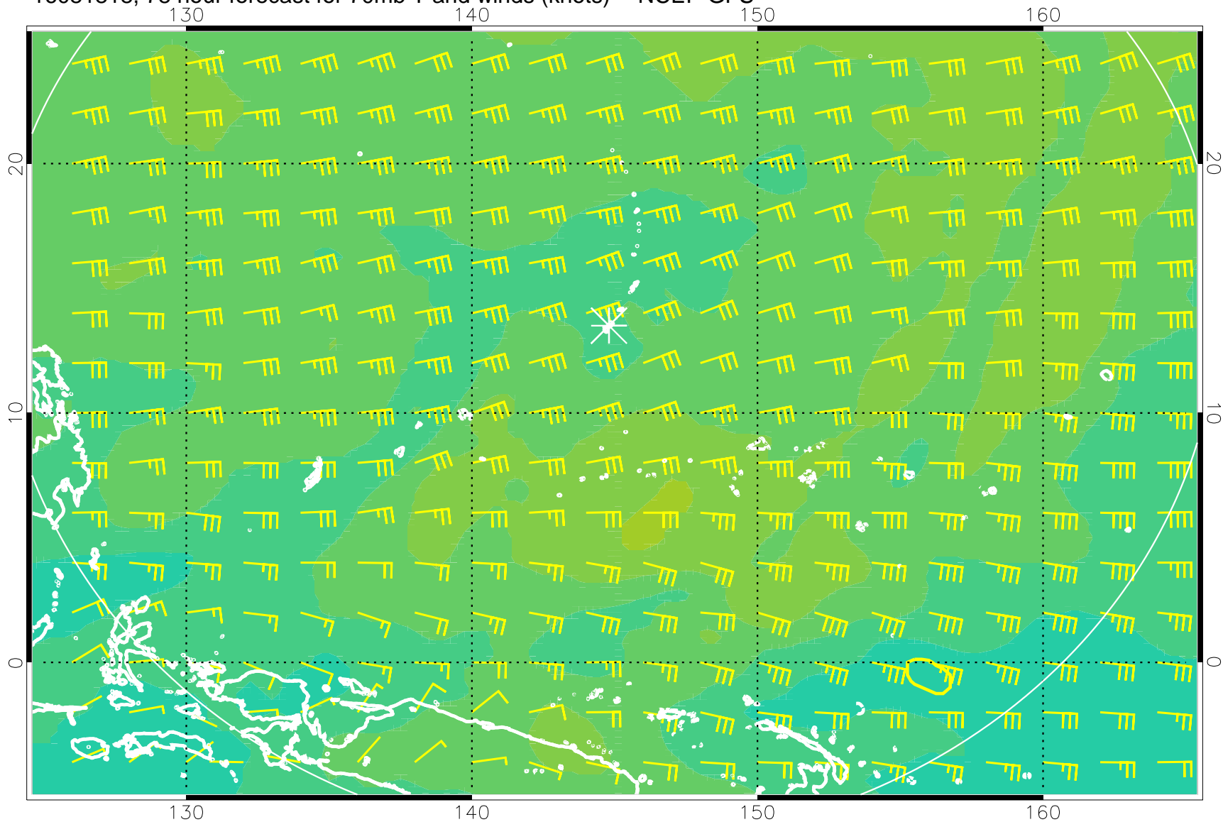
16081818, 78 hour forecast for 70mb T and winds (knots) -- NCEP GFS
