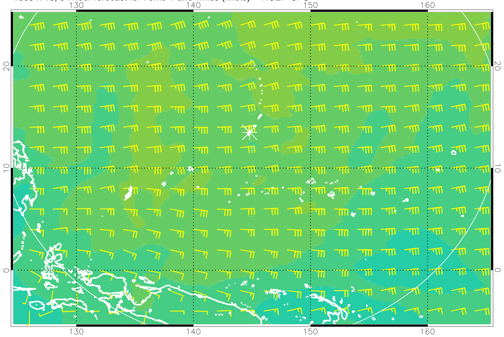
16081718, 54 hour forecast for 70mb T and winds (knots) -- NCEP GFS
