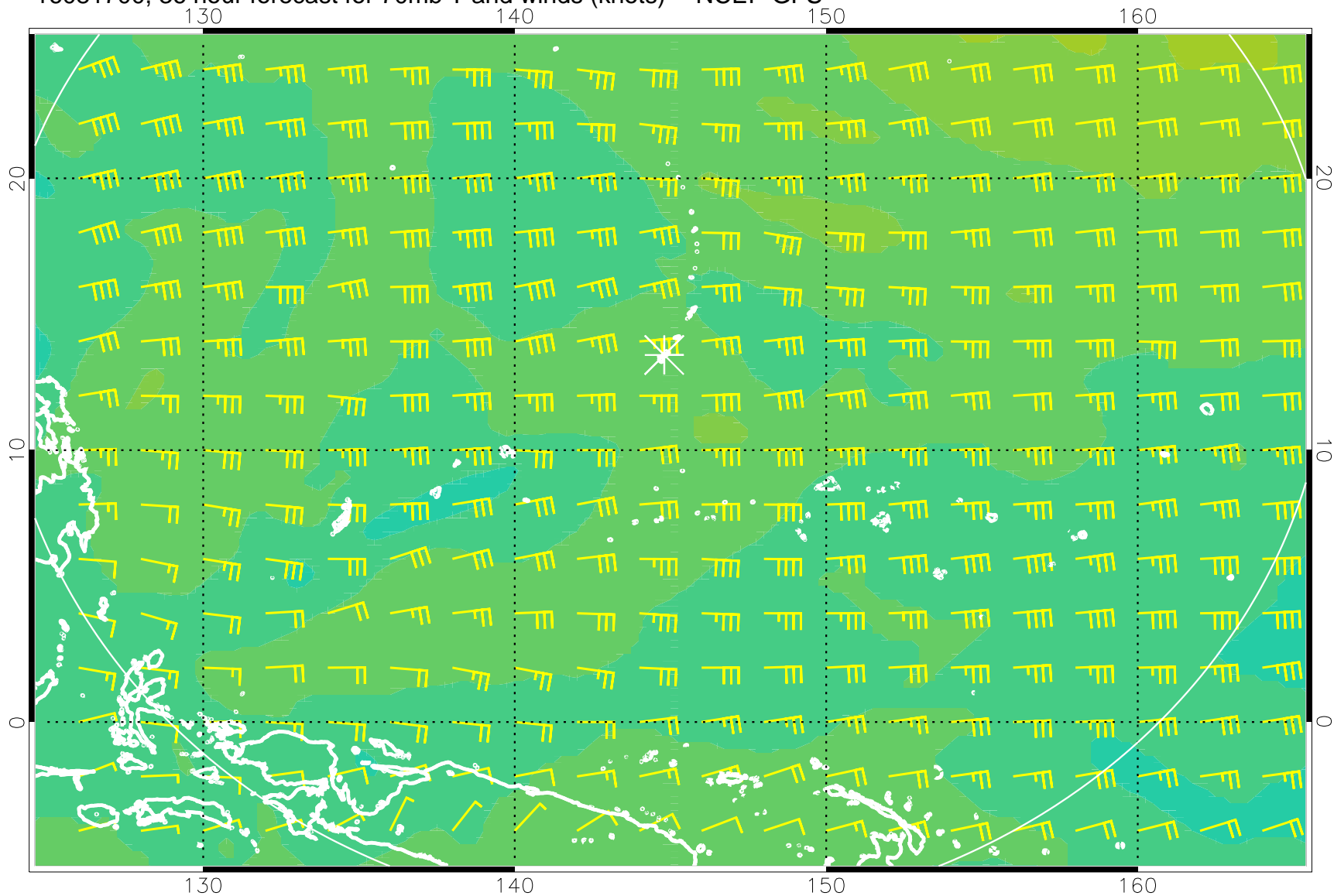
16081700, 36 hour forecast for 70mb T and winds (knots) -- NCEP GFS
