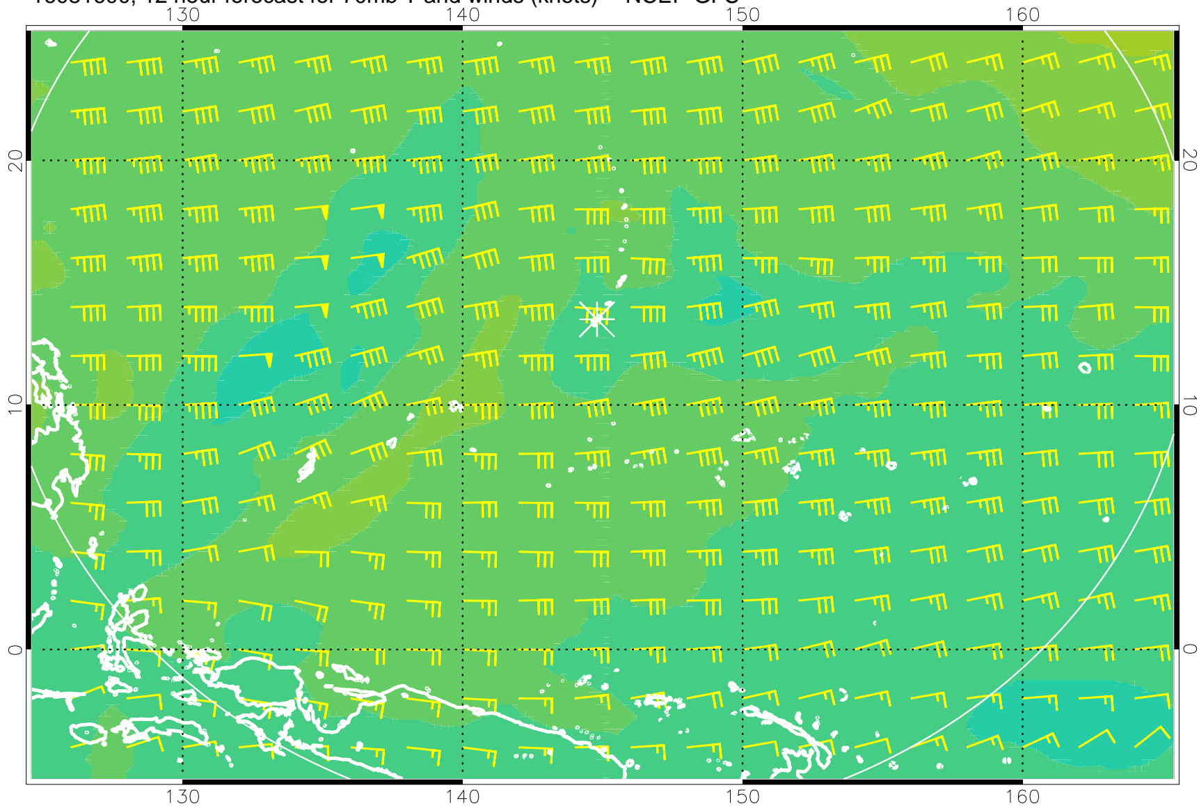
16081600, 12 hour forecast for 70mb T and winds (knots) -- NCEP GFS
