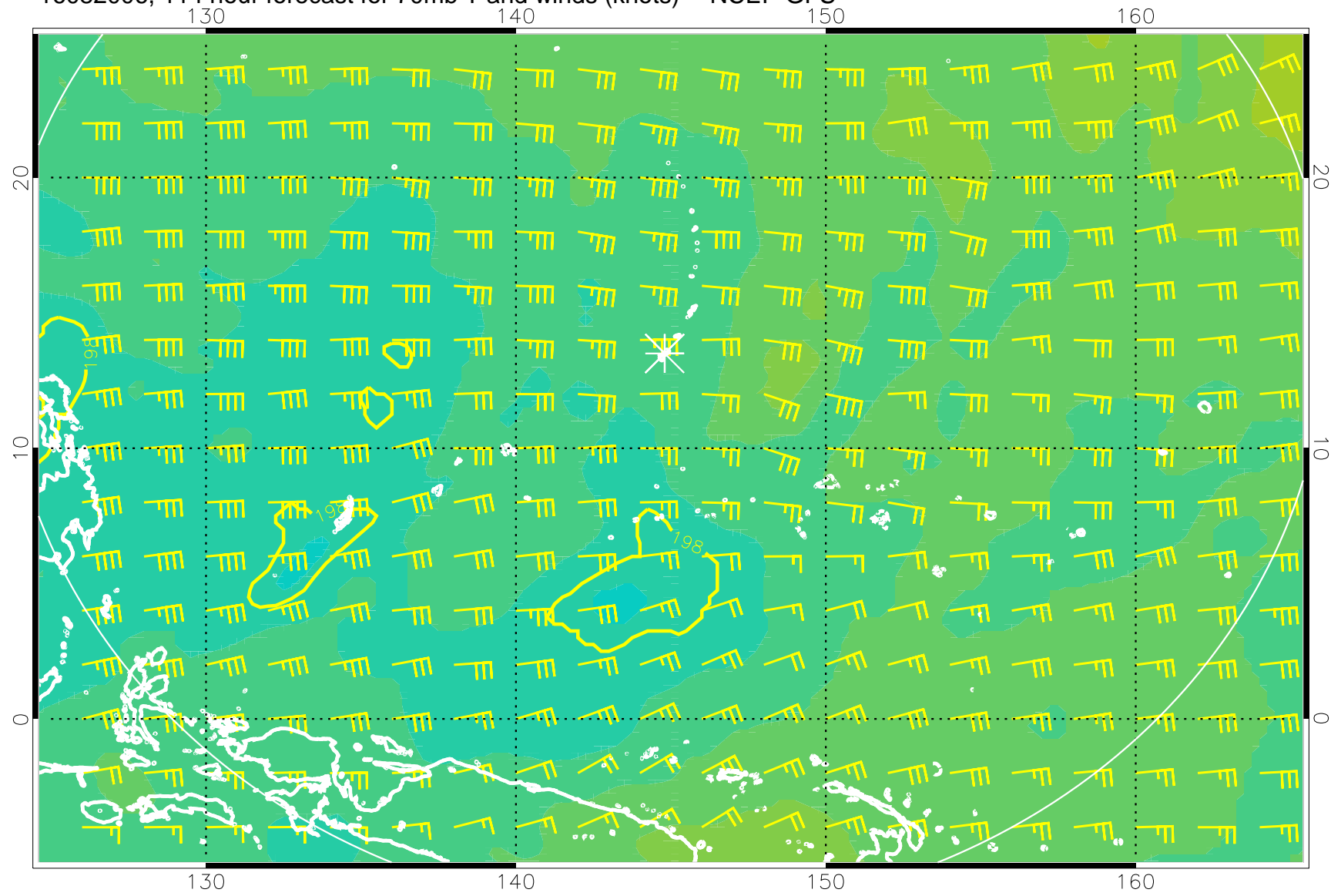
16082006, 114 hour forecast for 70mb T and winds (knots) -- NCEP GFS
