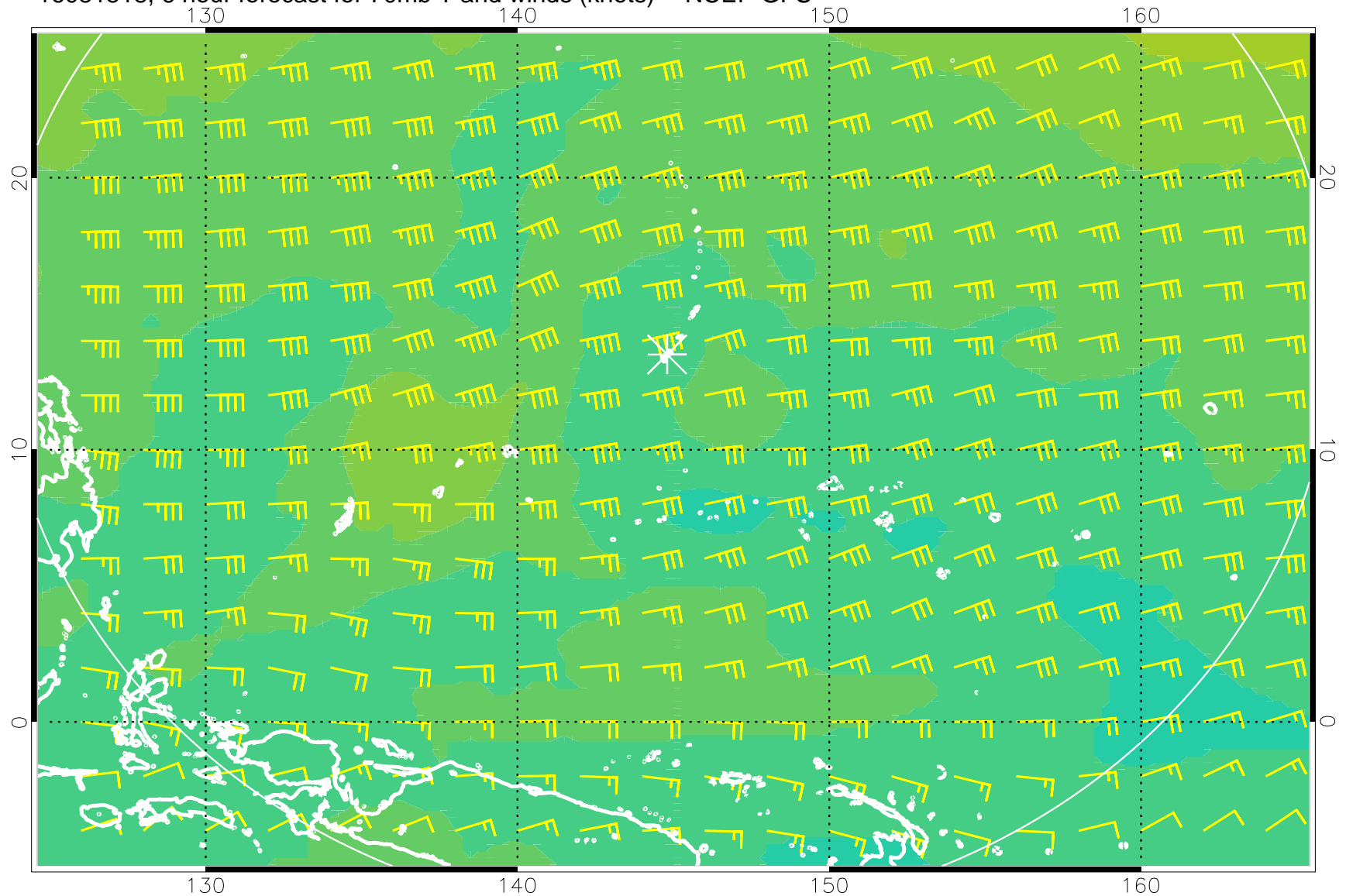
16081518, 6 hour forecast for 70mb T and winds (knots) -- NCEP GFS
