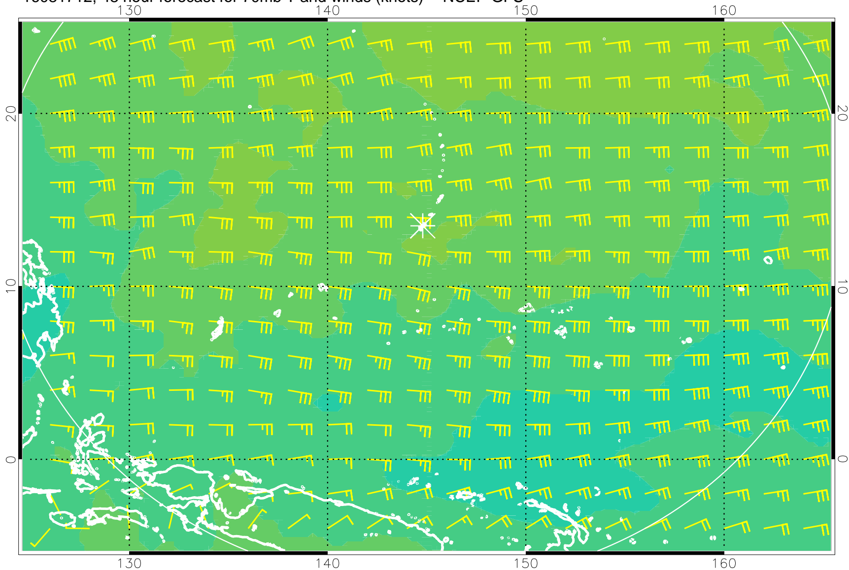
16081712, 48 hour forecast for 70mb T and winds (knots) -- NCEP GFS
