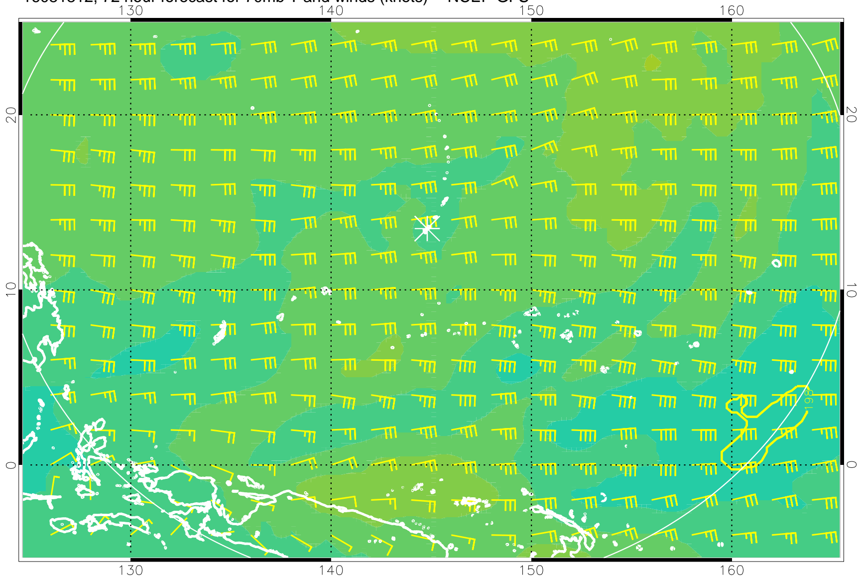
16081812, 72 hour forecast for 70mb T and winds (knots) -- NCEP GFS
