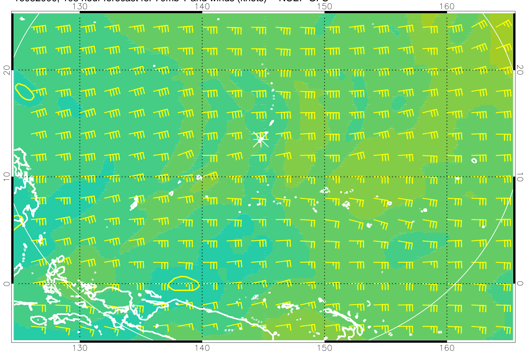
16082000, 108 hour forecast for 70mb T and winds (knots) -- NCEP GFS
