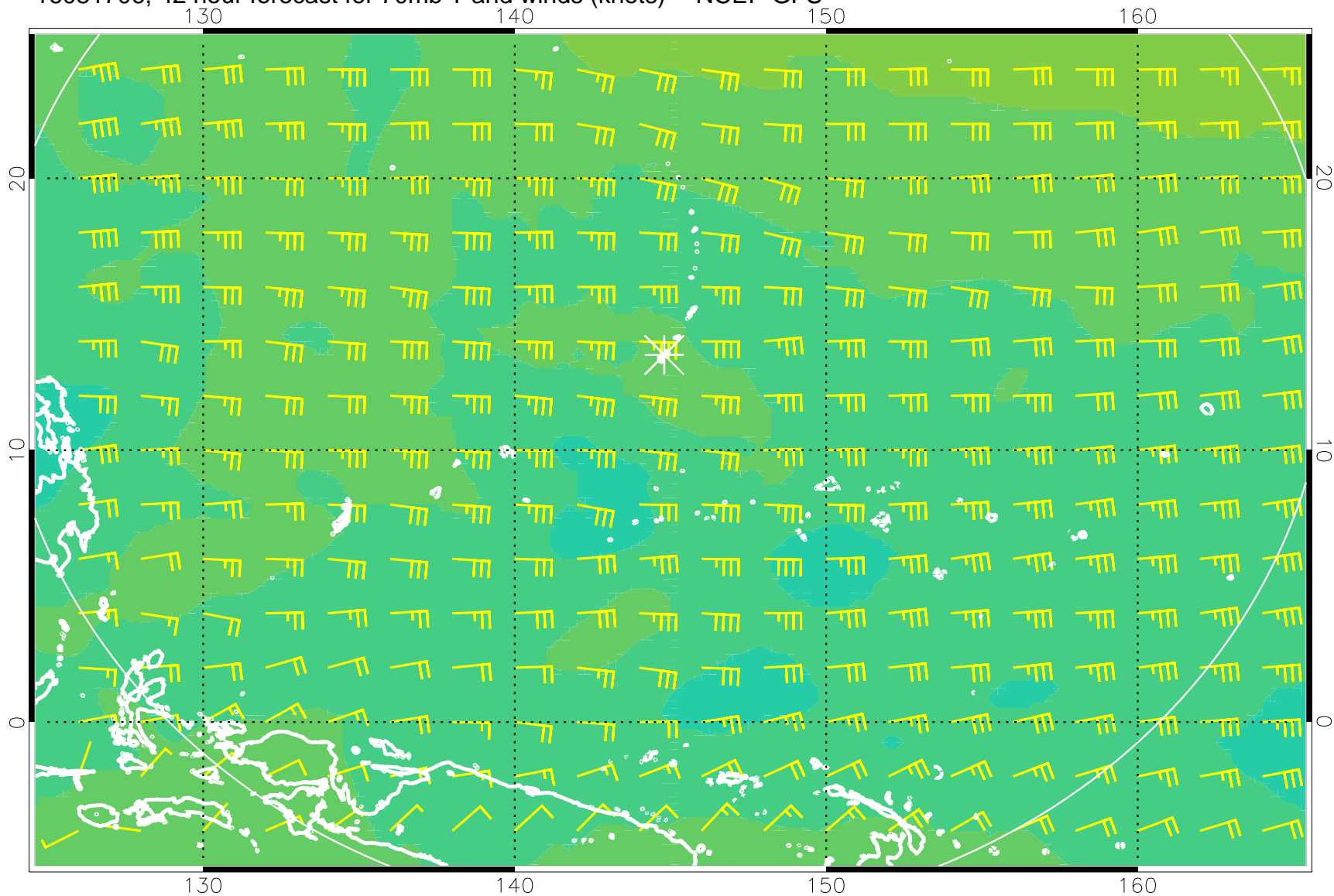
16081706, 42 hour forecast for 70mb T and winds (knots) -- NCEP GFS
