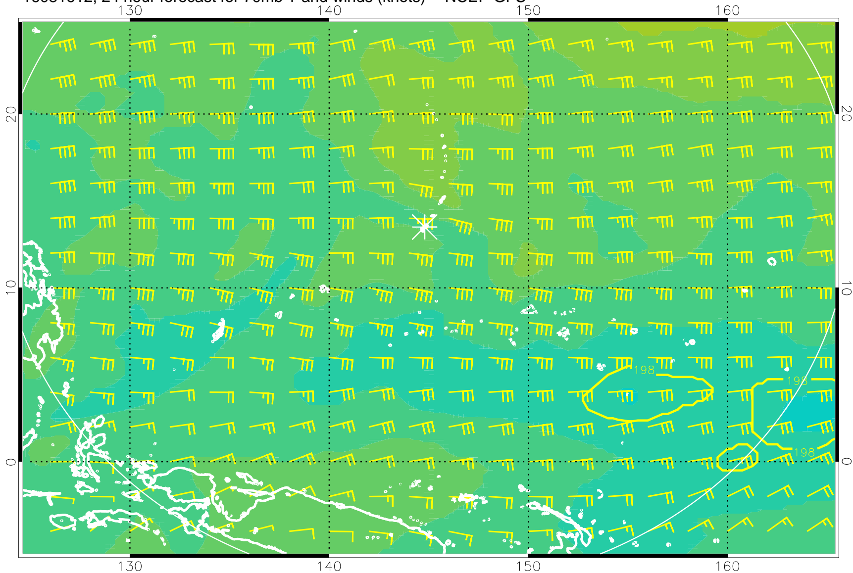
16081612, 24 hour forecast for 70mb T and winds (knots) -- NCEP GFS
