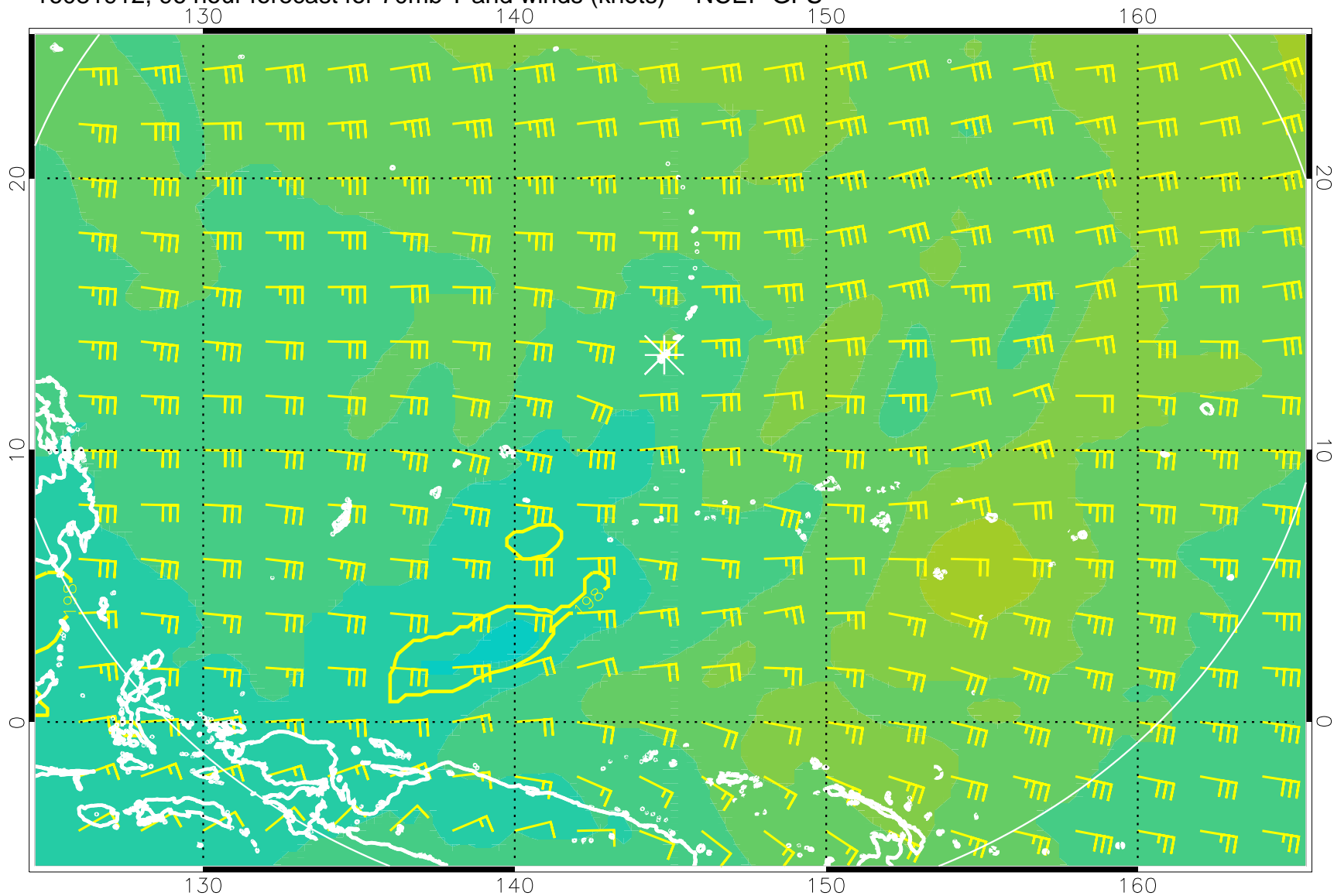
16081912, 96 hour forecast for 70mb T and winds (knots) -- NCEP GFS
