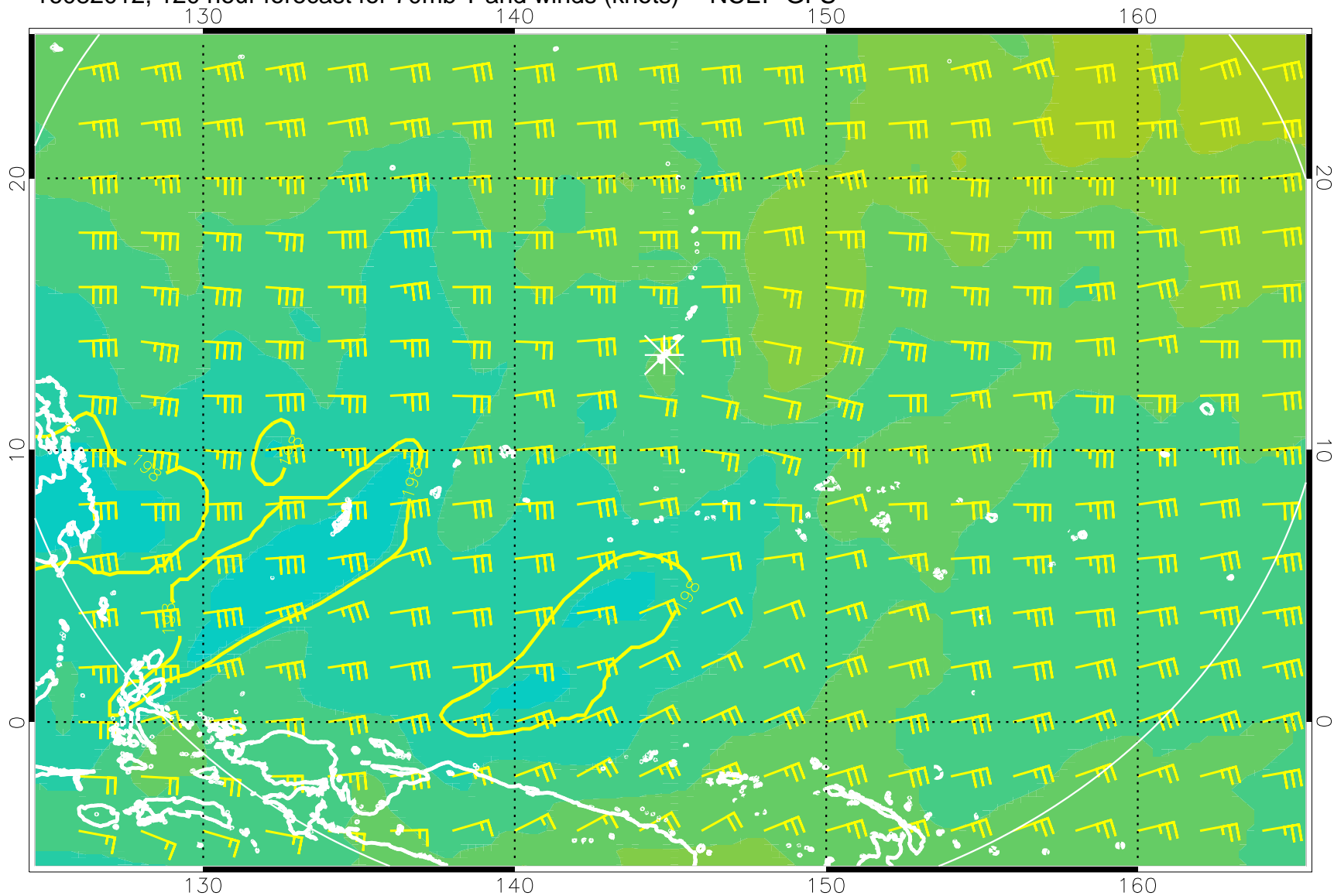
16082012, 120 hour forecast for 70mb T and winds (knots) -- NCEP GFS
