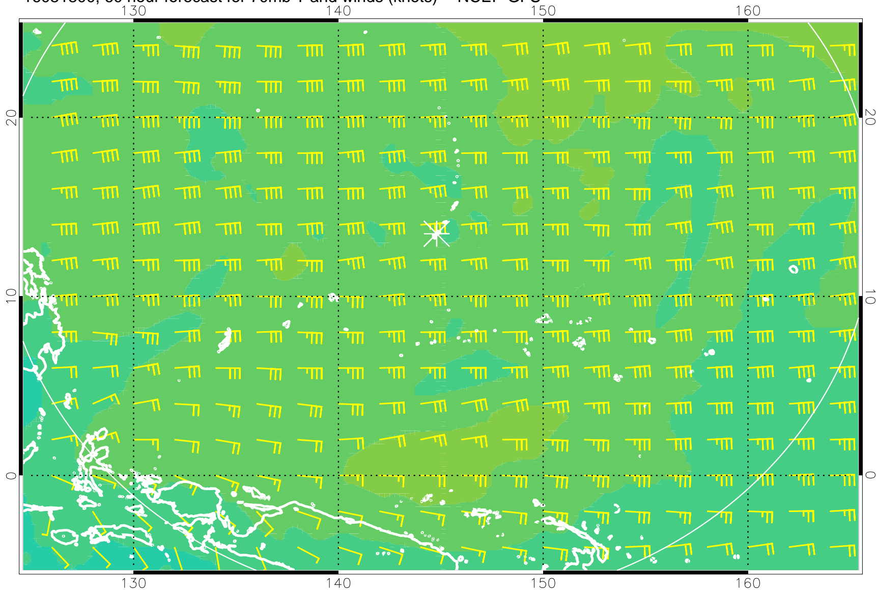
16081800, 60 hour forecast for 70mb T and winds (knots) -- NCEP GFS
