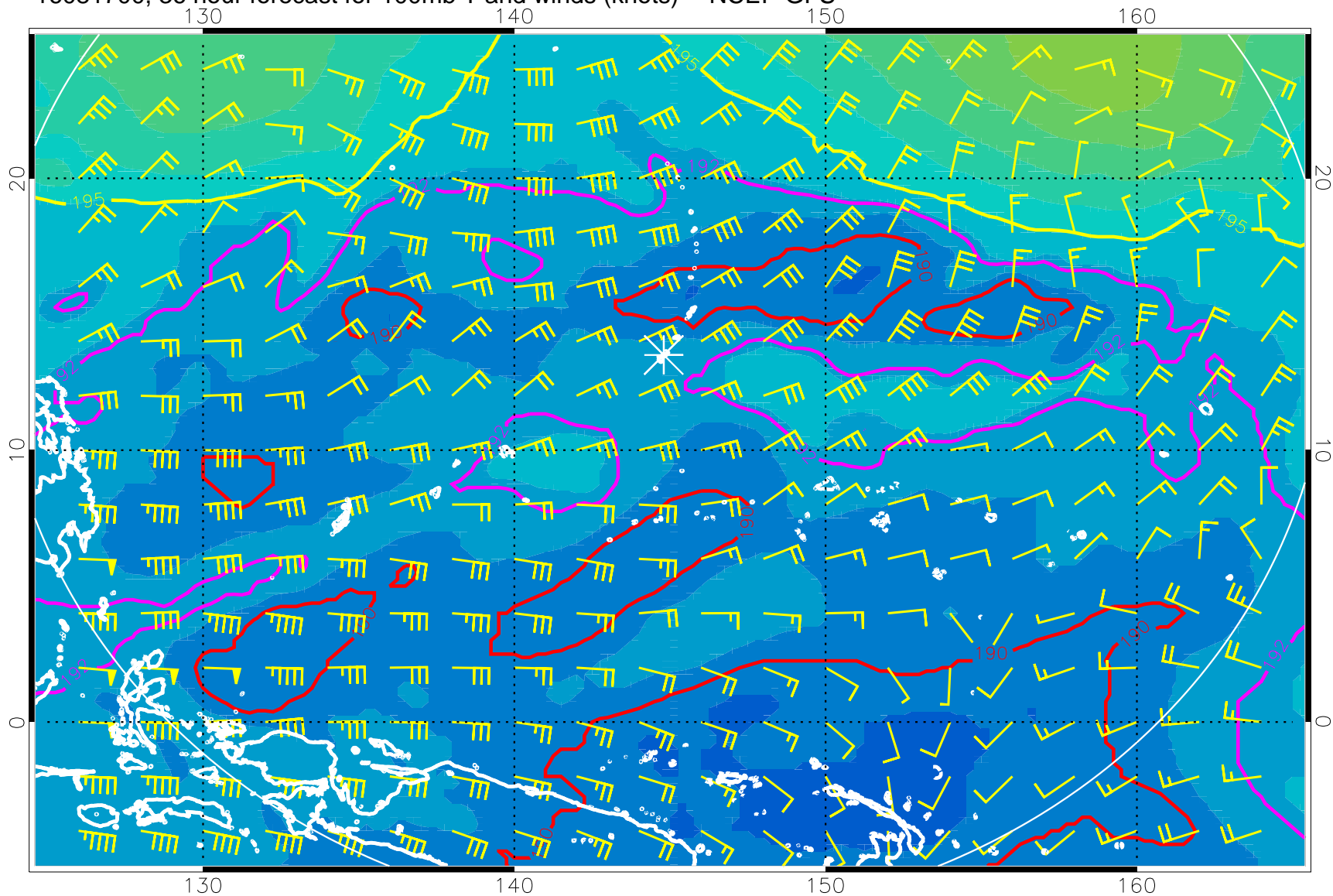
16081700, 36 hour forecast for 100mb T and winds (knots) -- NCEP GFS
