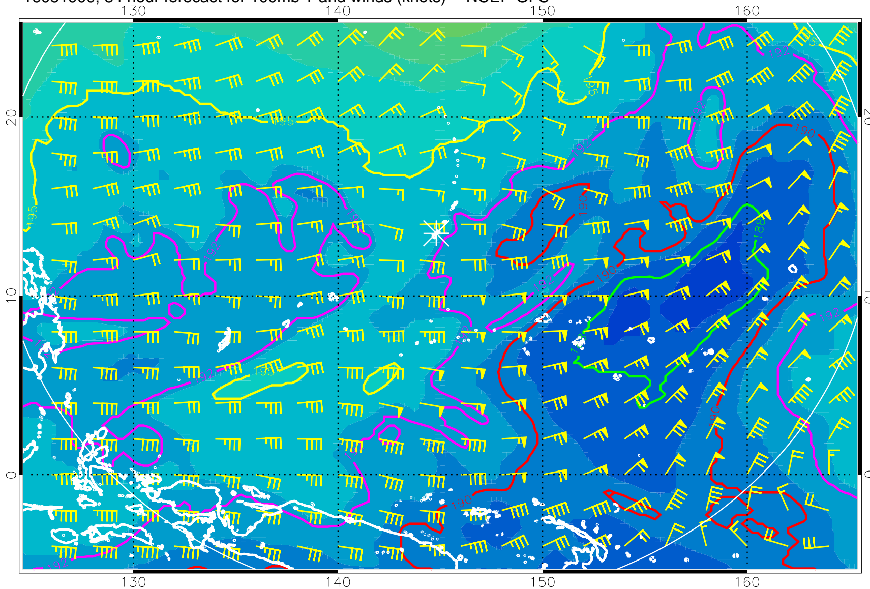
16081900, 84 hour forecast for 100mb T and winds (knots) -- NCEP GFS
