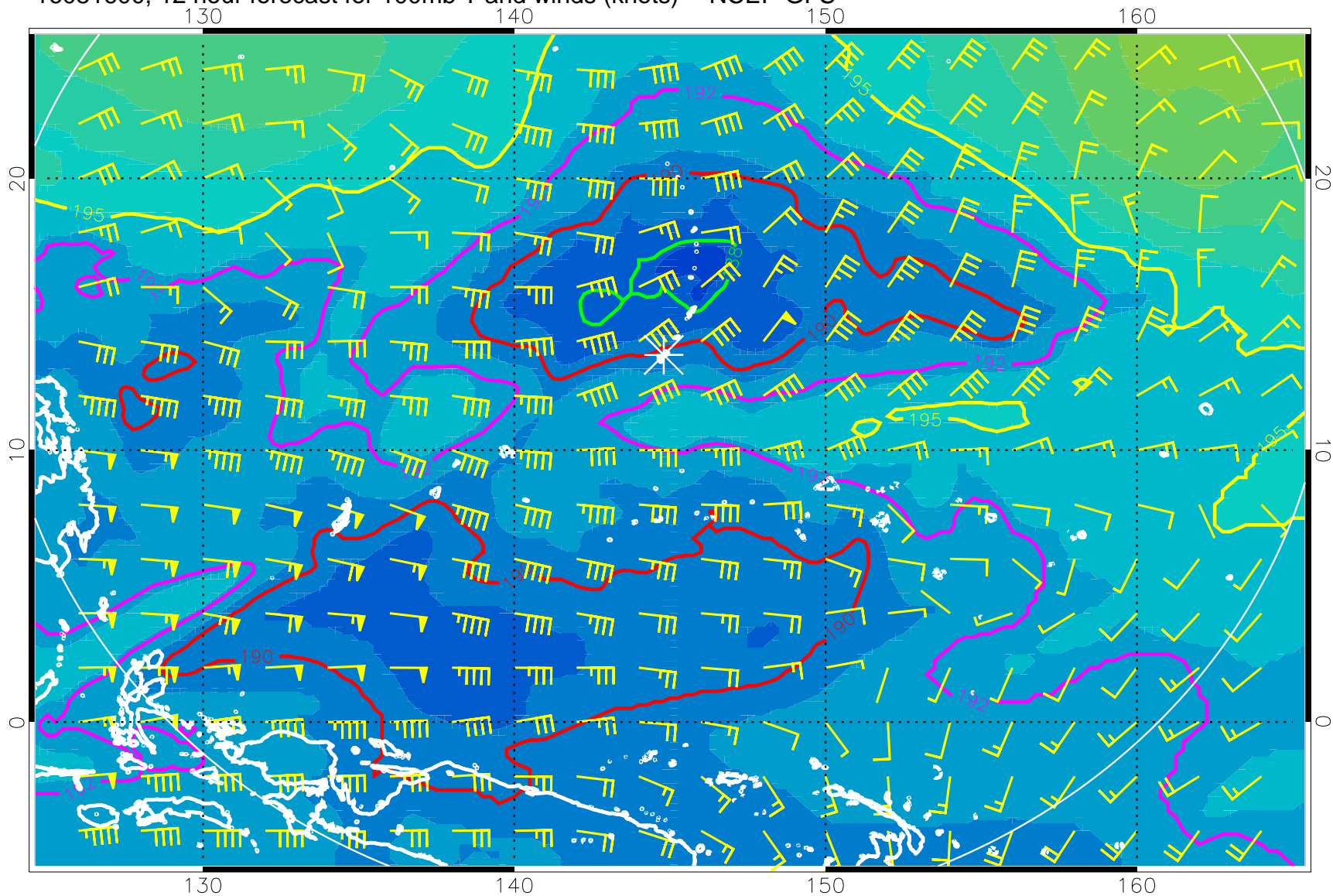
16081600, 12 hour forecast for 100mb T and winds (knots) -- NCEP GFS
