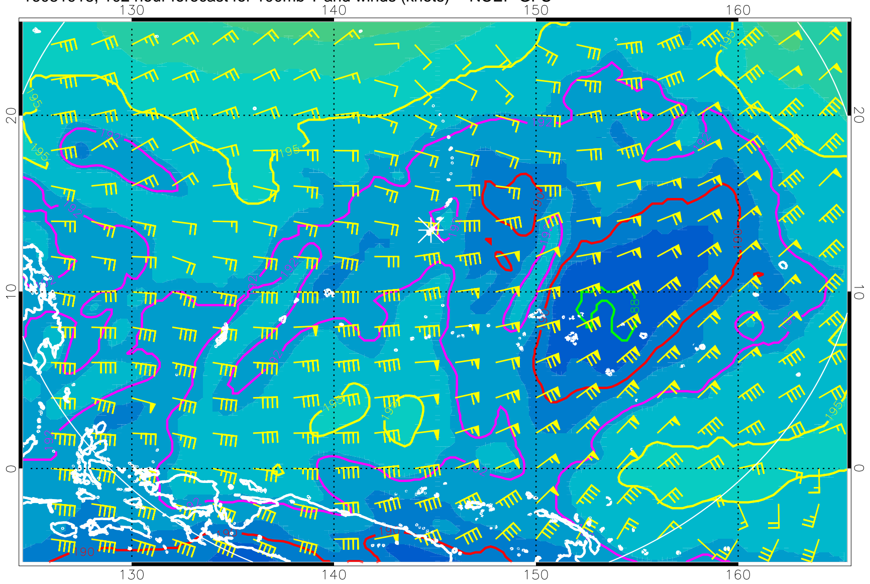
16081918, 102 hour forecast for 100mb T and winds (knots) -- NCEP GFS
