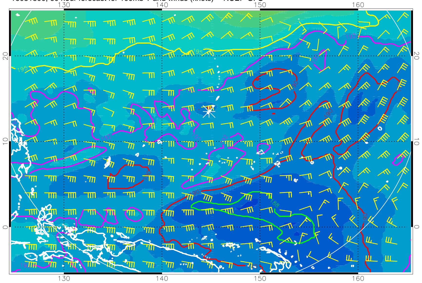
16081800, 60 hour forecast for 100mb T and winds (knots) -- NCEP GFS
