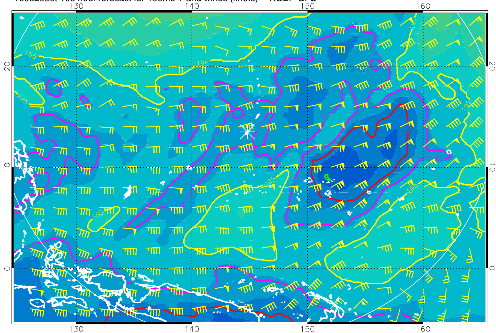
16082000, 108 hour forecast for 100mb T and winds (knots) -- NCEP GFS
