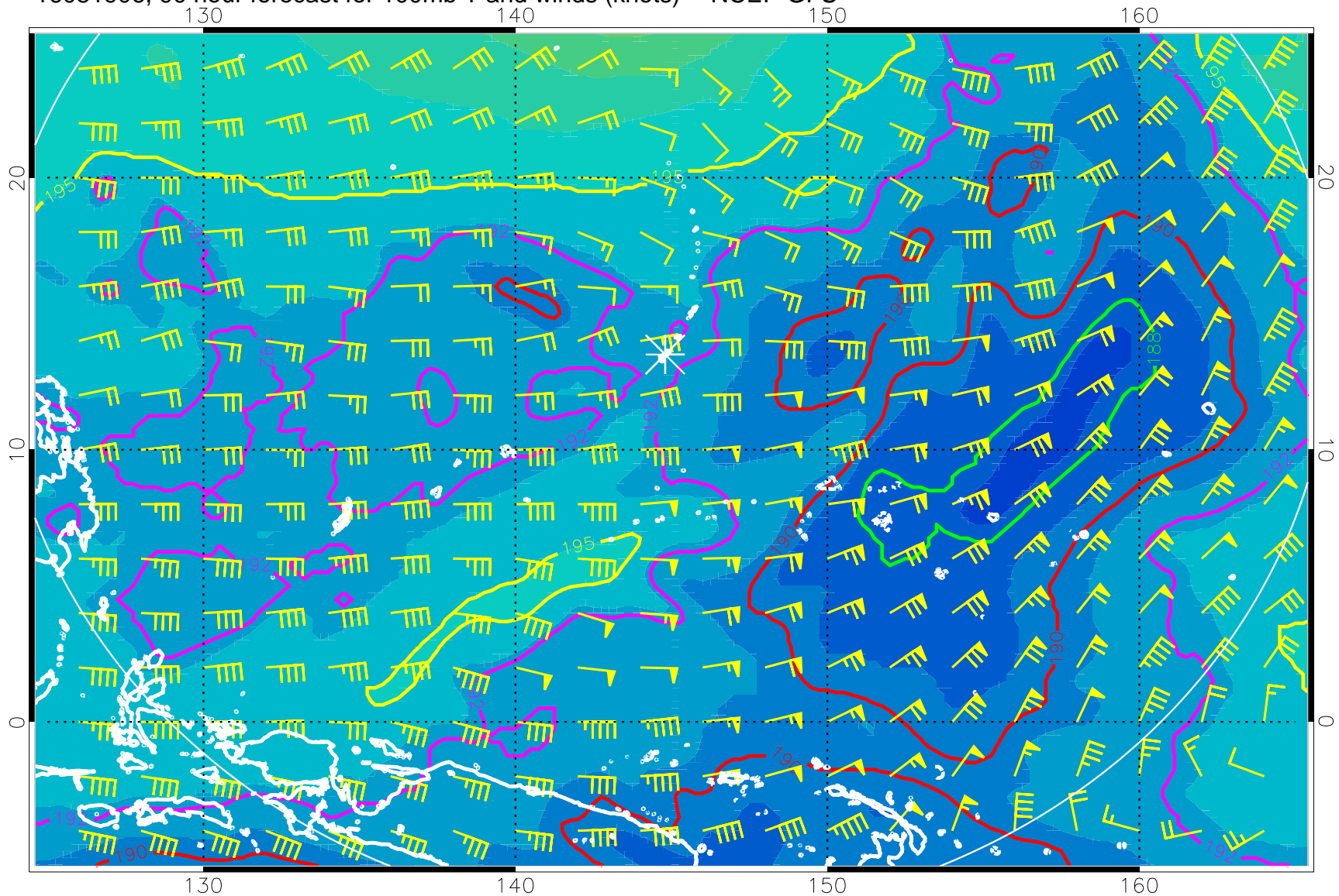
16081906, 90 hour forecast for 100mb T and winds (knots) -- NCEP GFS
