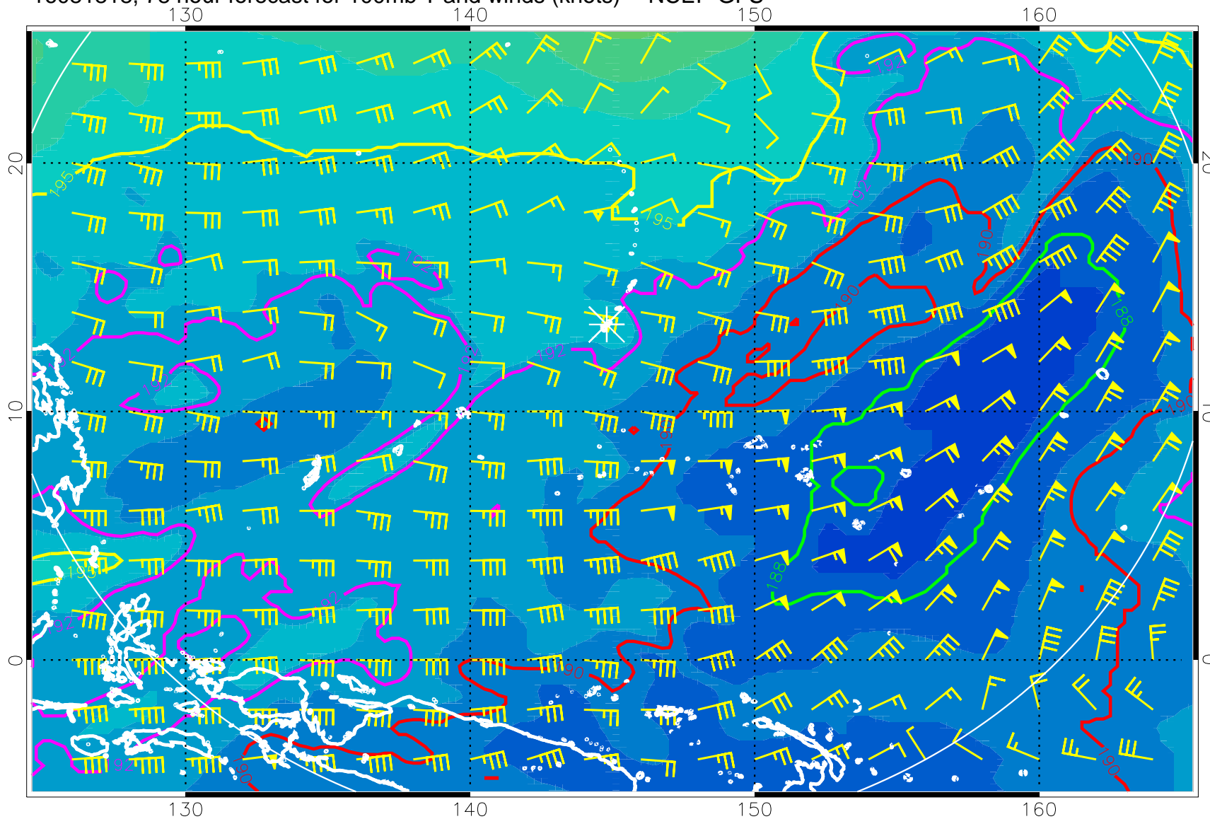
16081818, 78 hour forecast for 100mb T and winds (knots) -- NCEP GFS
