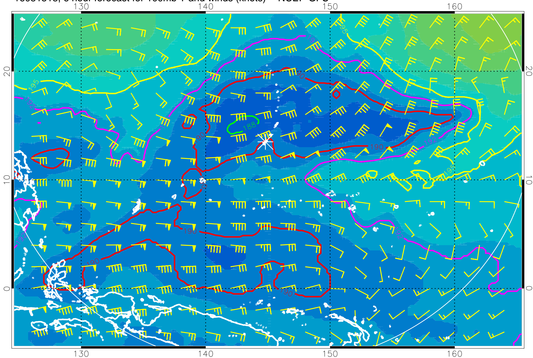
16081518, 6 hour forecast for 100mb T and winds (knots) -- NCEP GFS
