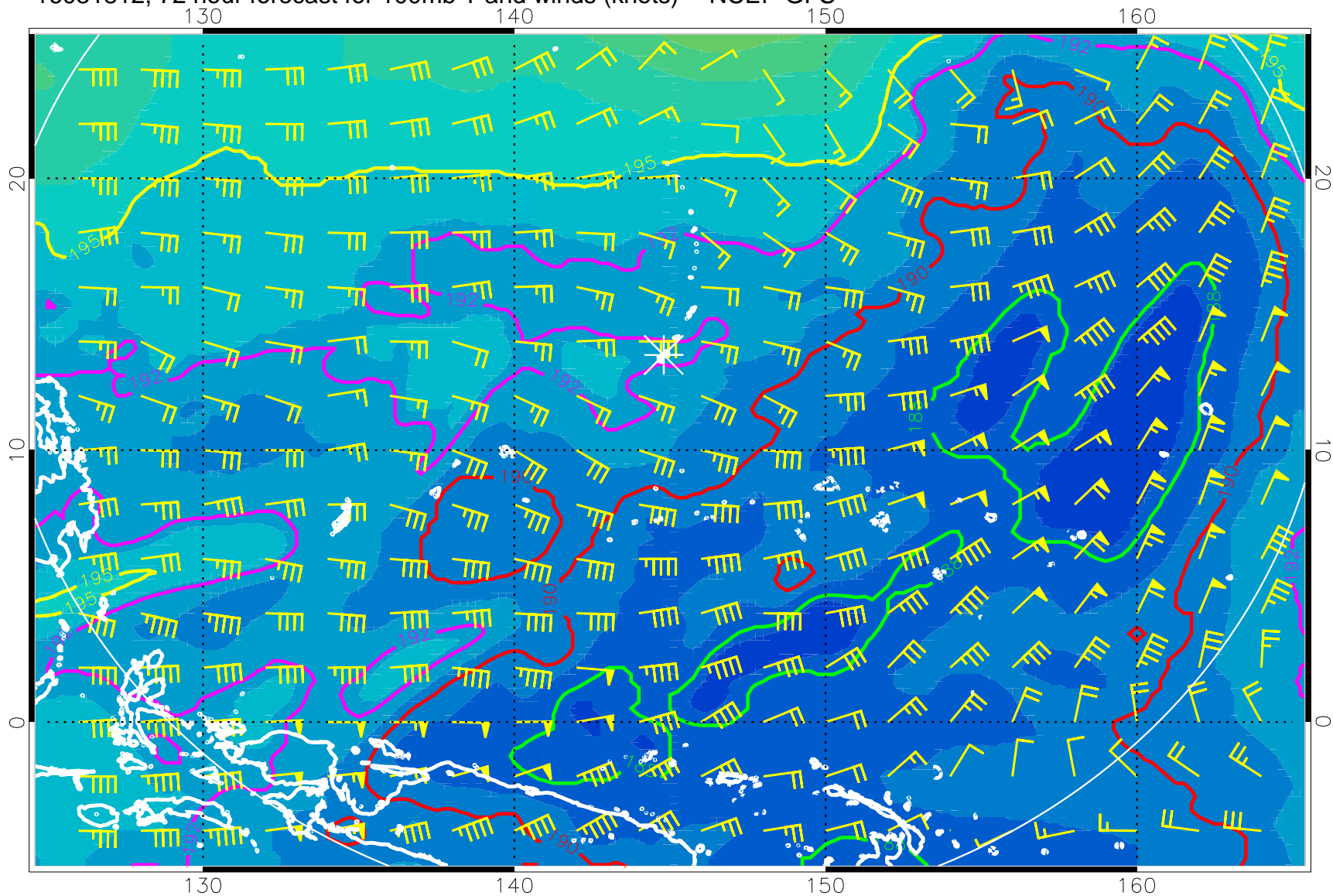
16081812, 72 hour forecast for 100mb T and winds (knots) -- NCEP GFS
