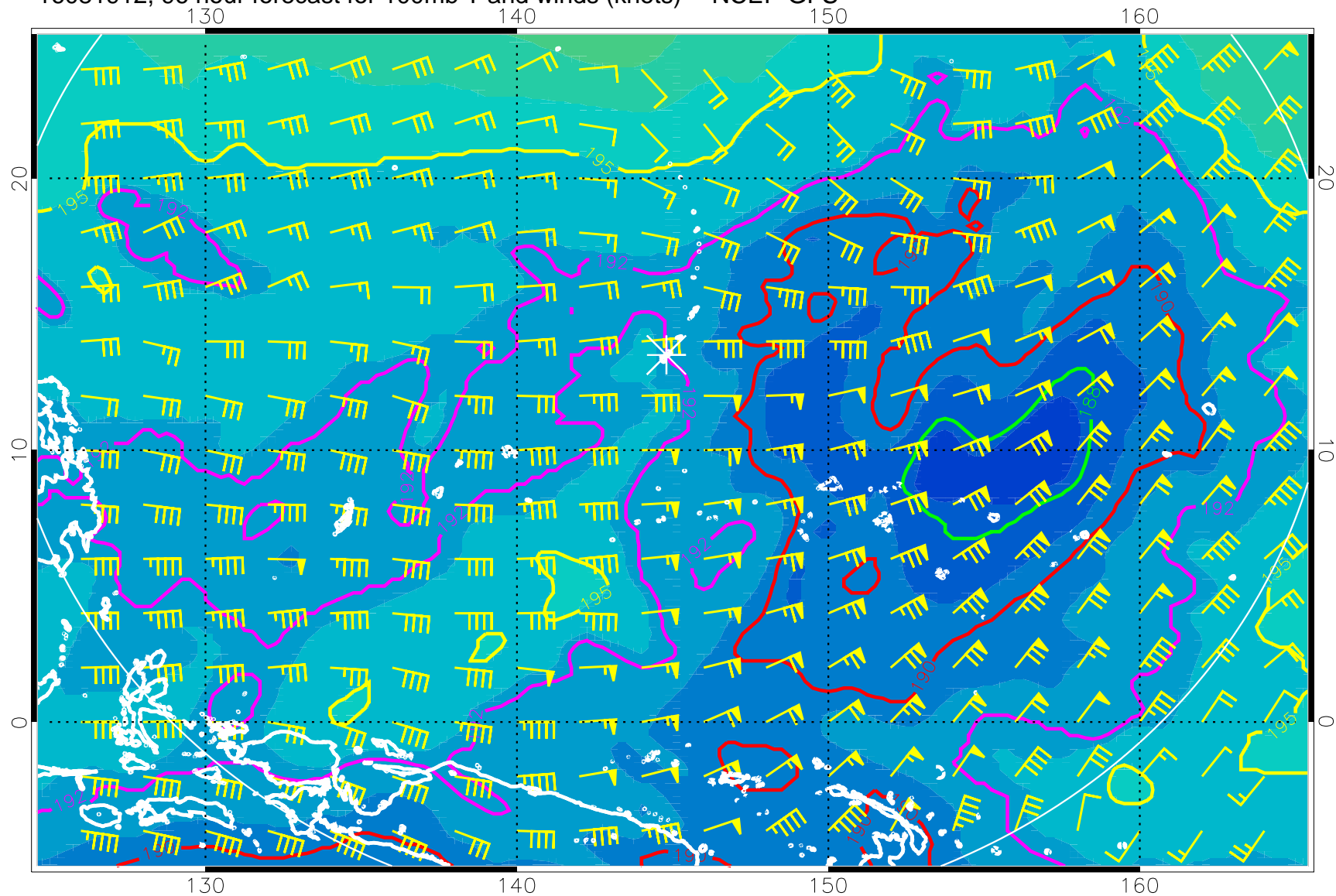
16081912, 96 hour forecast for 100mb T and winds (knots) -- NCEP GFS
