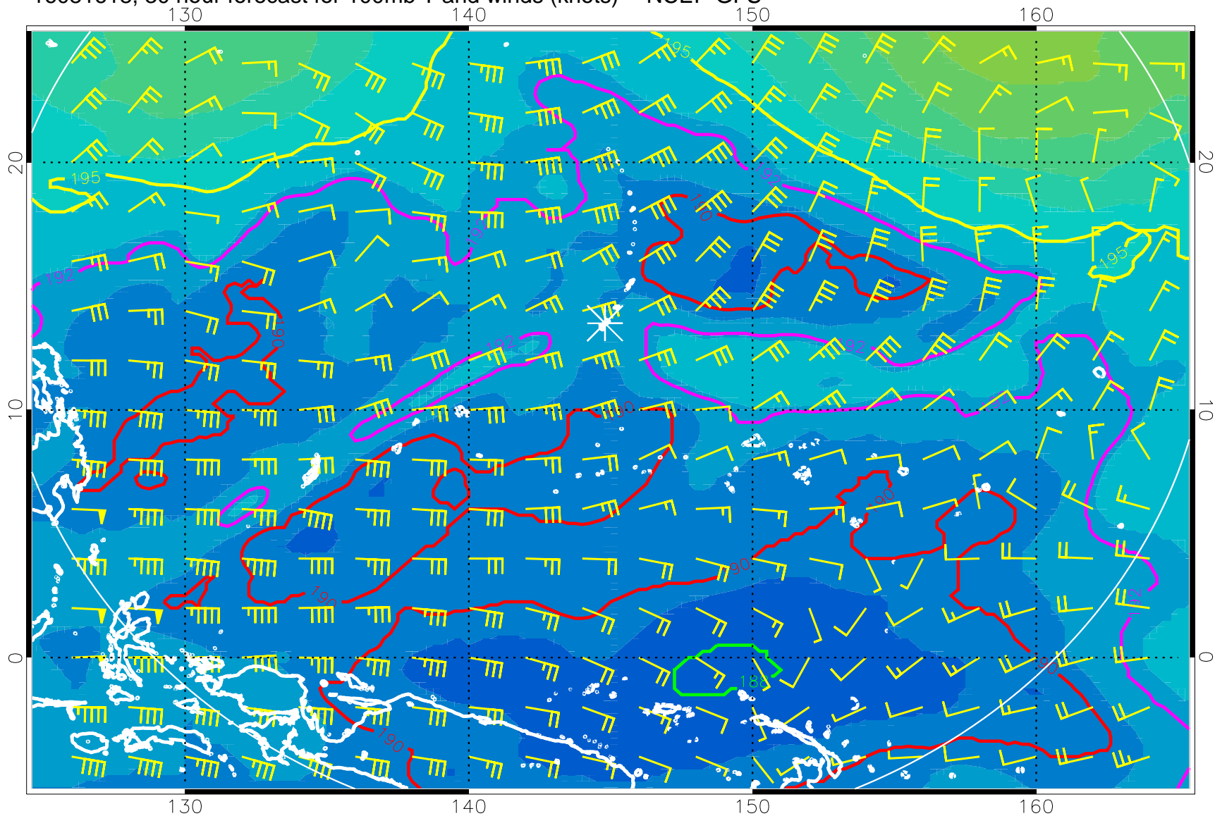
16081618, 30 hour forecast for 100mb T and winds (knots) -- NCEP GFS
