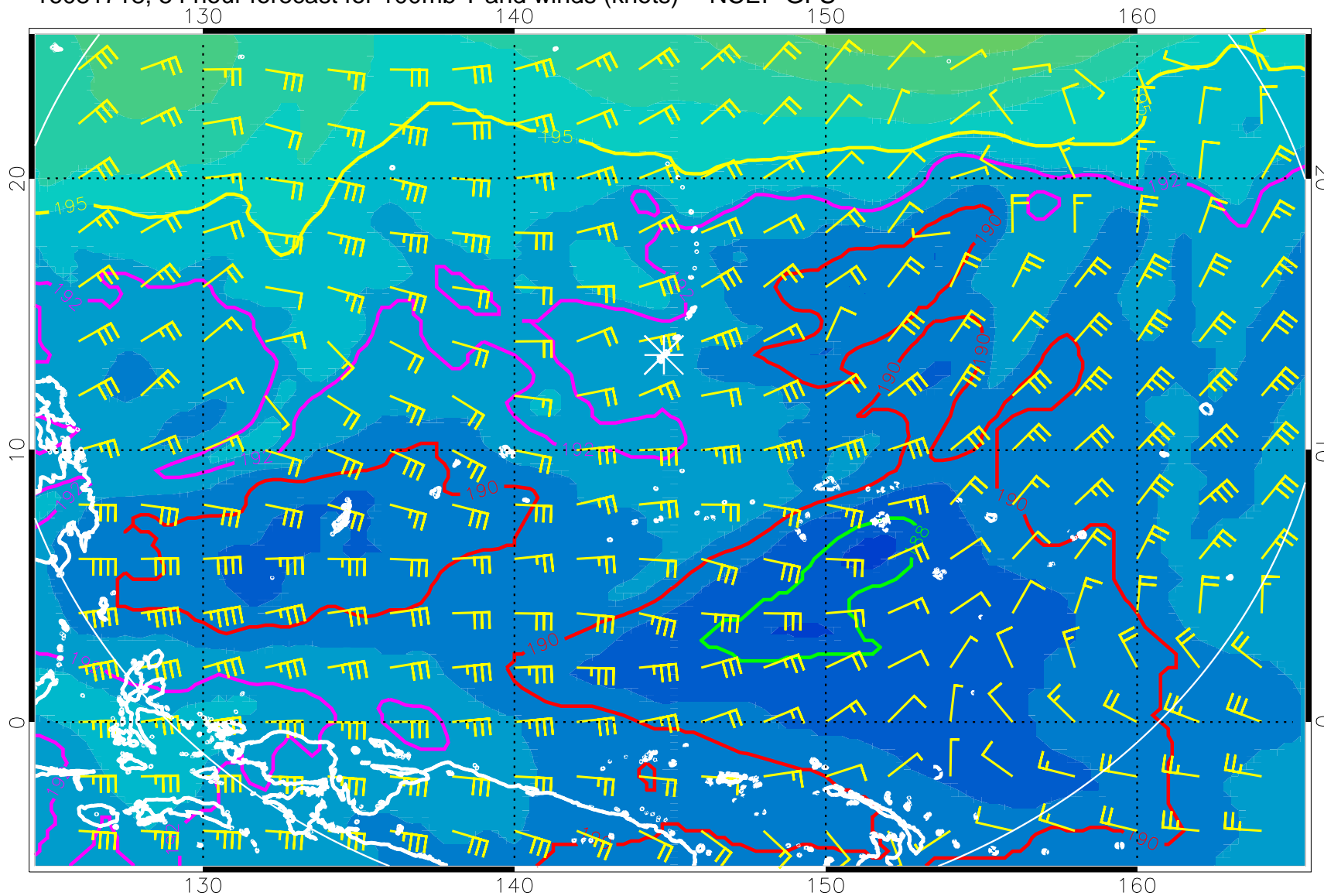
16081718, 54 hour forecast for 100mb T and winds (knots) -- NCEP GFS
