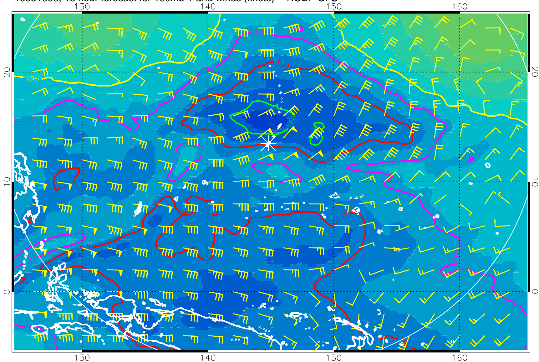
16081606, 18 hour forecast for 100mb T and winds (knots) -- NCEP GFS
