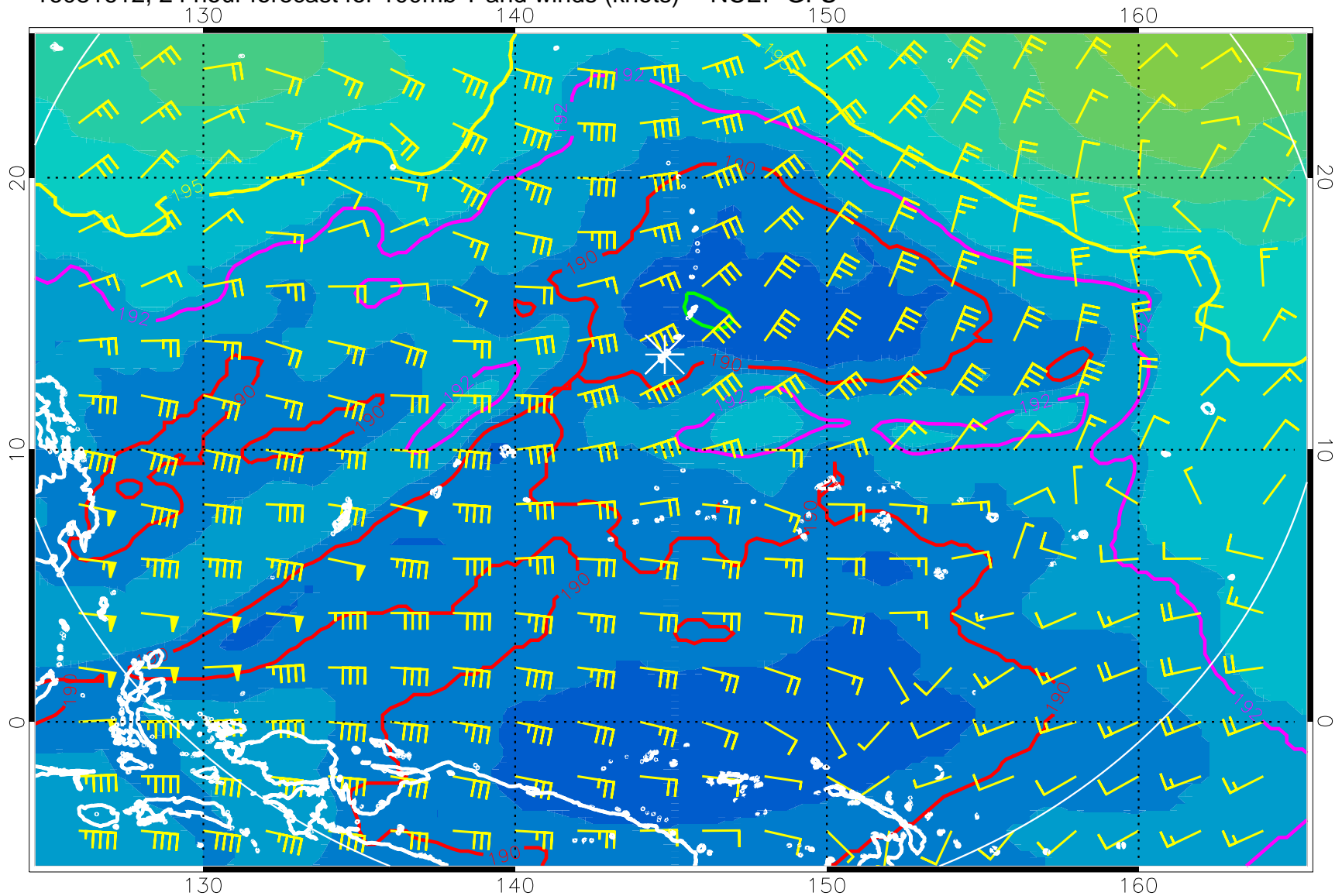
16081612, 24 hour forecast for 100mb T and winds (knots) -- NCEP GFS
