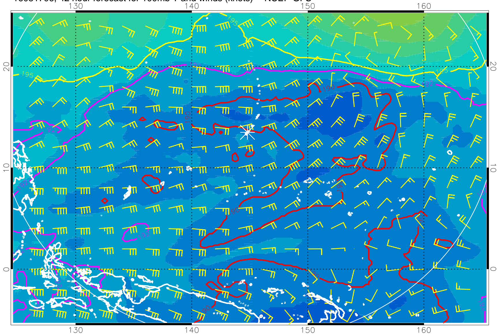
16081706, 42 hour forecast for 100mb T and winds (knots) -- NCEP GFS
