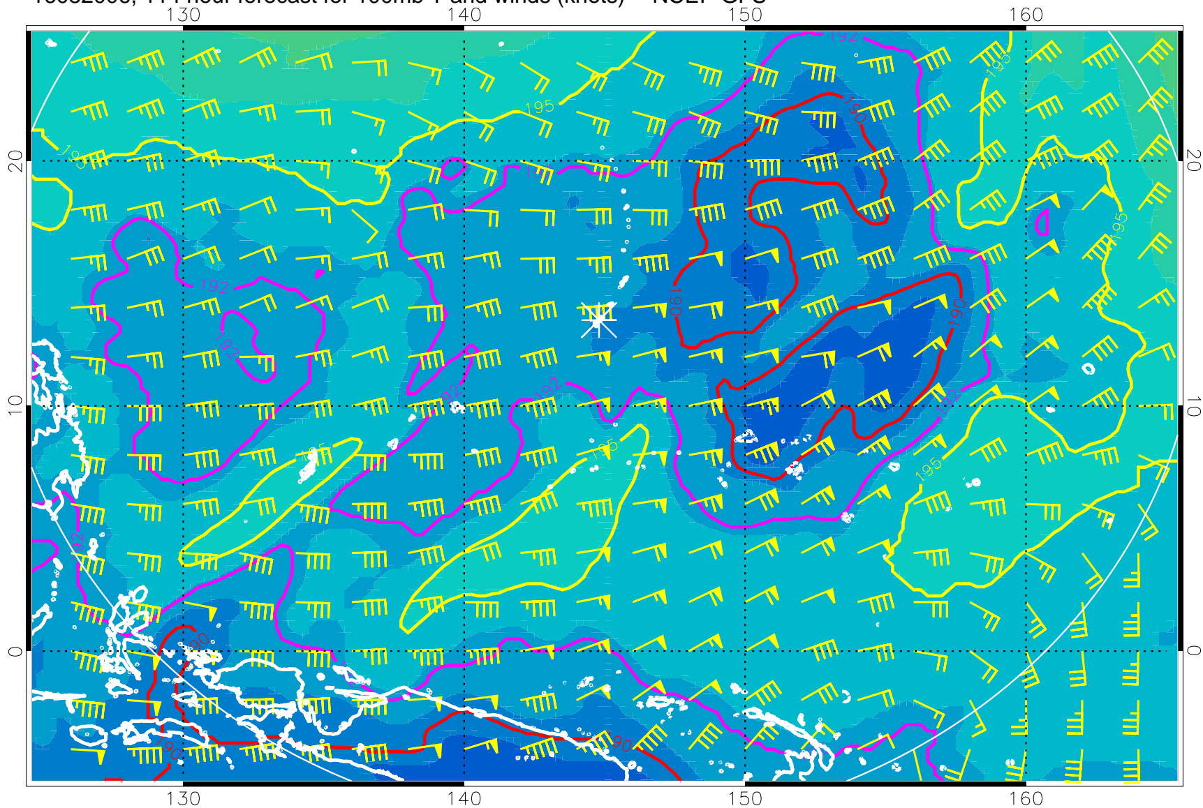
16082006, 114 hour forecast for 100mb T and winds (knots) -- NCEP GFS
