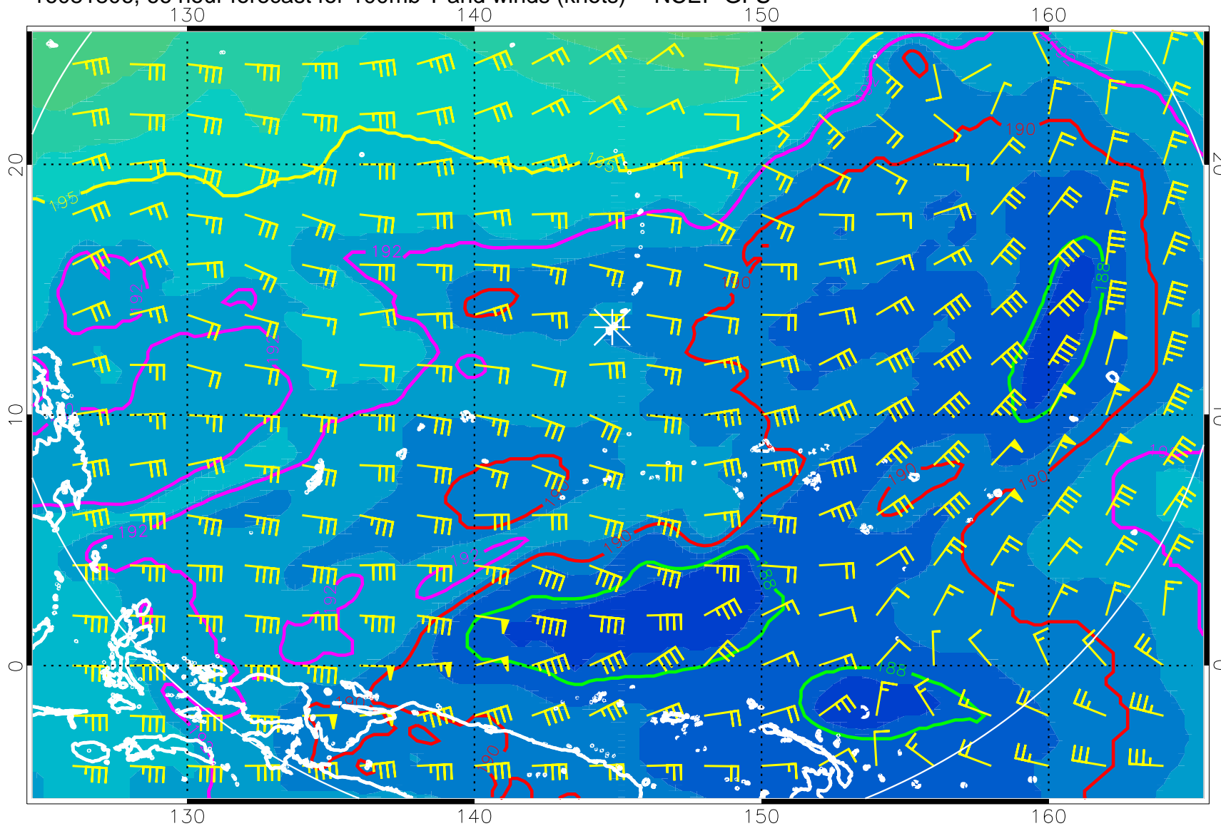
16081806, 66 hour forecast for 100mb T and winds (knots) -- NCEP GFS
