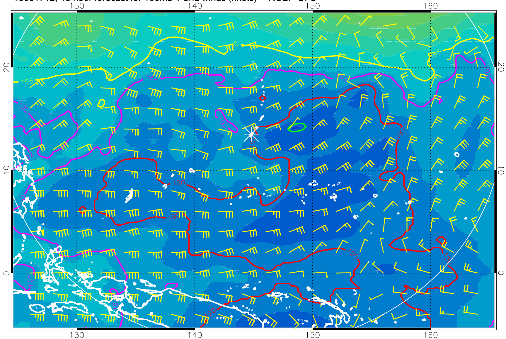
16081712, 48 hour forecast for 100mb T and winds (knots) -- NCEP GFS
