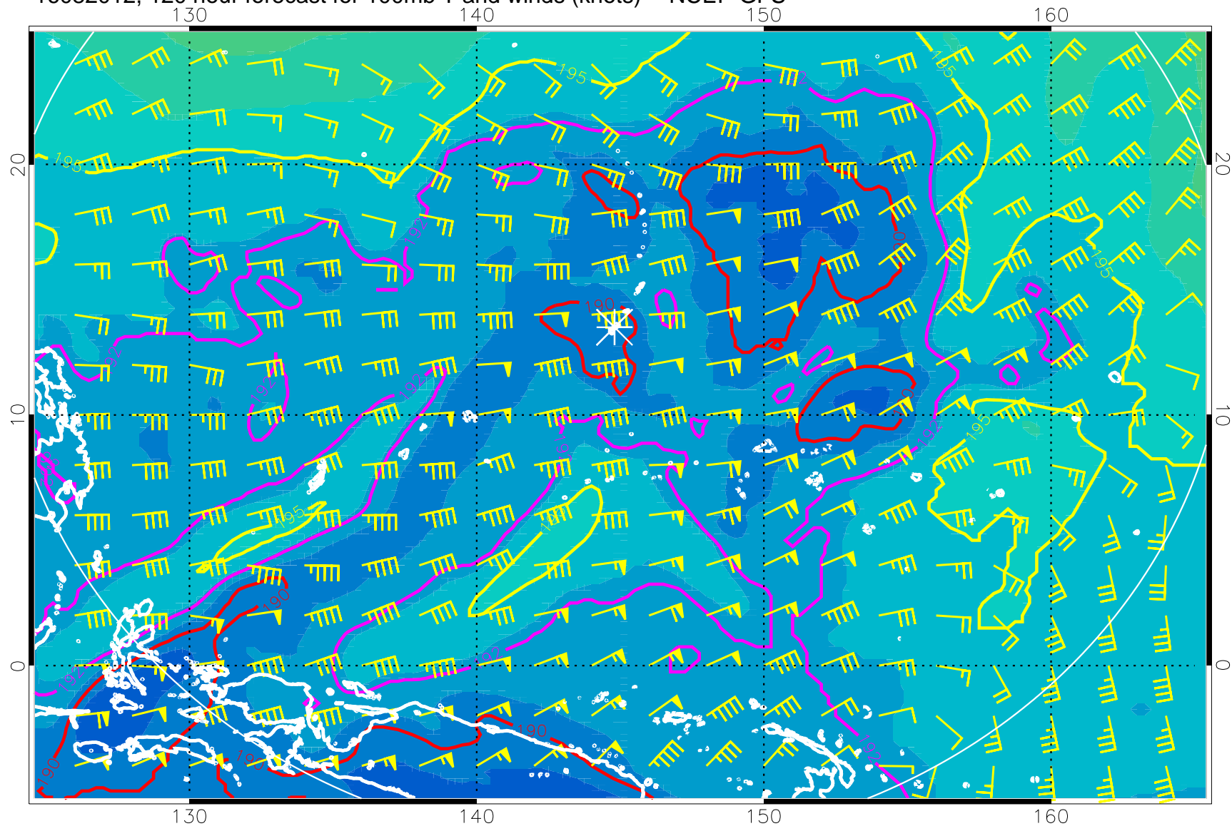
16082012, 120 hour forecast for 100mb T and winds (knots) -- NCEP GFS
