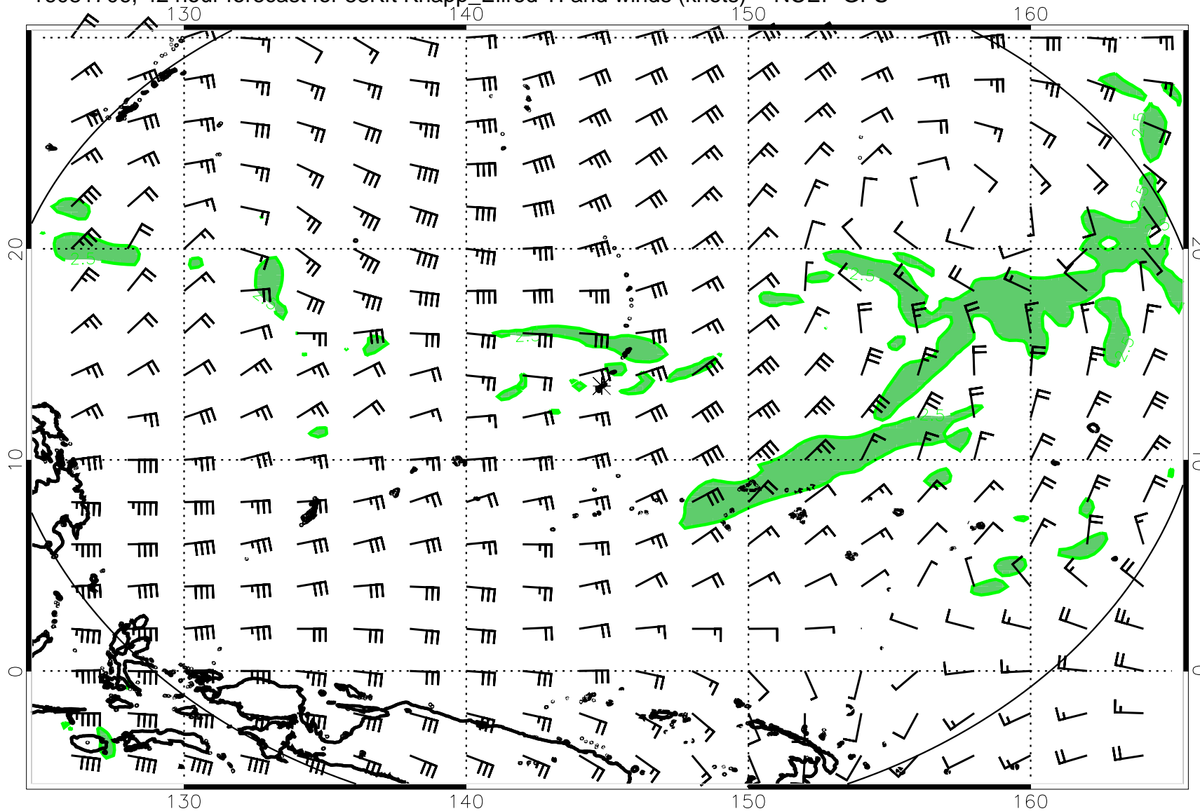
16081706, 42 hour forecast for 53Kft Knapp_Ellrod TI and winds (knots) -- NCEP GFS
