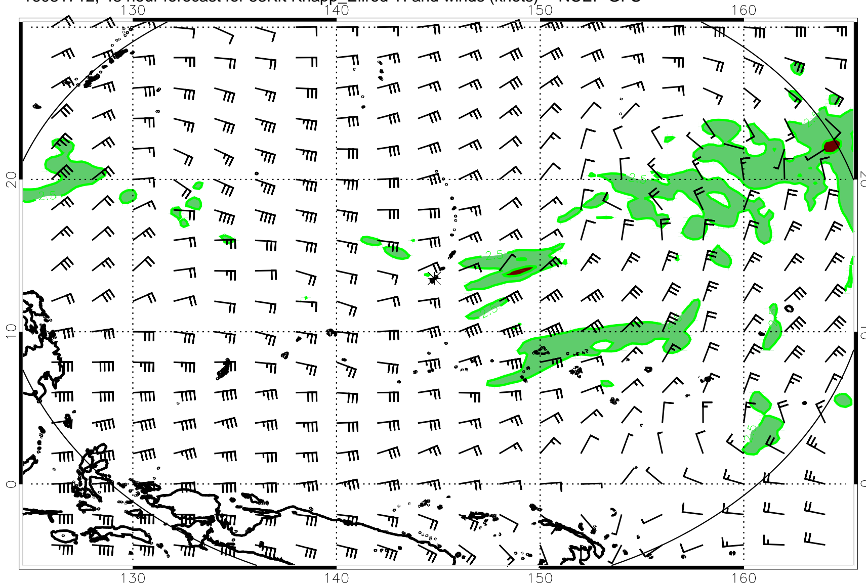
16081712, 48 hour forecast for 53Kft Knapp_Ellrod TI and winds (knots) -- NCEP GFS
