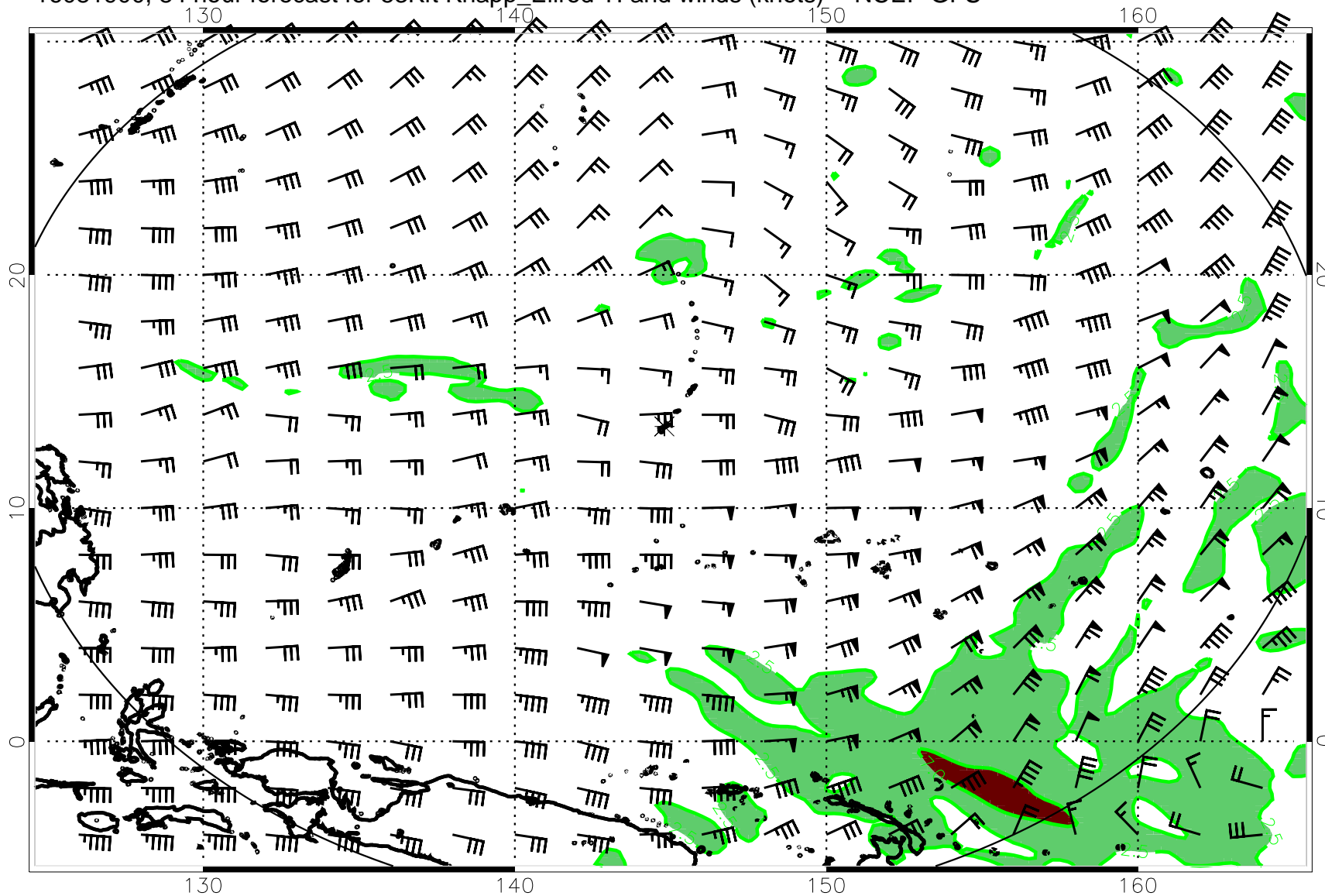
16081900, 84 hour forecast for 53Kft Knapp_Ellrod TI and winds (knots) -- NCEP GFS
