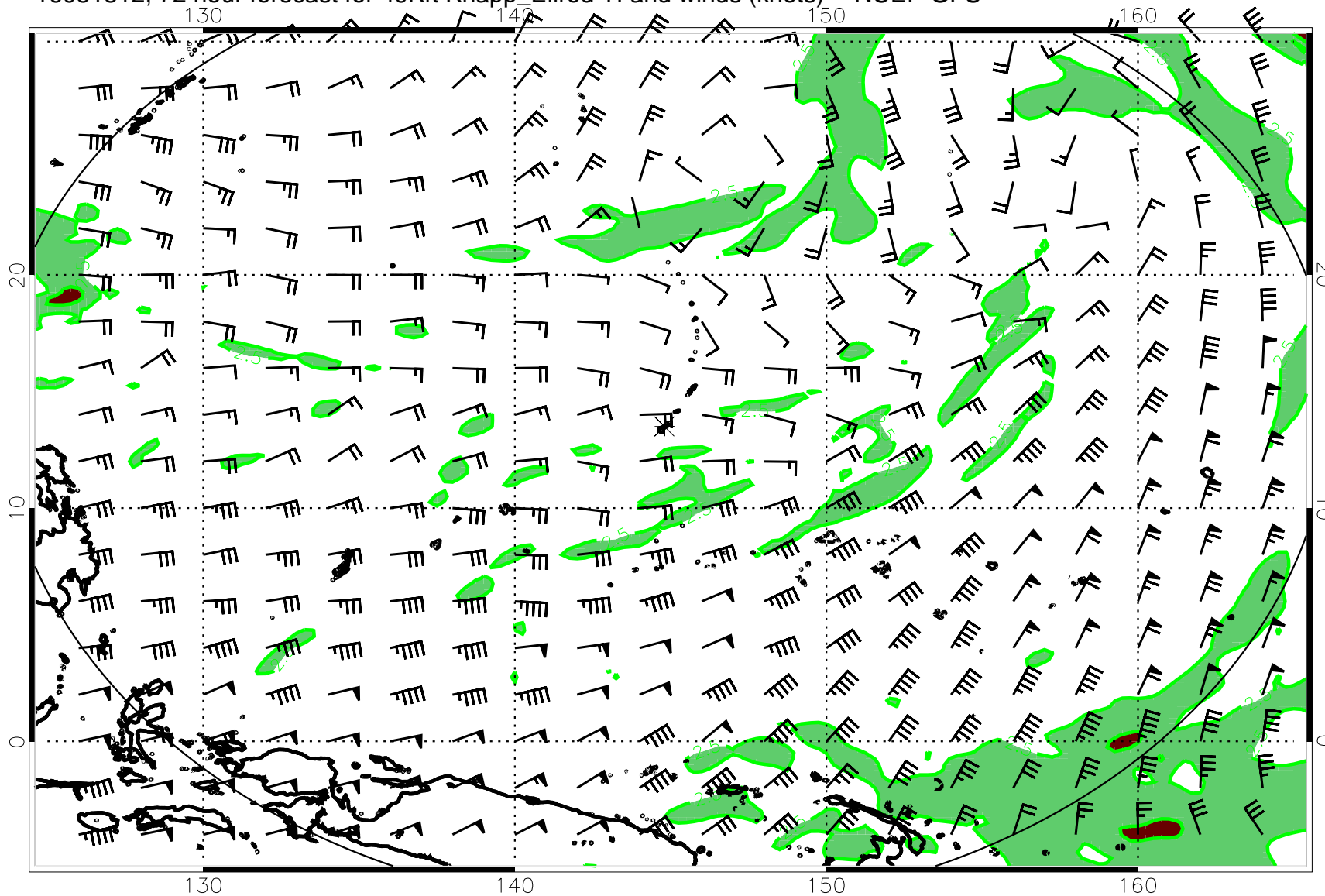
16081812, 72 hour forecast for 49Kft Knapp_Ellrod TI and winds (knots) -- NCEP GFS
