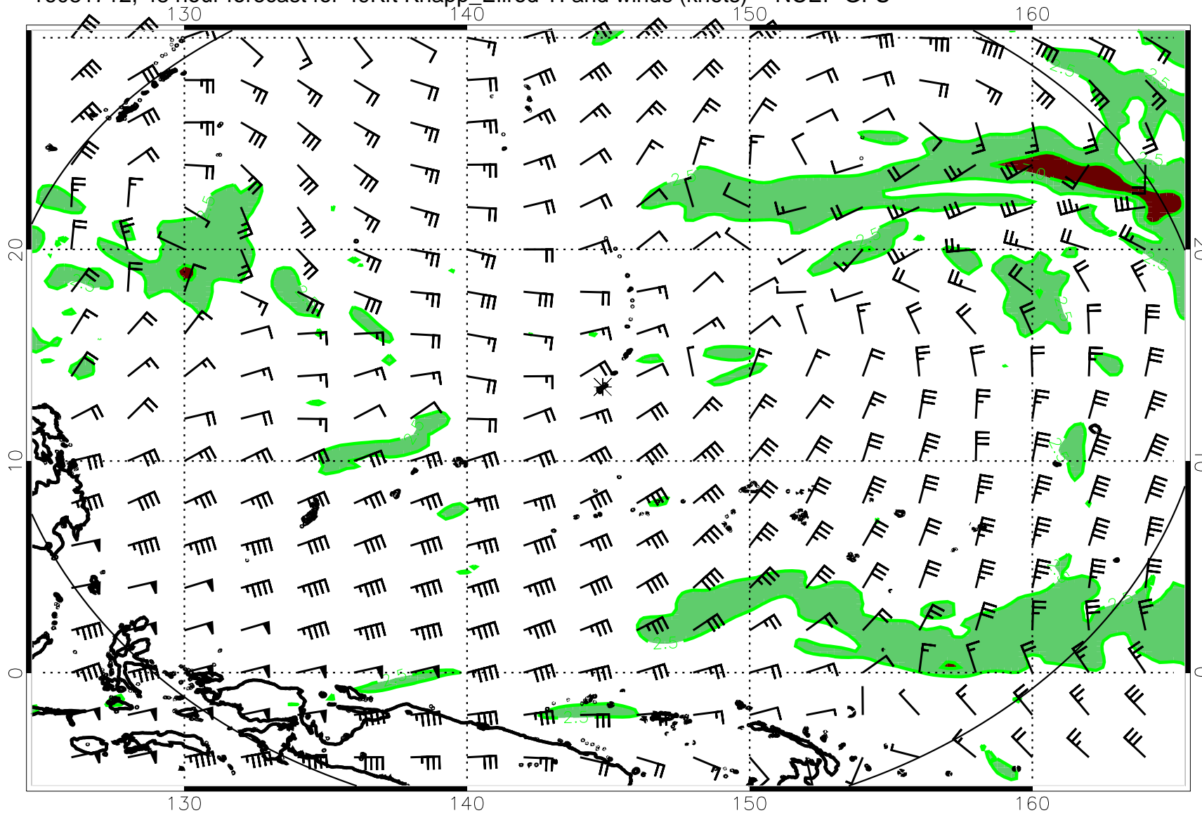
16081712, 48 hour forecast for 49Kft Knapp_Ellrod TI and winds (knots) -- NCEP GFS
