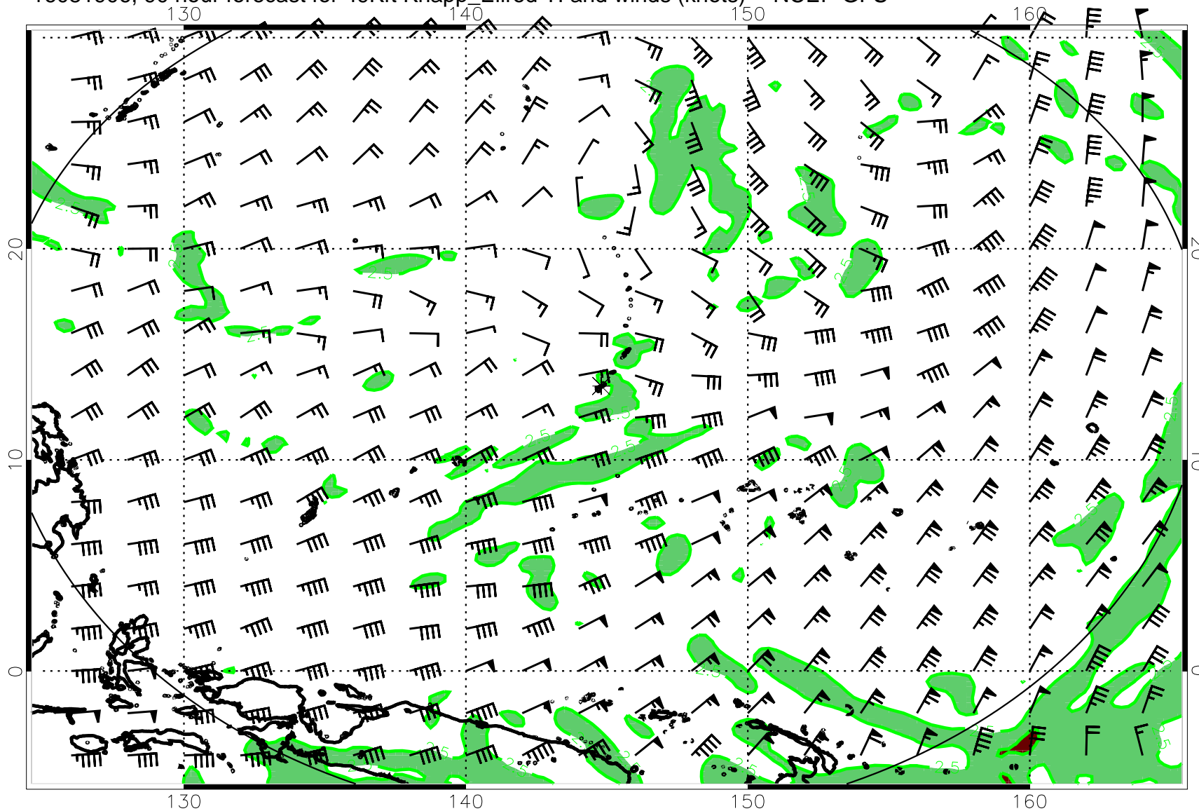
16081906, 90 hour forecast for 49Kft Knapp_Ellrod TI and winds (knots) -- NCEP GFS
