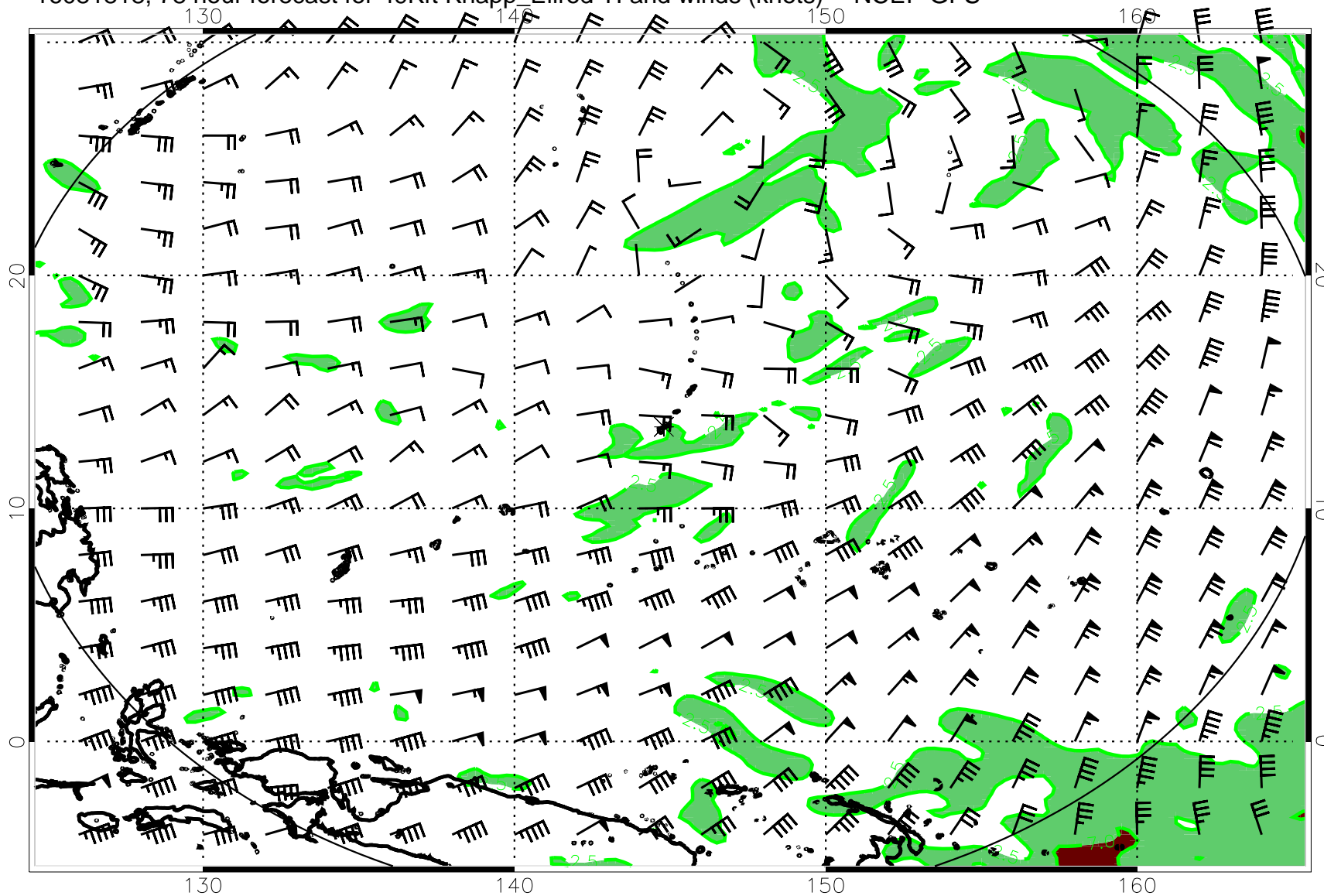
16081818, 78 hour forecast for 49Kft Knapp_Ellrod TI and winds (knots) -- NCEP GFS
