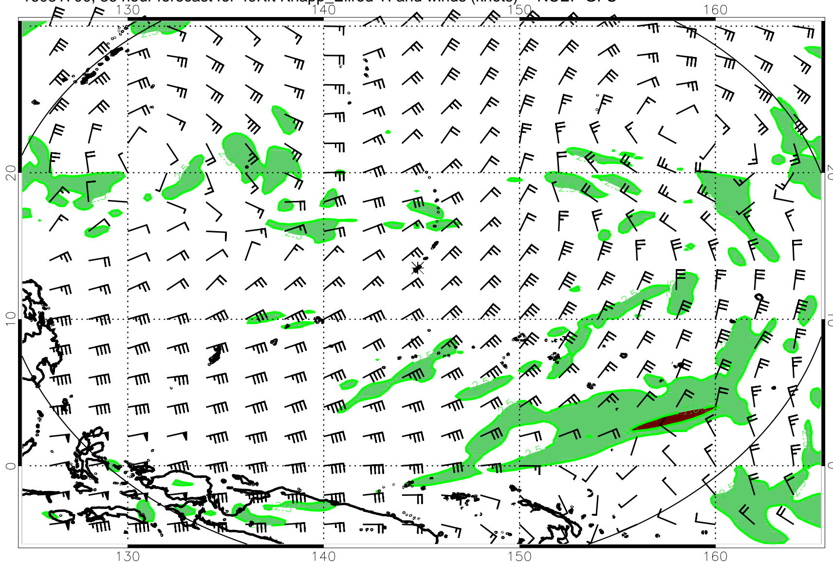
16081700, 36 hour forecast for 49Kft Knapp_Ellrod TI and winds (knots) -- NCEP GFS
