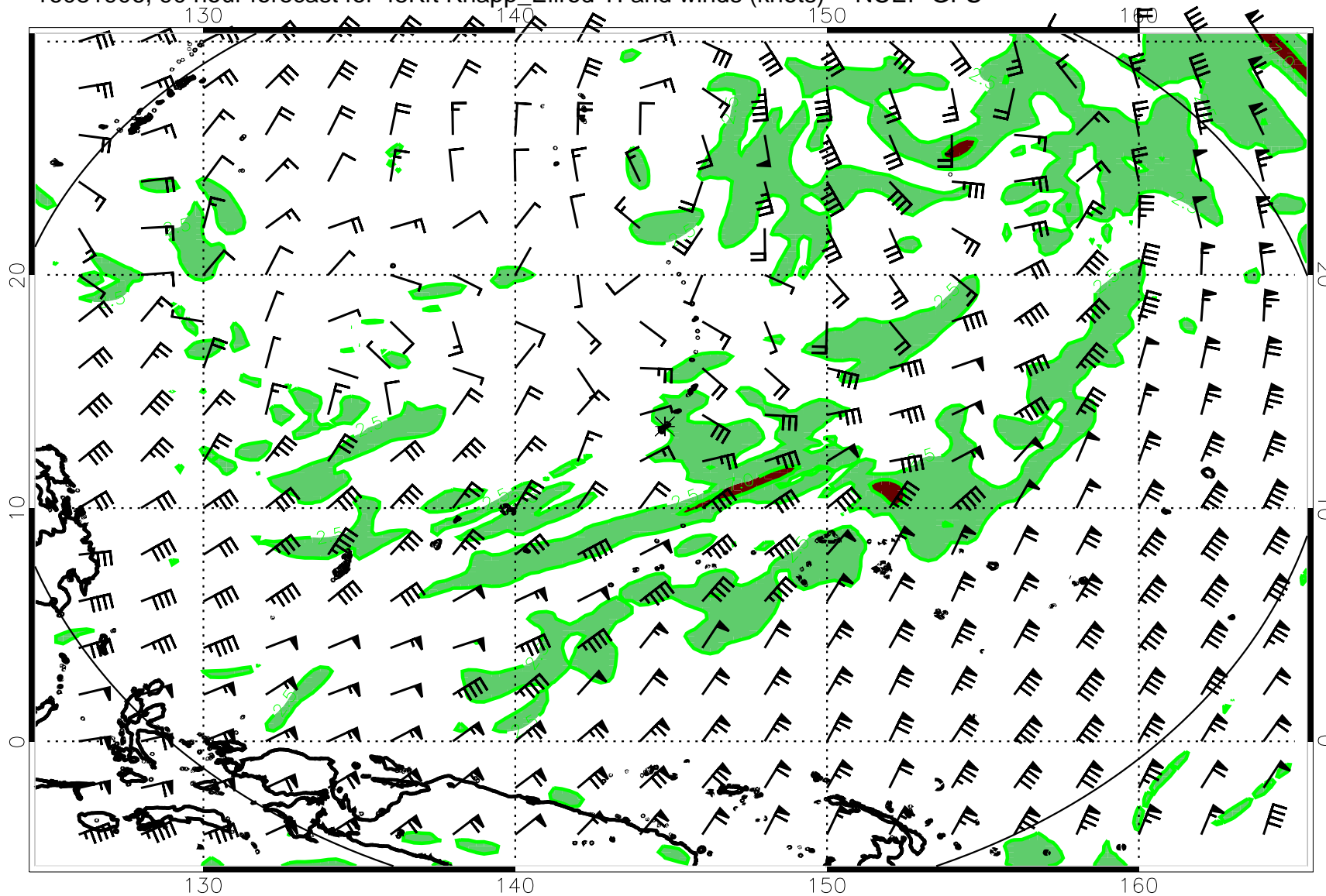
16081906, 90 hour forecast for 45Kft Knapp_Ellrod TI and winds (knots) -- NCEP GFS
