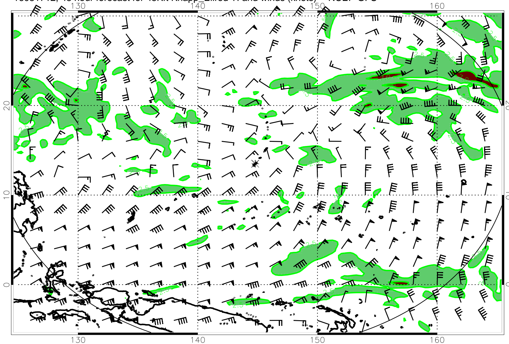
16081712, 48 hour forecast for 45Kft Knapp_Ellrod TI and winds (knots) -- NCEP GFS
