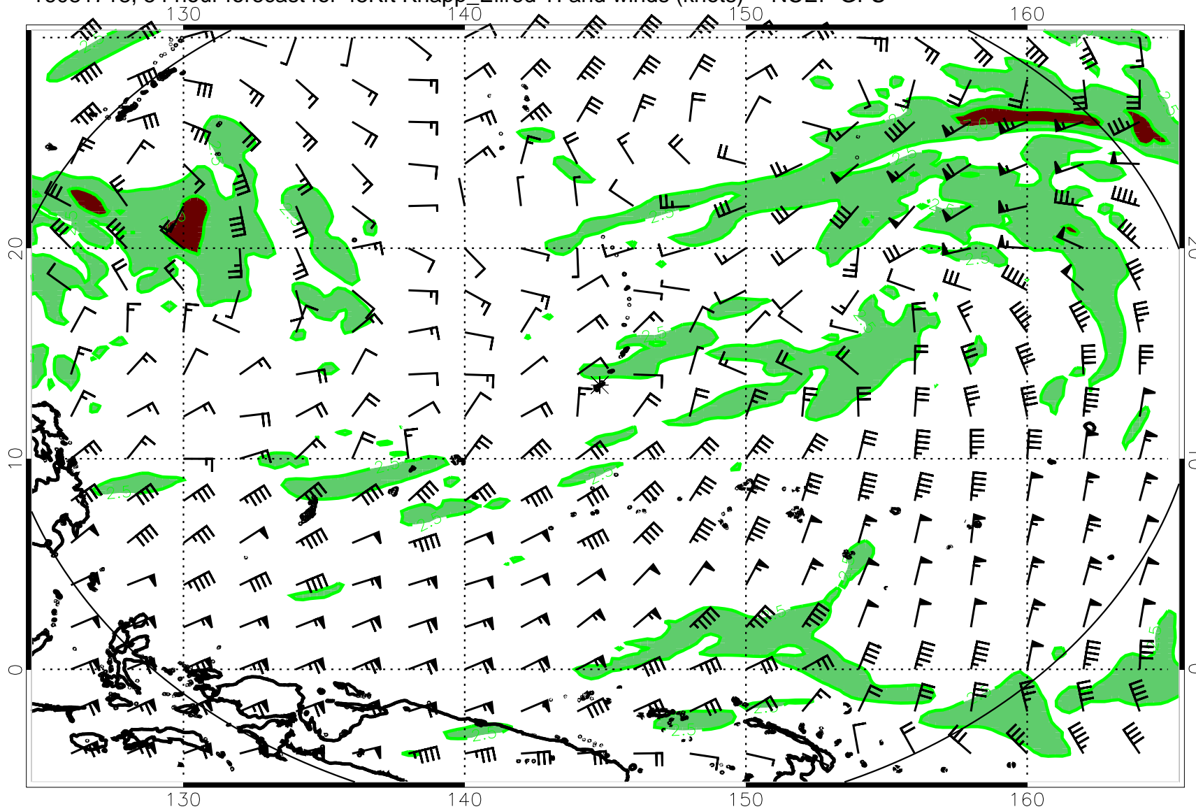
16081718, 54 hour forecast for 45Kft Knapp_Ellrod TI and winds (knots) -- NCEP GFS
