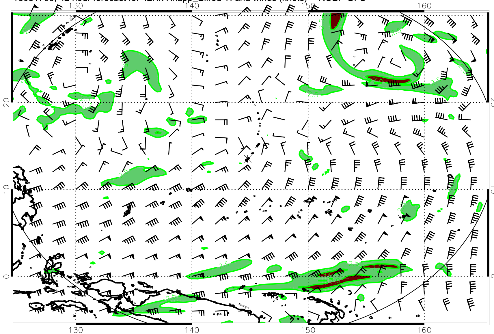
16081706, 42 hour forecast for 42Kft Knapp_Ellrod TI and winds (knots) -- NCEP GFS
