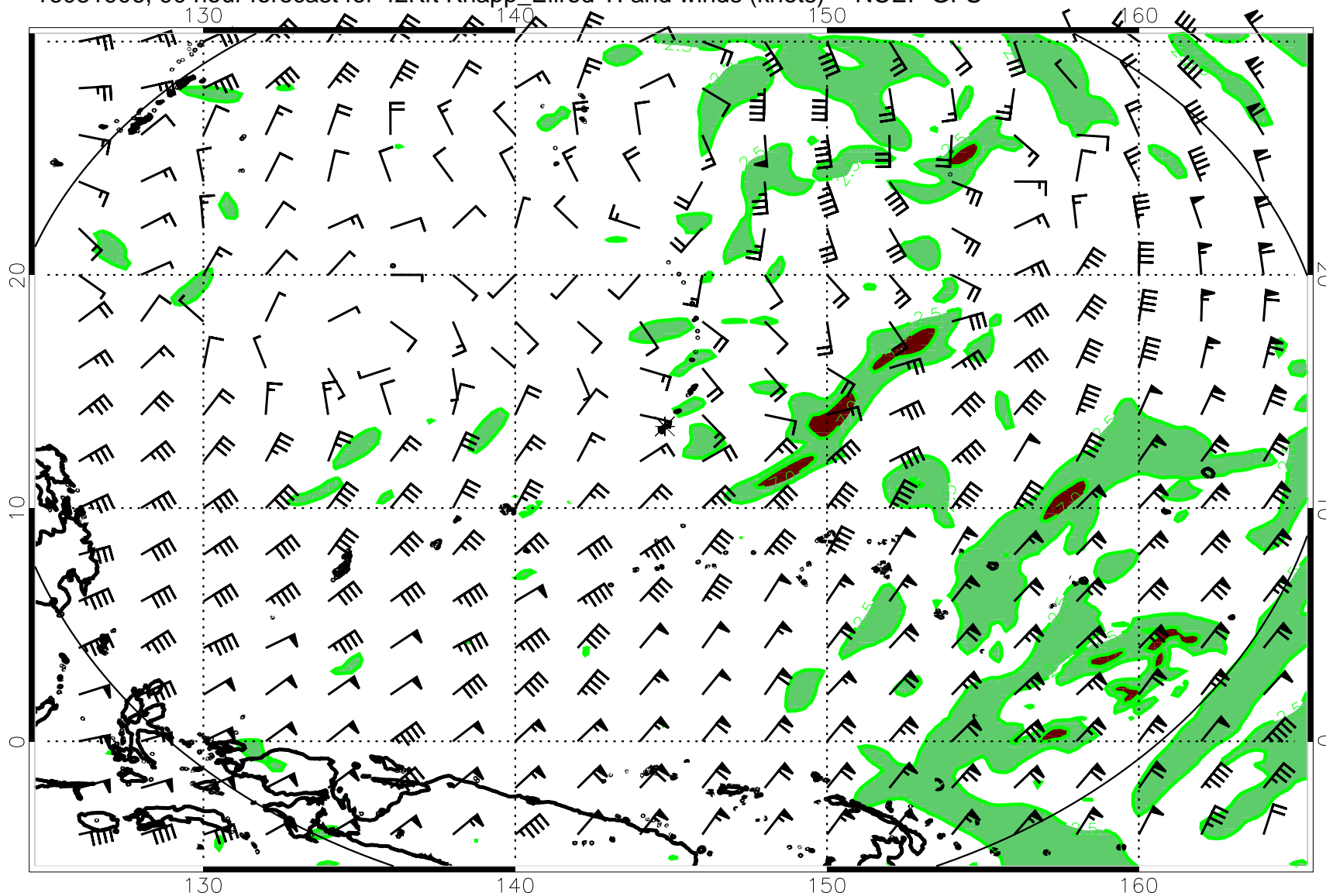
16081906, 90 hour forecast for 42Kft Knapp_Ellrod TI and winds (knots) -- NCEP GFS
