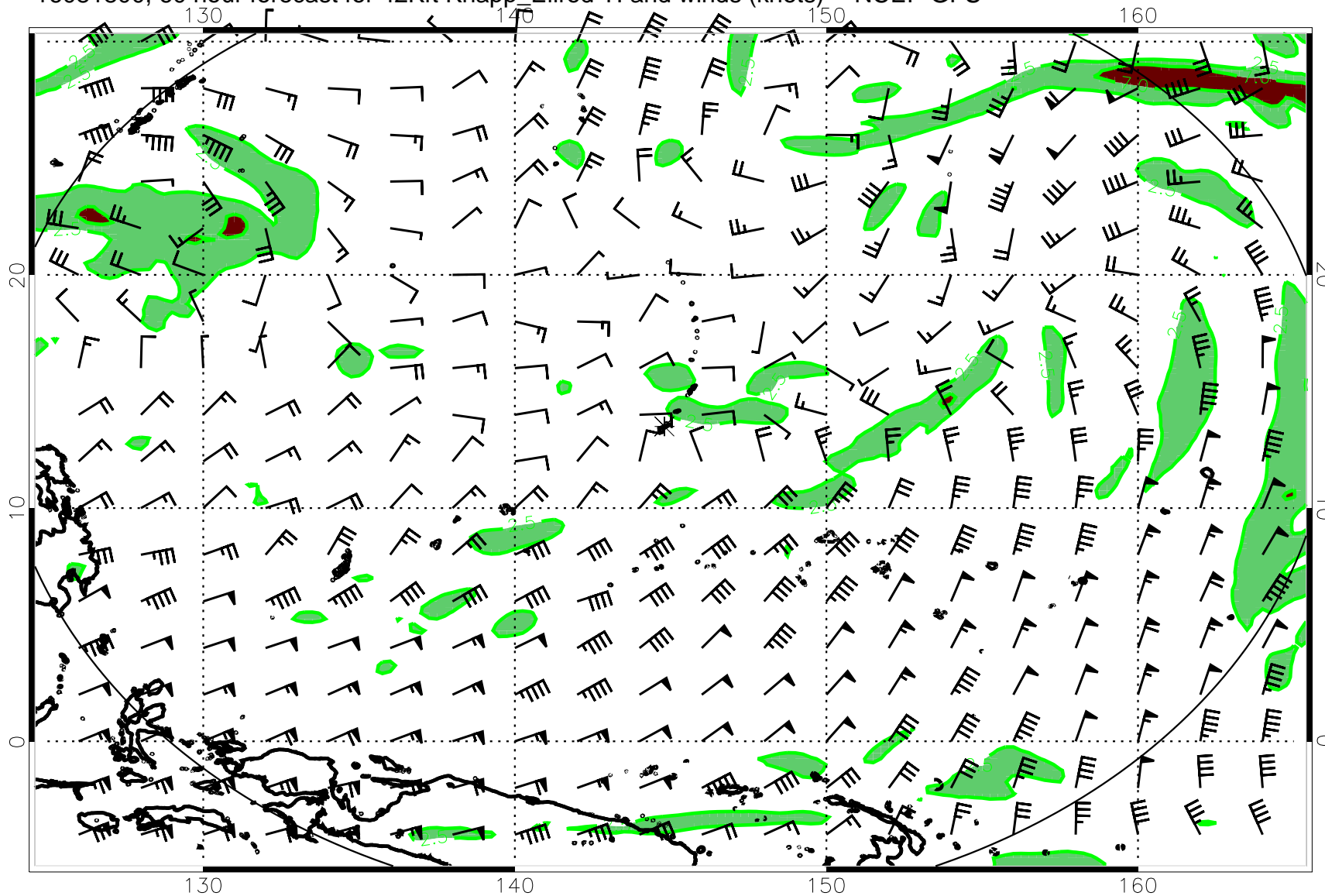
16081800, 60 hour forecast for 42Kft Knapp_Ellrod TI and winds (knots) -- NCEP GFS
