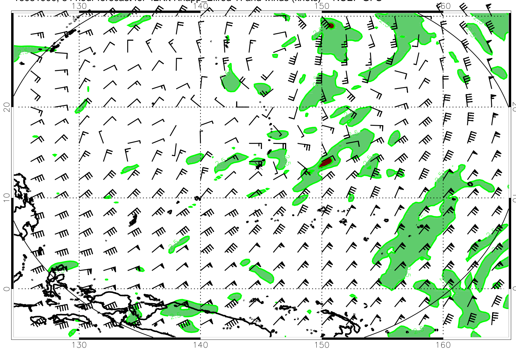
16081900, 84 hour forecast for 42Kft Knapp_Ellrod TI and winds (knots) -- NCEP GFS
