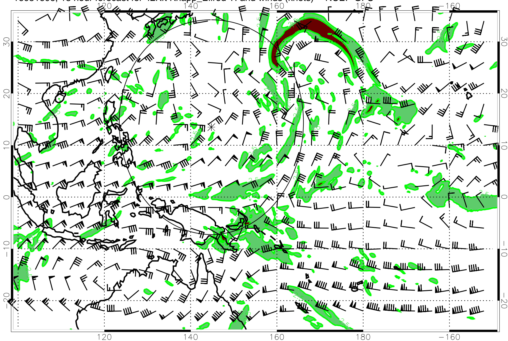
16081606, 18 hour forecast for 42Kft Knapp_Ellrod TI and winds (knots) -- NCEP GFS
