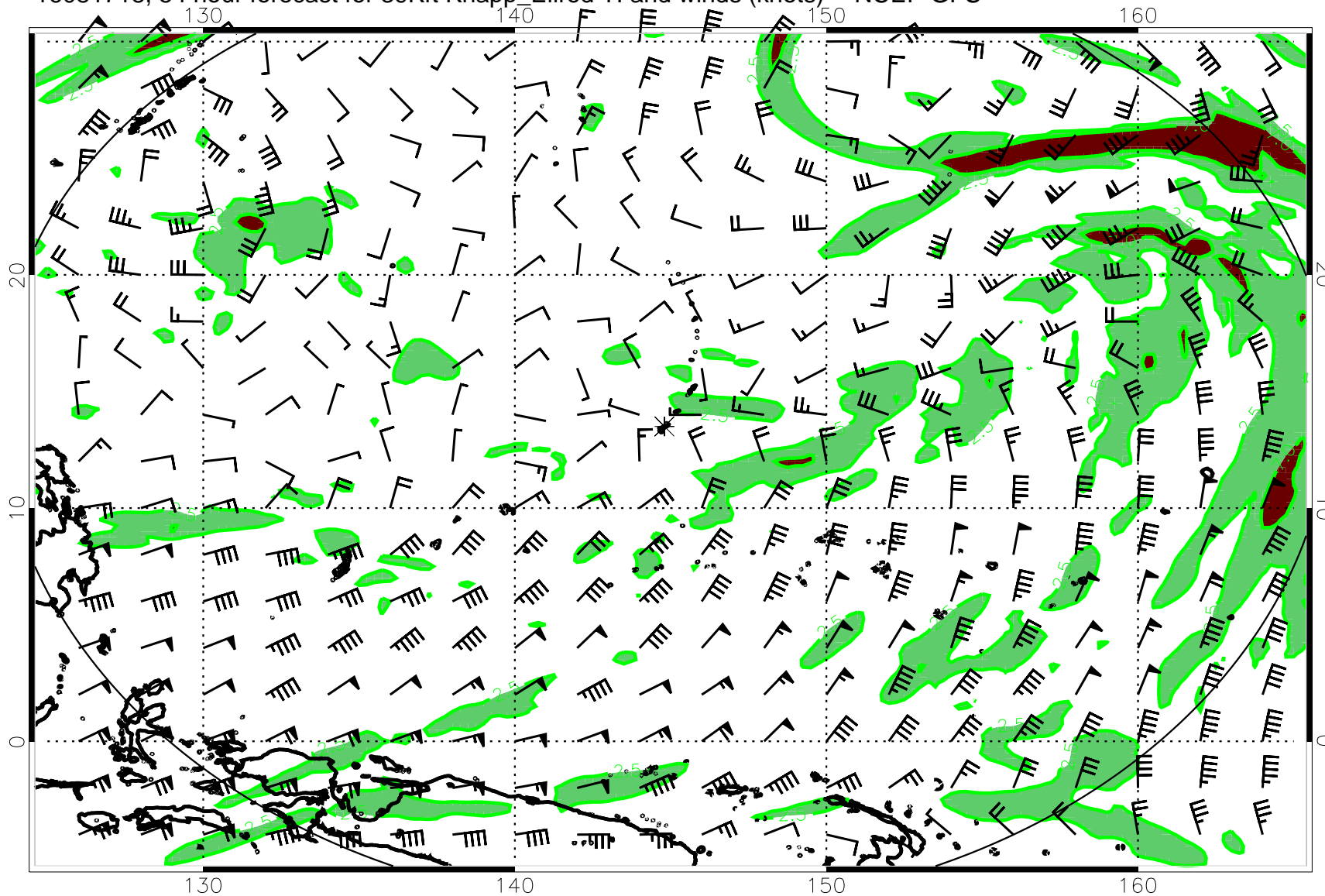
16081718, 54 hour forecast for 39Kft Knapp_Ellrod TI and winds (knots) -- NCEP GFS
