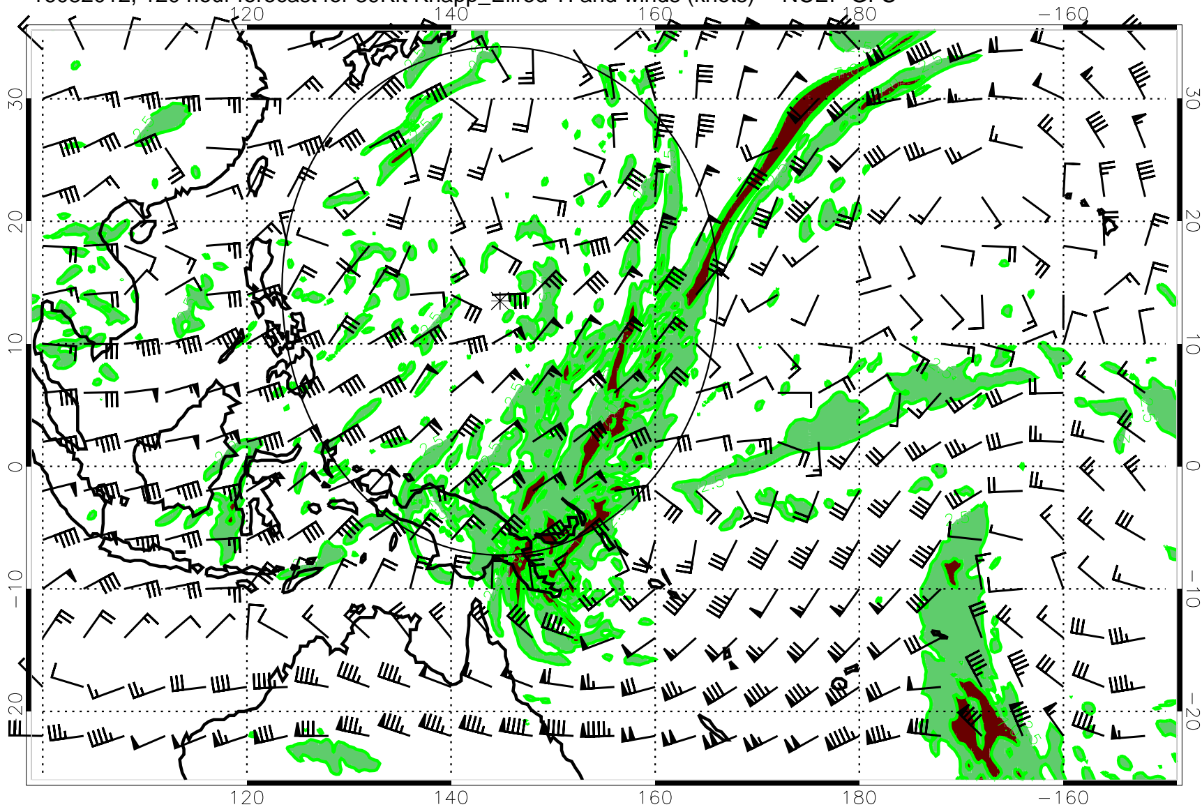
16082012, 120 hour forecast for 39Kft Knapp_Ellrod TI and winds (knots) -- NCEP GFS
