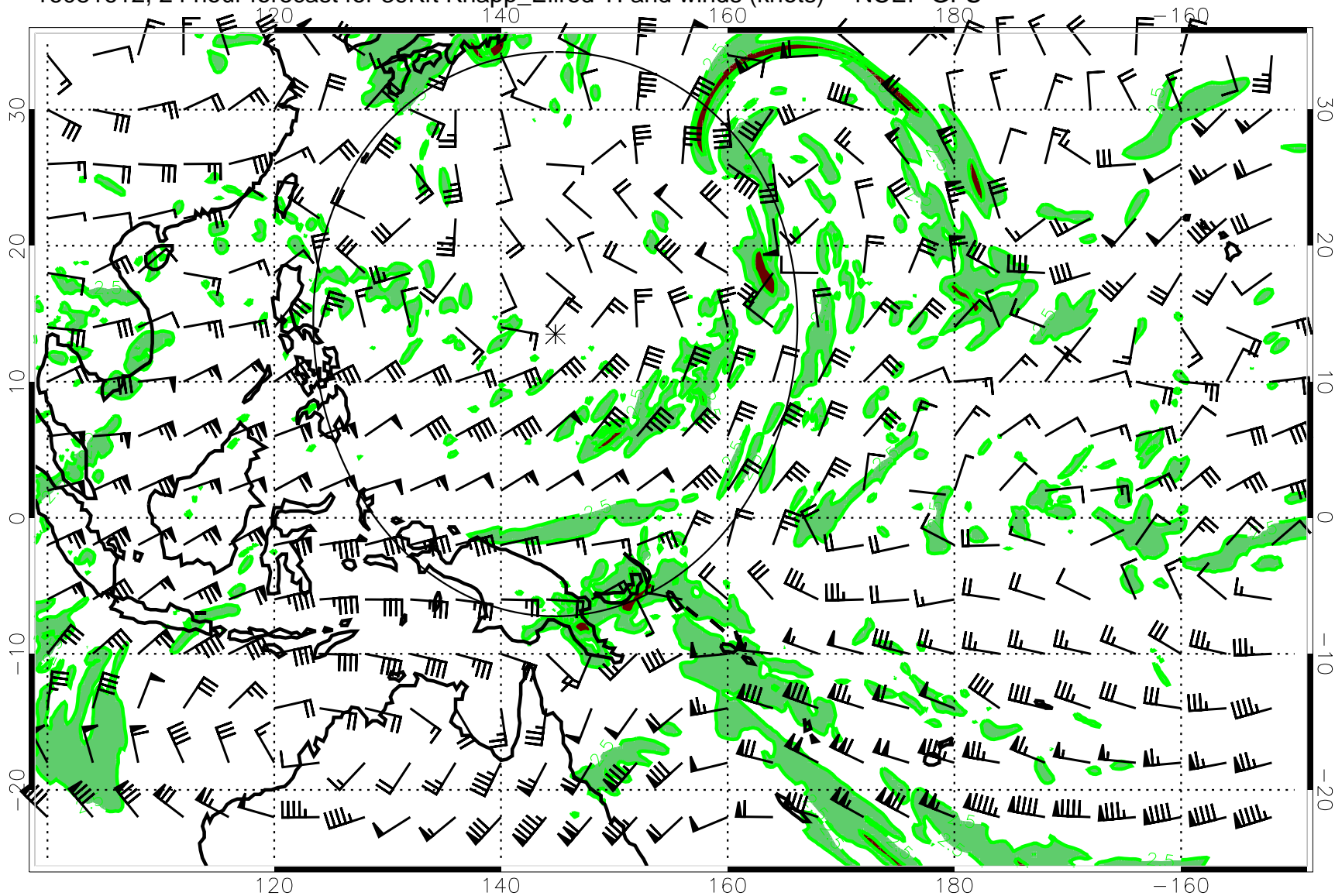
16081612, 24 hour forecast for 39Kft Knapp_Ellrod TI and winds (knots) -- NCEP GFS
