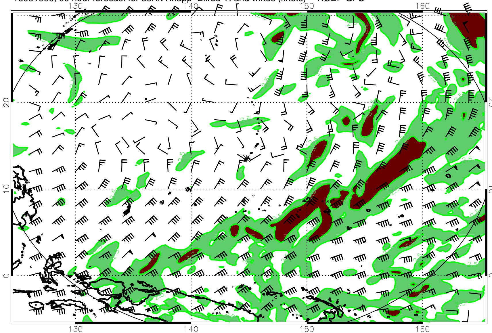
16081906, 90 hour forecast for 36Kft Knapp_Ellrod TI and winds (knots) -- NCEP GFS
