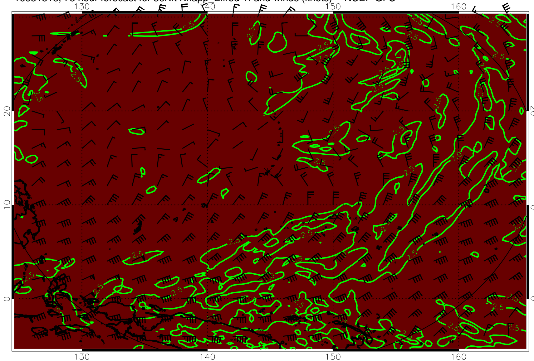
16081818, 78 hour forecast for 36Kft Knapp_Ellrod TI and winds (knots) -- NCEP GFS
