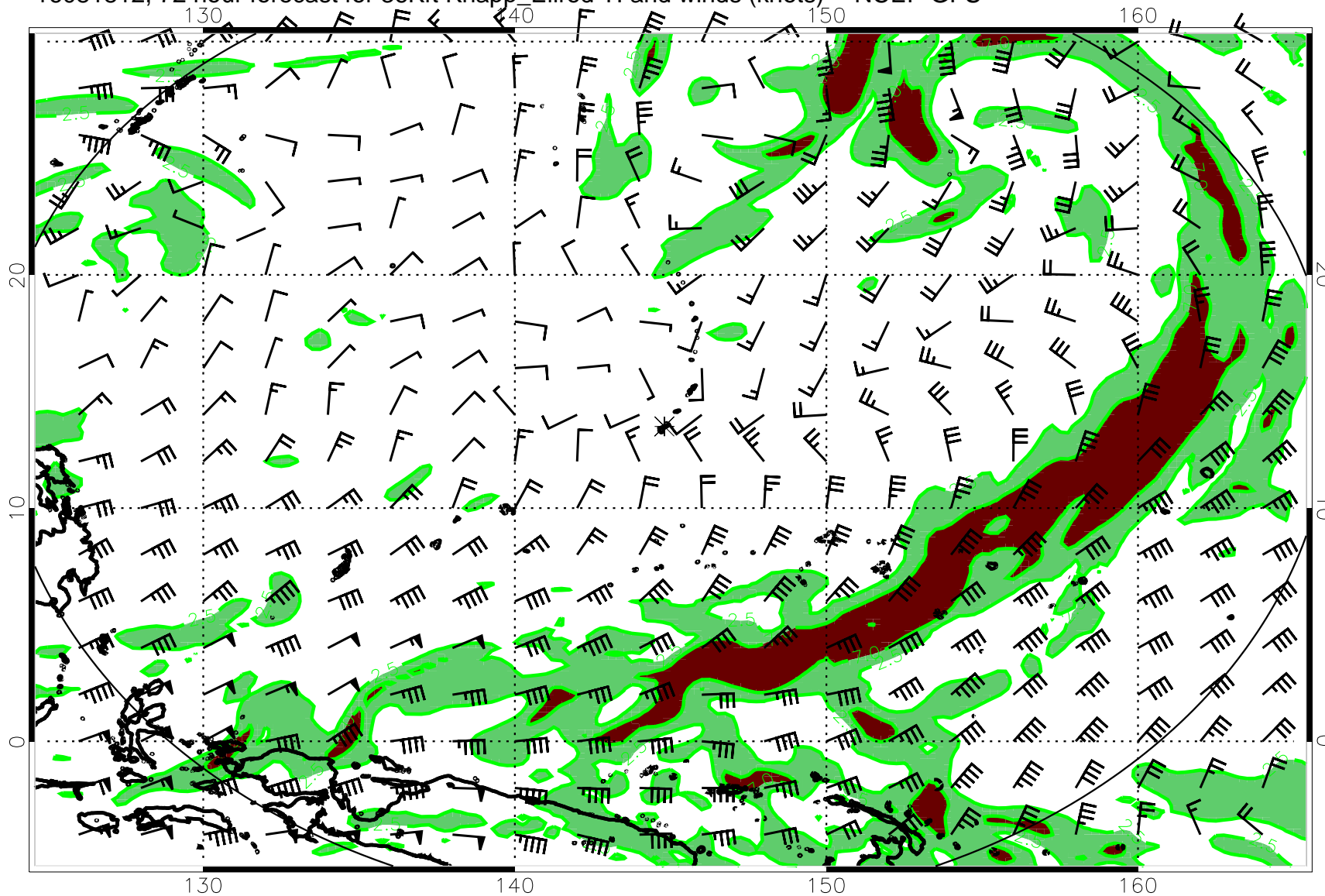
16081812, 72 hour forecast for 36Kft Knapp_Ellrod TI and winds (knots) -- NCEP GFS
