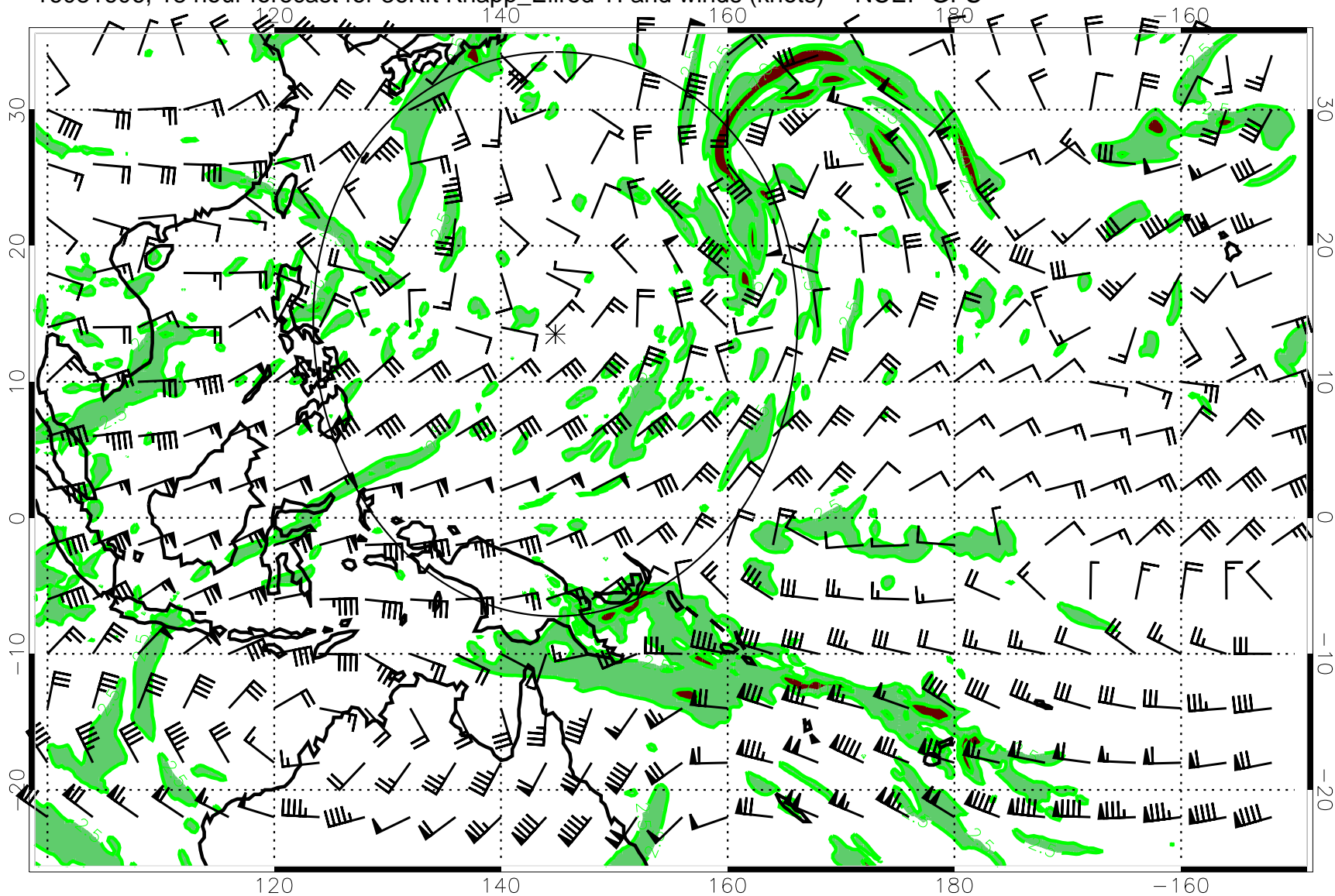
16081606, 18 hour forecast for 36Kft Knapp_Ellrod TI and winds (knots) -- NCEP GFS
