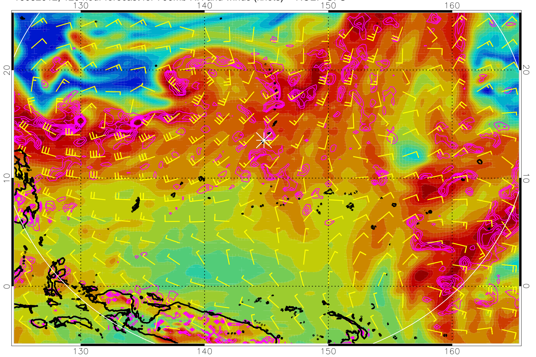
16082012, 120 hour forecast for 700mb RH and winds (knots) -- NCEP GFS
