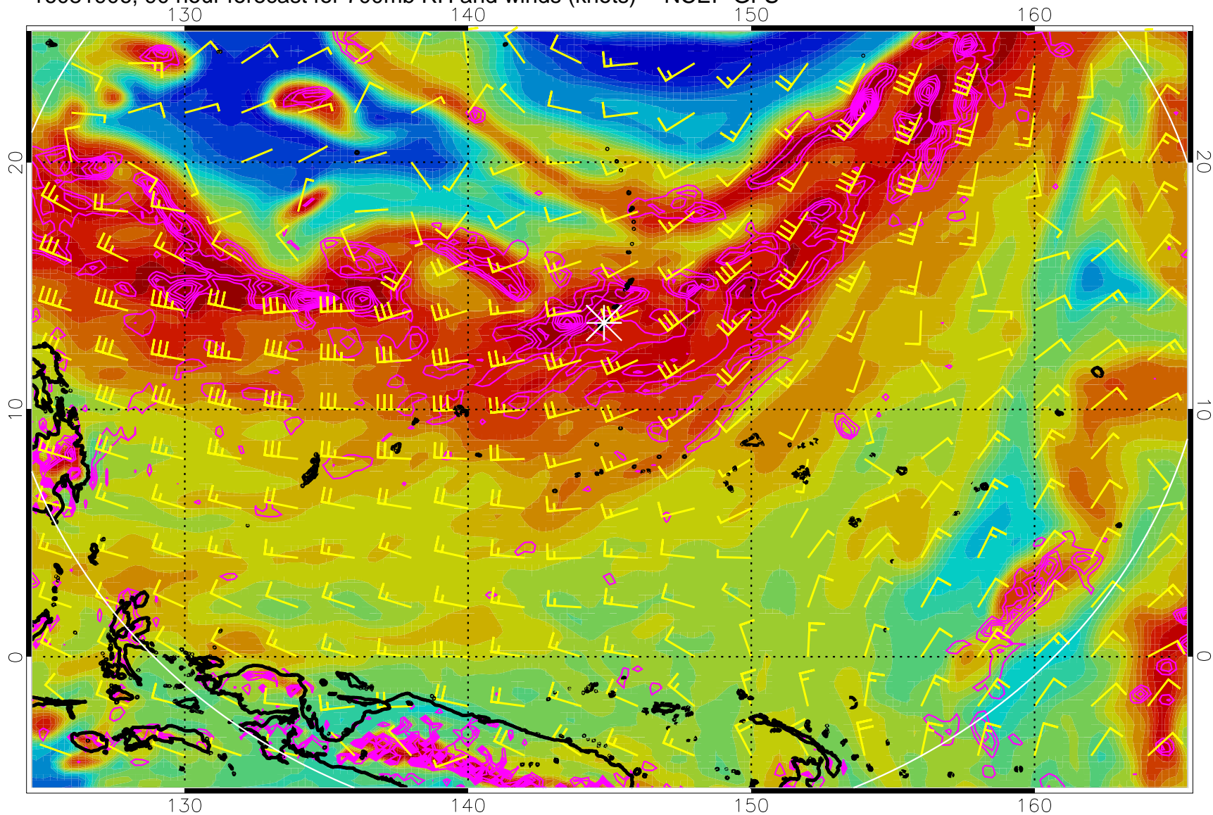
16081906, 90 hour forecast for 700mb RH and winds (knots) -- NCEP GFS
