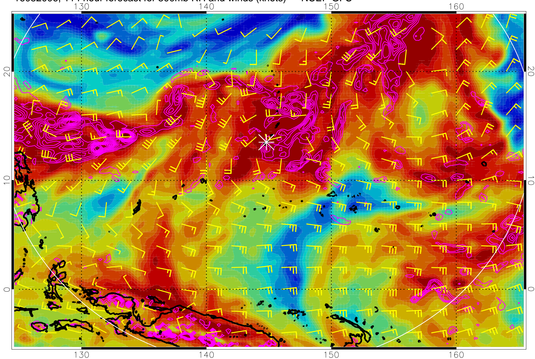
16082006, 114 hour forecast for 500mb RH and winds (knots) -- NCEP GFS
