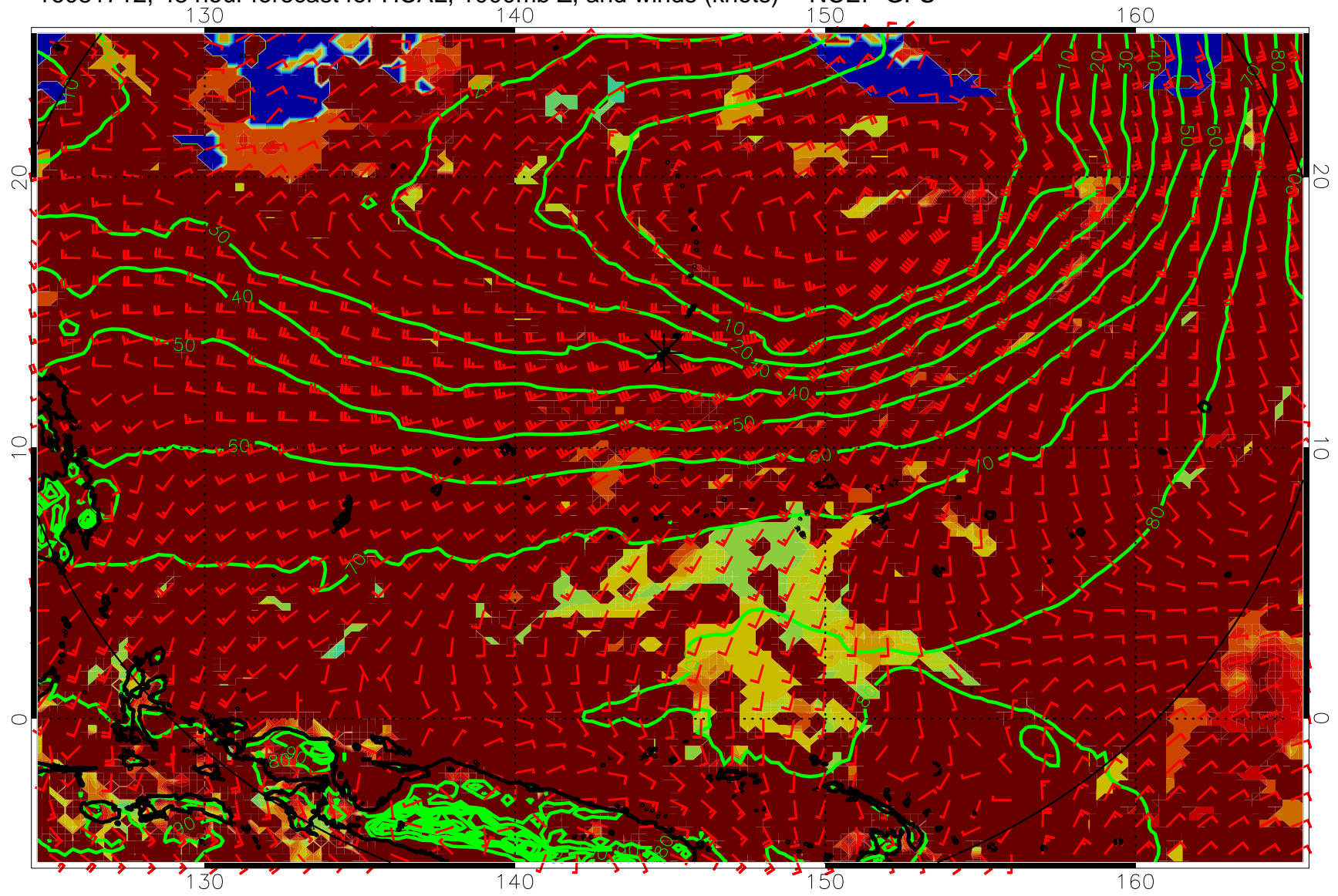
16081712, 48 hour forecast for HCAL, 1000mb Z, and winds (knots) -- NCEP GFS
