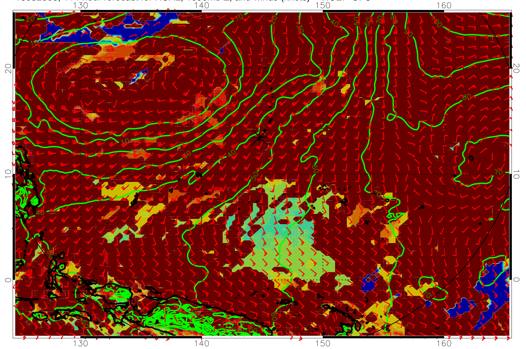
16082006, 114 hour forecast for HCAL, 1000mb Z, and winds (knots) -- NCEP GFS
