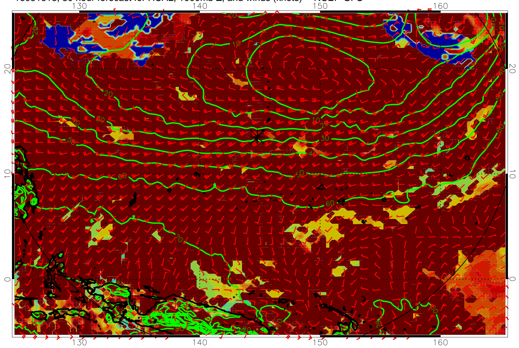
16081618, 30 hour forecast for HCAL, 1000mb Z, and winds (knots) -- NCEP GFS
