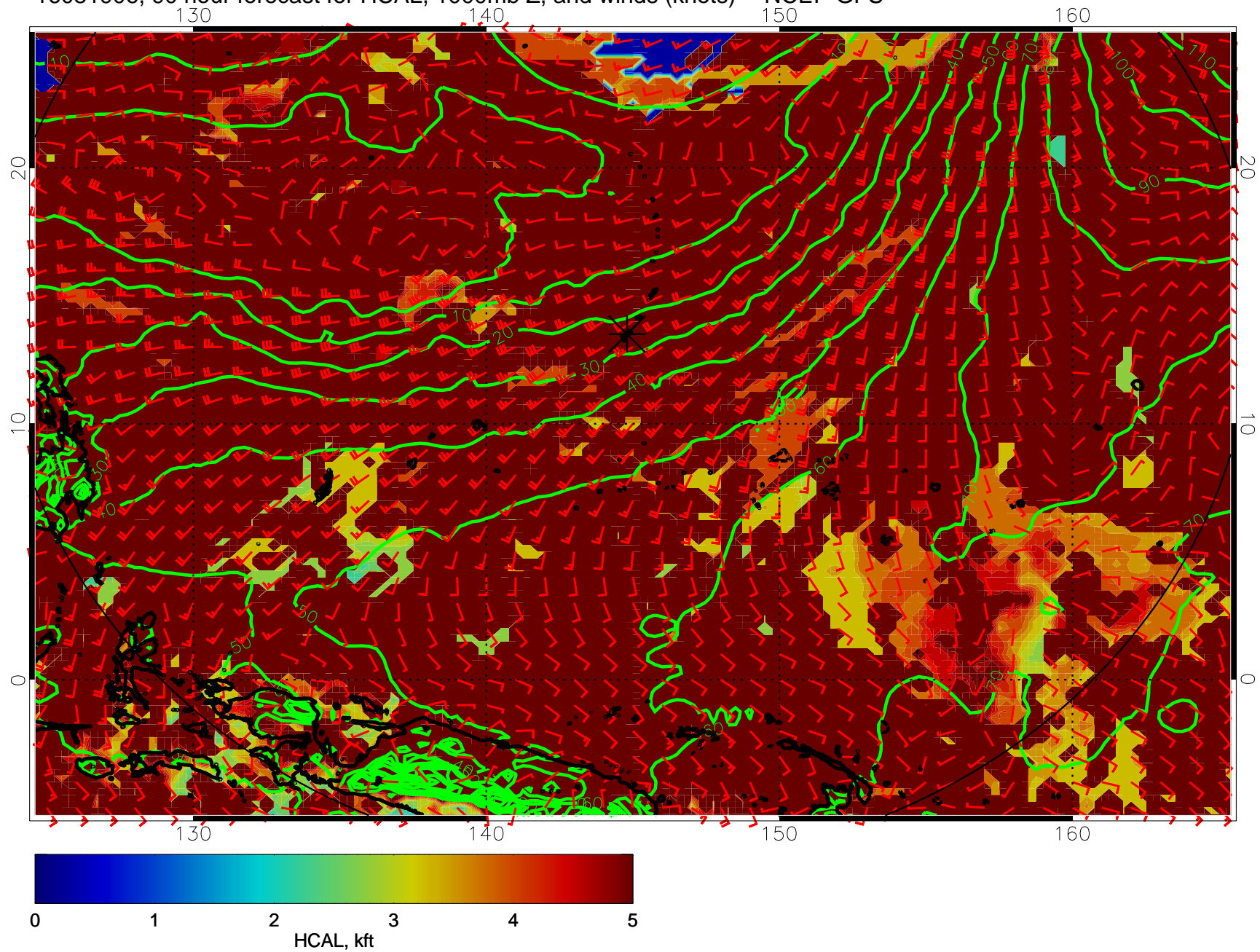
16081906, 90 hour forecast for HCAL, 1000mb Z, and winds (knots) -- NCEP GFS
