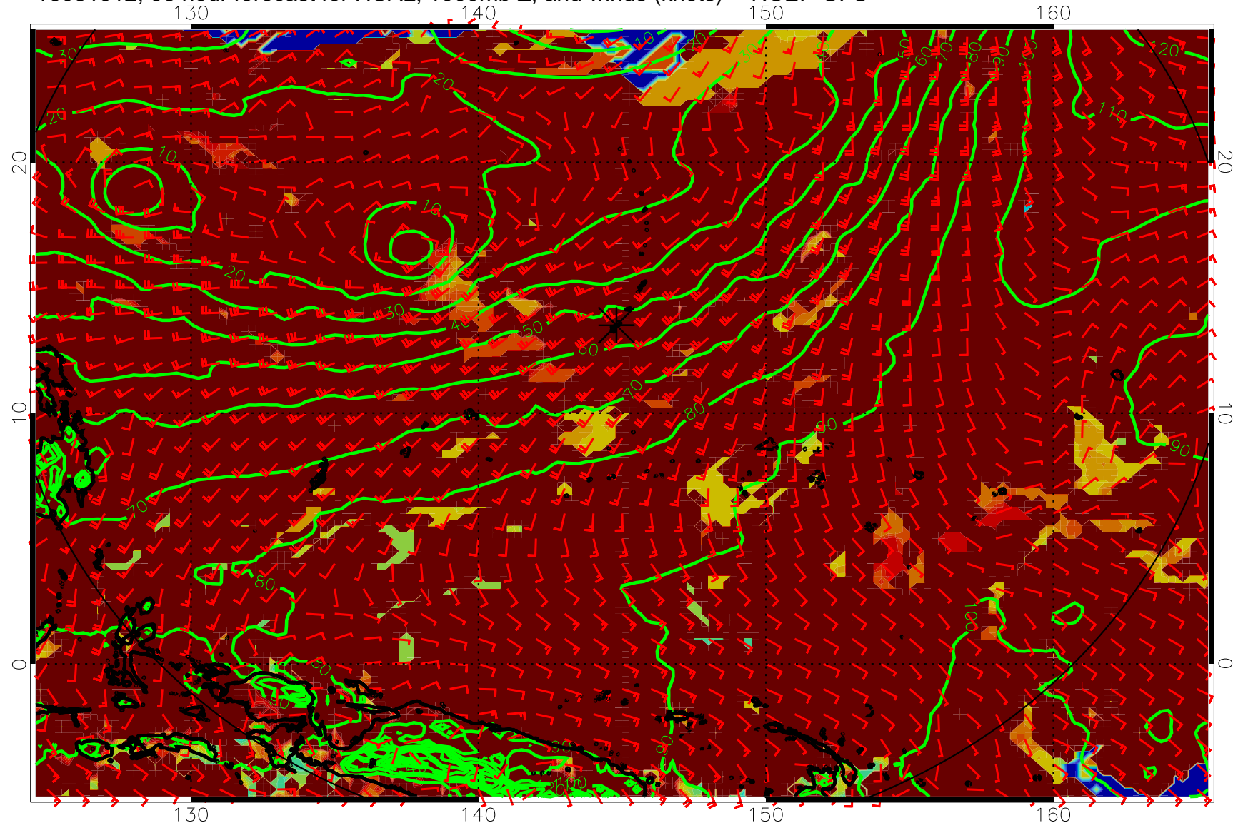
16081912, 96 hour forecast for HCAL, 1000mb Z, and winds (knots) -- NCEP GFS
