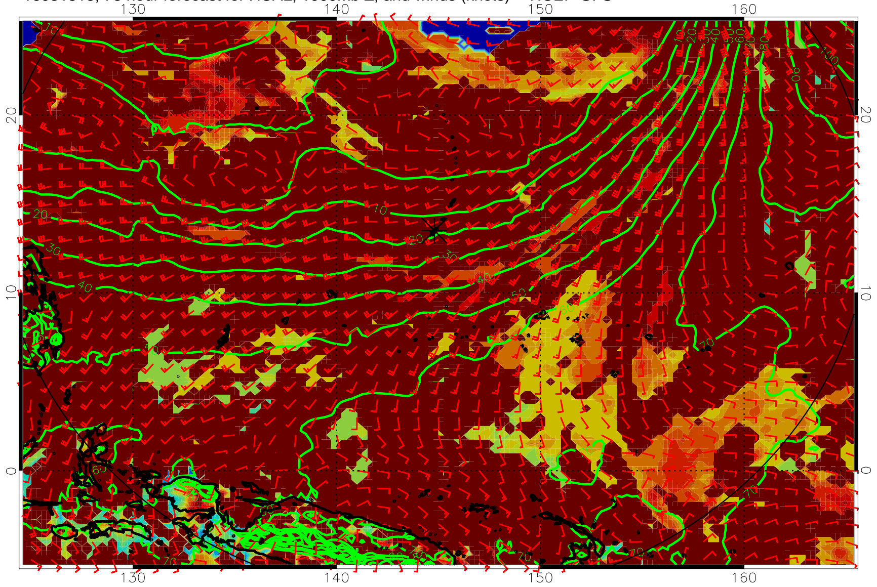
16081818, 78 hour forecast for HCAL, 1000mb Z, and winds (knots) -- NCEP GFS
