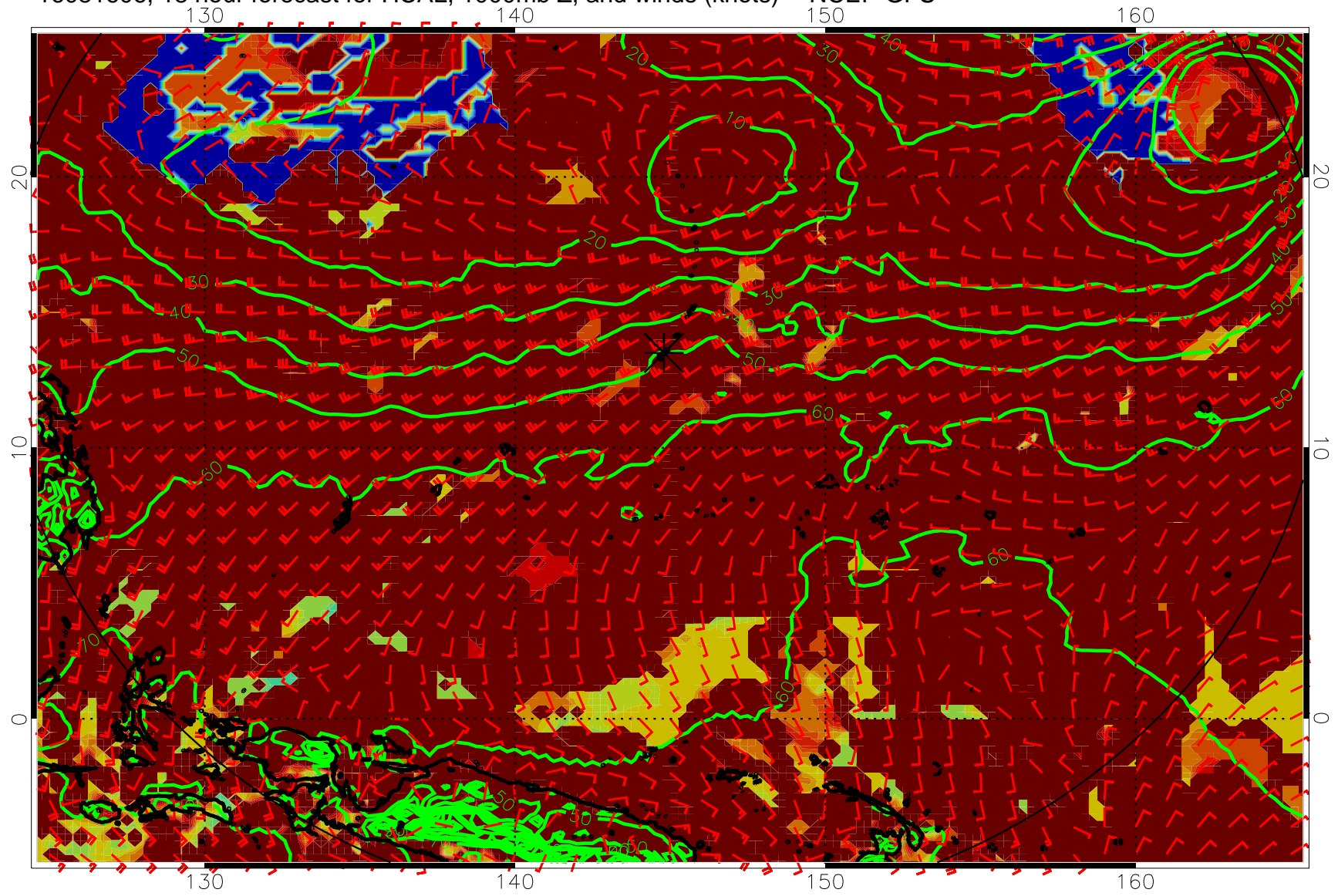
16081606, 18 hour forecast for HCAL, 1000mb Z, and winds (knots) -- NCEP GFS
