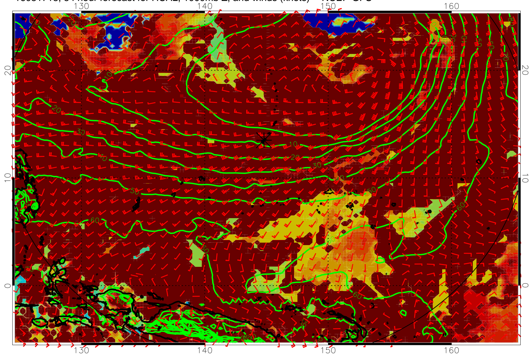
16081718, 54 hour forecast for HCAL, 1000mb Z, and winds (knots) -- NCEP GFS
