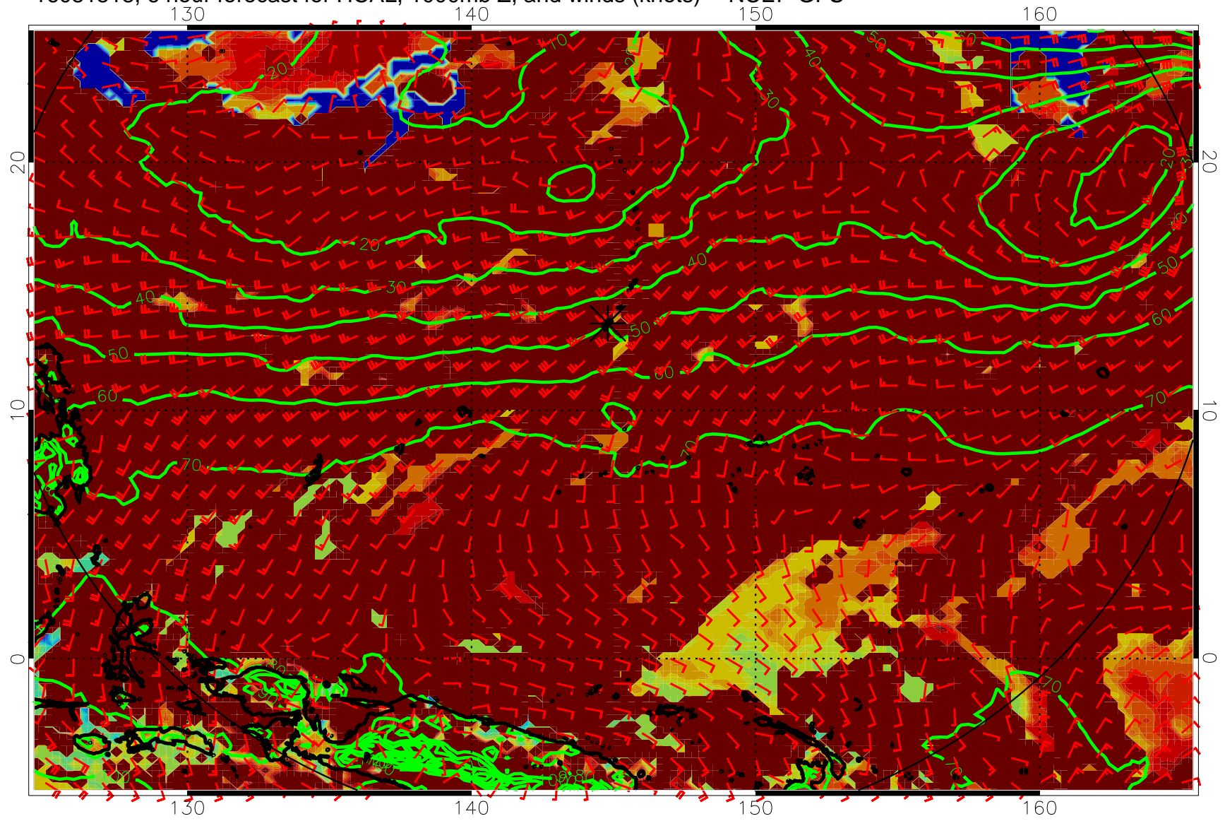
16081518, 6 hour forecast for HCAL, 1000mb Z, and winds (knots) -- NCEP GFS
