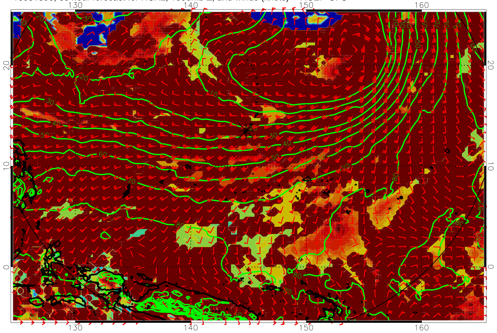
16081800, 60 hour forecast for HCAL, 1000mb Z, and winds (knots) -- NCEP GFS
