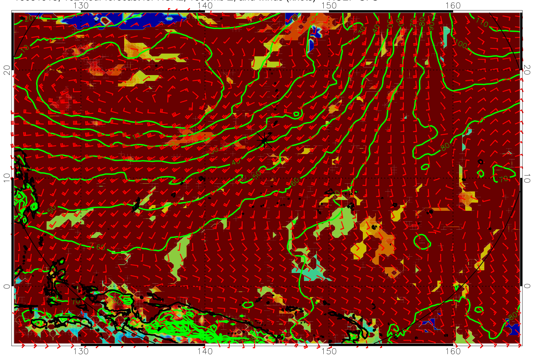
16081918, 102 hour forecast for HCAL, 1000mb Z, and winds (knots) -- NCEP GFS
