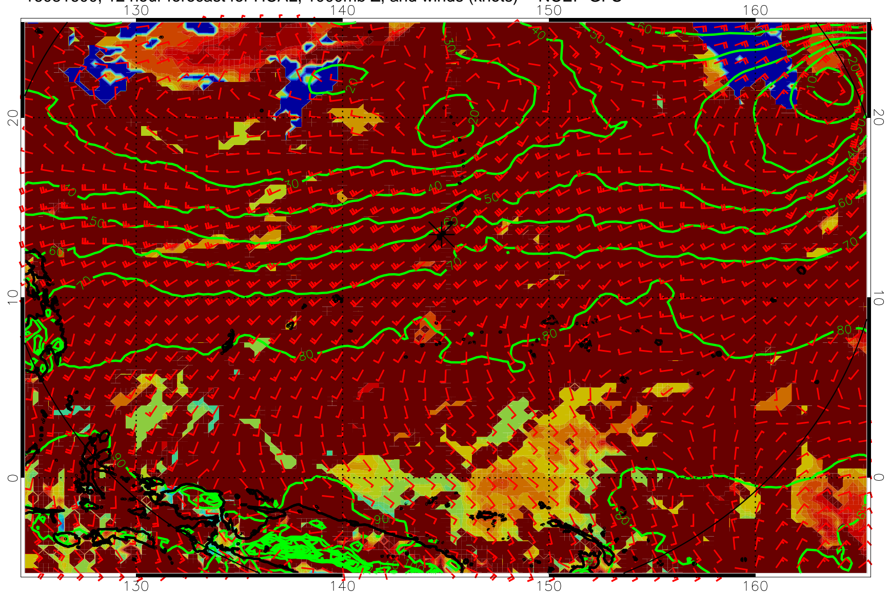
16081600, 12 hour forecast for HCAL, 1000mb Z, and winds (knots) -- NCEP GFS
