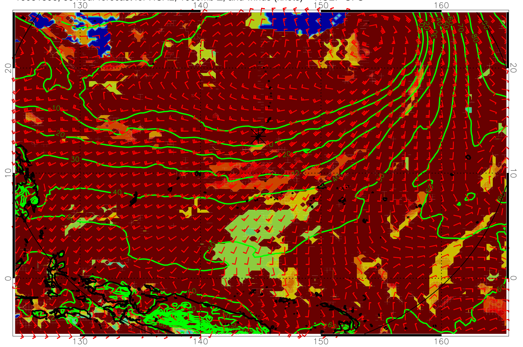
16081806, 66 hour forecast for HCAL, 1000mb Z, and winds (knots) -- NCEP GFS
