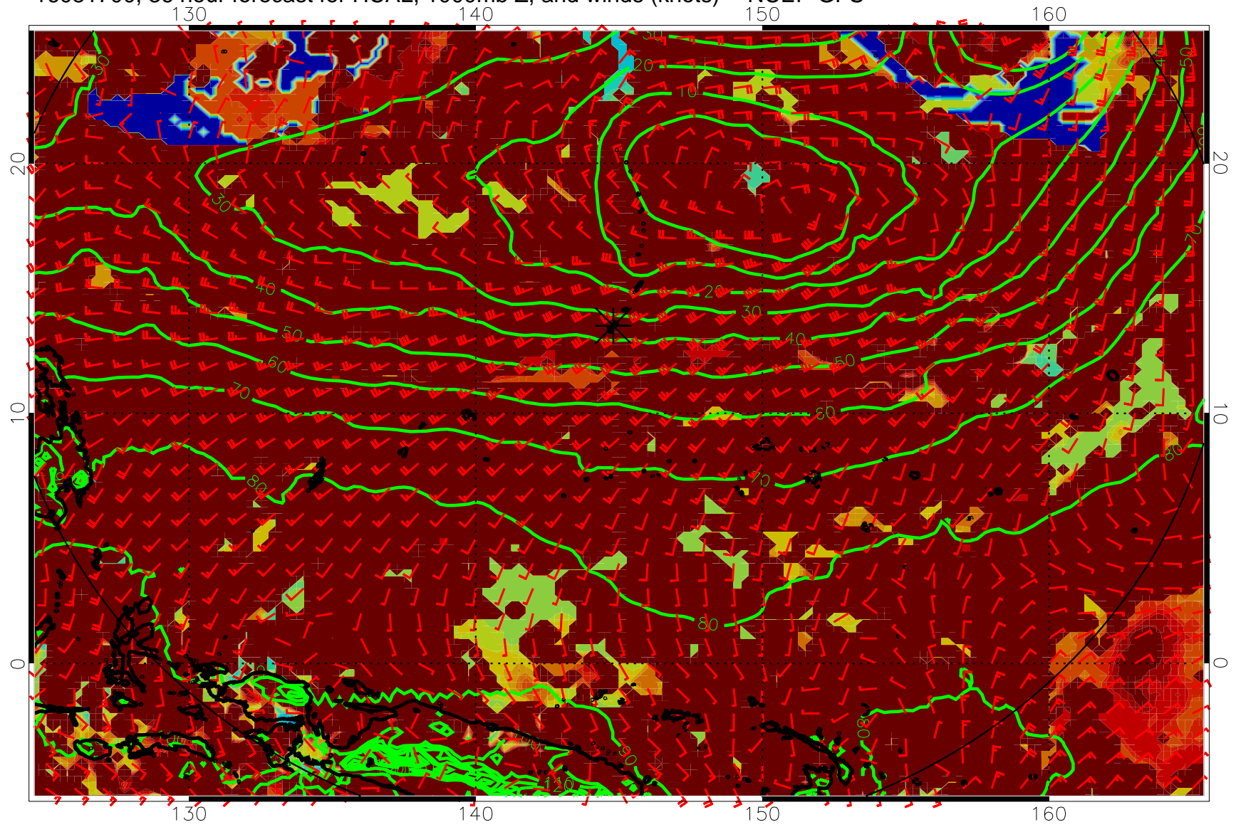
16081700, 36 hour forecast for HCAL, 1000mb Z, and winds (knots) -- NCEP GFS
