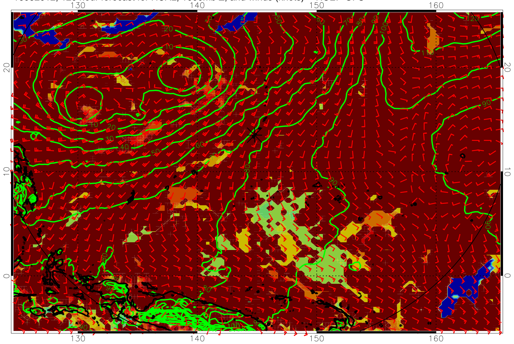
16082012, 120 hour forecast for HCAL, 1000mb Z, and winds (knots) -- NCEP GFS
