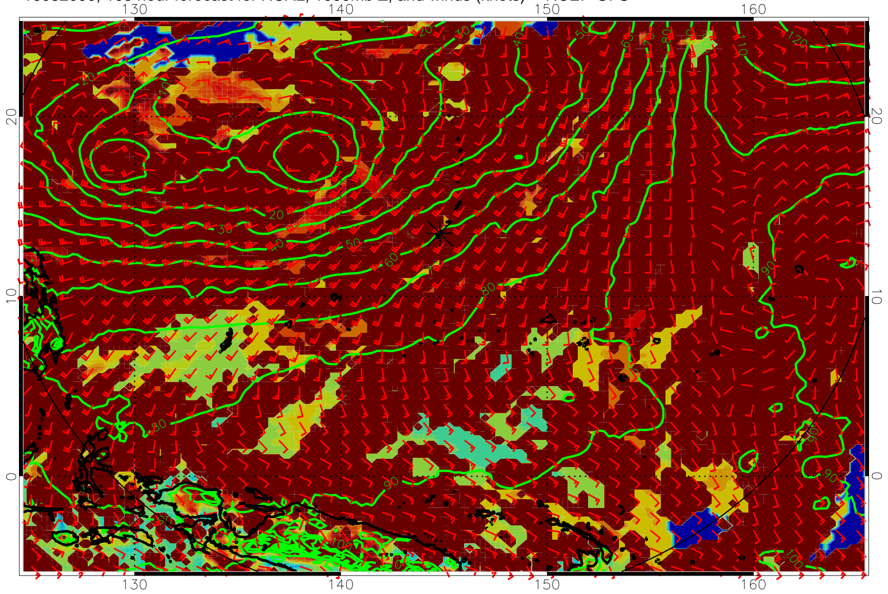
16082000, 108 hour forecast for HCAL, 1000mb Z, and winds (knots) -- NCEP GFS
