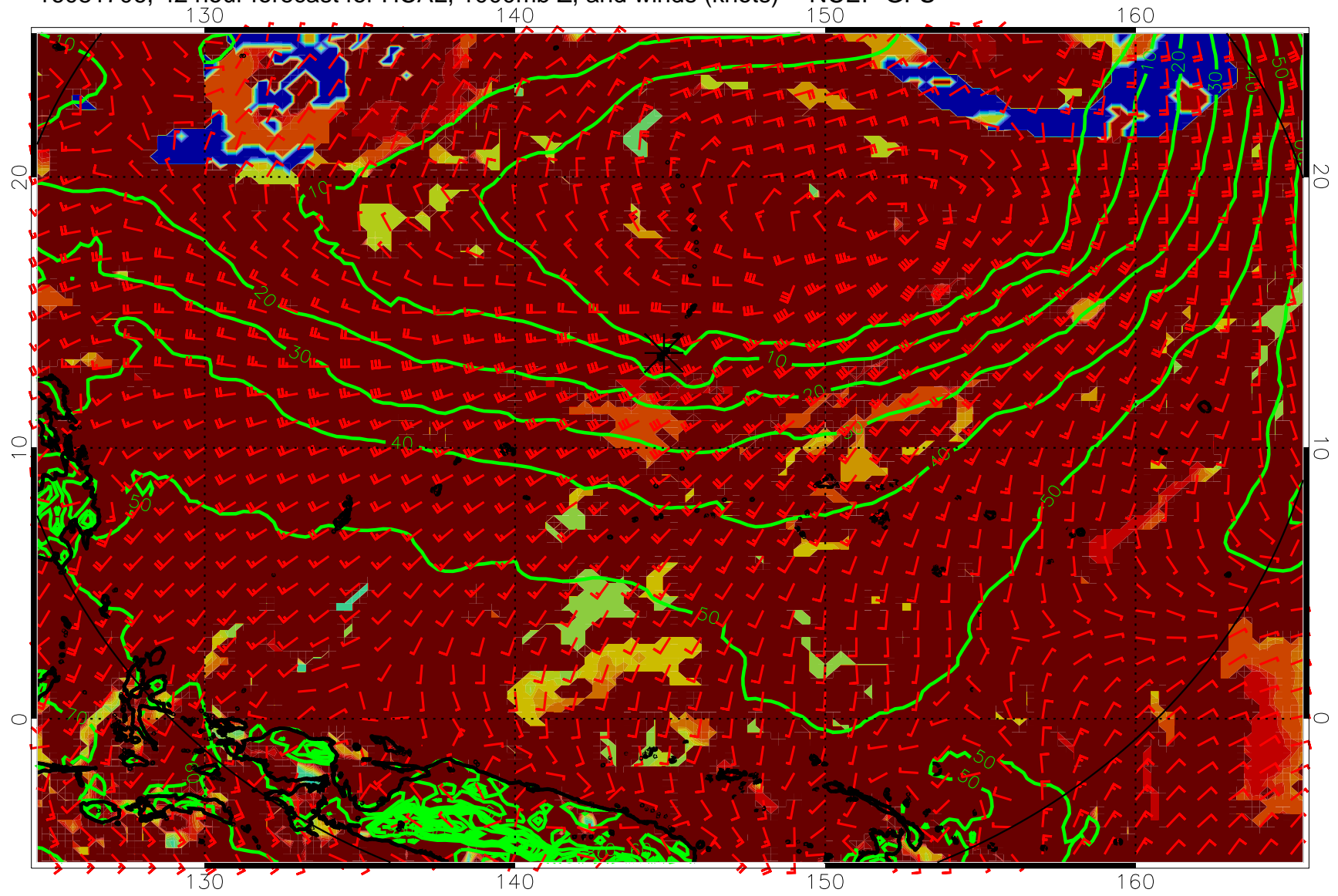
16081706, 42 hour forecast for HCAL, 1000mb Z, and winds (knots) -- NCEP GFS
