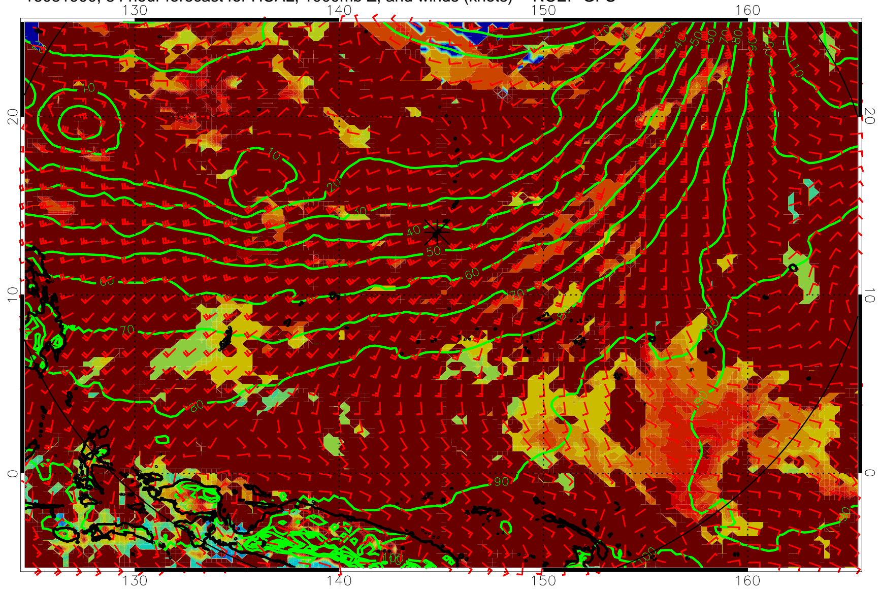
16081900, 84 hour forecast for HCAL, 1000mb Z, and winds (knots) -- NCEP GFS
