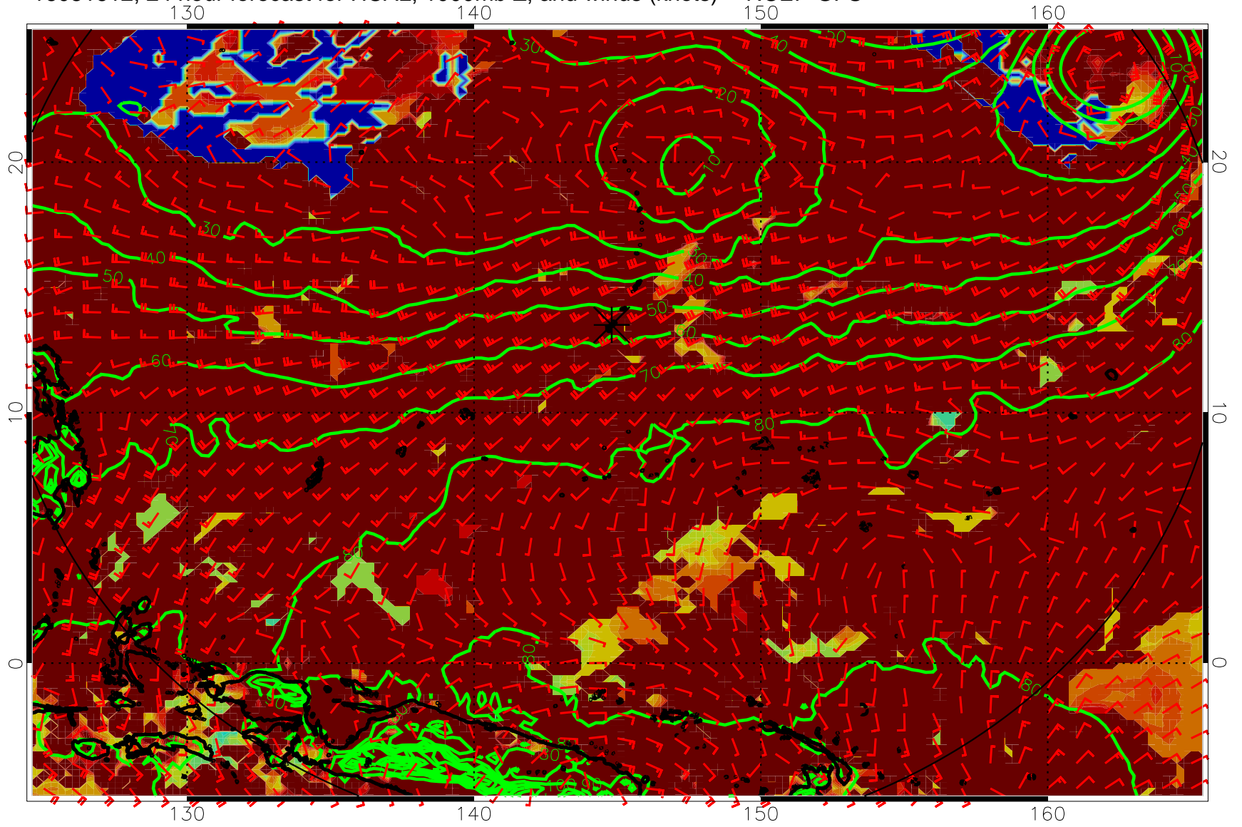
16081612, 24 hour forecast for HCAL, 1000mb Z, and winds (knots) -- NCEP GFS
