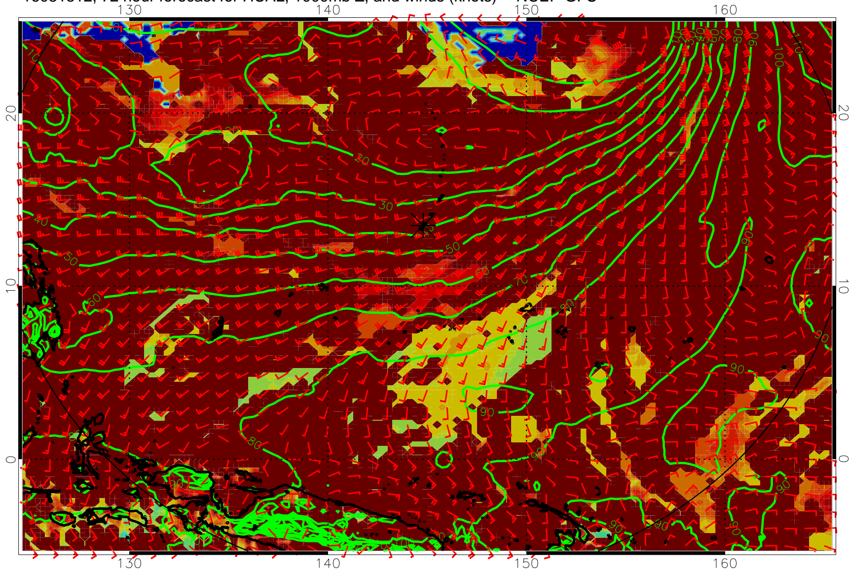
16081812, 72 hour forecast for HCAL, 1000mb Z, and winds (knots) -- NCEP GFS
