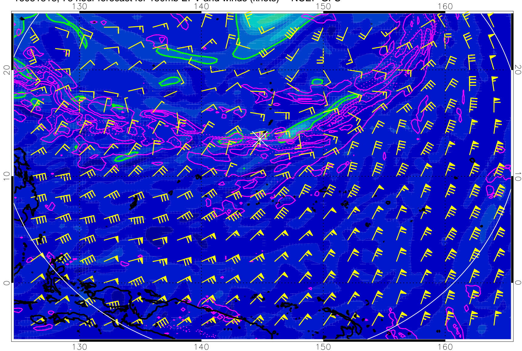
16081818, 78 hour forecast for 150mb EPV and winds (knots) -- NCEP GFS
