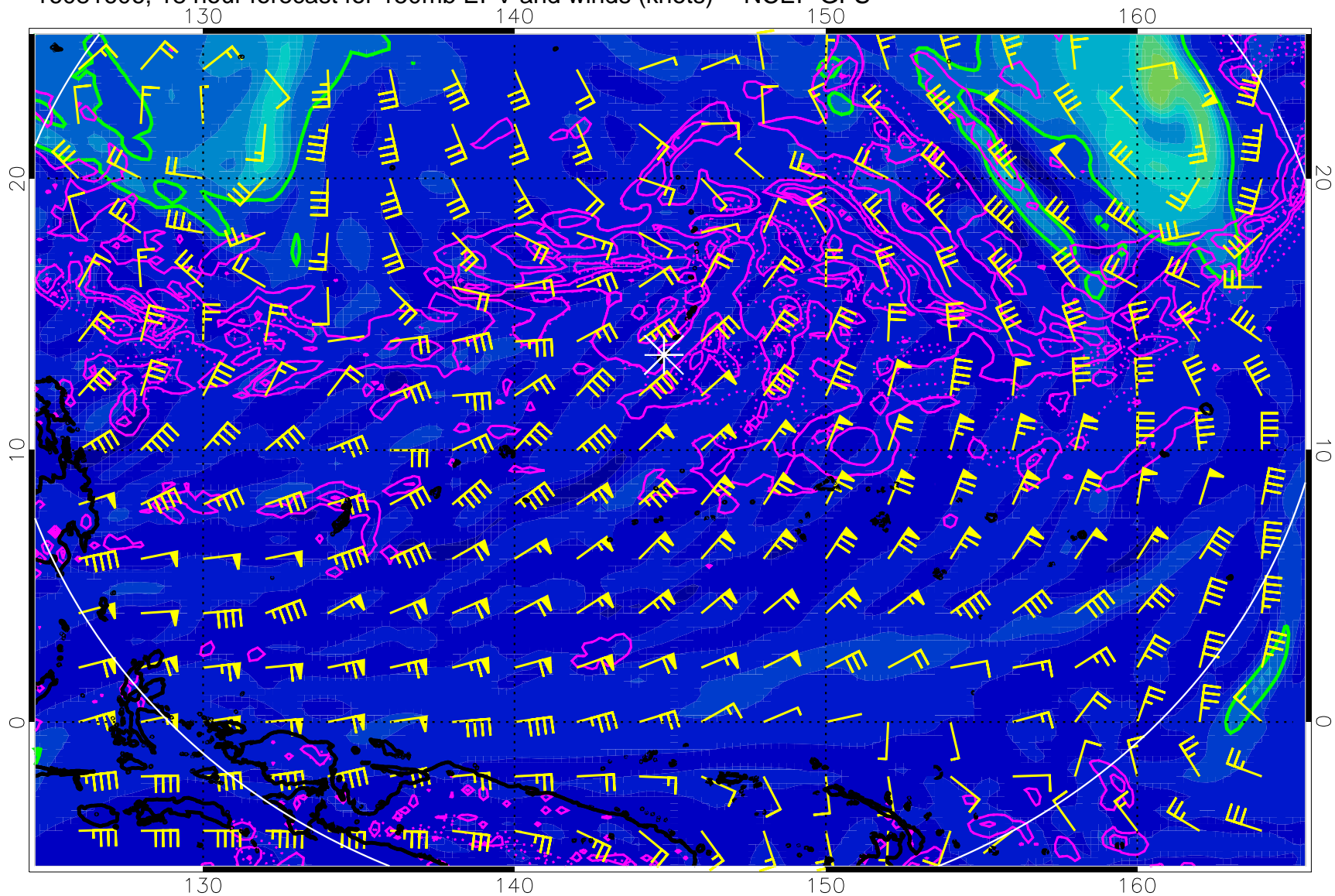
16081606, 18 hour forecast for 150mb EPV and winds (knots) -- NCEP GFS
