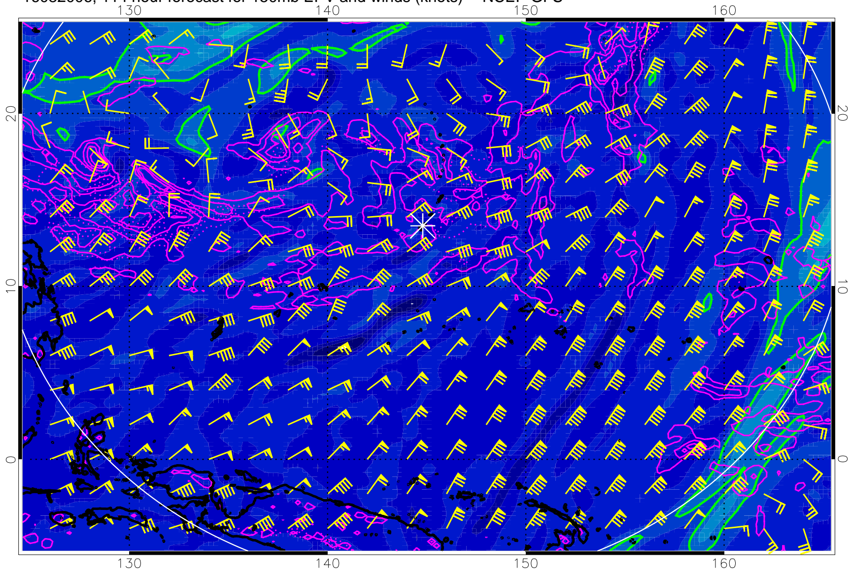
16082006, 114 hour forecast for 150mb EPV and winds (knots) -- NCEP GFS
