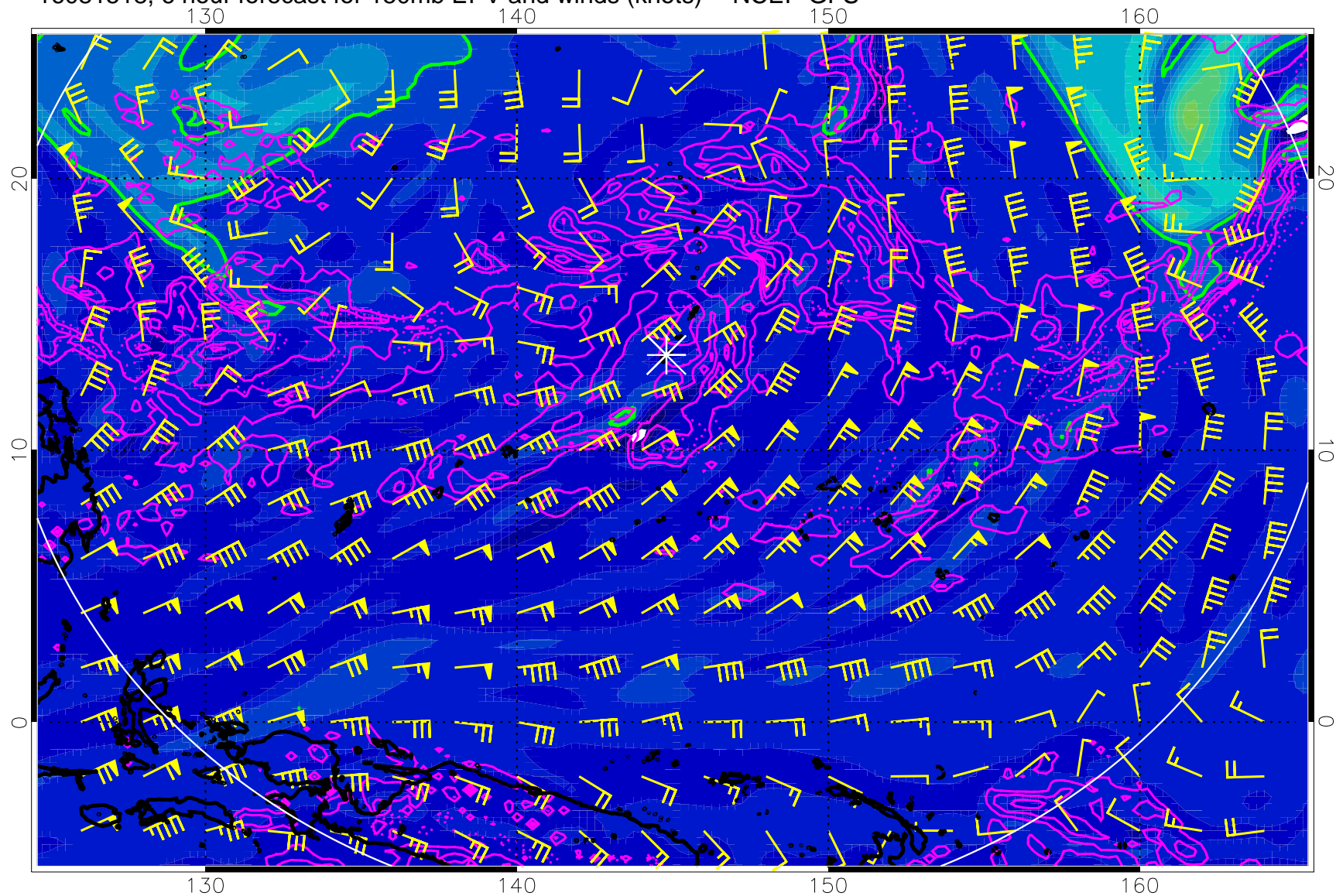
16081518, 6 hour forecast for 150mb EPV and winds (knots) -- NCEP GFS
