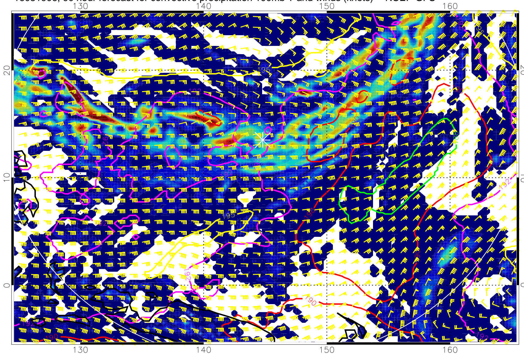
16081906, 90 hour forecast for convective precipitation 100mb T and winds (knots) -- NCEP GFS
