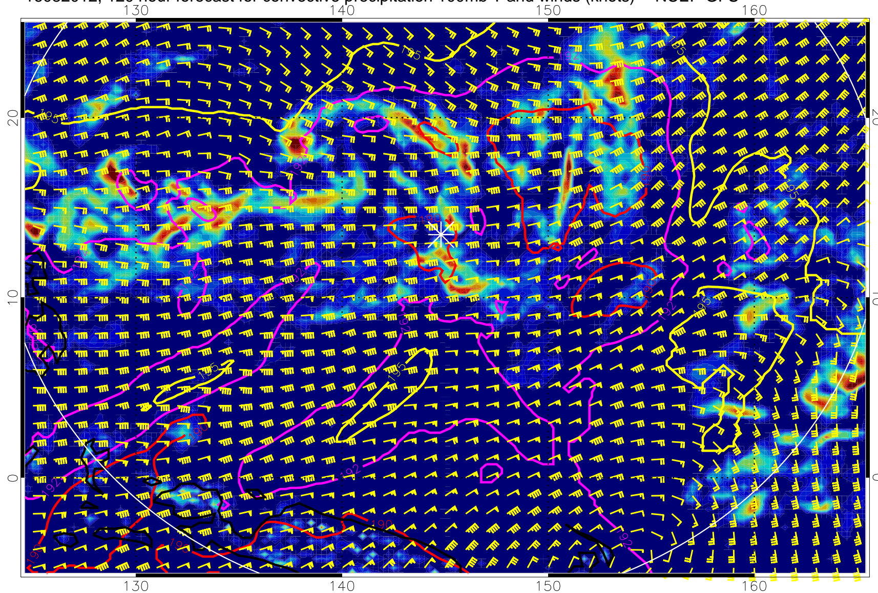
16082012, 120 hour forecast for convective precipitation 100mb T and winds (knots) -- NCEP GFS
