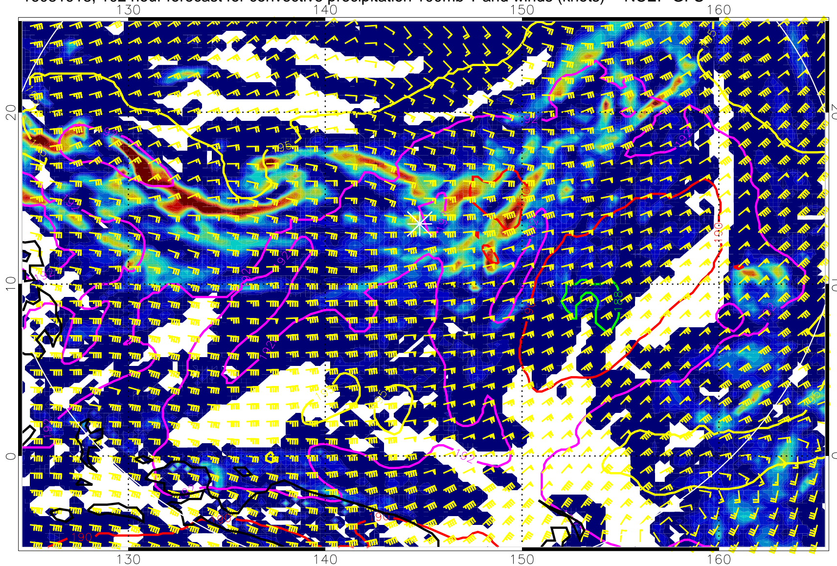
16081918, 102 hour forecast for convective precipitation 100mb T and winds (knots) -- NCEP GFS
