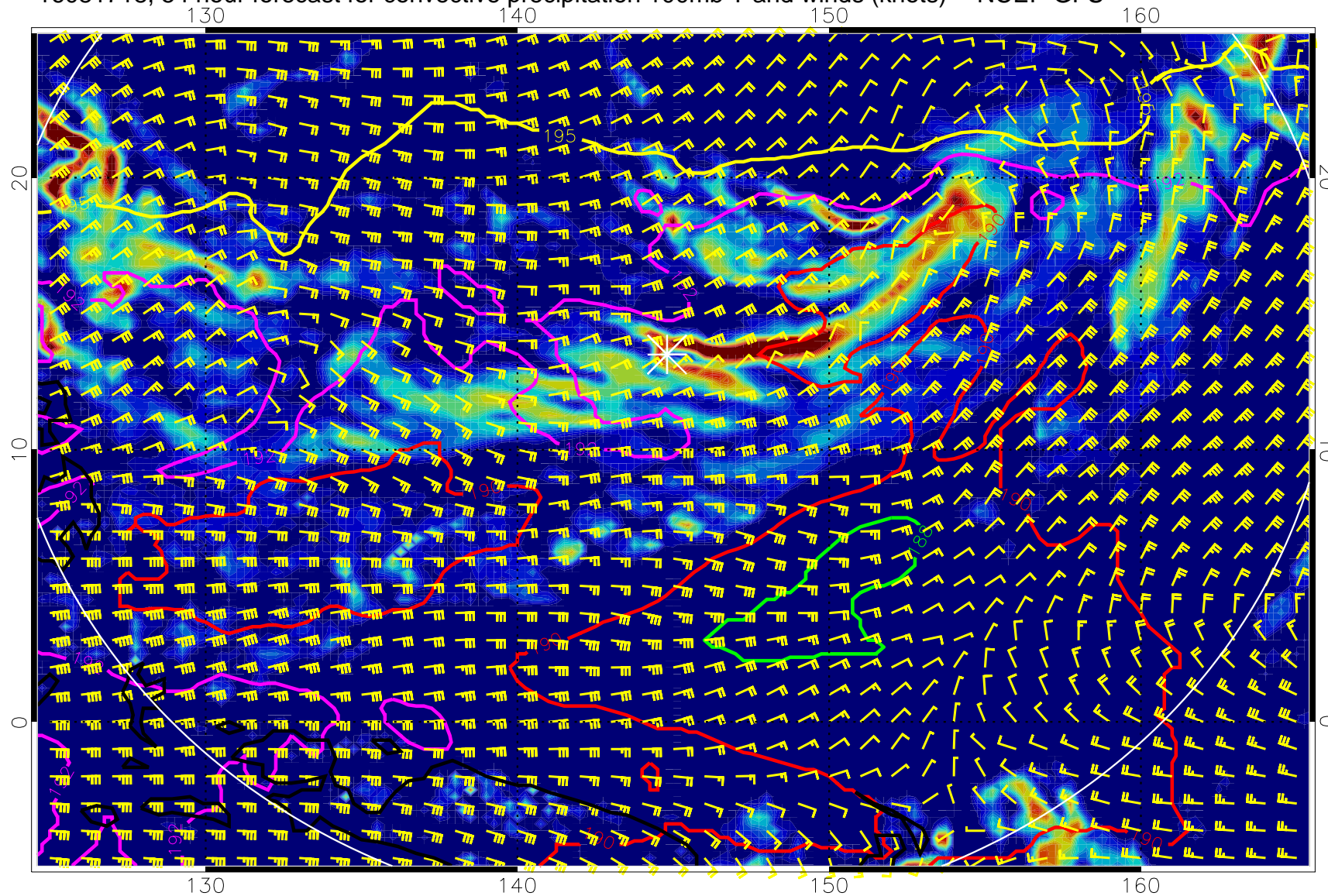
16081718, 54 hour forecast for convective precipitation 100mb T and winds (knots) -- NCEP GFS
