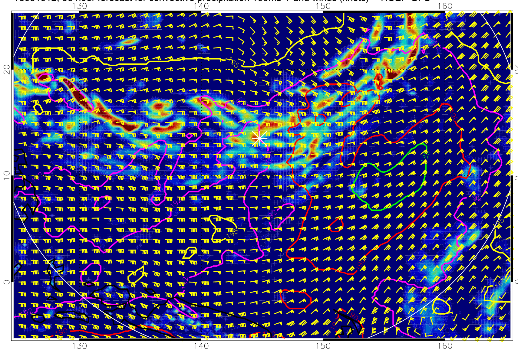
16081912, 96 hour forecast for convective precipitation 100mb T and winds (knots) -- NCEP GFS
