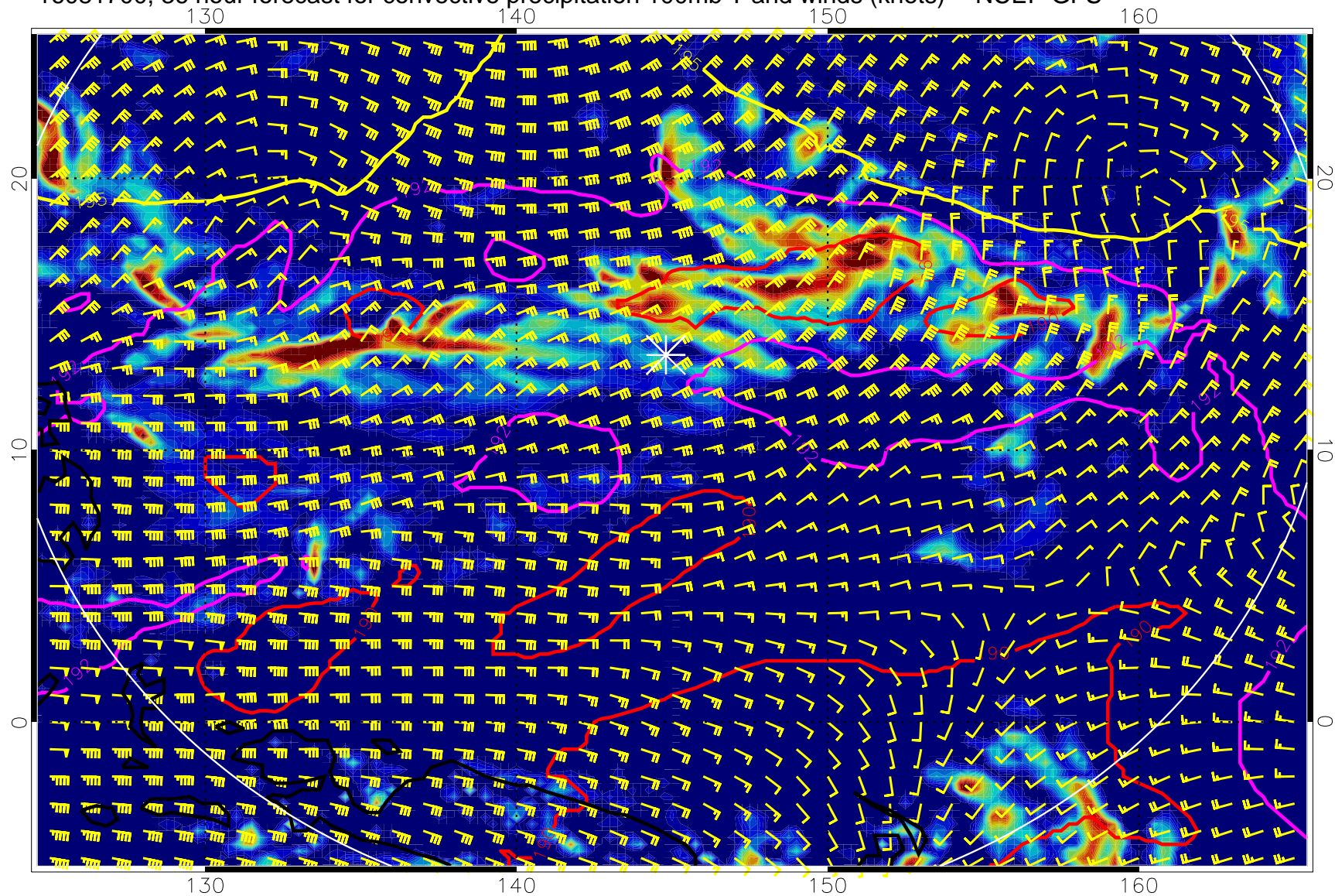
16081700, 36 hour forecast for convective precipitation 100mb T and winds (knots) -- NCEP GFS
