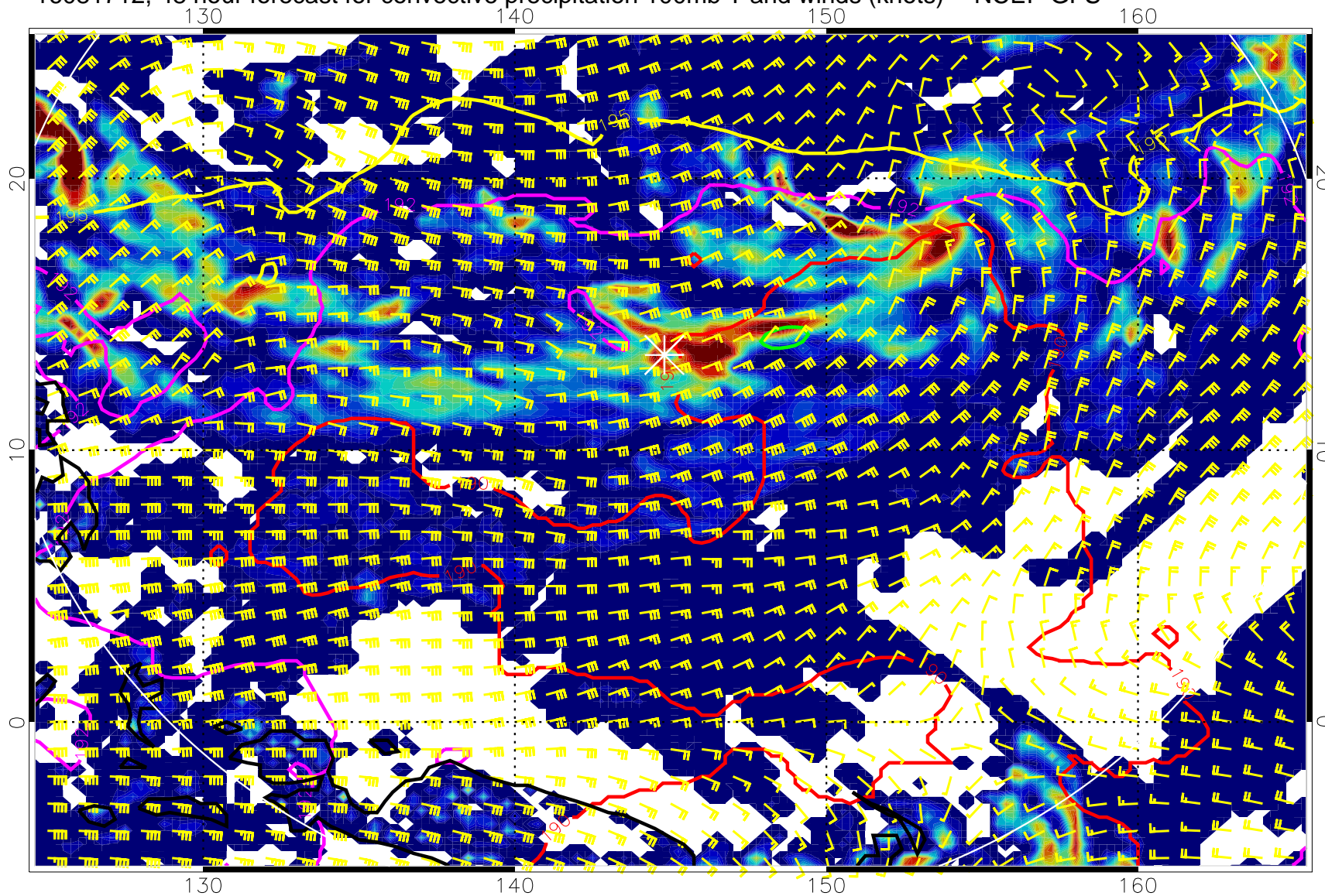
16081712, 48 hour forecast for convective precipitation 100mb T and winds (knots) -- NCEP GFS
