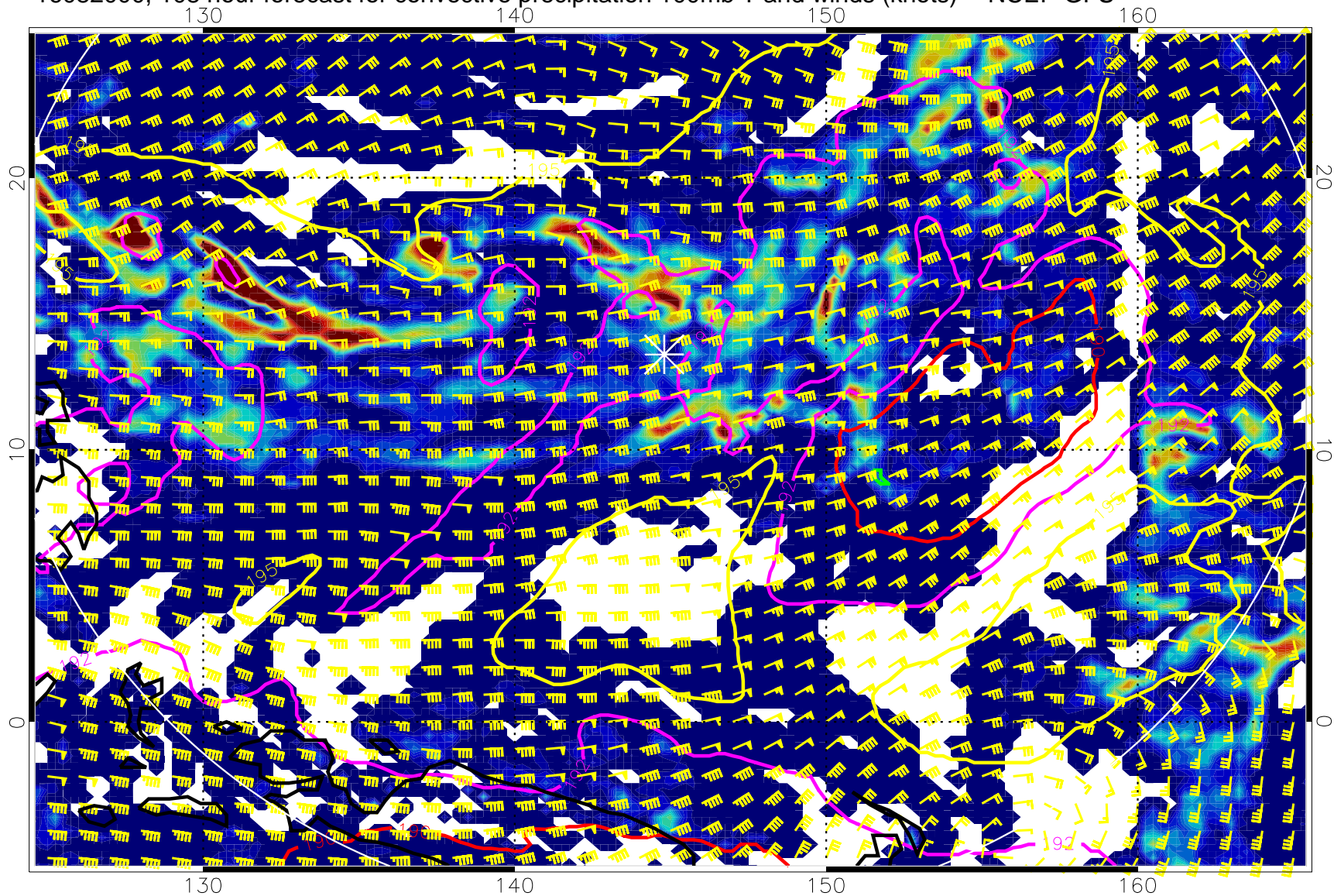
16082000, 108 hour forecast for convective precipitation 100mb T and winds (knots) -- NCEP GFS
