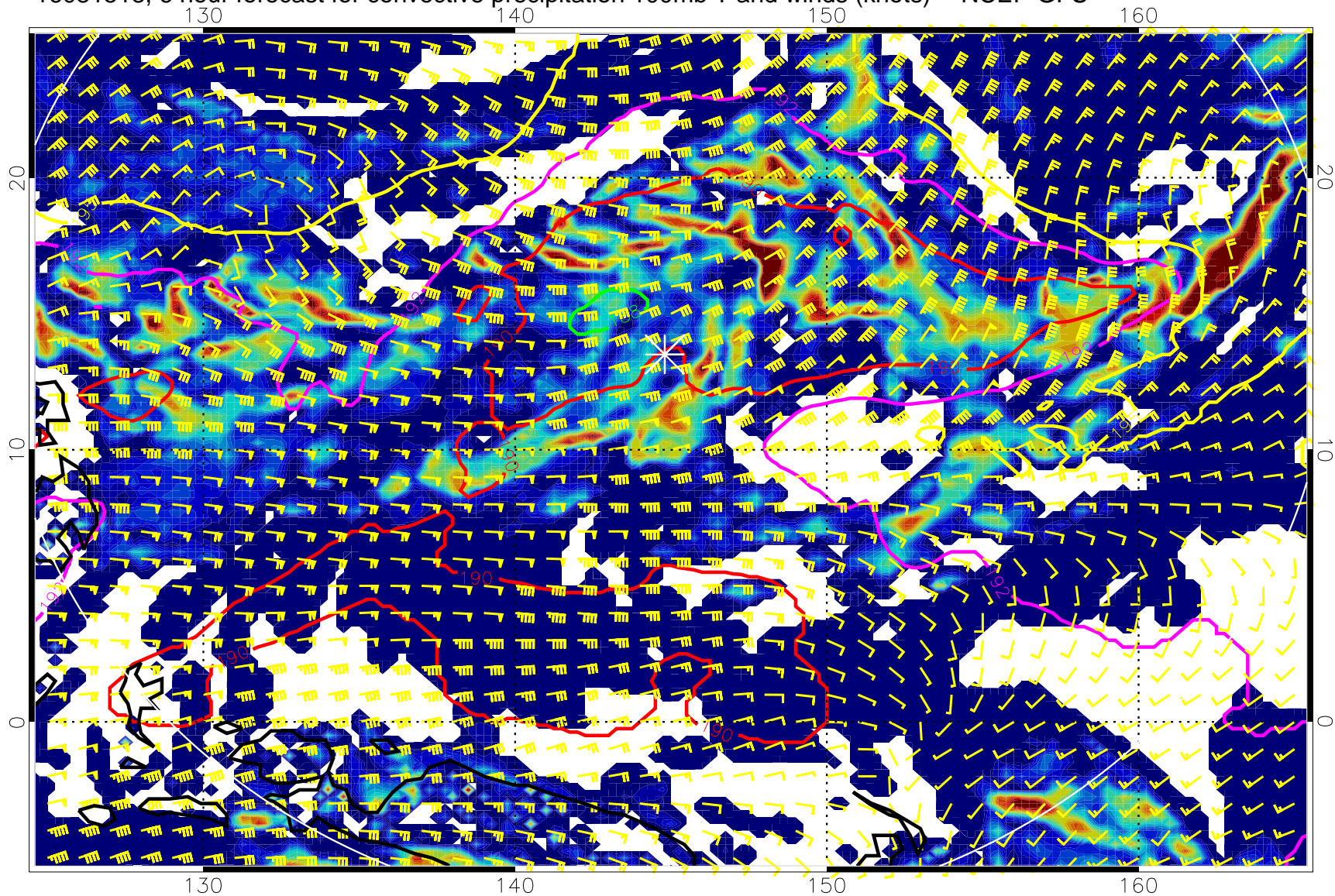
16081518, 6 hour forecast for convective precipitation 100mb T and winds (knots) -- NCEP GFS
