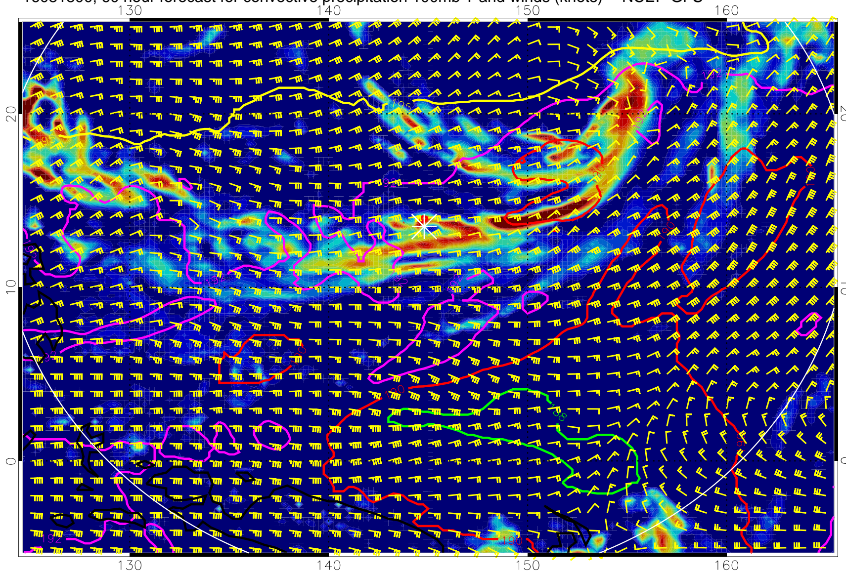
16081800, 60 hour forecast for convective precipitation 100mb T and winds (knots) -- NCEP GFS
