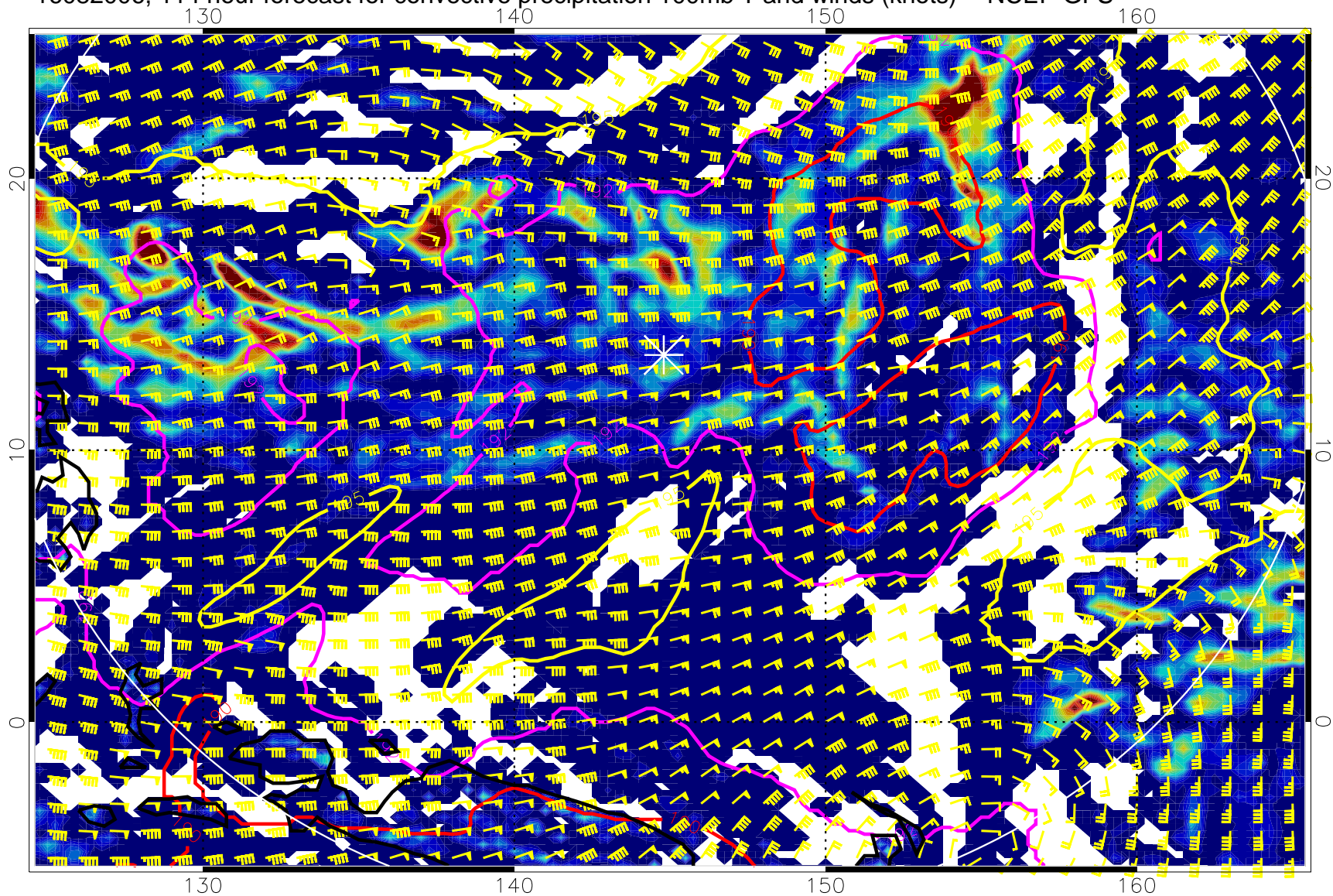
16082006, 114 hour forecast for convective precipitation 100mb T and winds (knots) -- NCEP GFS
