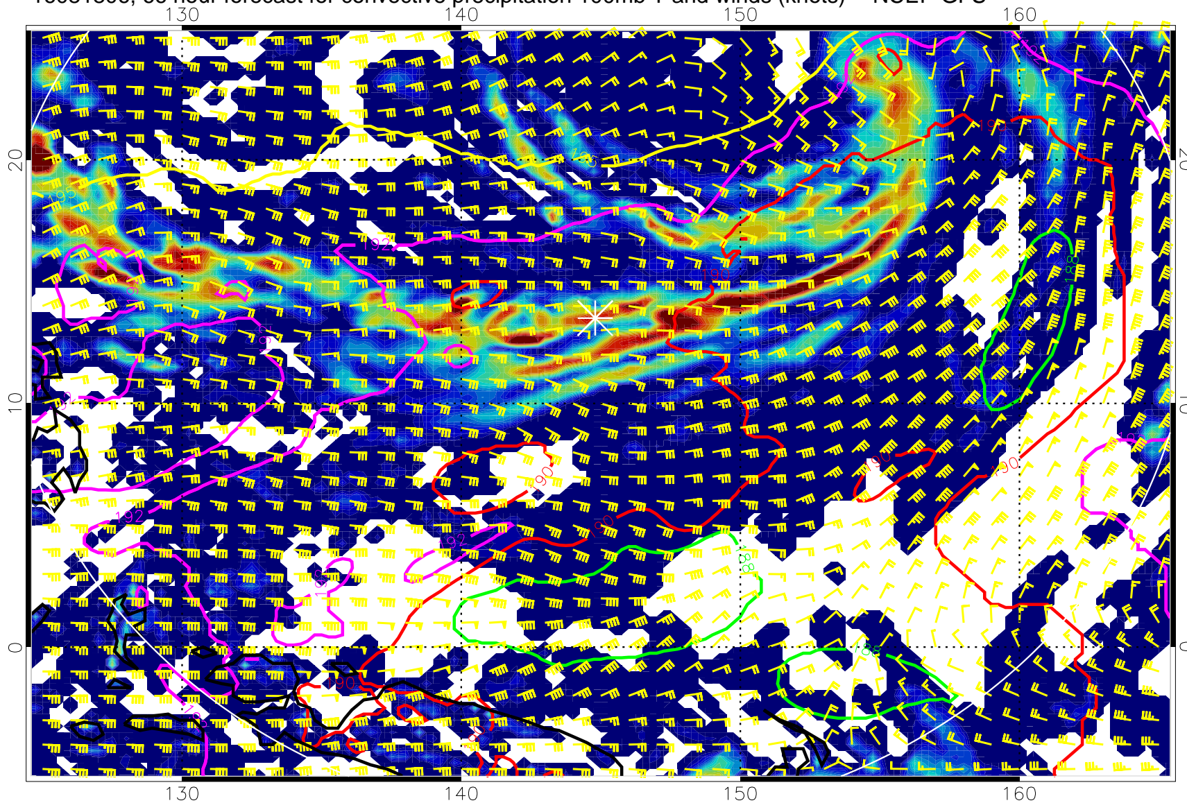
16081806, 66 hour forecast for convective precipitation 100mb T and winds (knots) -- NCEP GFS
