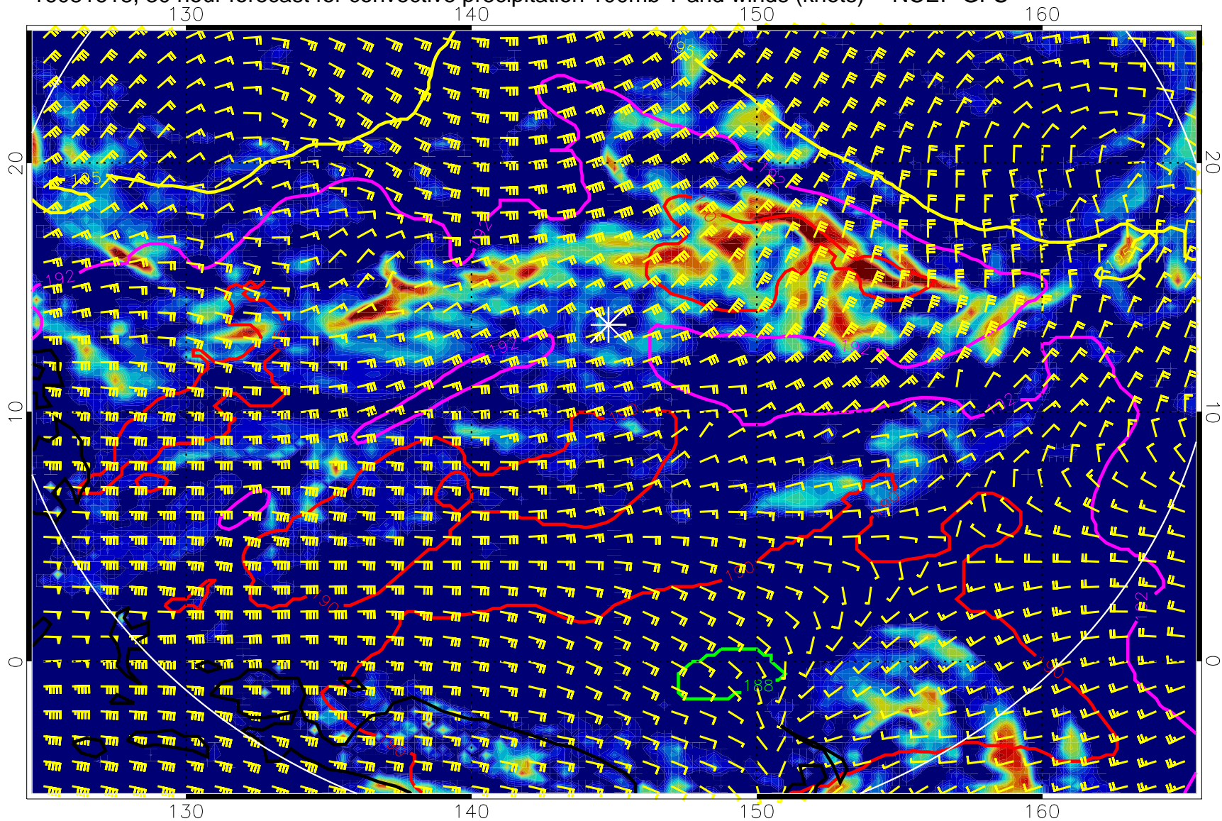
16081618, 30 hour forecast for convective precipitation 100mb T and winds (knots) -- NCEP GFS
