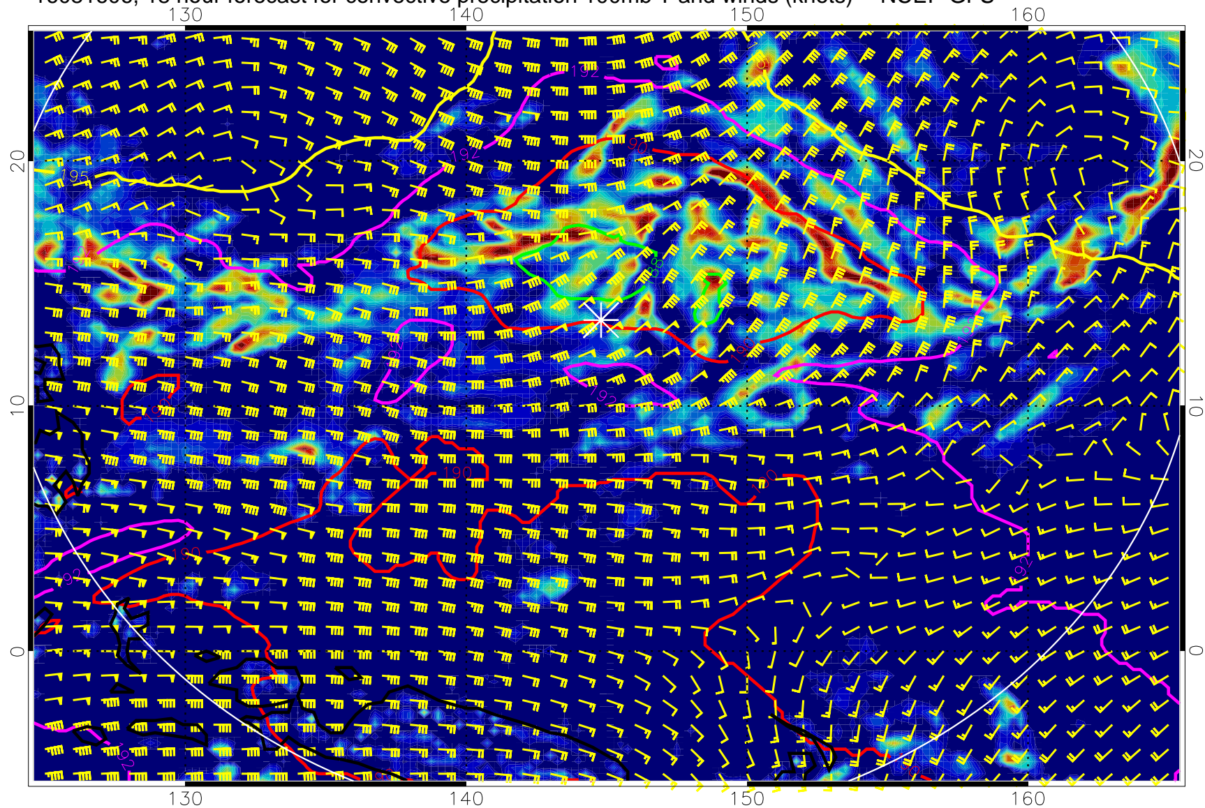
16081606, 18 hour forecast for convective precipitation 100mb T and winds (knots) -- NCEP GFS
