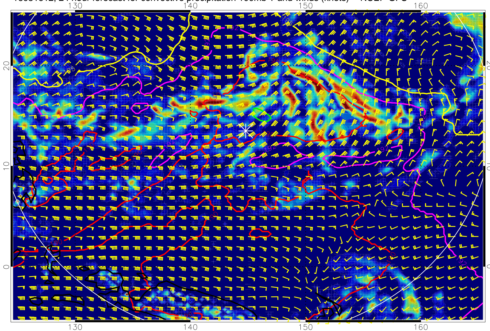
16081612, 24 hour forecast for convective precipitation 100mb T and winds (knots) -- NCEP GFS
