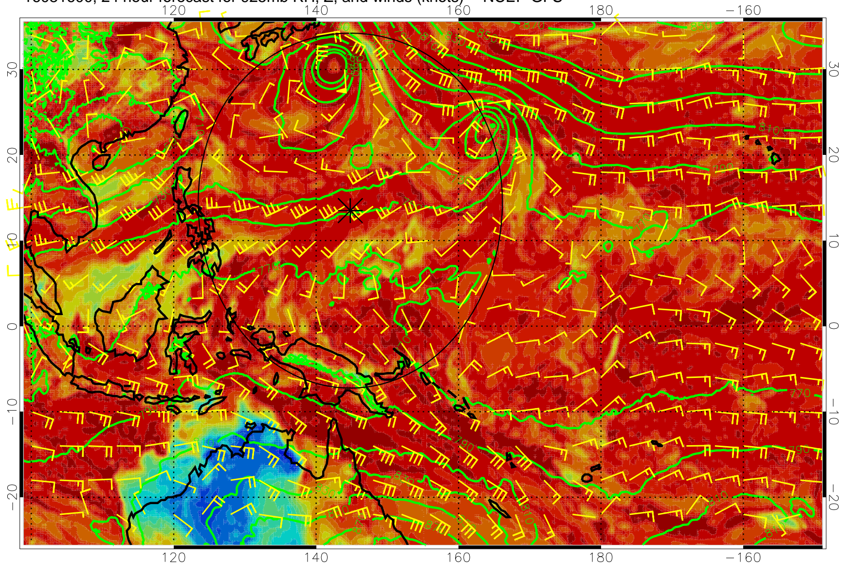
16081600, 24 hour forecast for 925mb RH, Z, and winds (knots) -- NCEP GFS
