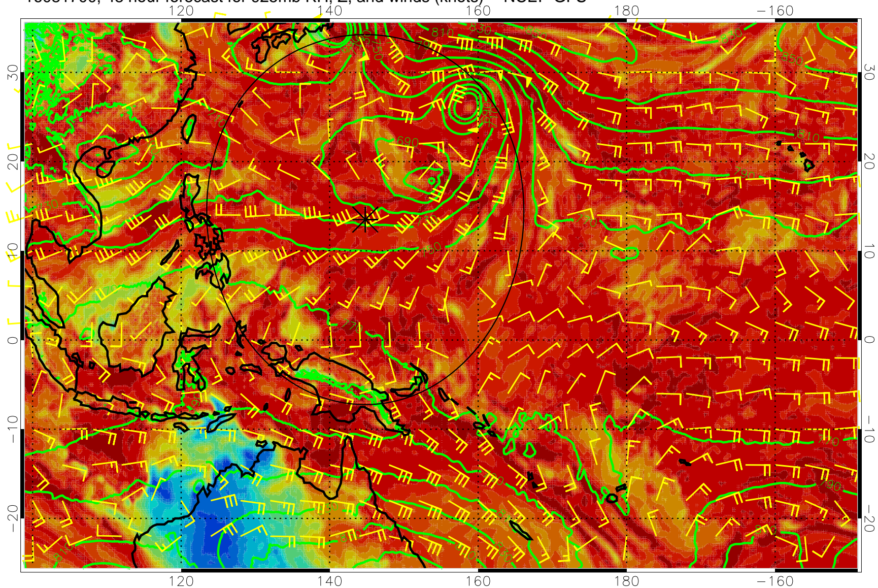
16081700, 48 hour forecast for 925mb RH, Z, and winds (knots) -- NCEP GFS
