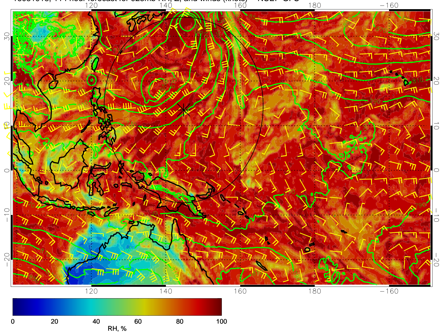
16081918, 114 hour forecast for 925mb RH, Z, and winds (knots) -- NCEP GFS
