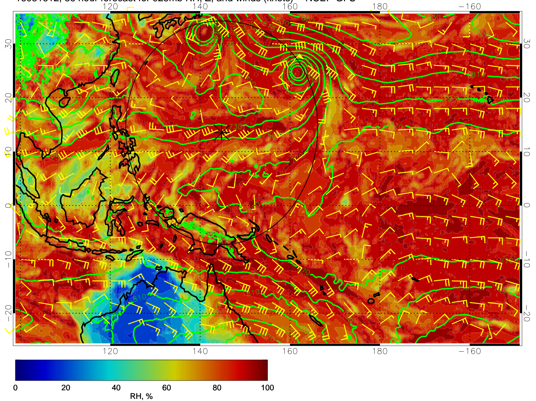
16081612, 36 hour forecast for 925mb RH, Z, and winds (knots) -- NCEP GFS
