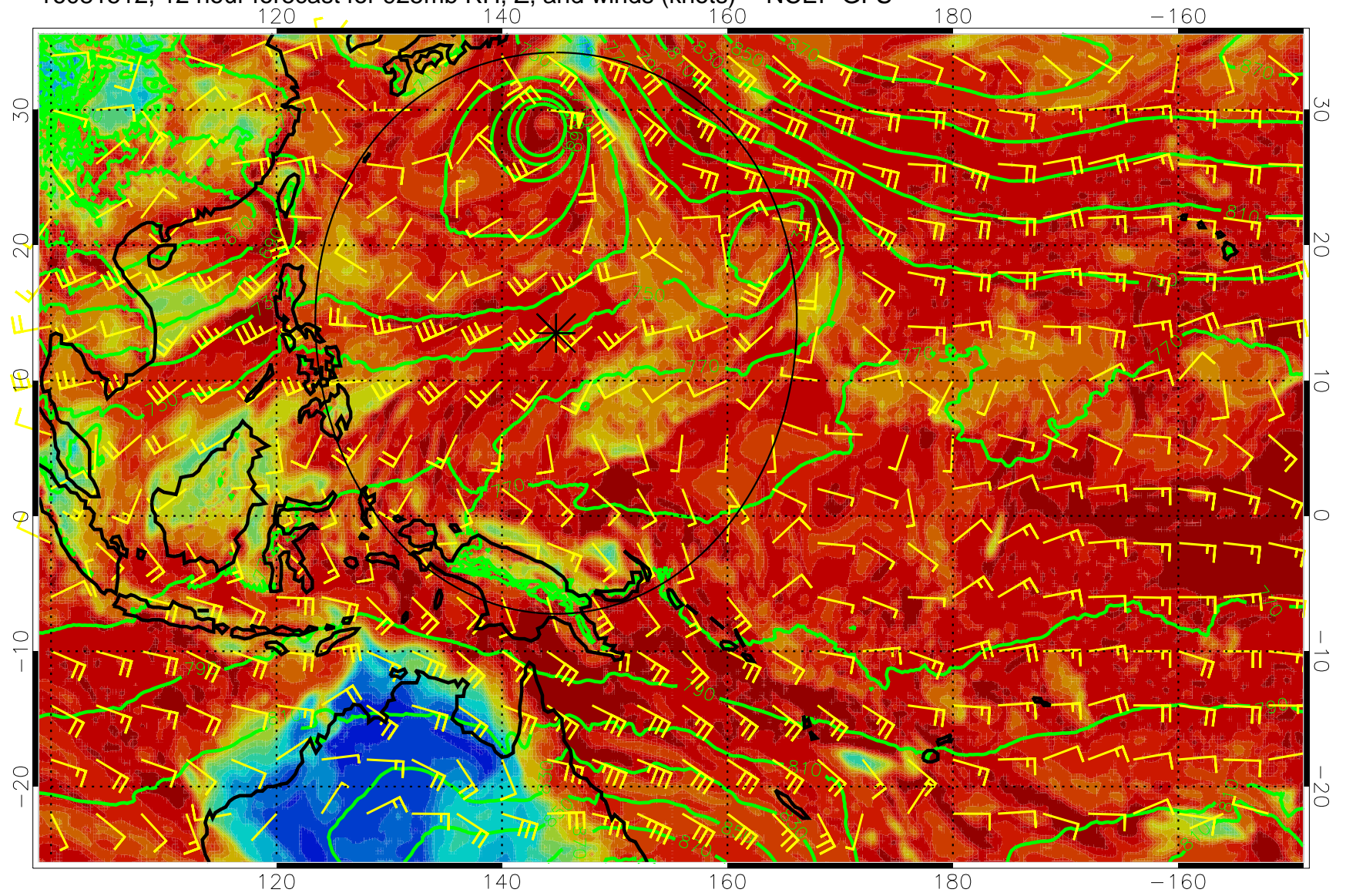
16081512, 12 hour forecast for 925mb RH, Z, and winds (knots) -- NCEP GFS
