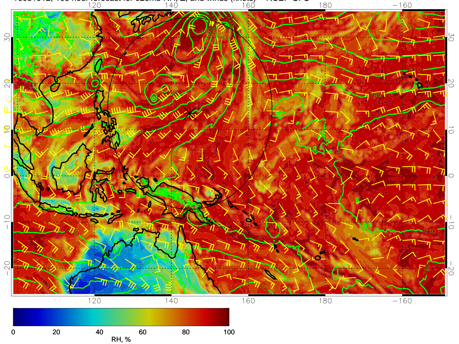
16081912, 108 hour forecast for 925mb RH, Z, and winds (knots) -- NCEP GFS
