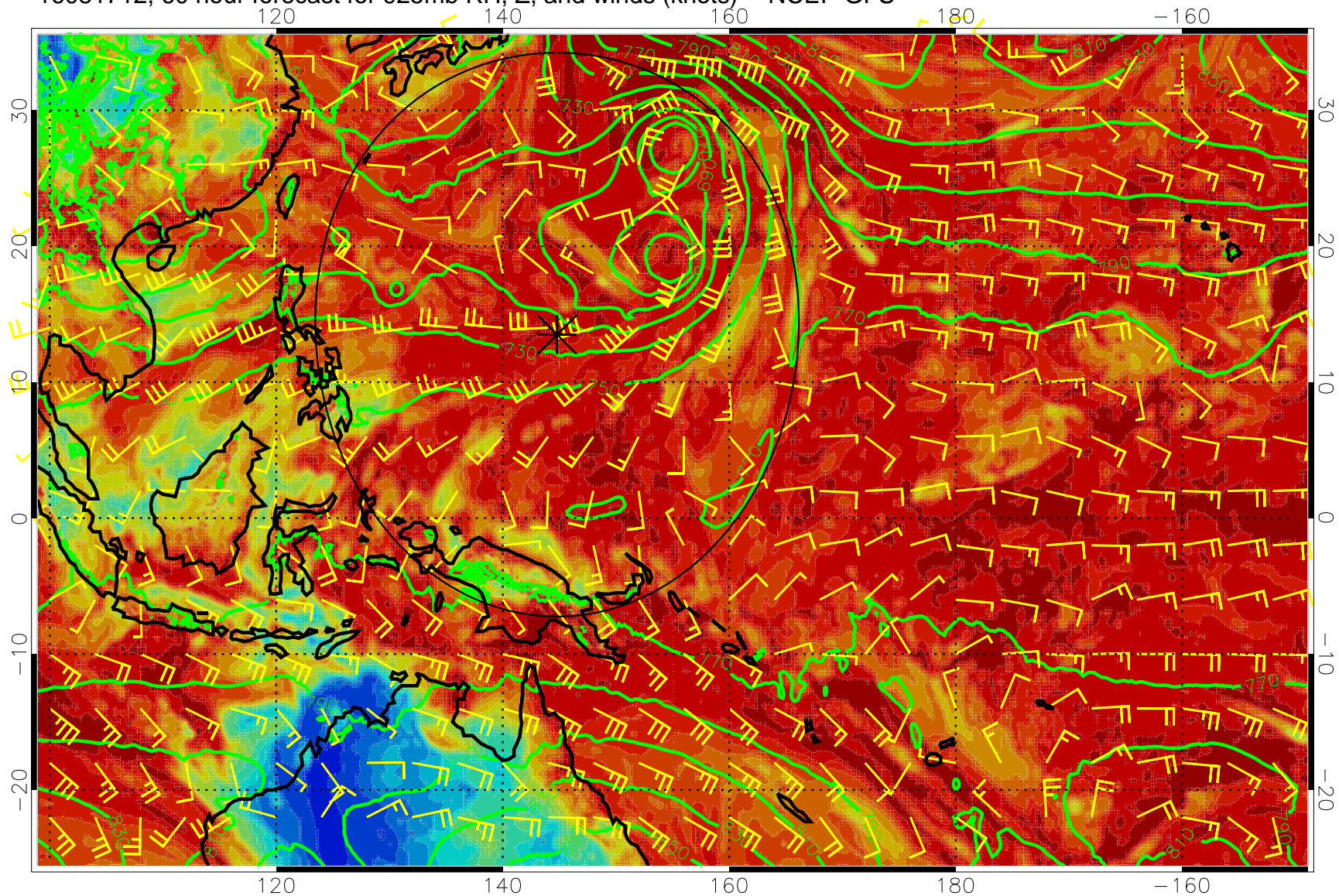
16081712, 60 hour forecast for 925mb RH, Z, and winds (knots) -- NCEP GFS
