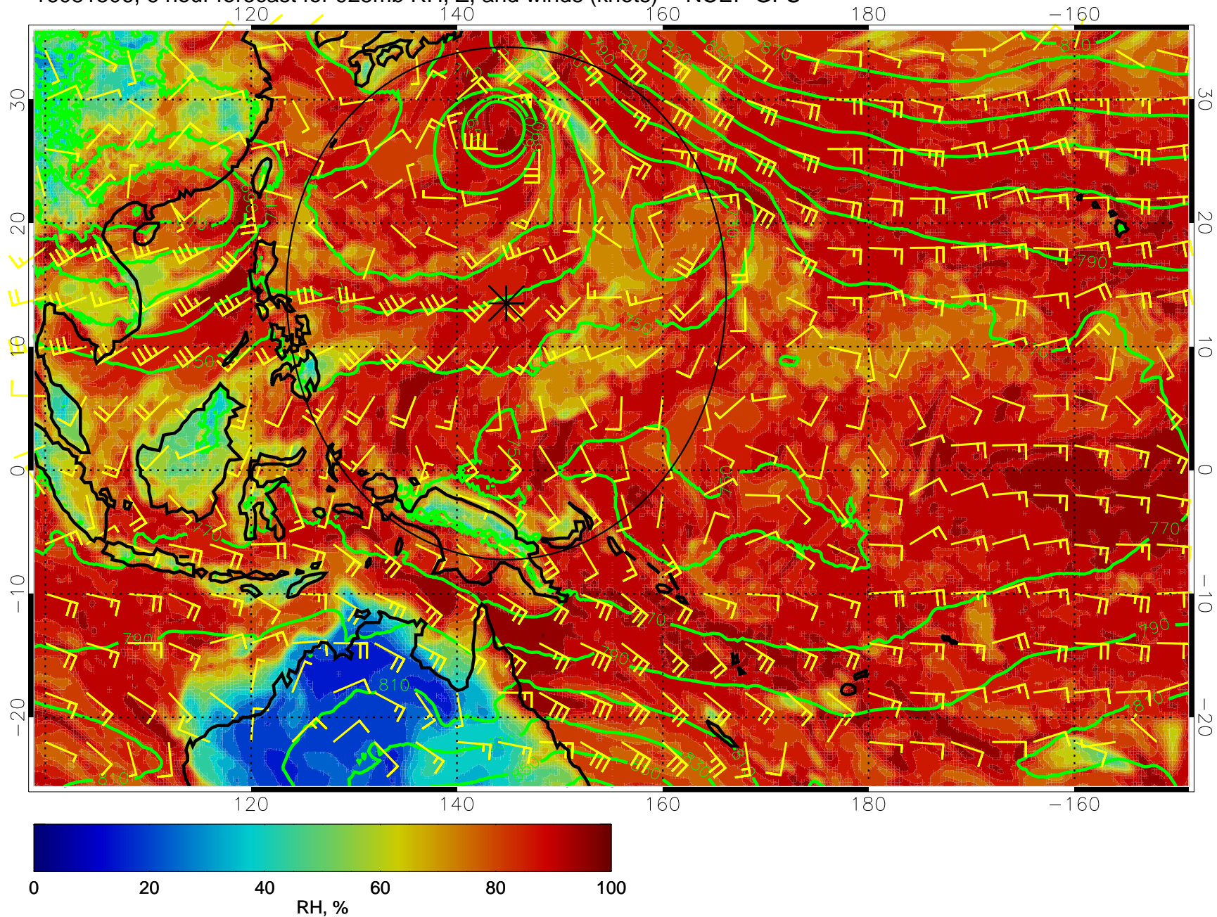
16081506, 6 hour forecast for 925mb RH, Z, and winds (knots) -- NCEP GFS
