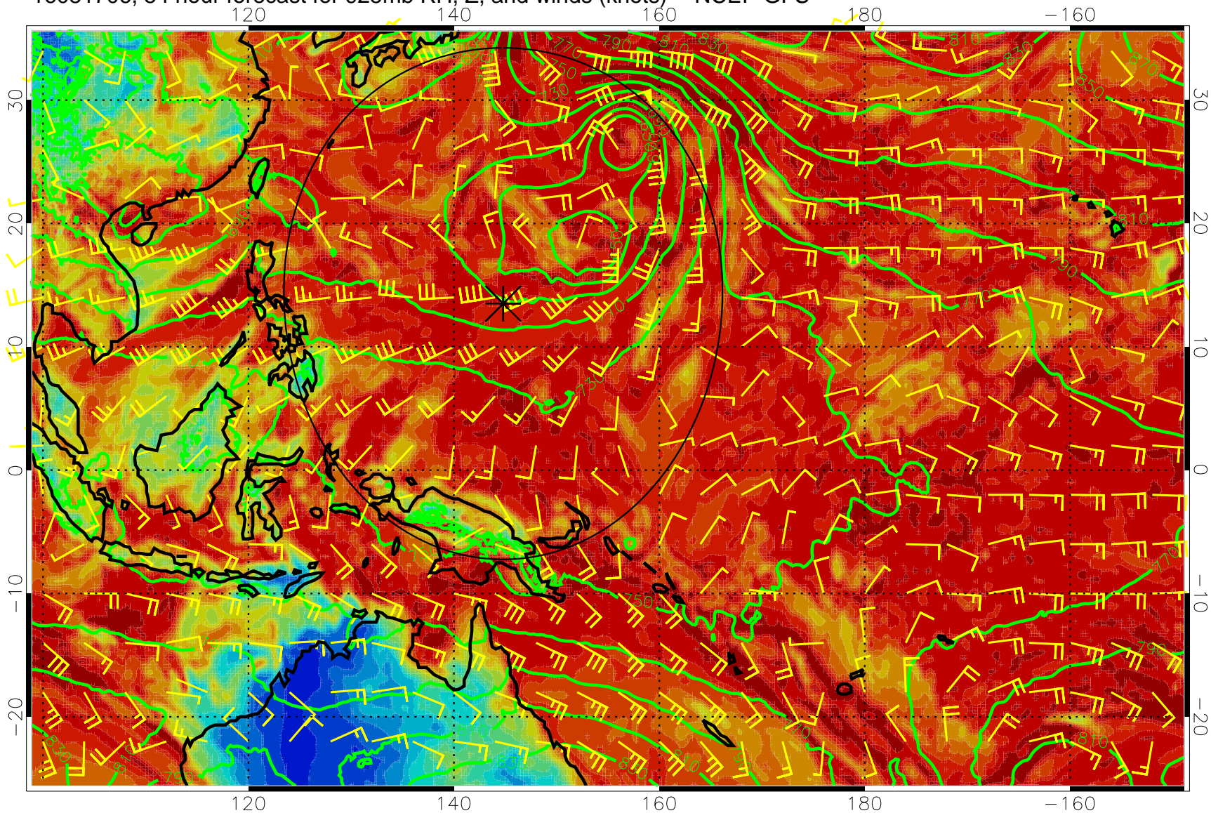
16081706, 54 hour forecast for 925mb RH, Z, and winds (knots) -- NCEP GFS
