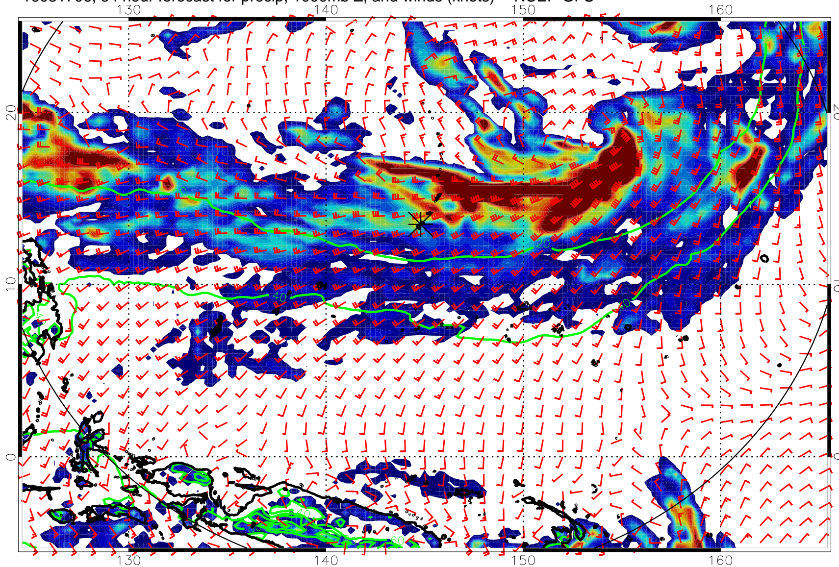
16081706, 54 hour forecast for precip, 1000mb Z, and winds (knots) -- NCEP GFS
