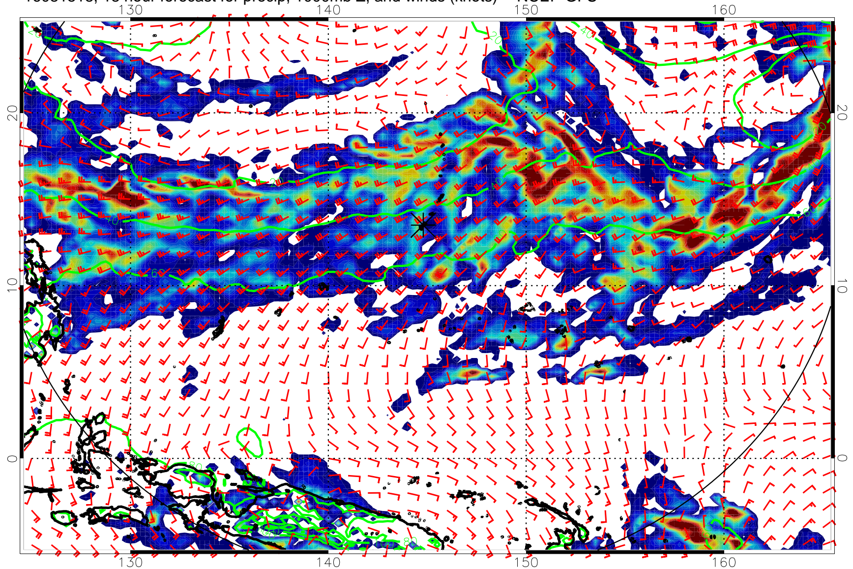
16081518, 18 hour forecast for precip, 1000mb Z, and winds (knots) -- NCEP GFS
