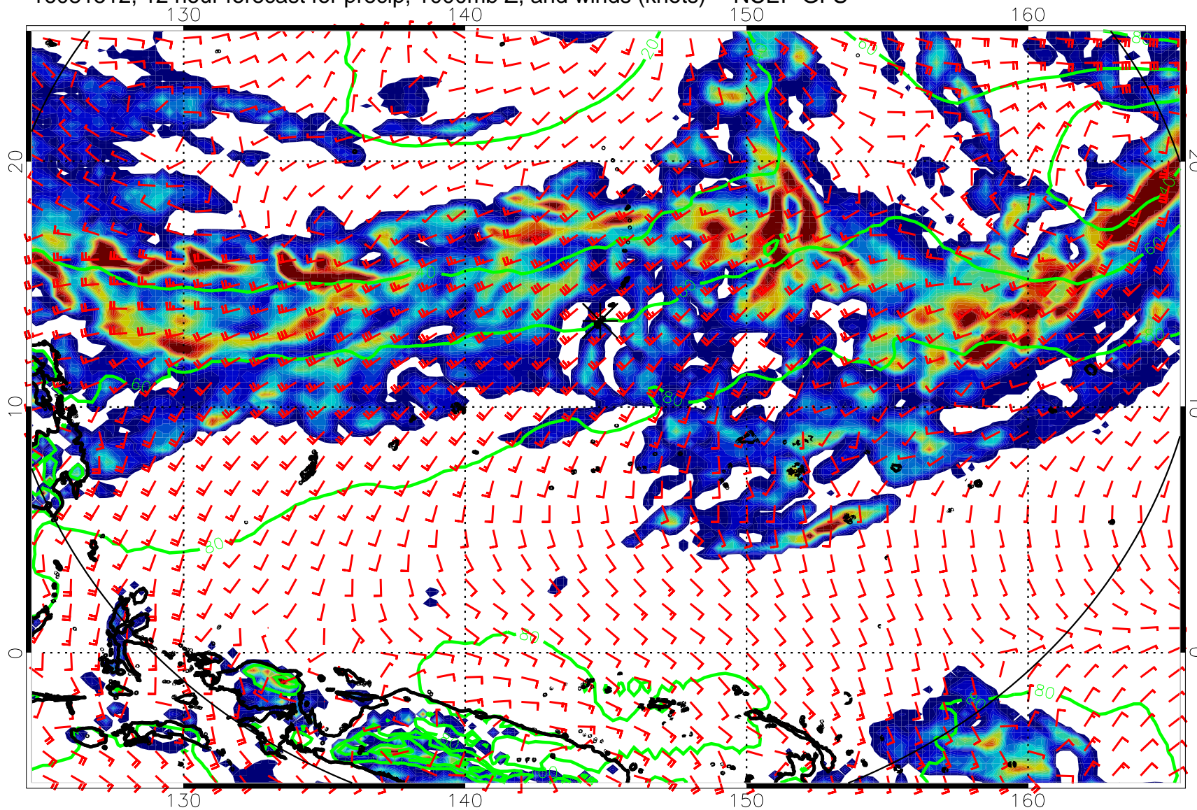
16081512, 12 hour forecast for precip, 1000mb Z, and winds (knots) -- NCEP GFS
