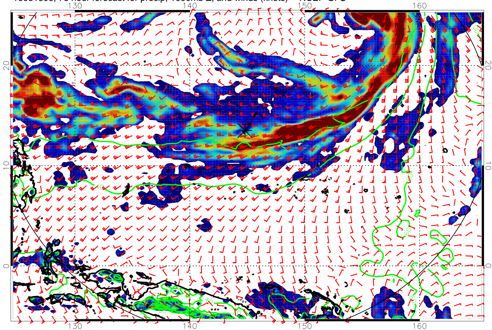
16081806, 78 hour forecast for precip, 1000mb Z, and winds (knots) -- NCEP GFS
