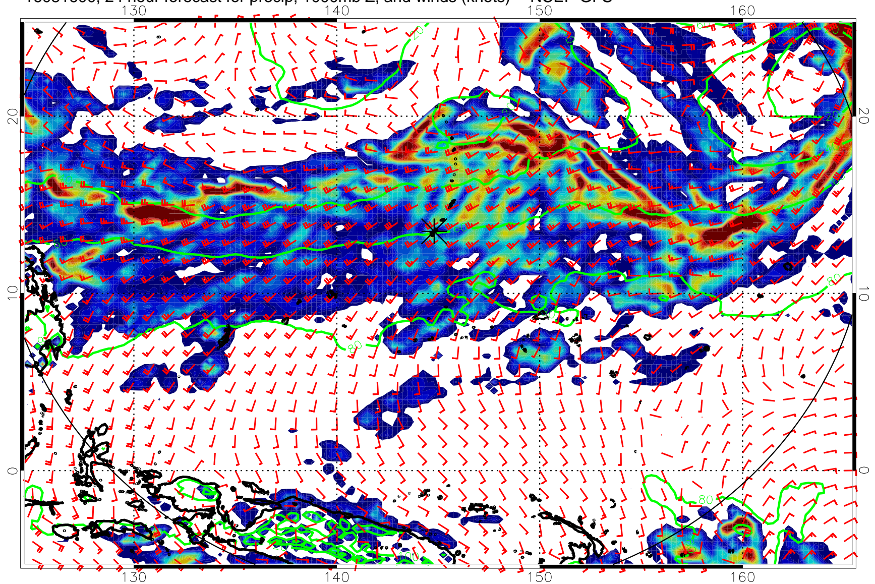
16081600, 24 hour forecast for precip, 1000mb Z, and winds (knots) -- NCEP GFS
