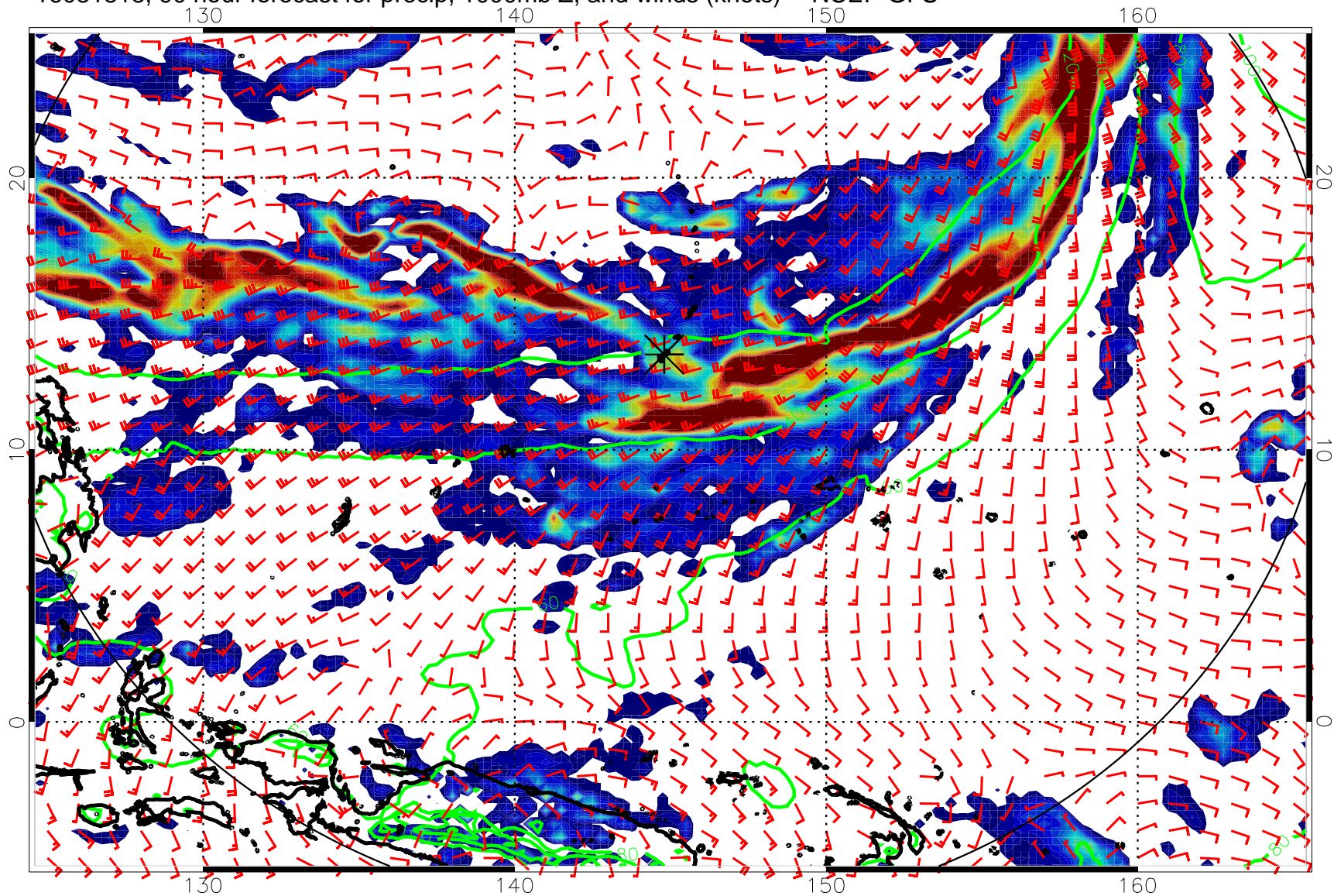
16081818, 90 hour forecast for precip, 1000mb Z, and winds (knots) -- NCEP GFS
