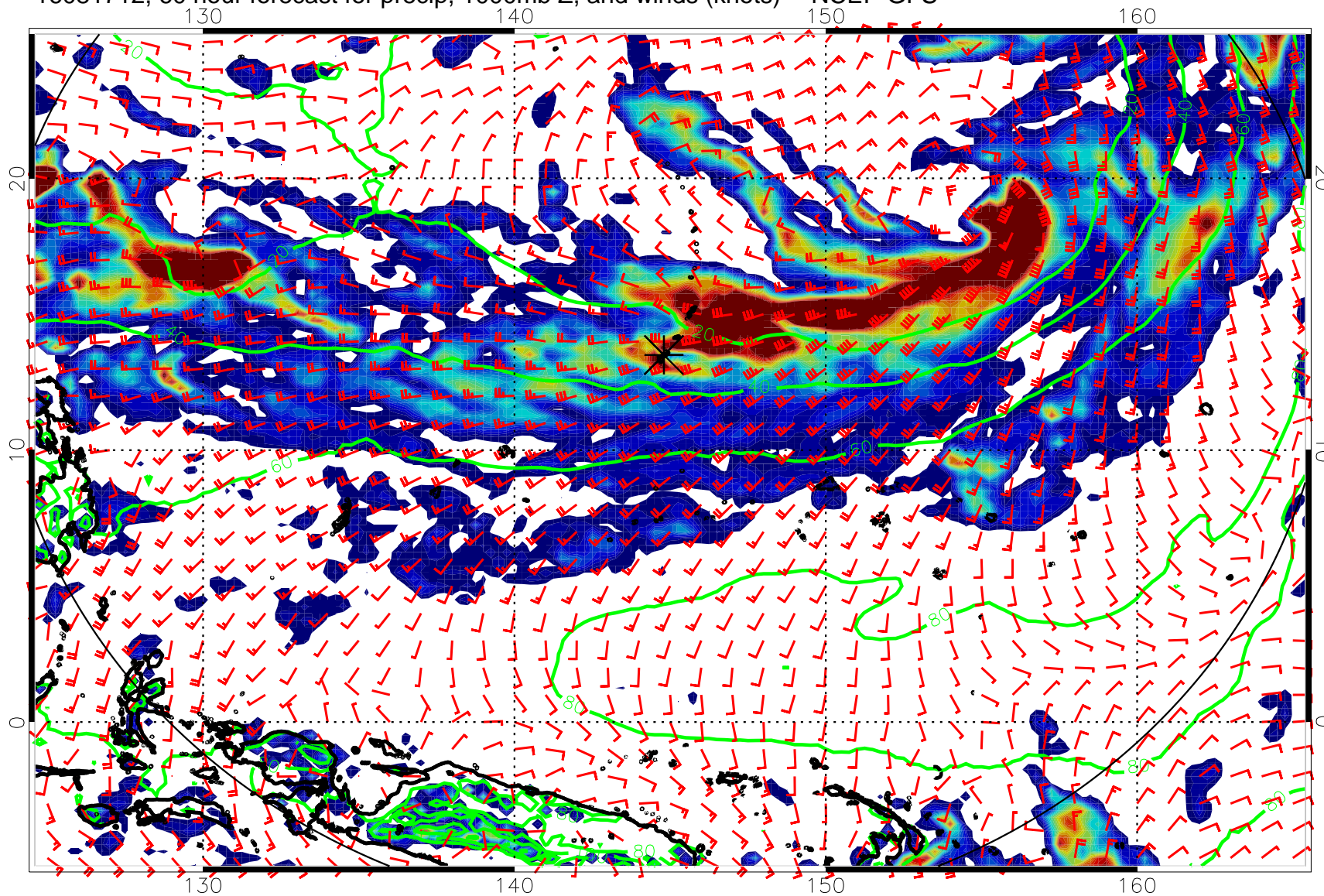
16081712, 60 hour forecast for precip, 1000mb Z, and winds (knots) -- NCEP GFS
