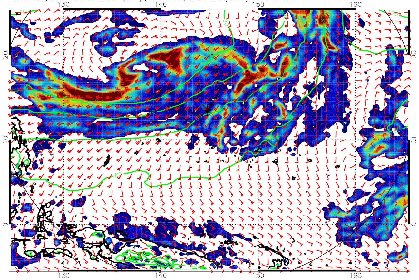
16082000, 120 hour forecast for precip, 1000mb Z, and winds (knots) -- NCEP GFS
