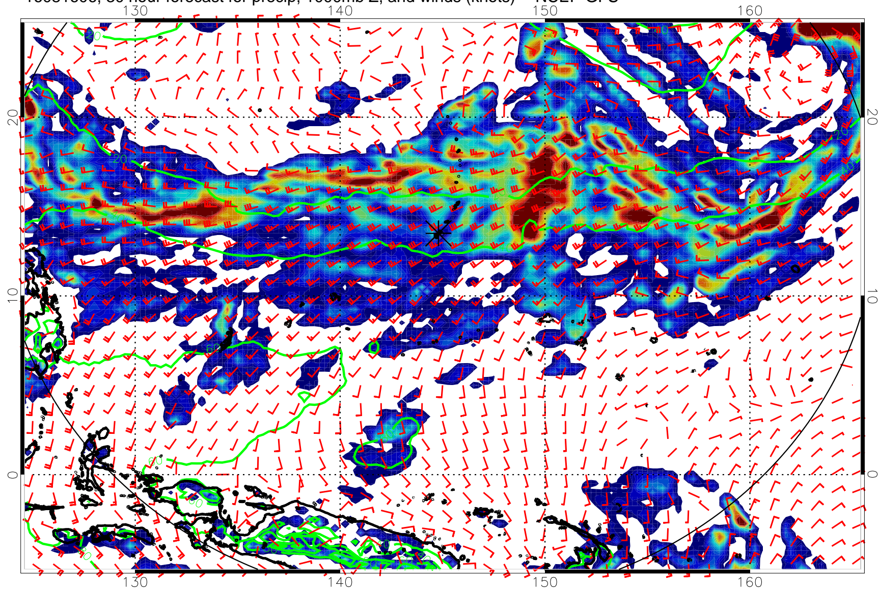
16081606, 30 hour forecast for precip, 1000mb Z, and winds (knots) -- NCEP GFS
