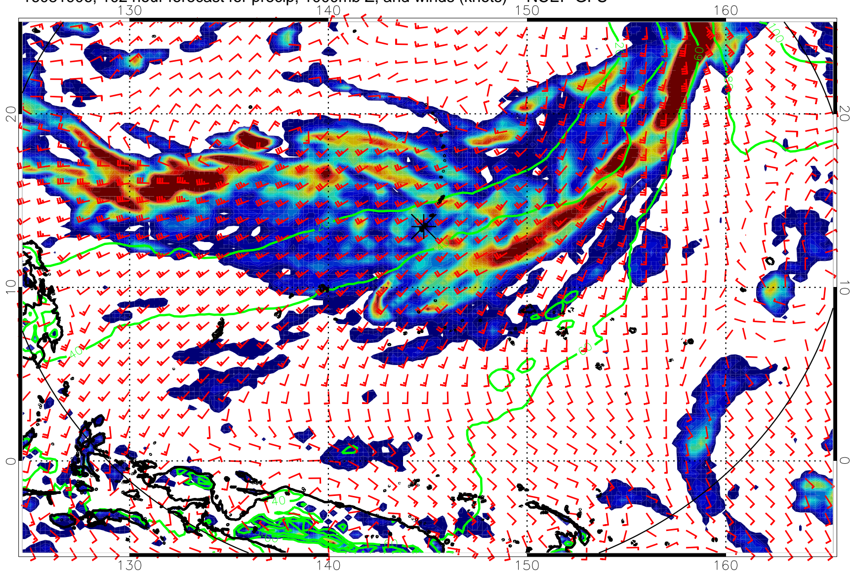
16081906, 102 hour forecast for precip, 1000mb Z, and winds (knots) -- NCEP GFS
