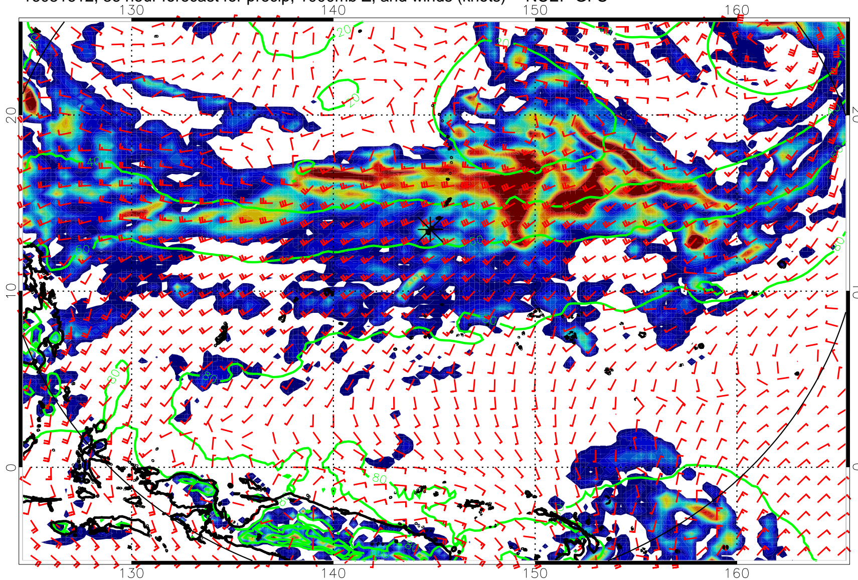
16081612, 36 hour forecast for precip, 1000mb Z, and winds (knots) -- NCEP GFS
