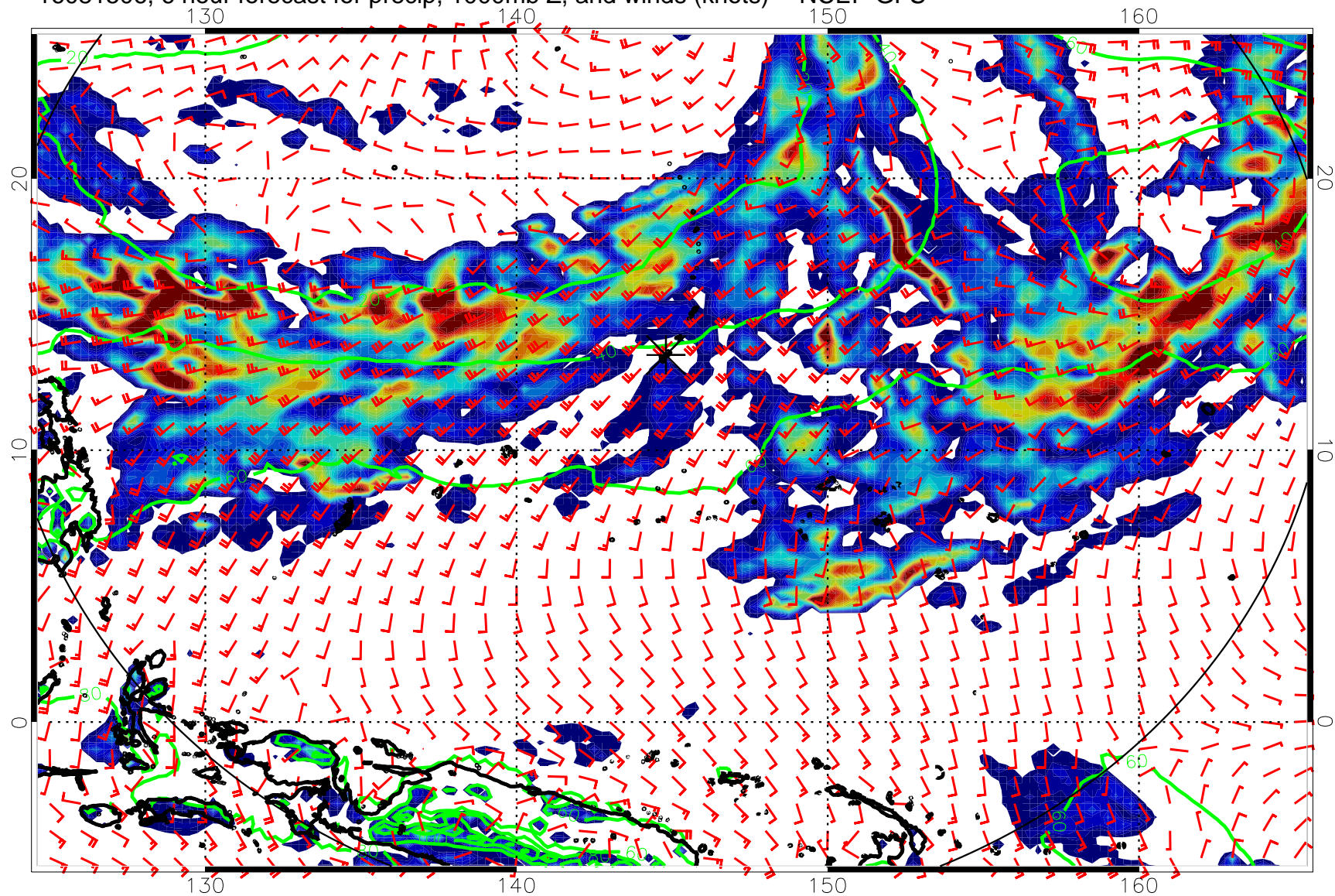
16081506, 6 hour forecast for precip, 1000mb Z, and winds (knots) -- NCEP GFS
