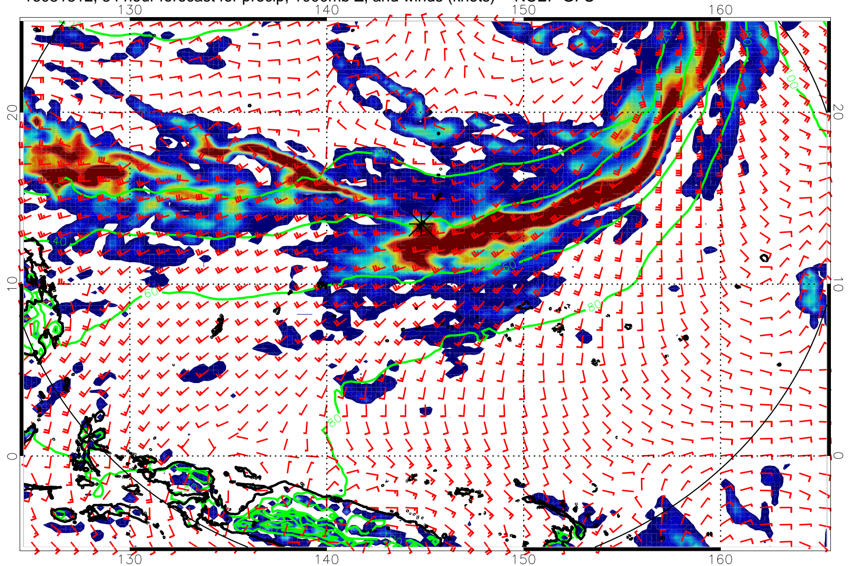
16081812, 84 hour forecast for precip, 1000mb Z, and winds (knots) -- NCEP GFS
