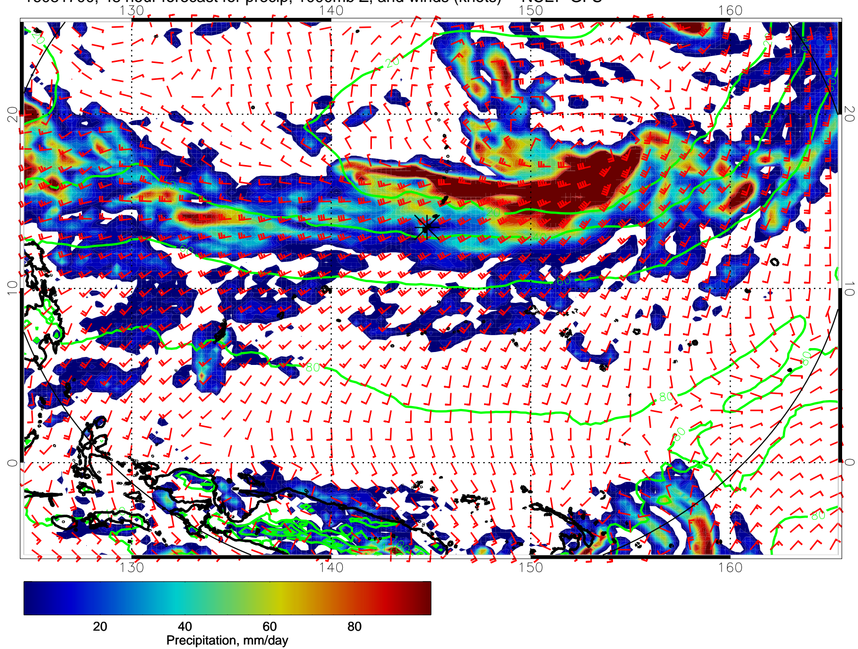
16081700, 48 hour forecast for precip, 1000mb Z, and winds (knots) -- NCEP GFS
