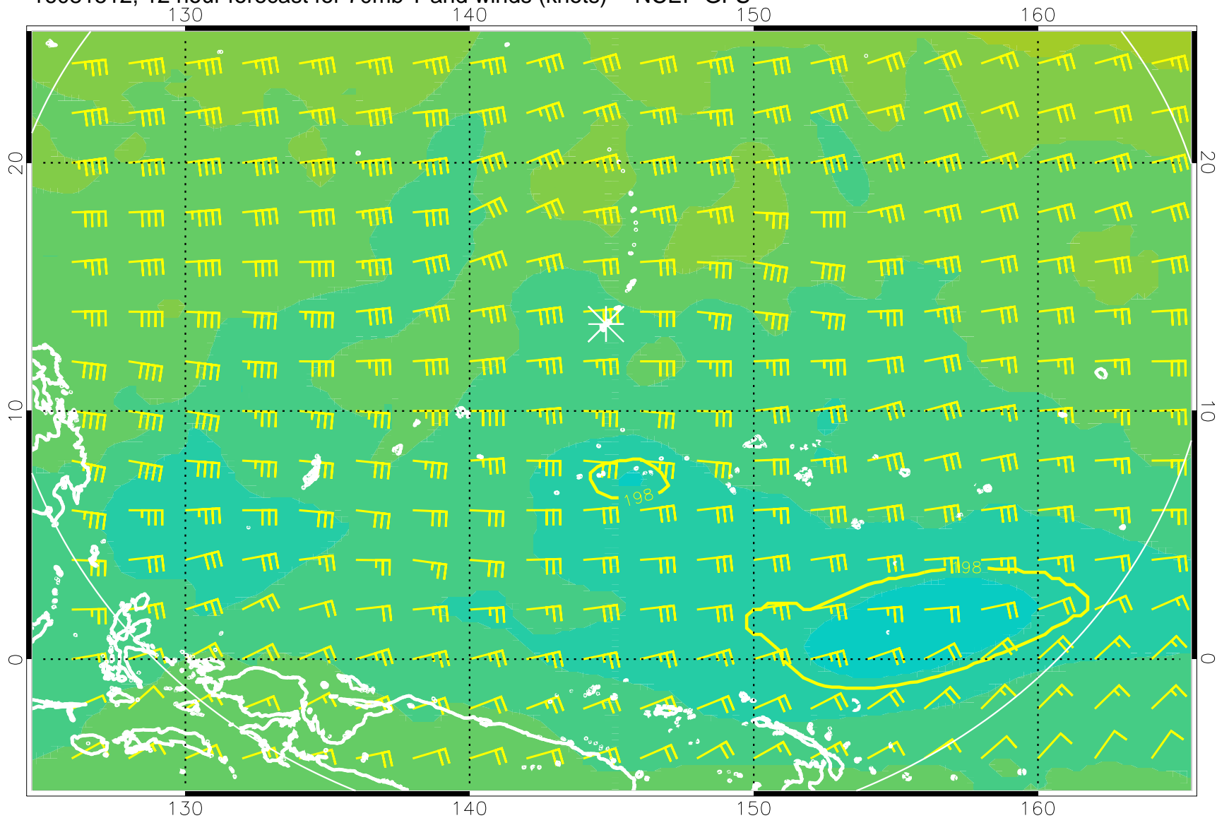
16081512, 12 hour forecast for 70mb T and winds (knots) -- NCEP GFS
