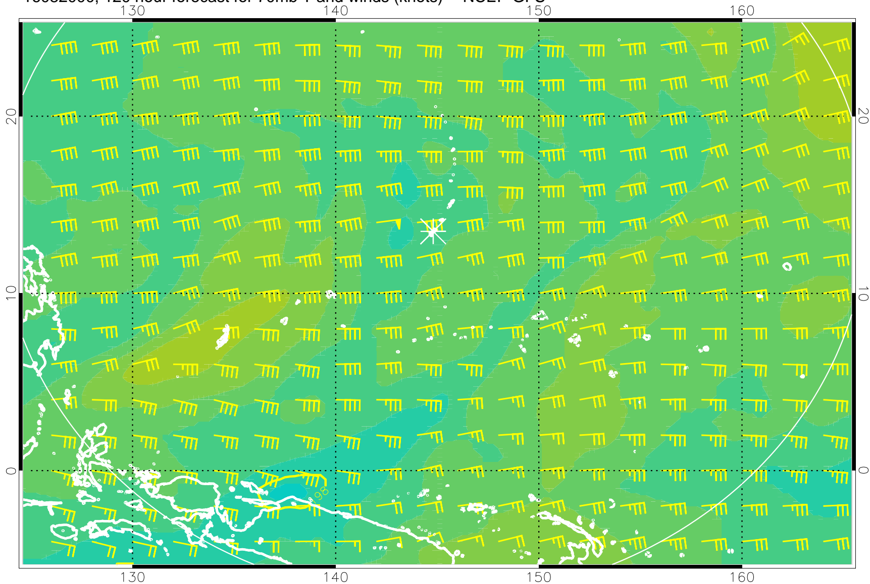
16082000, 120 hour forecast for 70mb T and winds (knots) -- NCEP GFS
