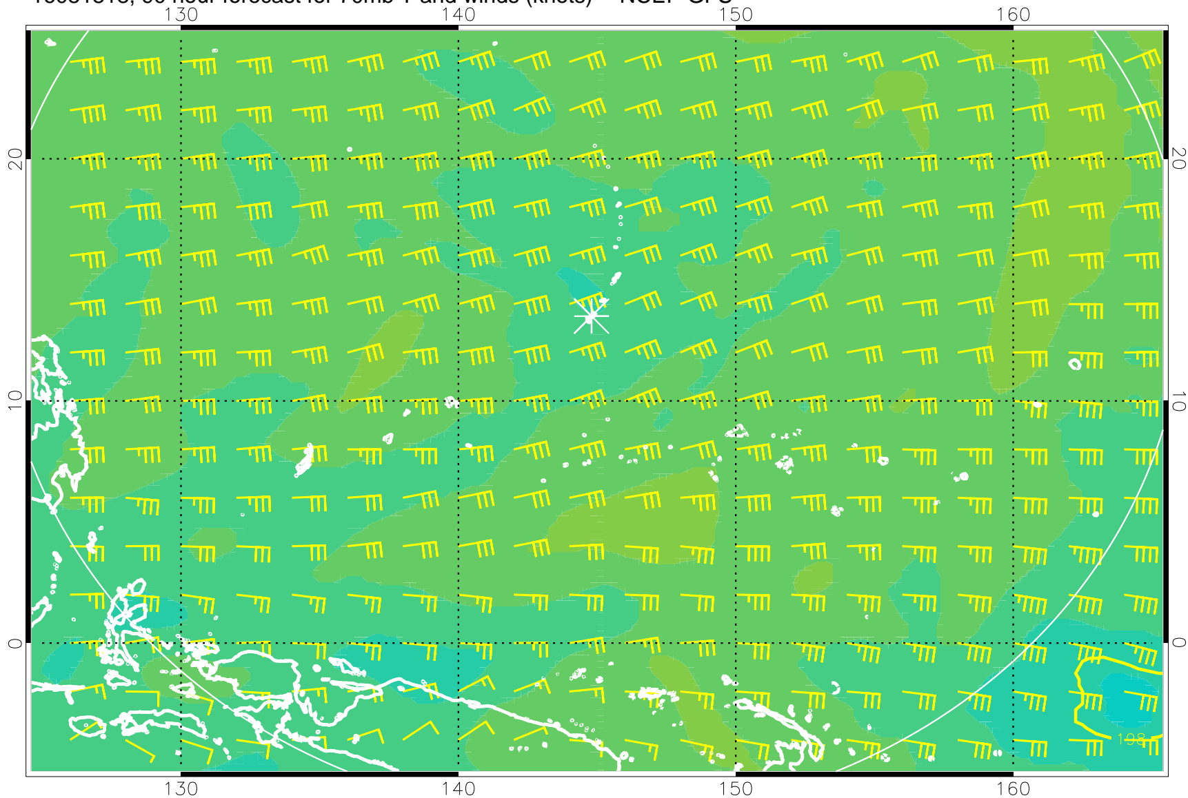
16081818, 90 hour forecast for 70mb T and winds (knots) -- NCEP GFS
