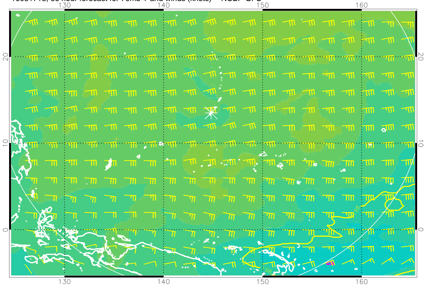
16081718, 66 hour forecast for 70mb T and winds (knots) -- NCEP GFS
