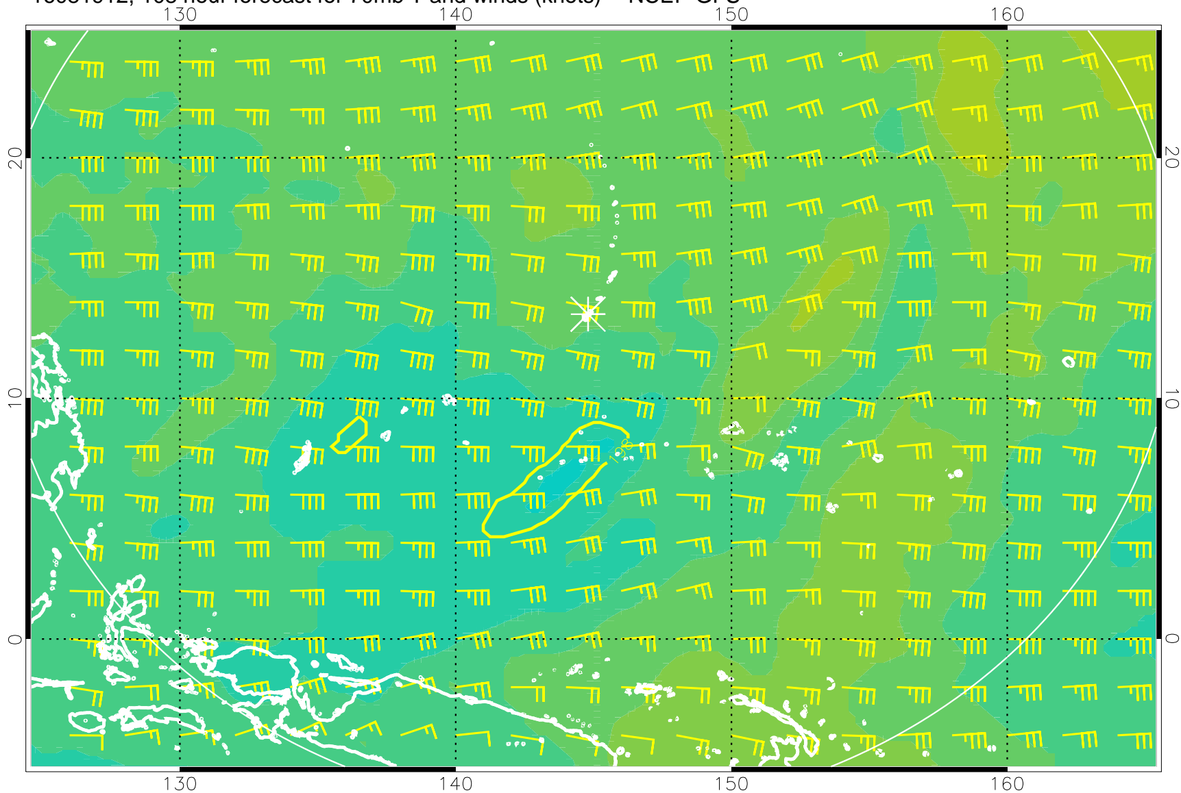
16081912, 108 hour forecast for 70mb T and winds (knots) -- NCEP GFS
