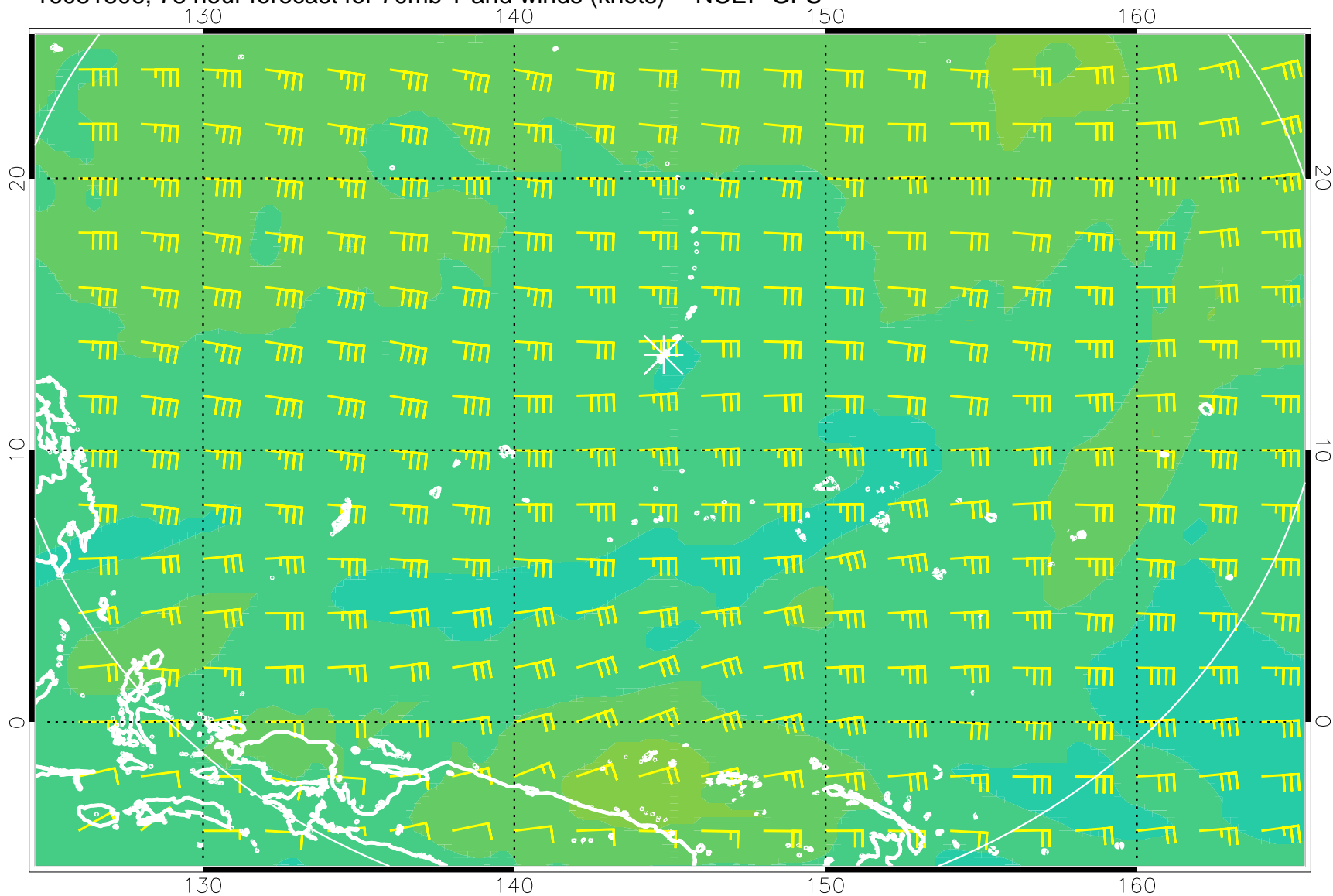
16081806, 78 hour forecast for 70mb T and winds (knots) -- NCEP GFS
