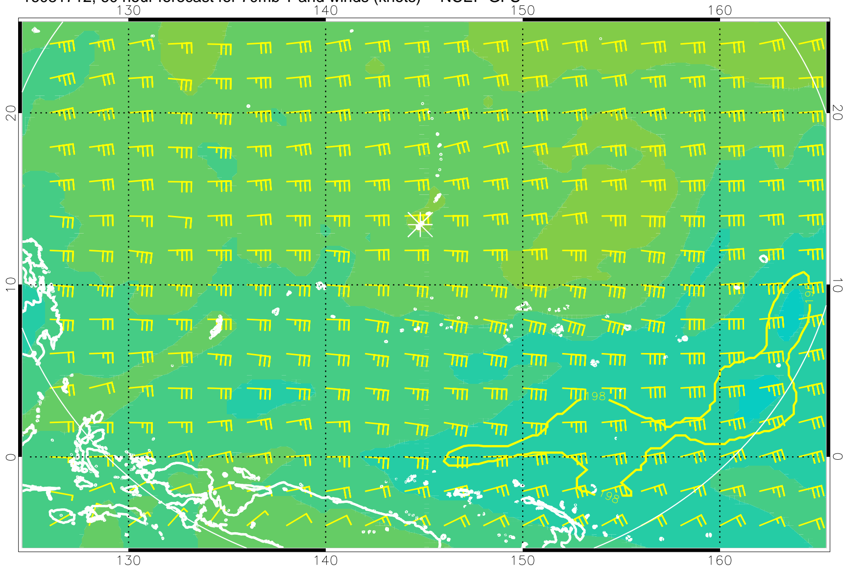
16081712, 60 hour forecast for 70mb T and winds (knots) -- NCEP GFS
