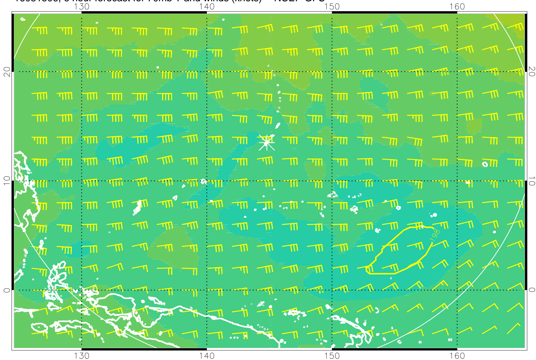
16081506, 6 hour forecast for 70mb T and winds (knots) -- NCEP GFS
