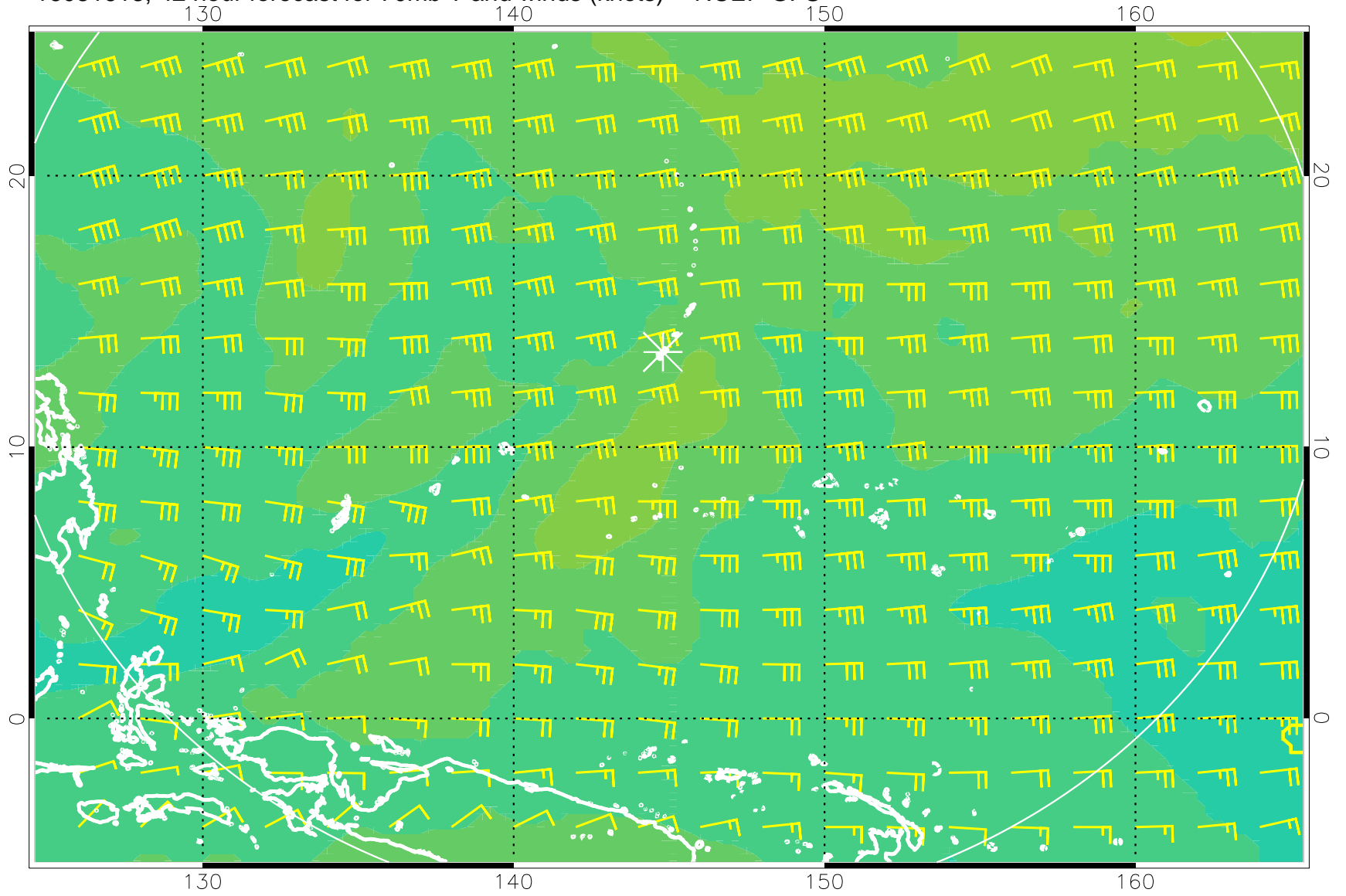
16081618, 42 hour forecast for 70mb T and winds (knots) -- NCEP GFS
