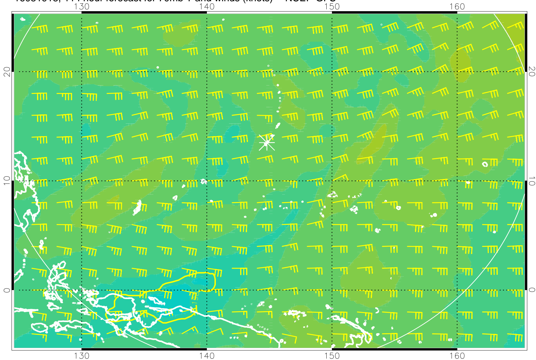
16081918, 114 hour forecast for 70mb T and winds (knots) -- NCEP GFS
