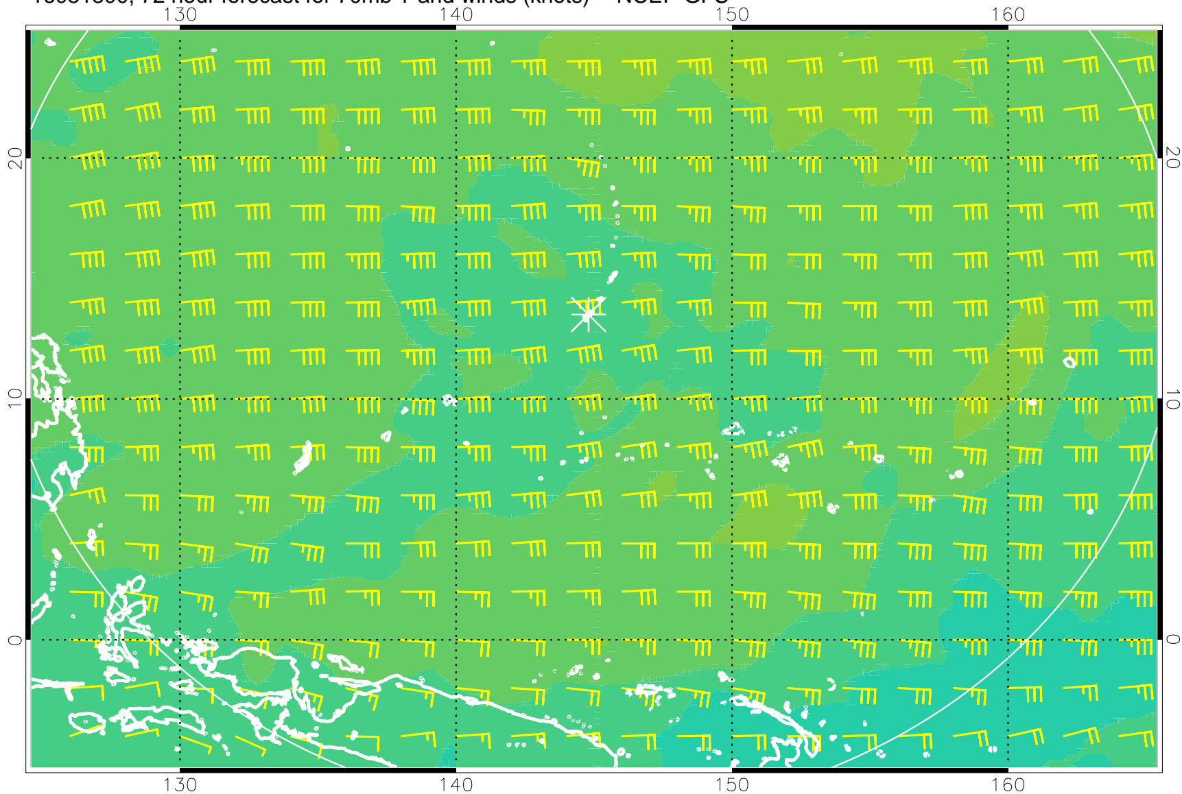
16081800, 72 hour forecast for 70mb T and winds (knots) -- NCEP GFS
