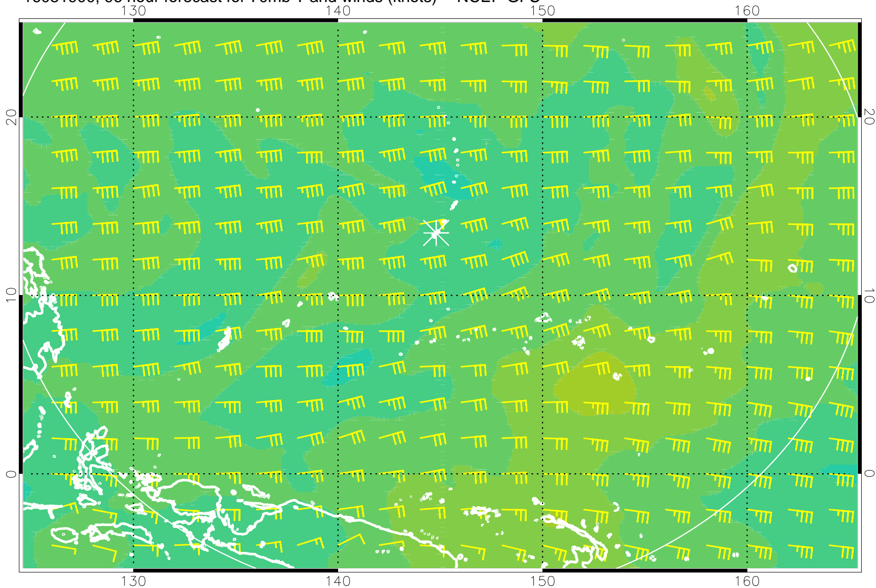
16081900, 96 hour forecast for 70mb T and winds (knots) -- NCEP GFS
