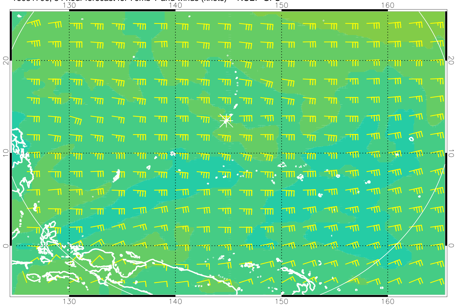
16081706, 54 hour forecast for 70mb T and winds (knots) -- NCEP GFS
