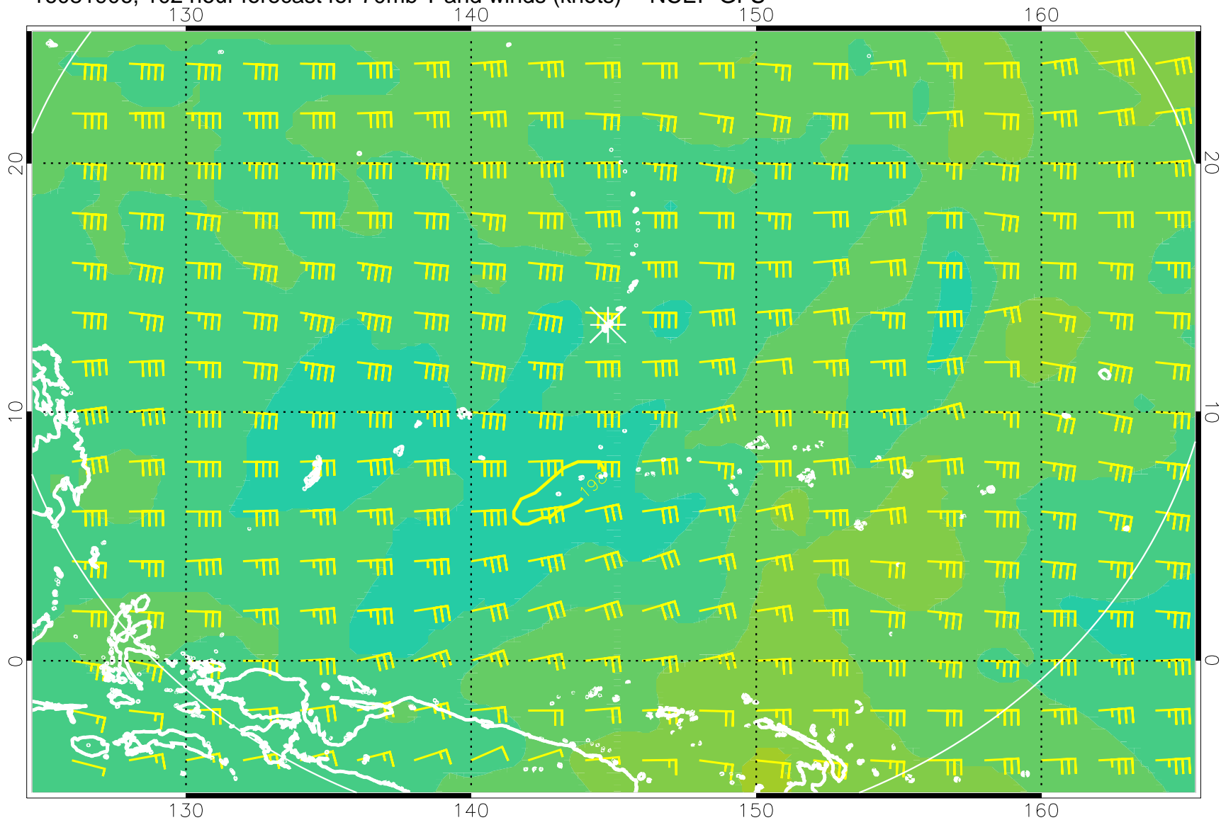
16081906, 102 hour forecast for 70mb T and winds (knots) -- NCEP GFS
