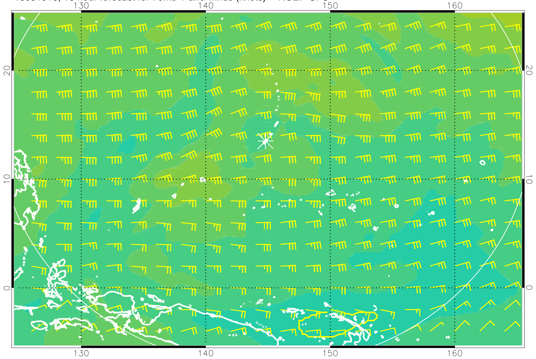
16081518, 18 hour forecast for 70mb T and winds (knots) -- NCEP GFS
