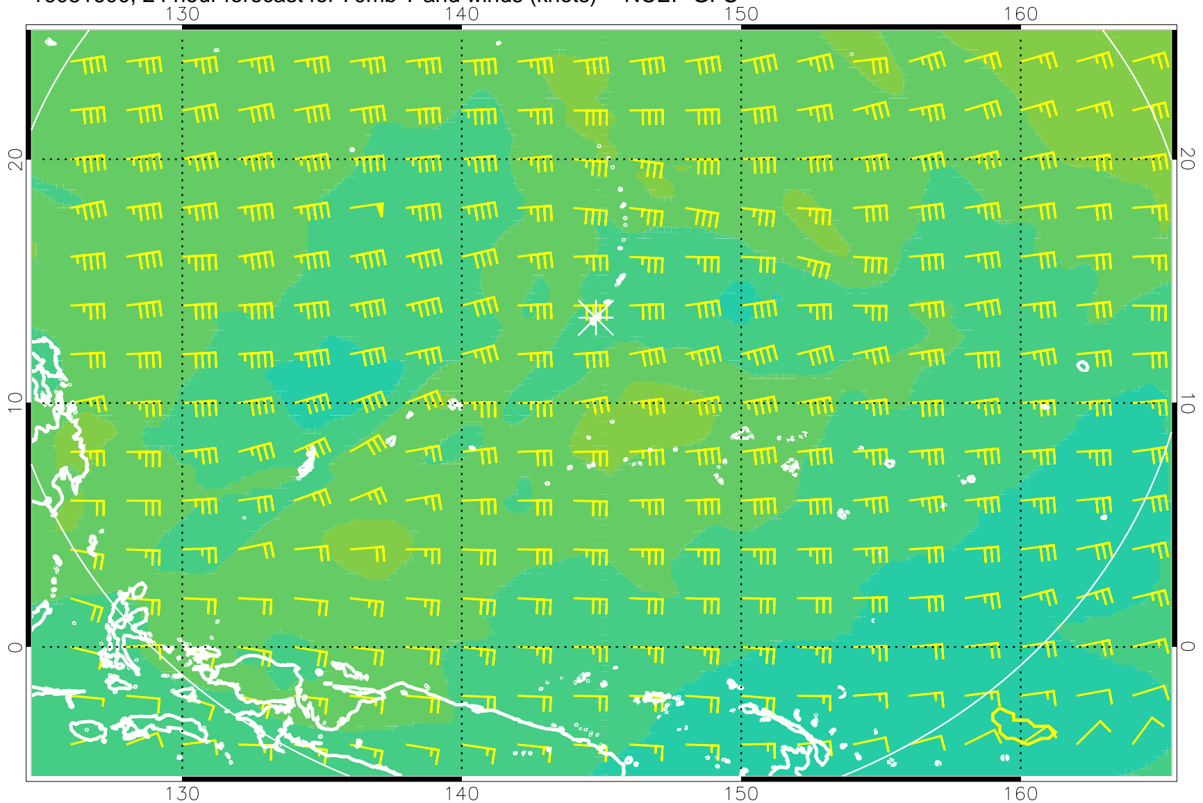
16081600, 24 hour forecast for 70mb T and winds (knots) -- NCEP GFS
