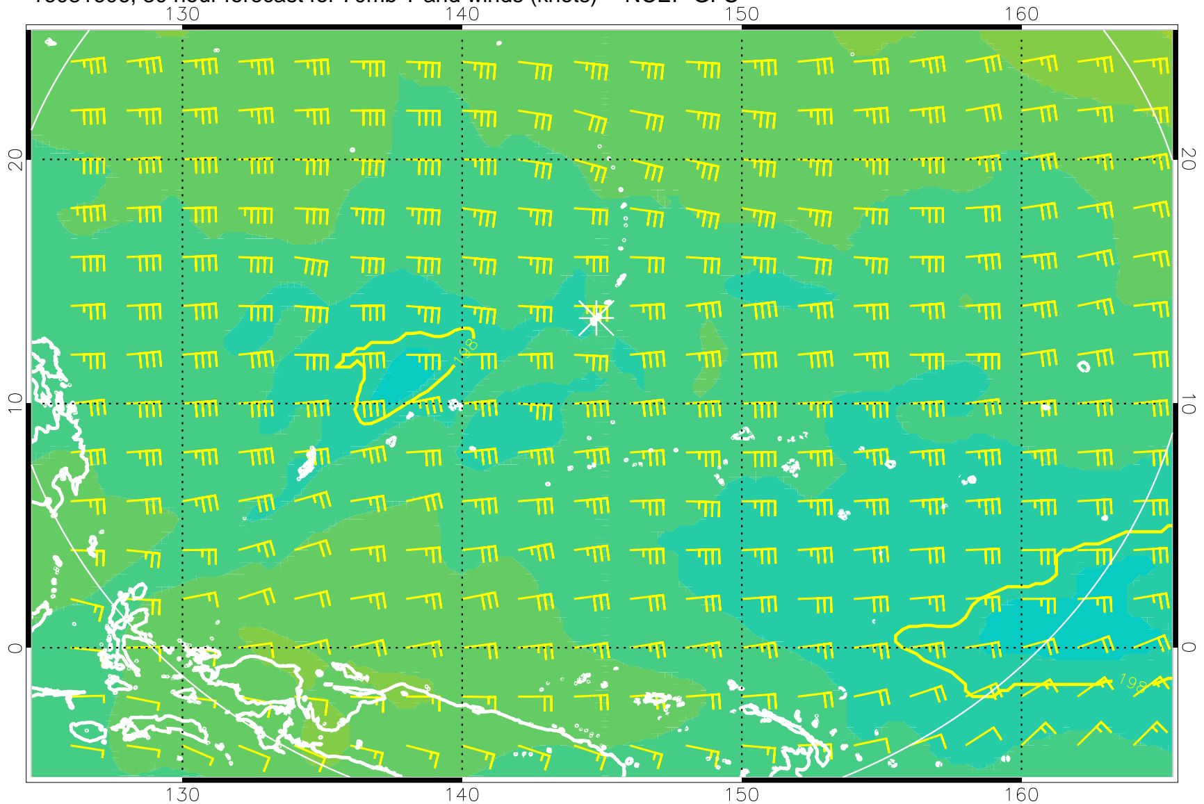
16081606, 30 hour forecast for 70mb T and winds (knots) -- NCEP GFS
