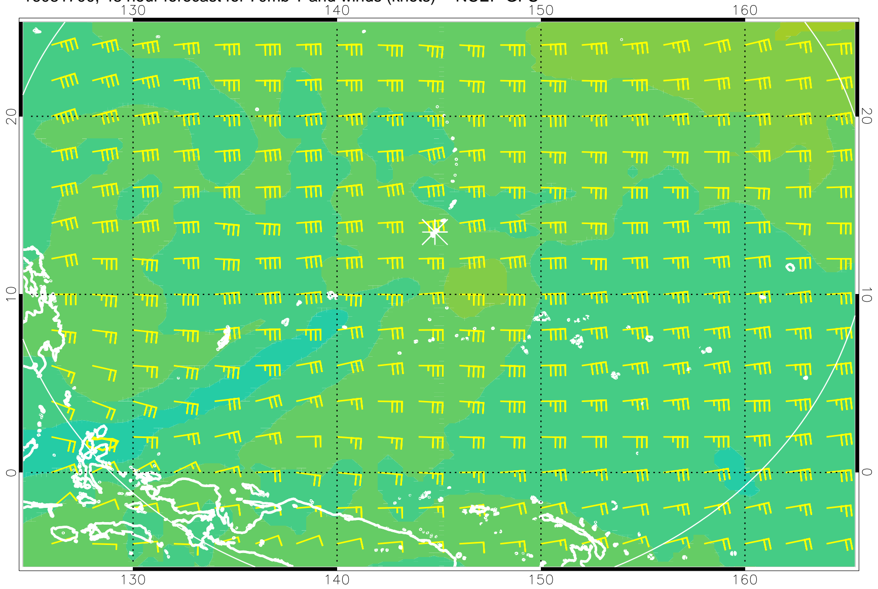
16081700, 48 hour forecast for 70mb T and winds (knots) -- NCEP GFS
