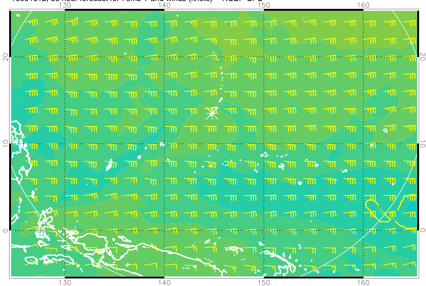
16081612, 36 hour forecast for 70mb T and winds (knots) -- NCEP GFS
