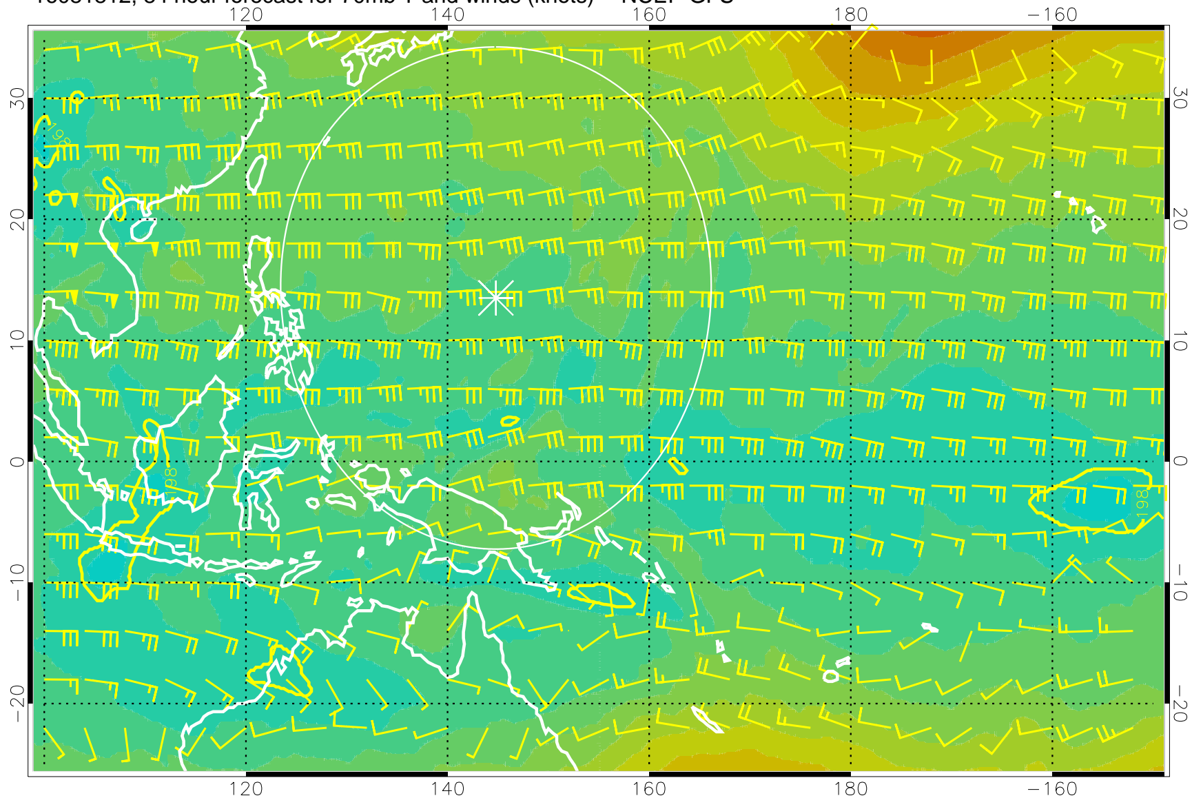
16081812, 84 hour forecast for 70mb T and winds (knots) -- NCEP GFS
