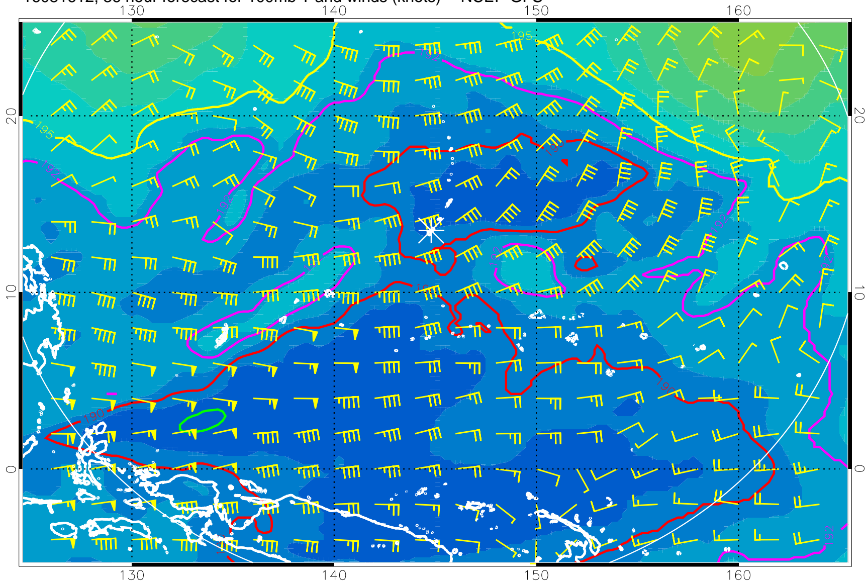
16081612, 36 hour forecast for 100mb T and winds (knots) -- NCEP GFS
