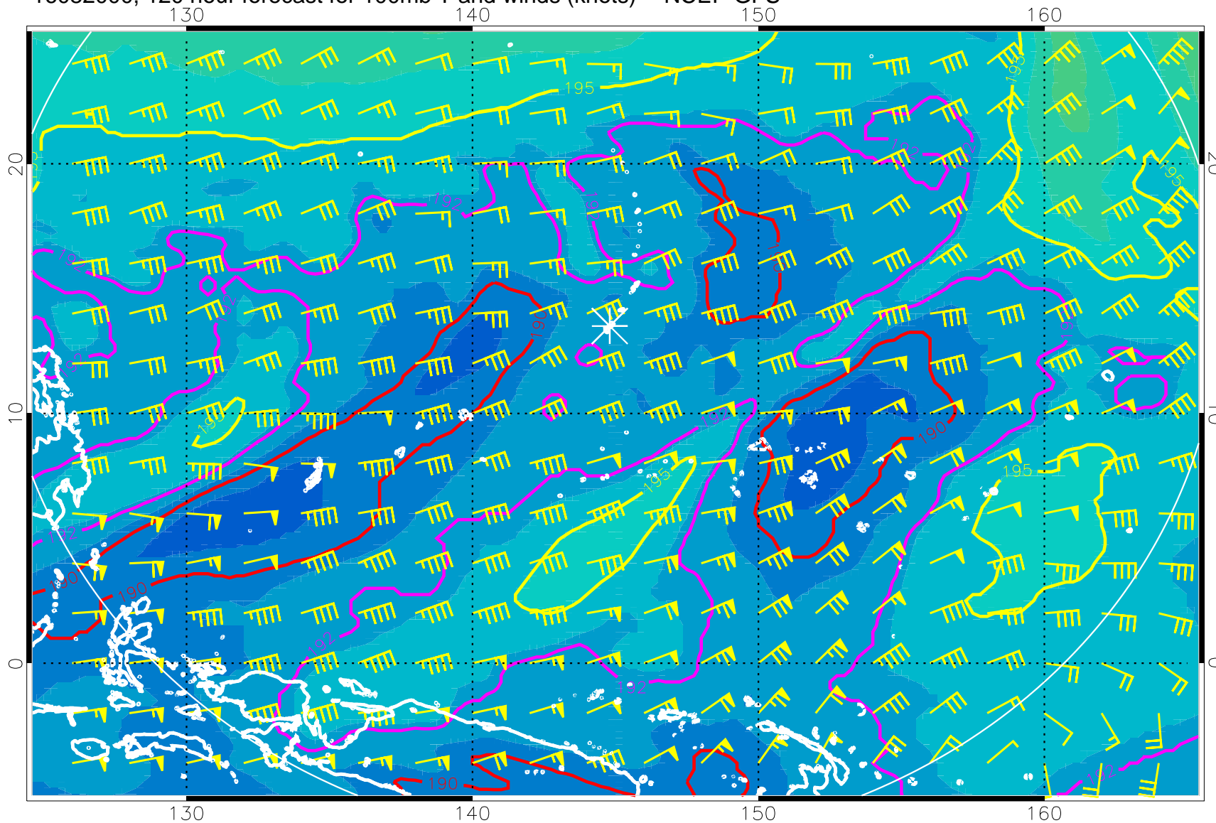
16082000, 120 hour forecast for 100mb T and winds (knots) -- NCEP GFS
