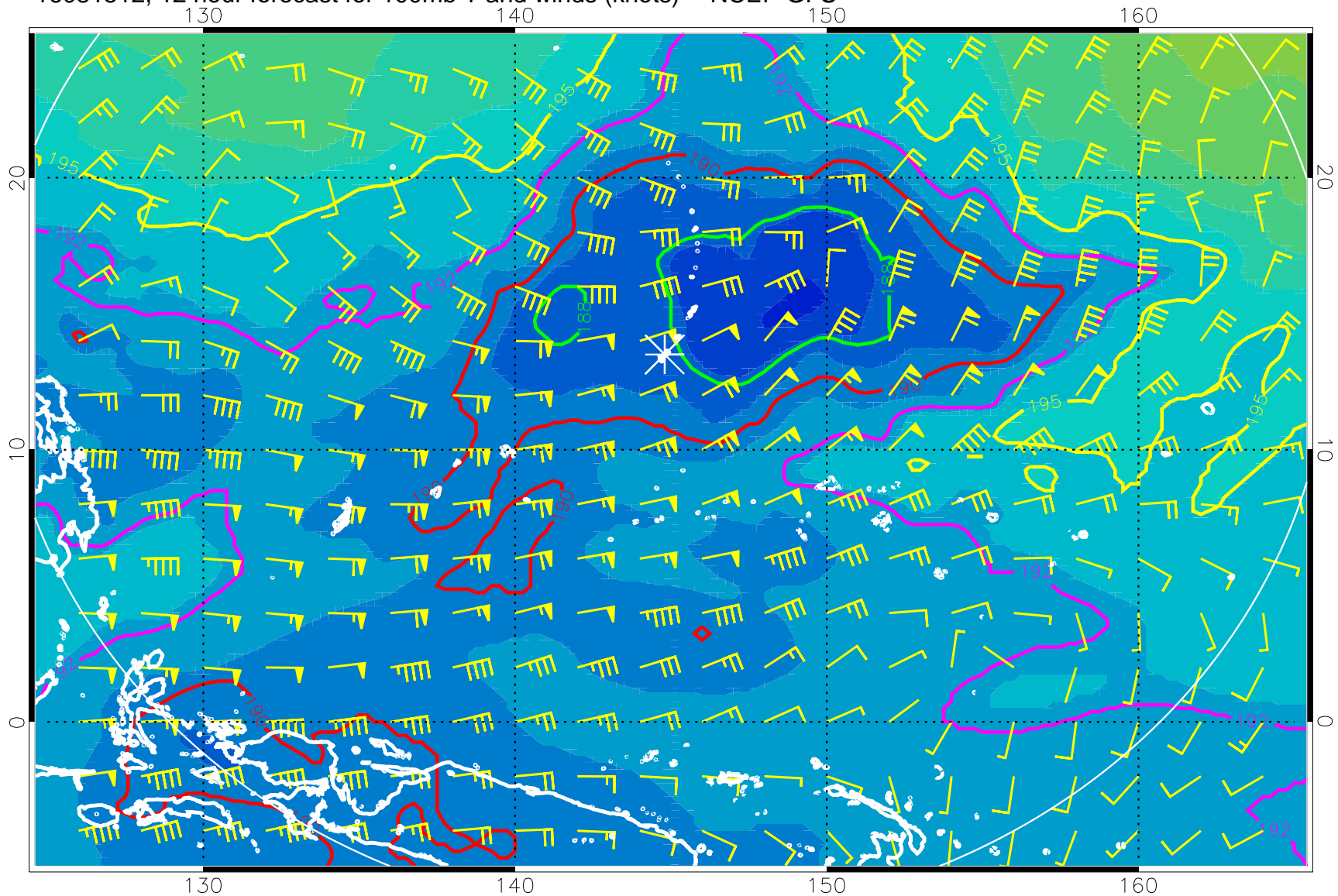
16081512, 12 hour forecast for 100mb T and winds (knots) -- NCEP GFS
