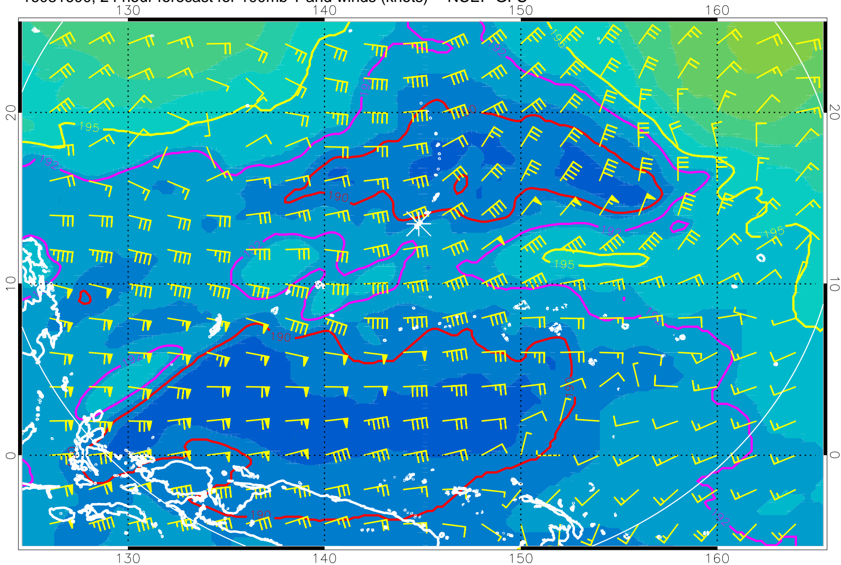
16081600, 24 hour forecast for 100mb T and winds (knots) -- NCEP GFS
