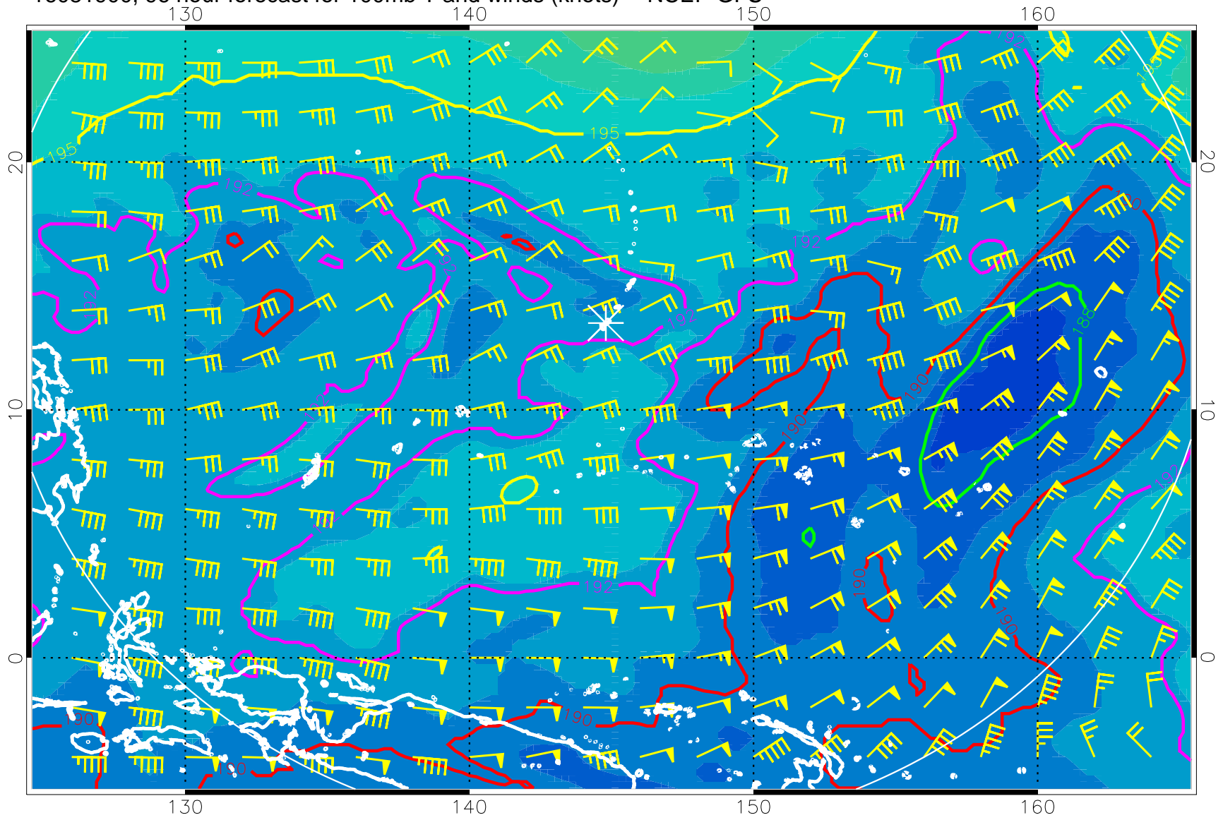
16081900, 96 hour forecast for 100mb T and winds (knots) -- NCEP GFS
