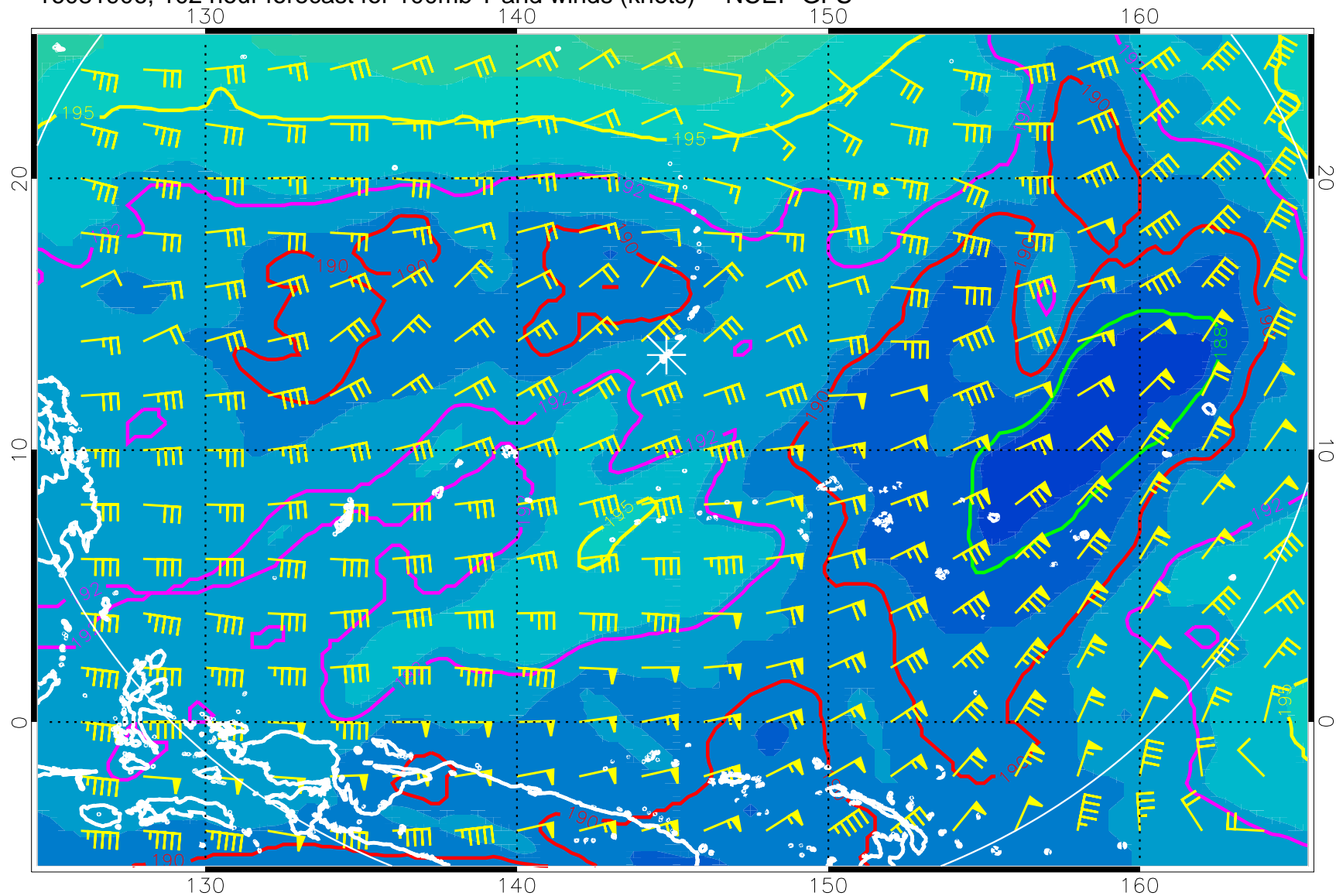
16081906, 102 hour forecast for 100mb T and winds (knots) -- NCEP GFS
