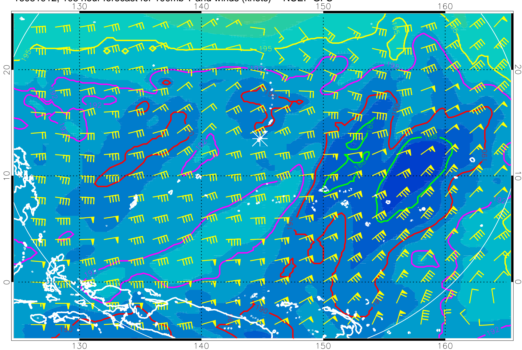
16081912, 108 hour forecast for 100mb T and winds (knots) -- NCEP GFS
