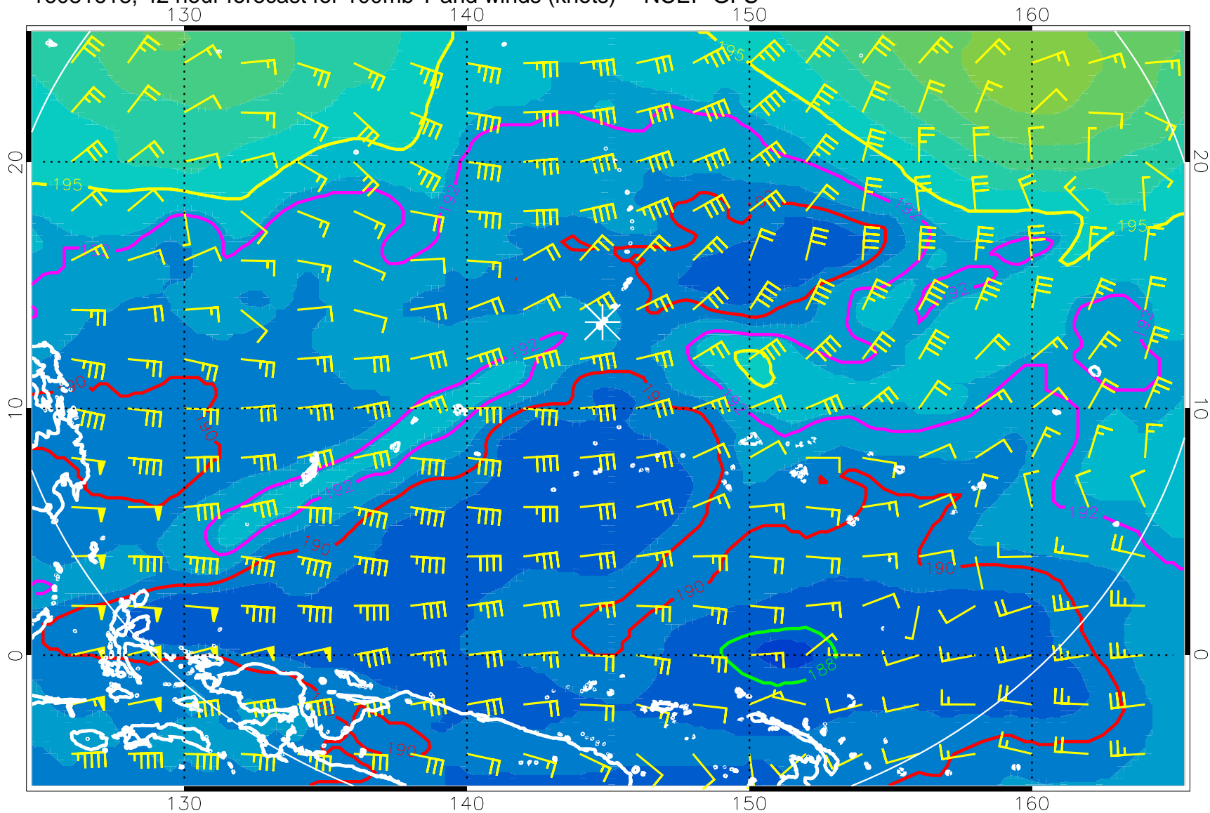
16081618, 42 hour forecast for 100mb T and winds (knots) -- NCEP GFS
