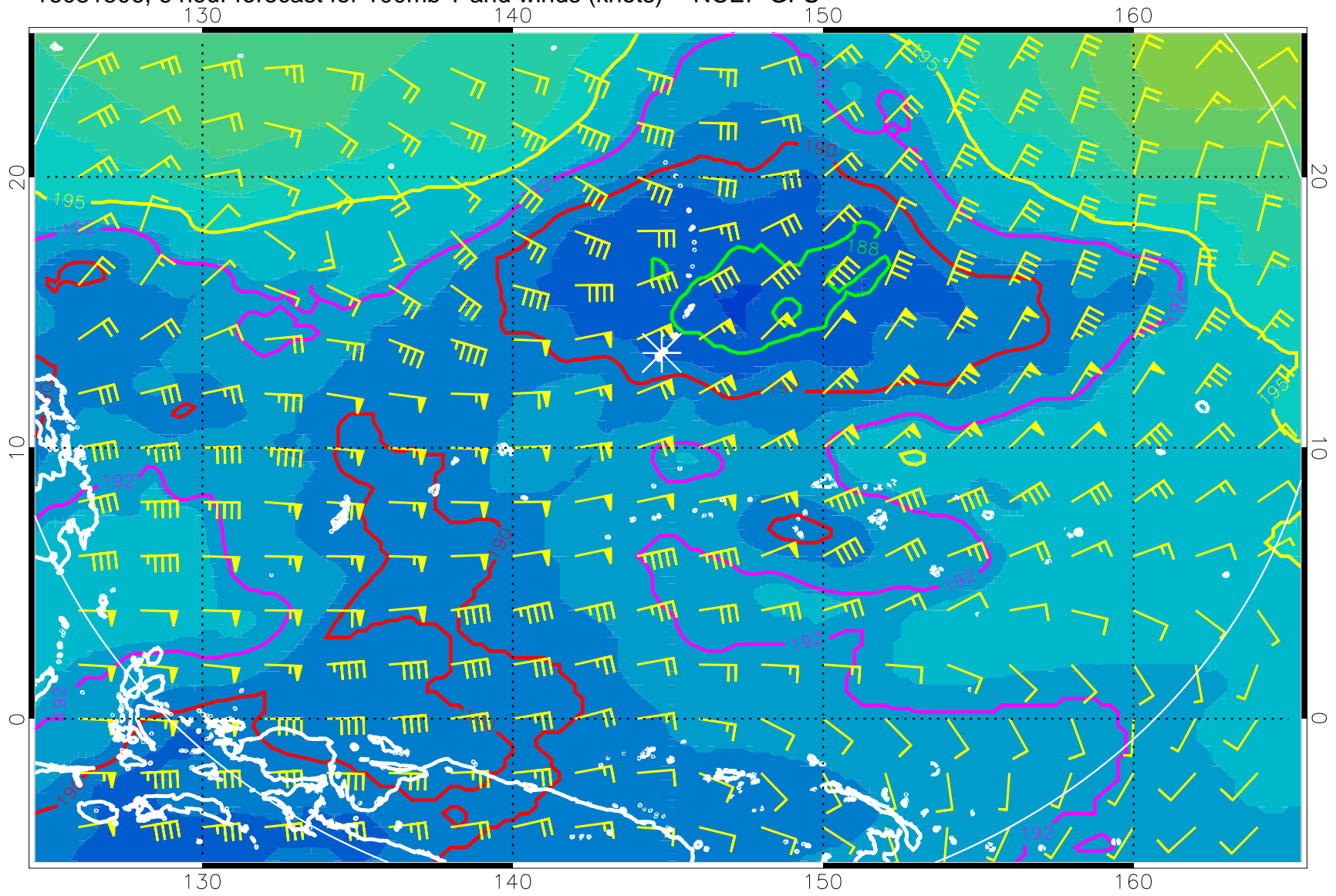
16081506, 6 hour forecast for 100mb T and winds (knots) -- NCEP GFS
