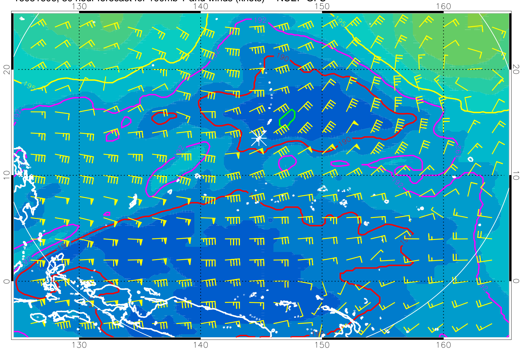
16081606, 30 hour forecast for 100mb T and winds (knots) -- NCEP GFS
