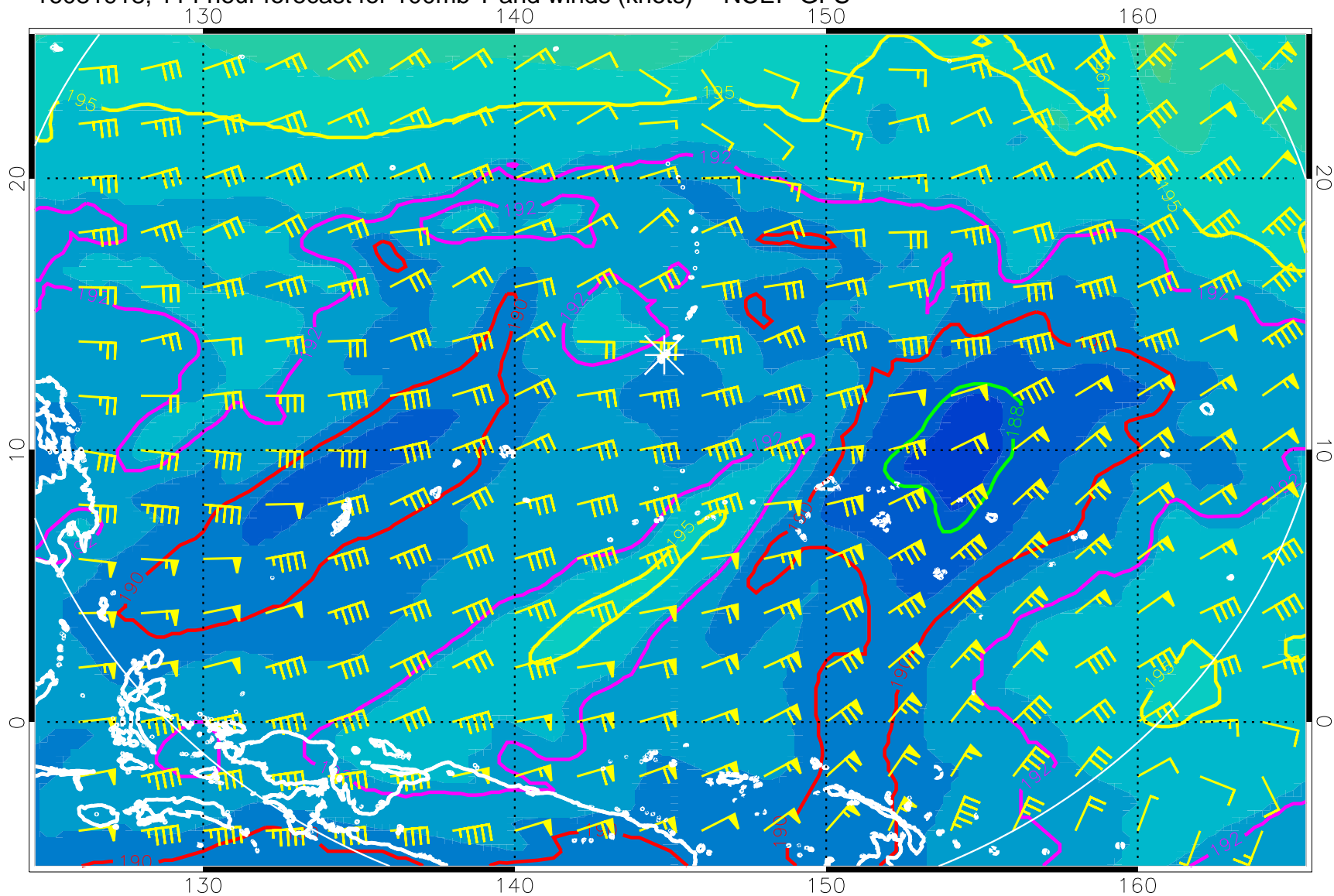
16081918, 114 hour forecast for 100mb T and winds (knots) -- NCEP GFS
