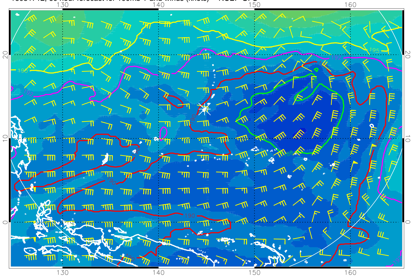
16081712, 60 hour forecast for 100mb T and winds (knots) -- NCEP GFS
