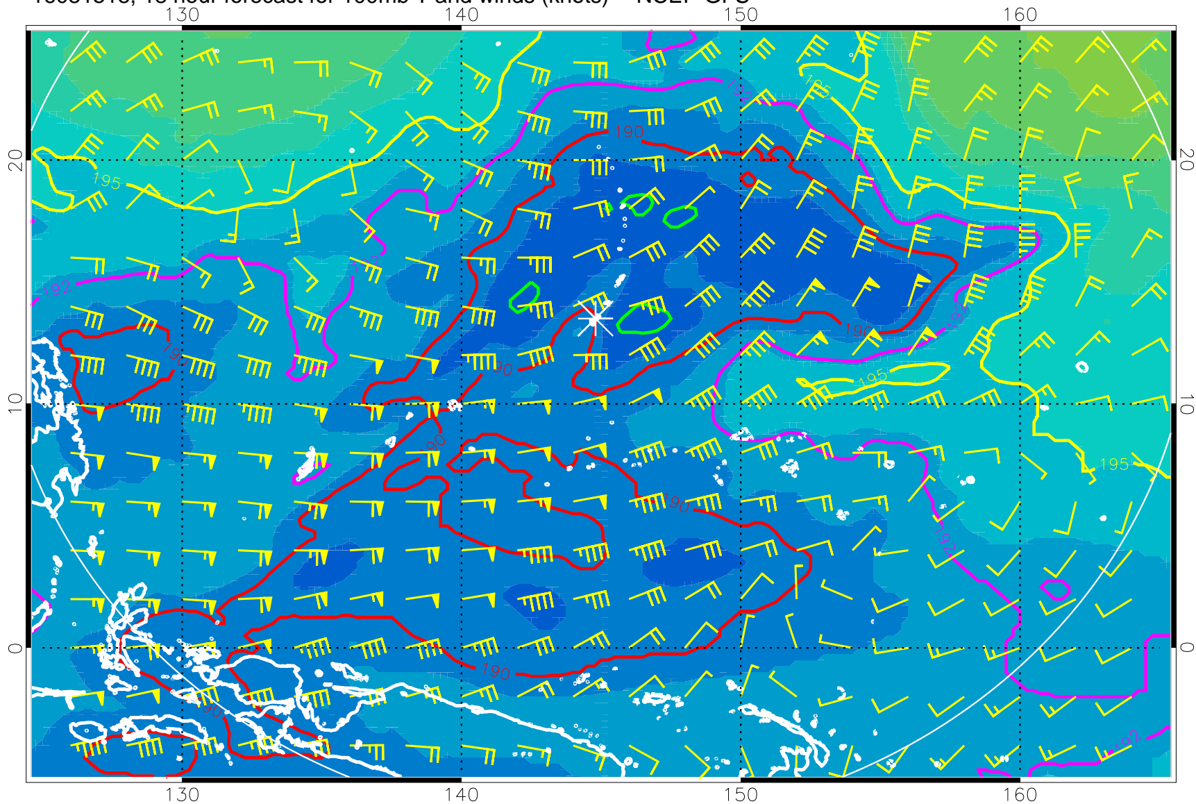
16081518, 18 hour forecast for 100mb T and winds (knots) -- NCEP GFS
