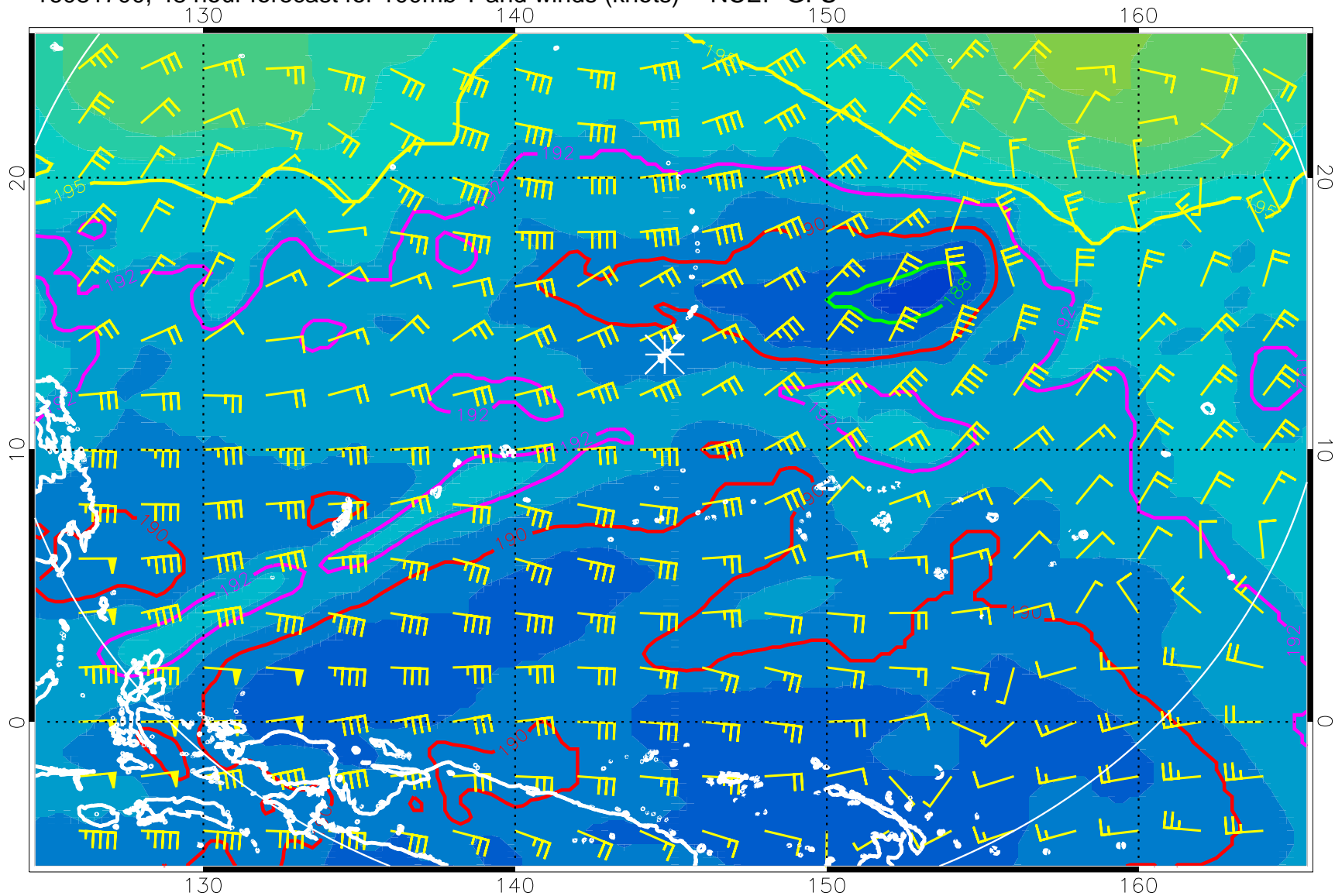
16081700, 48 hour forecast for 100mb T and winds (knots) -- NCEP GFS
