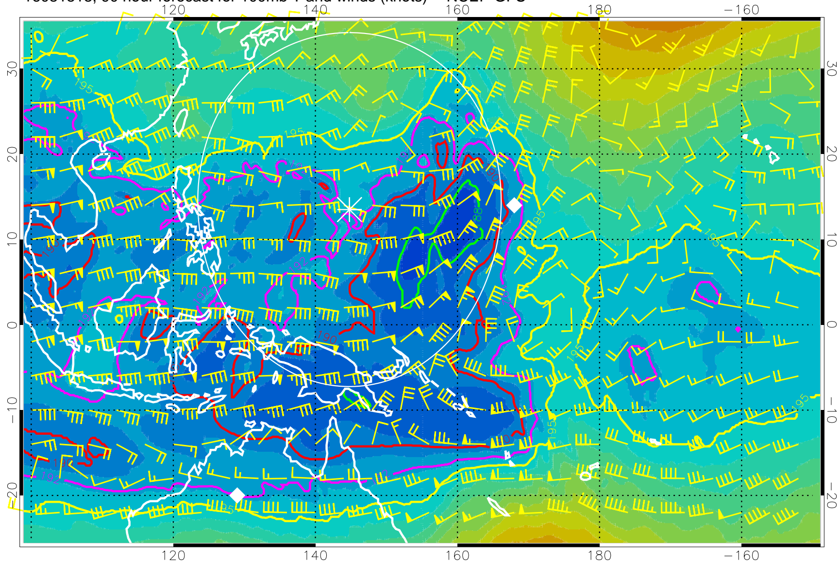
16081818, 90 hour forecast for 100mb T and winds (knots) -- NCEP GFS
