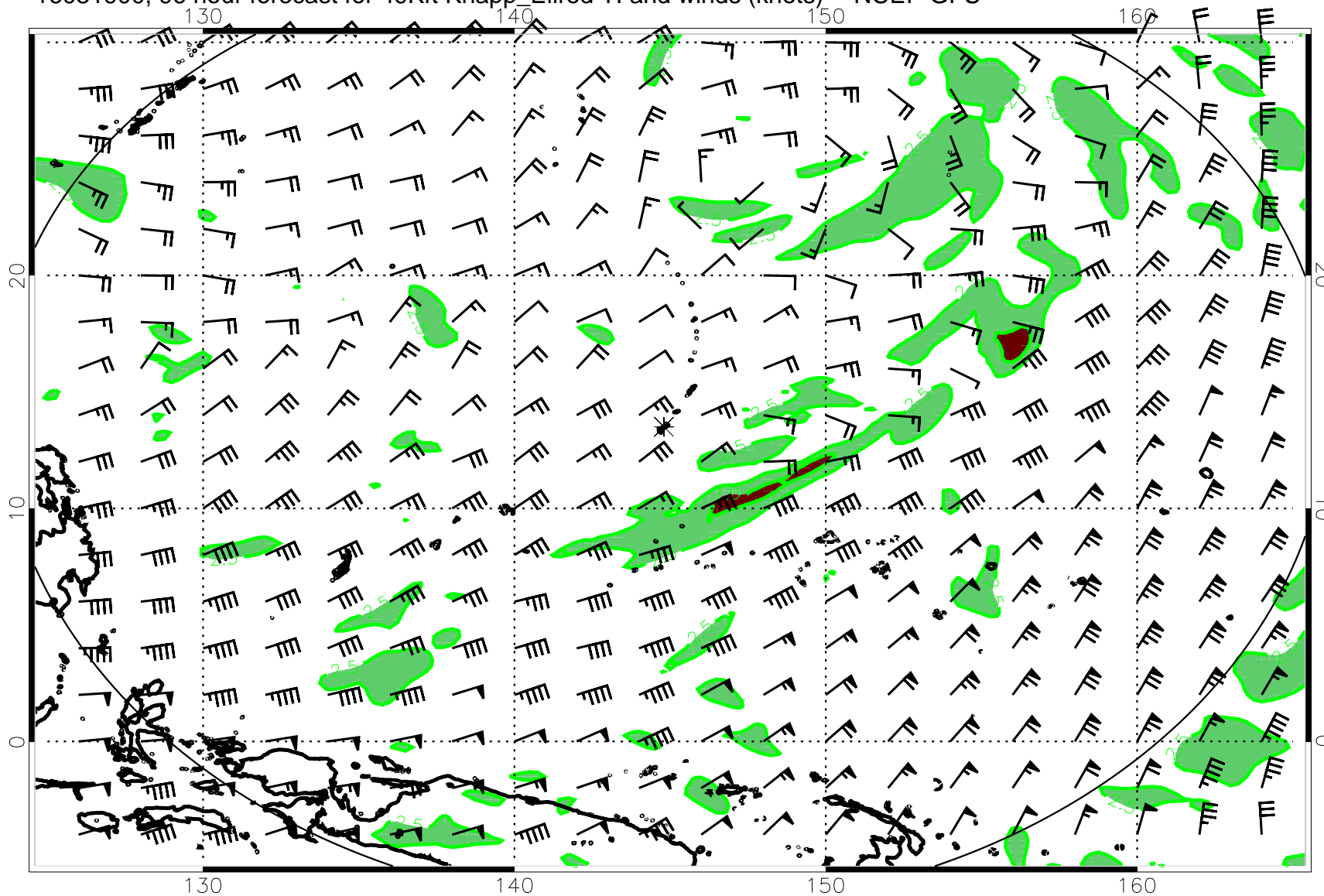
16081900, 96 hour forecast for 49Kft Knapp_Ellrod TI and winds (knots) -- NCEP GFS
