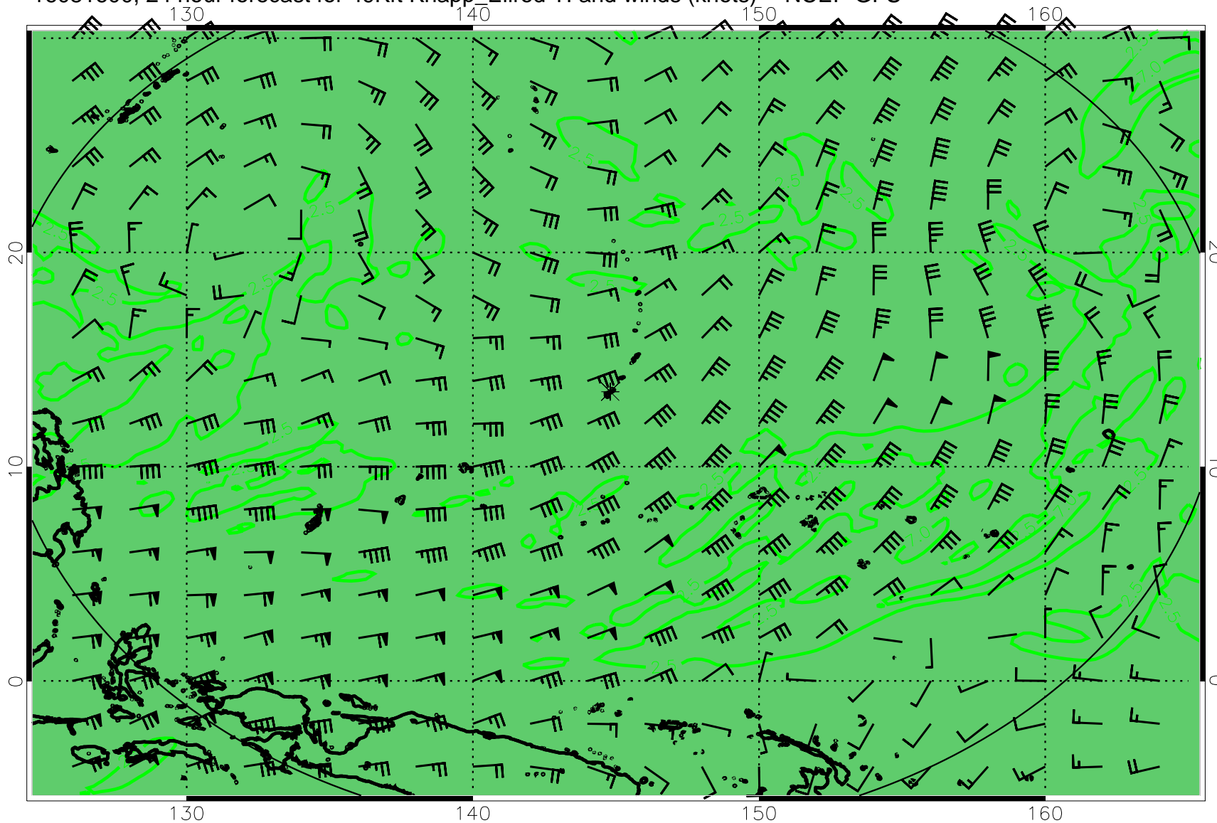
16081600, 24 hour forecast for 49Kft Knapp_Ellrod TI and winds (knots) -- NCEP GFS
