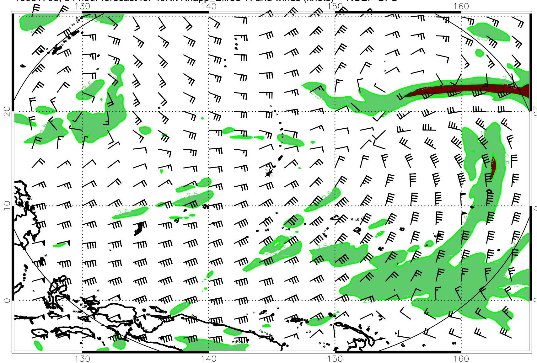
16081706, 54 hour forecast for 49Kft Knapp_Ellrod TI and winds (knots) -- NCEP GFS
