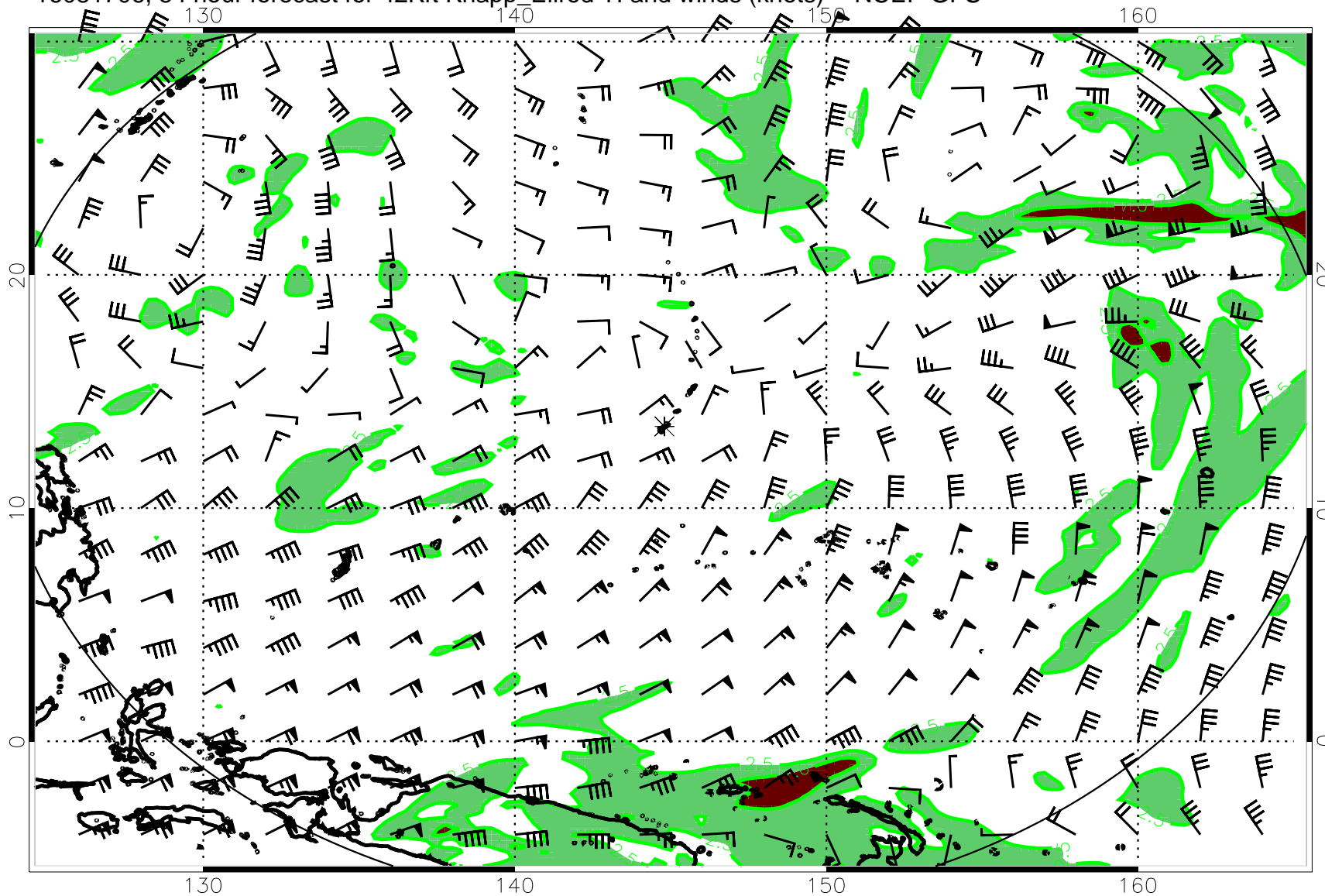
16081706, 54 hour forecast for 42Kft Knapp_Ellrod TI and winds (knots) -- NCEP GFS
