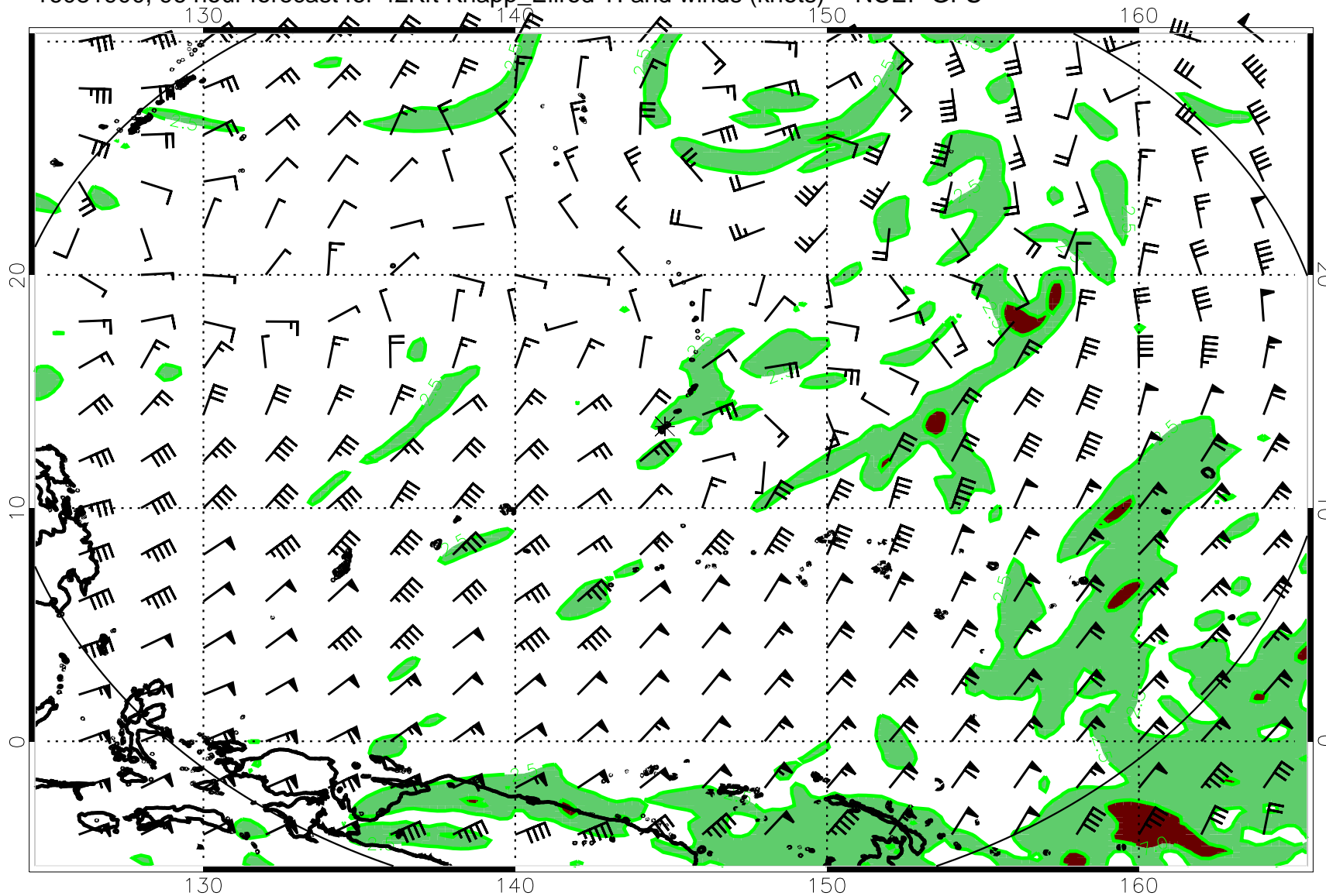
16081900, 96 hour forecast for 42Kft Knapp_Ellrod TI and winds (knots) -- NCEP GFS
