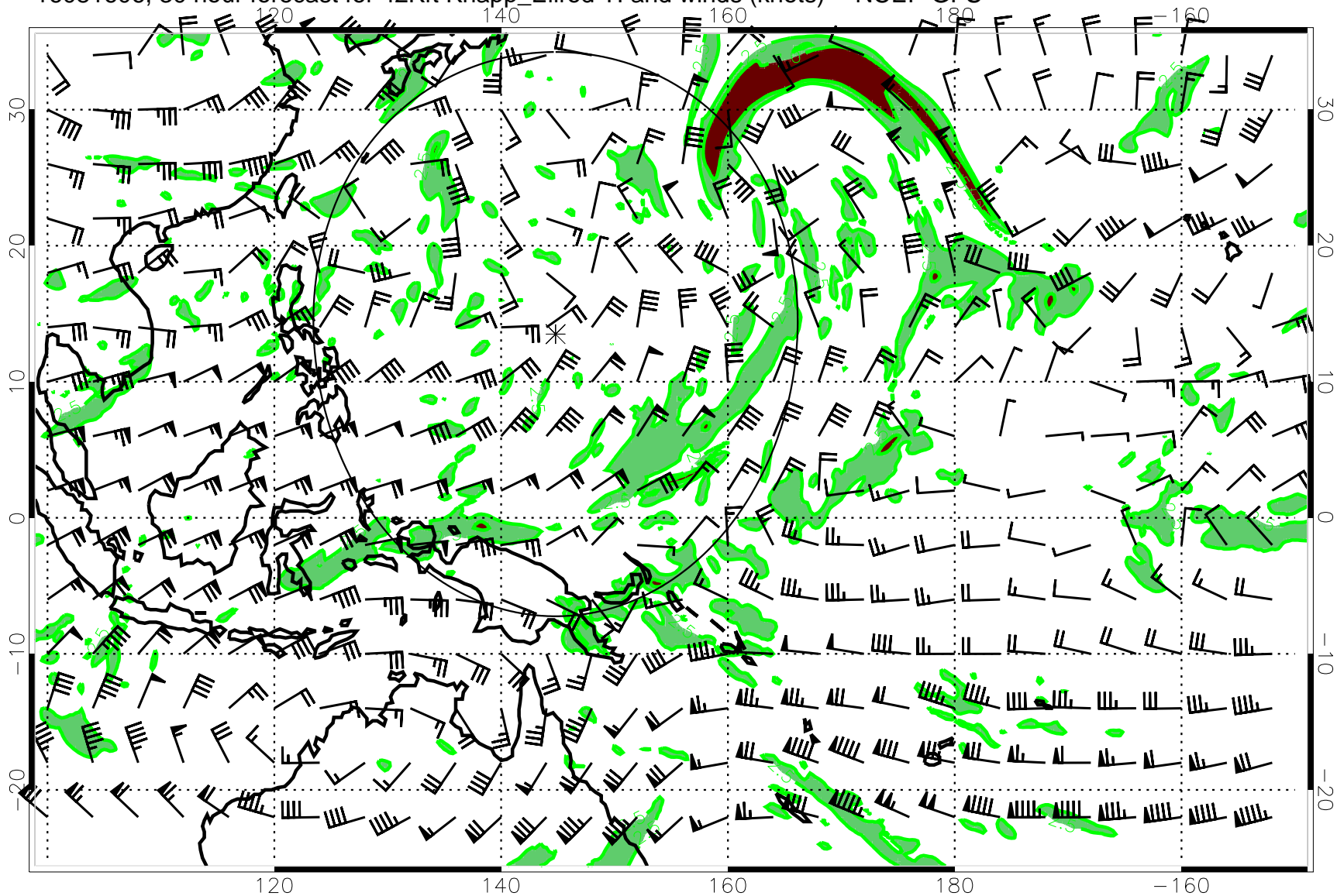
16081606, 30 hour forecast for 42Kft Knapp_Ellrod TI and winds (knots) -- NCEP GFS
