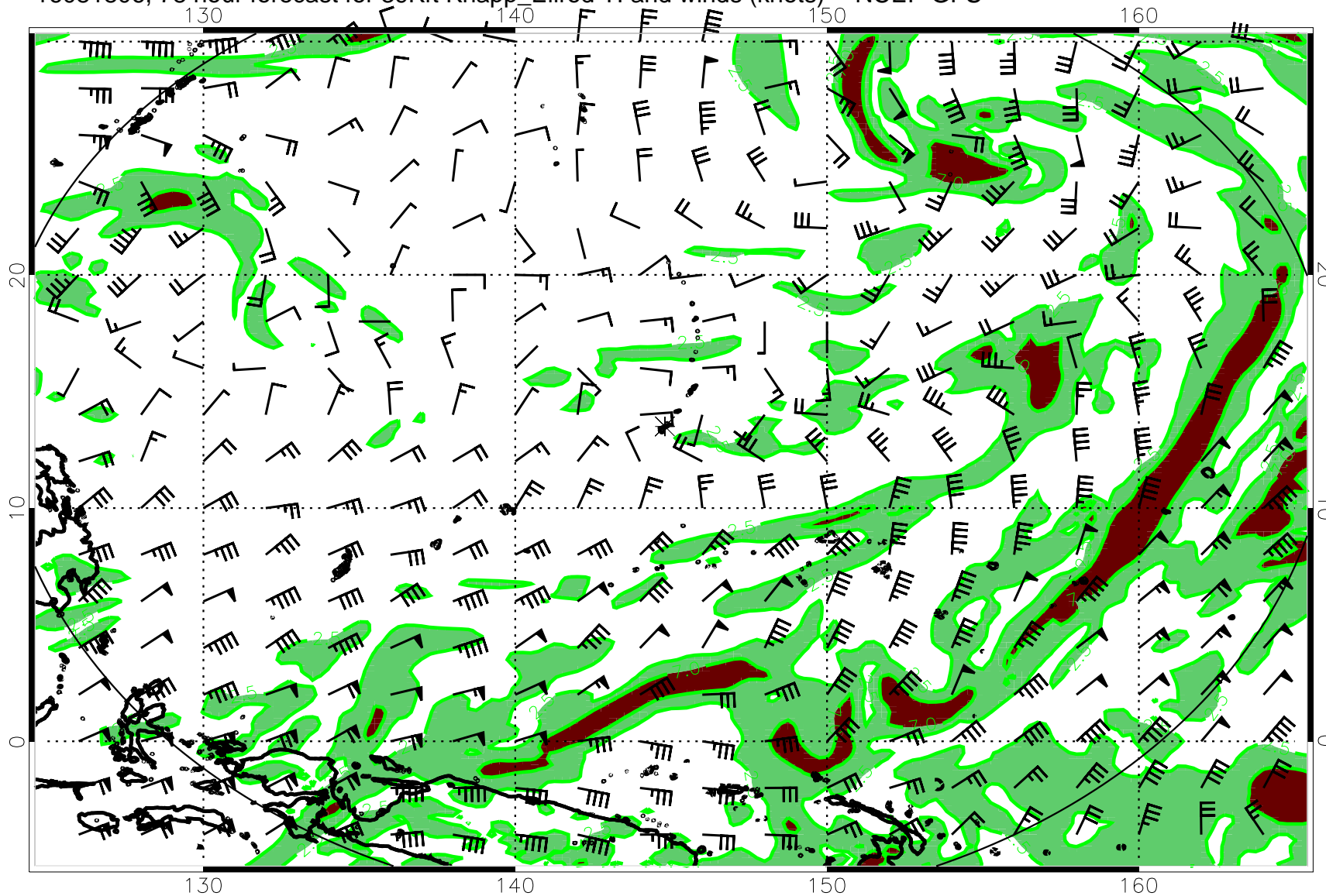
16081806, 78 hour forecast for 39Kft Knapp_Ellrod TI and winds (knots) -- NCEP GFS
