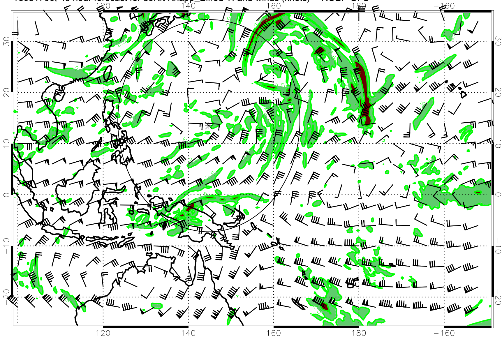
16081700, 48 hour forecast for 39Kft Knapp_Ellrod TI and winds (knots) -- NCEP GFS
