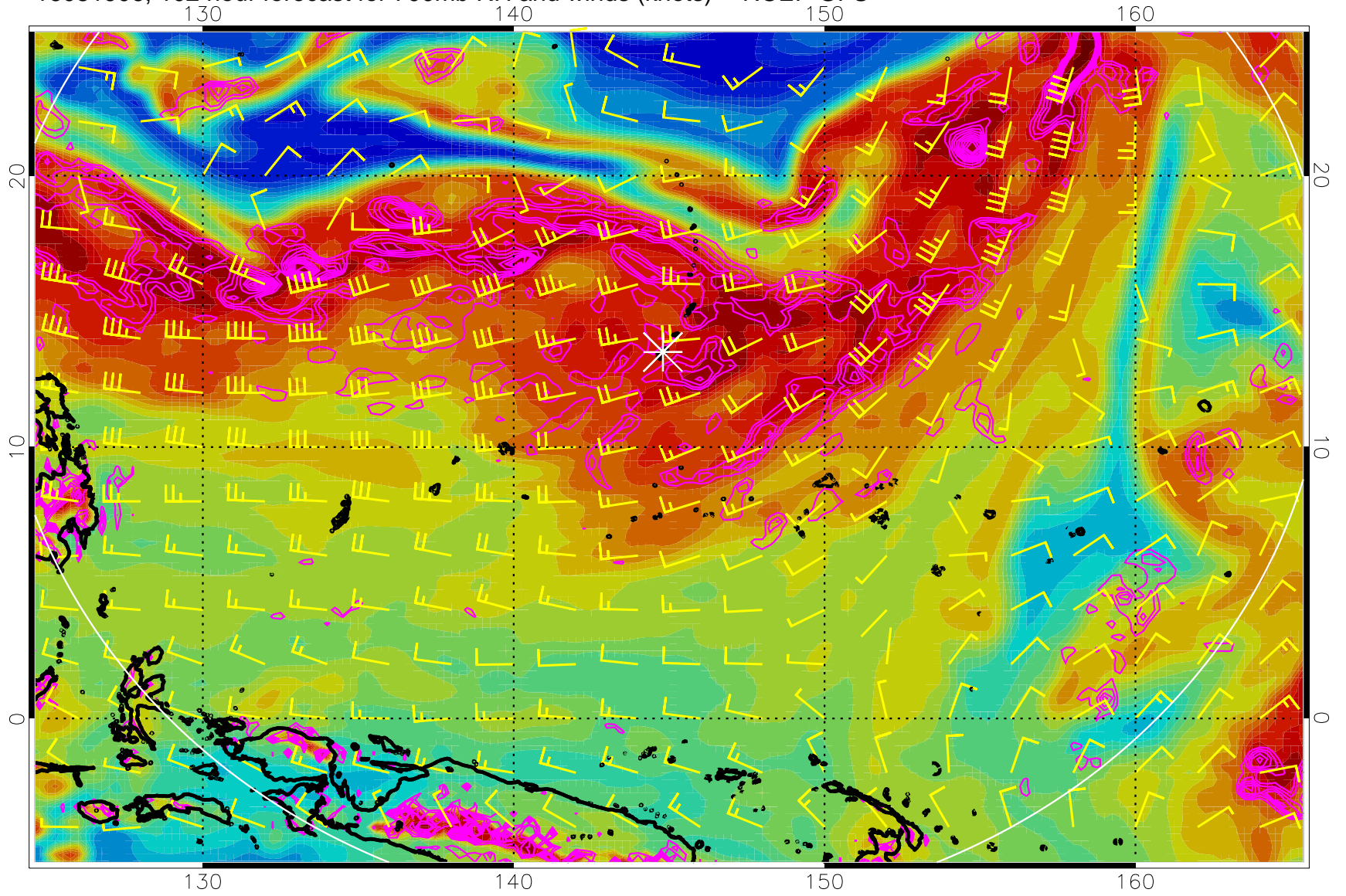
16081906, 102 hour forecast for 700mb RH and winds (knots) -- NCEP GFS
