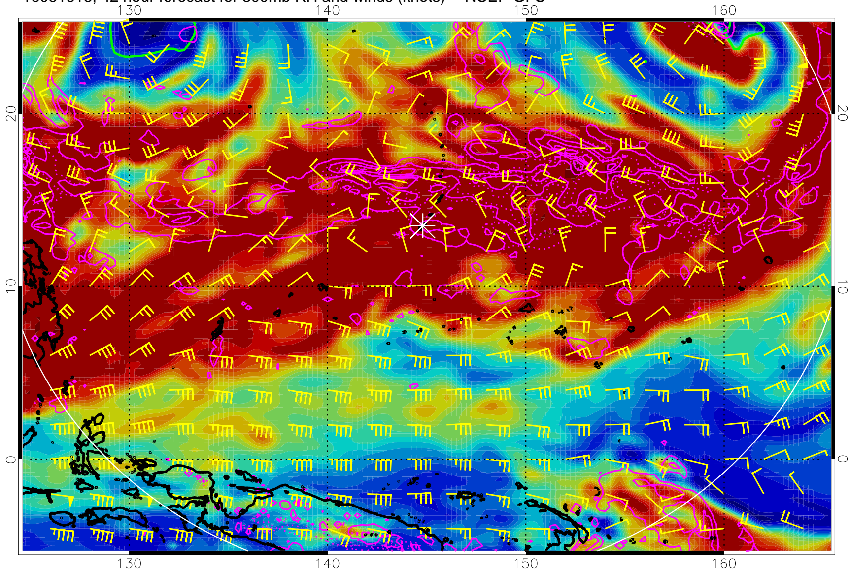
16081618, 42 hour forecast for 300mb RH and winds (knots) -- NCEP GFS
