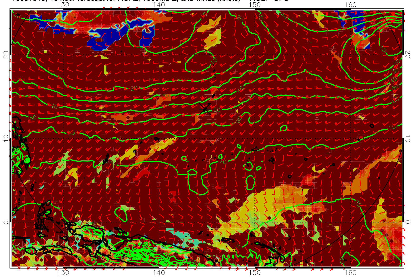
16081518, 18 hour forecast for HCAL, 1000mb Z, and winds (knots) -- NCEP GFS
