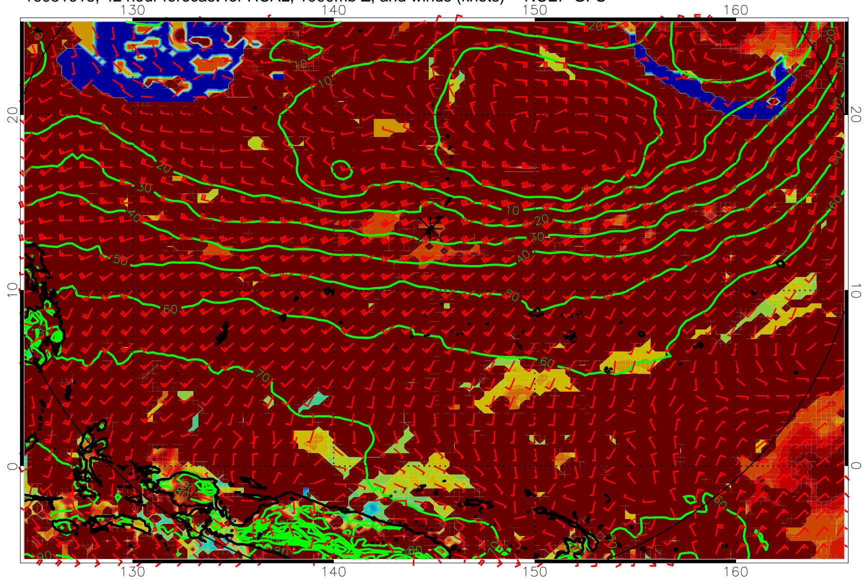
16081618, 42 hour forecast for HCAL, 1000mb Z, and winds (knots) -- NCEP GFS
