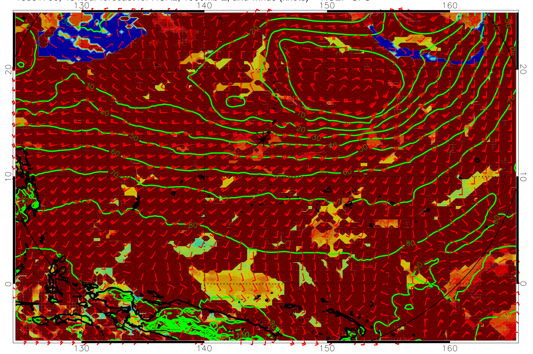
16081700, 48 hour forecast for HCAL, 1000mb Z, and winds (knots) -- NCEP GFS
