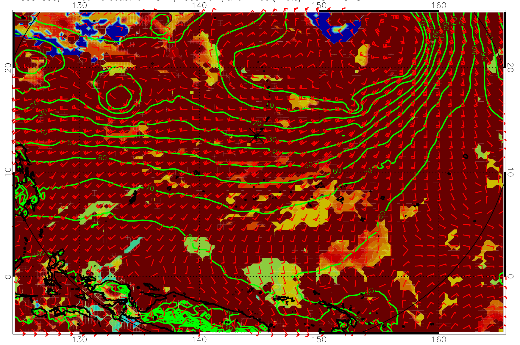
16081800, 72 hour forecast for HCAL, 1000mb Z, and winds (knots) -- NCEP GFS
