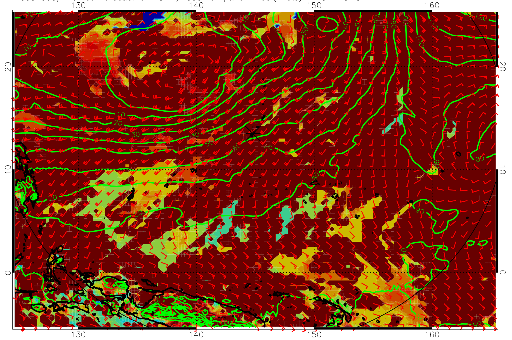
16082000, 120 hour forecast for HCAL, 1000mb Z, and winds (knots) -- NCEP GFS
