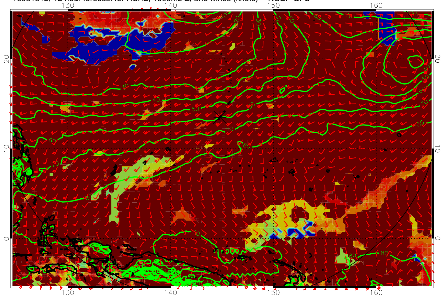
16081512, 12 hour forecast for HCAL, 1000mb Z, and winds (knots) -- NCEP GFS
