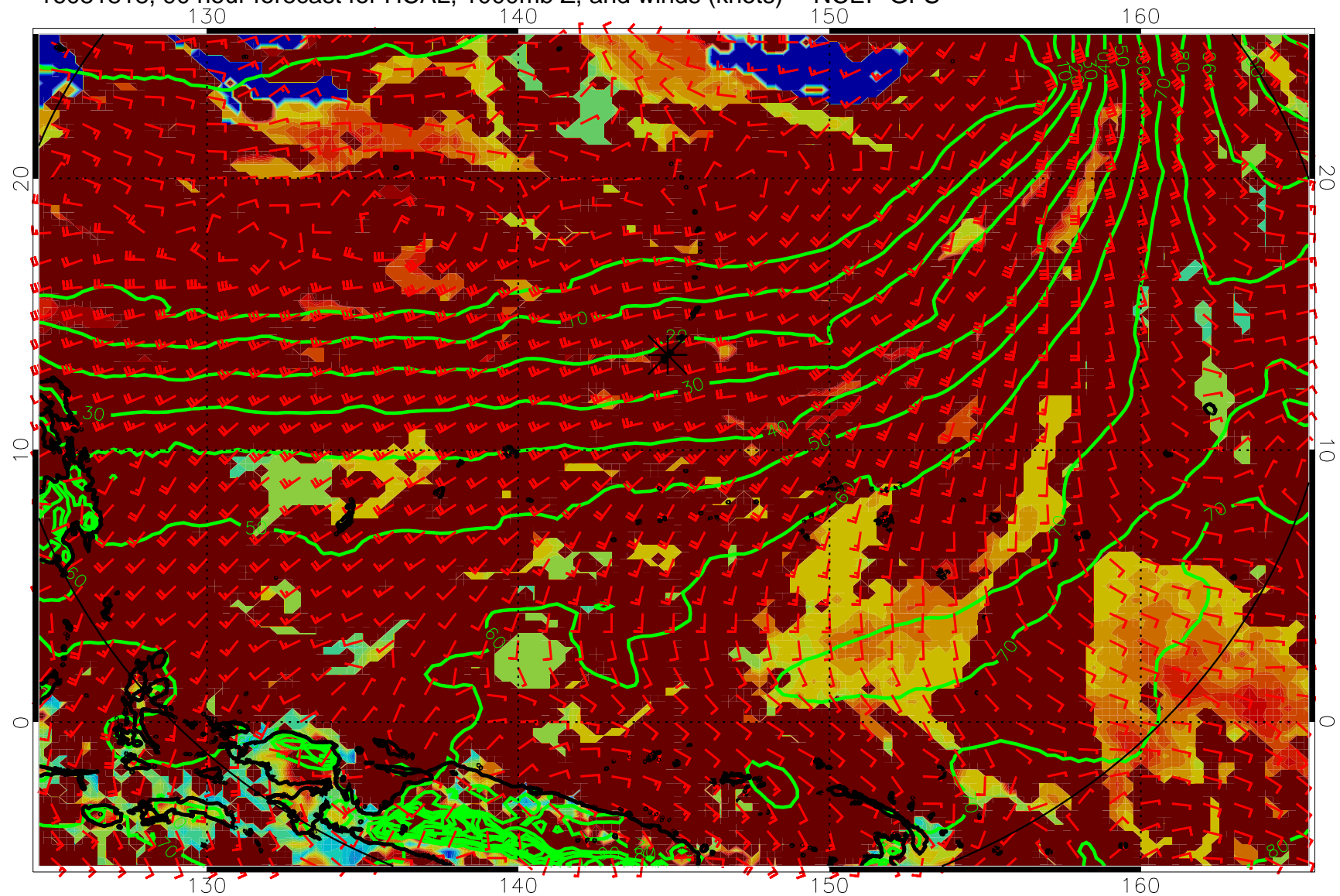
16081818, 90 hour forecast for HCAL, 1000mb Z, and winds (knots) -- NCEP GFS
