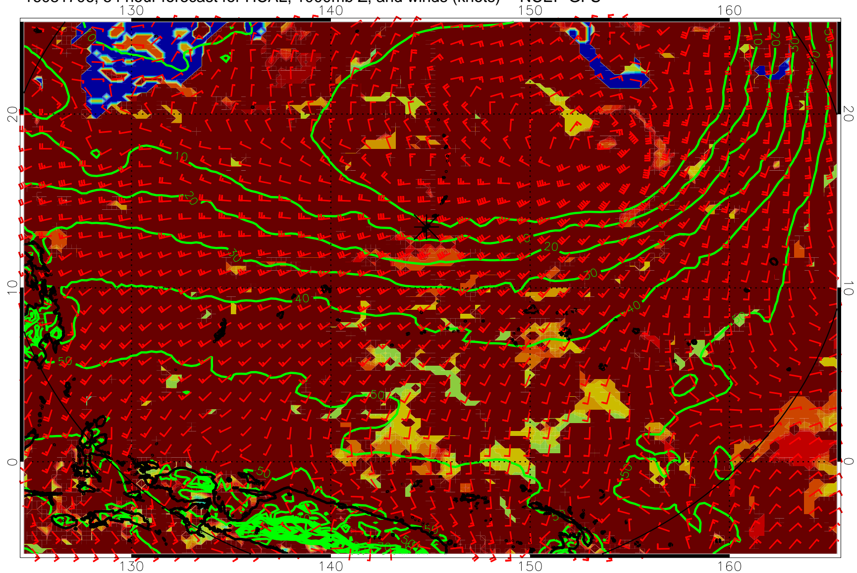
16081706, 54 hour forecast for HCAL, 1000mb Z, and winds (knots) -- NCEP GFS
