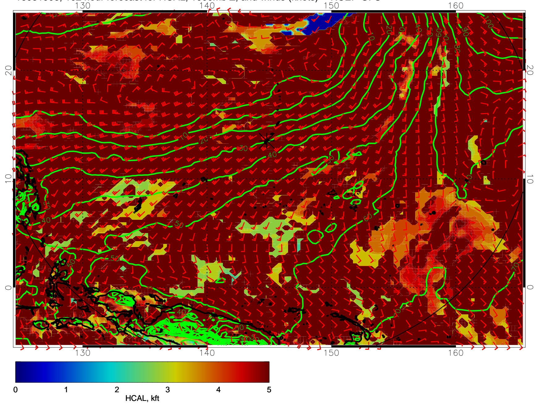
16081906, 102 hour forecast for HCAL, 1000mb Z, and winds (knots) -- NCEP GFS
