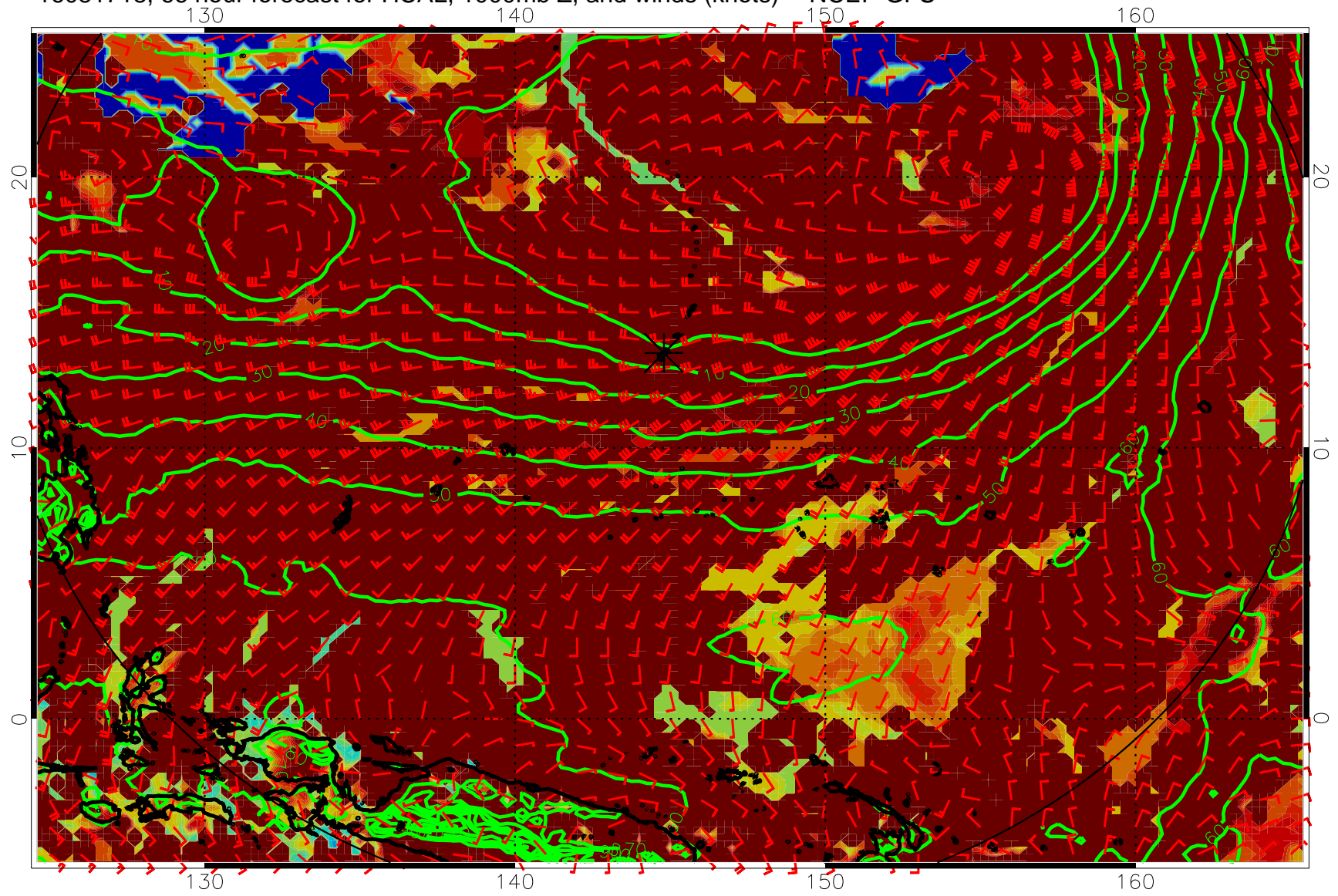
16081718, 66 hour forecast for HCAL, 1000mb Z, and winds (knots) -- NCEP GFS
