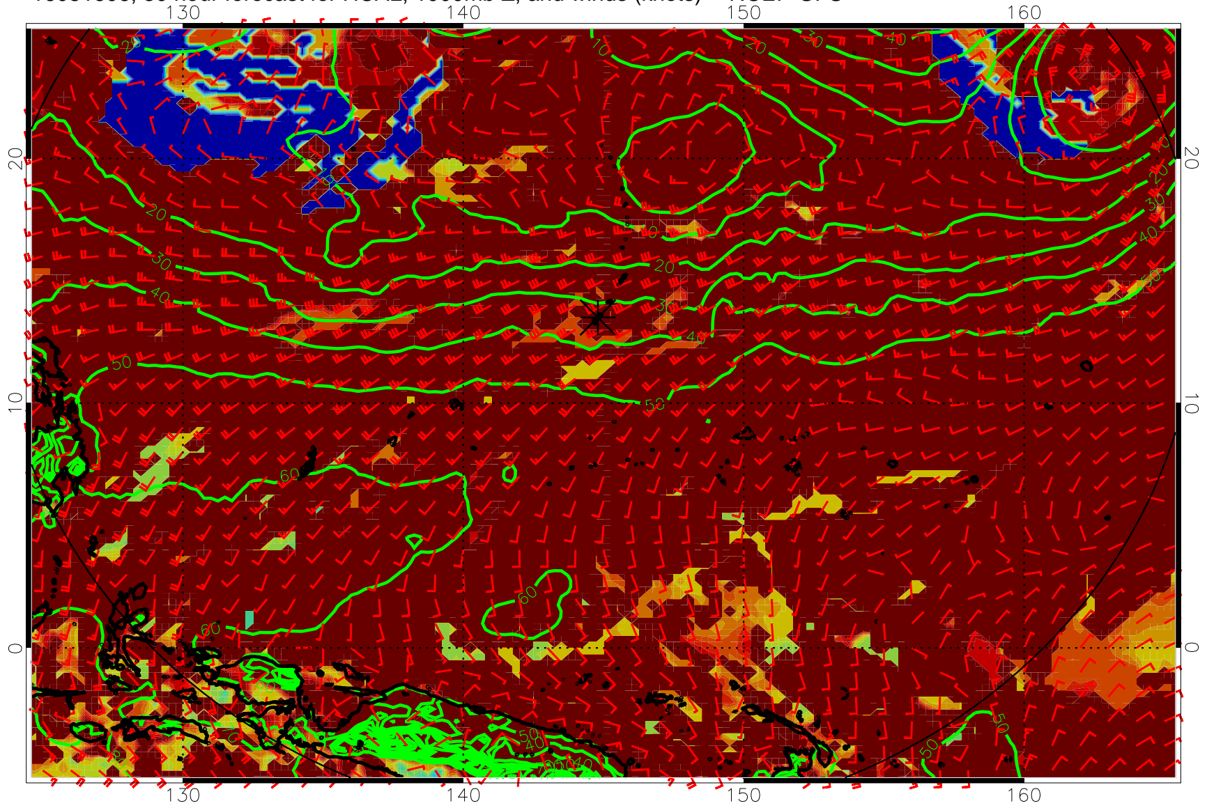
16081606, 30 hour forecast for HCAL, 1000mb Z, and winds (knots) -- NCEP GFS
