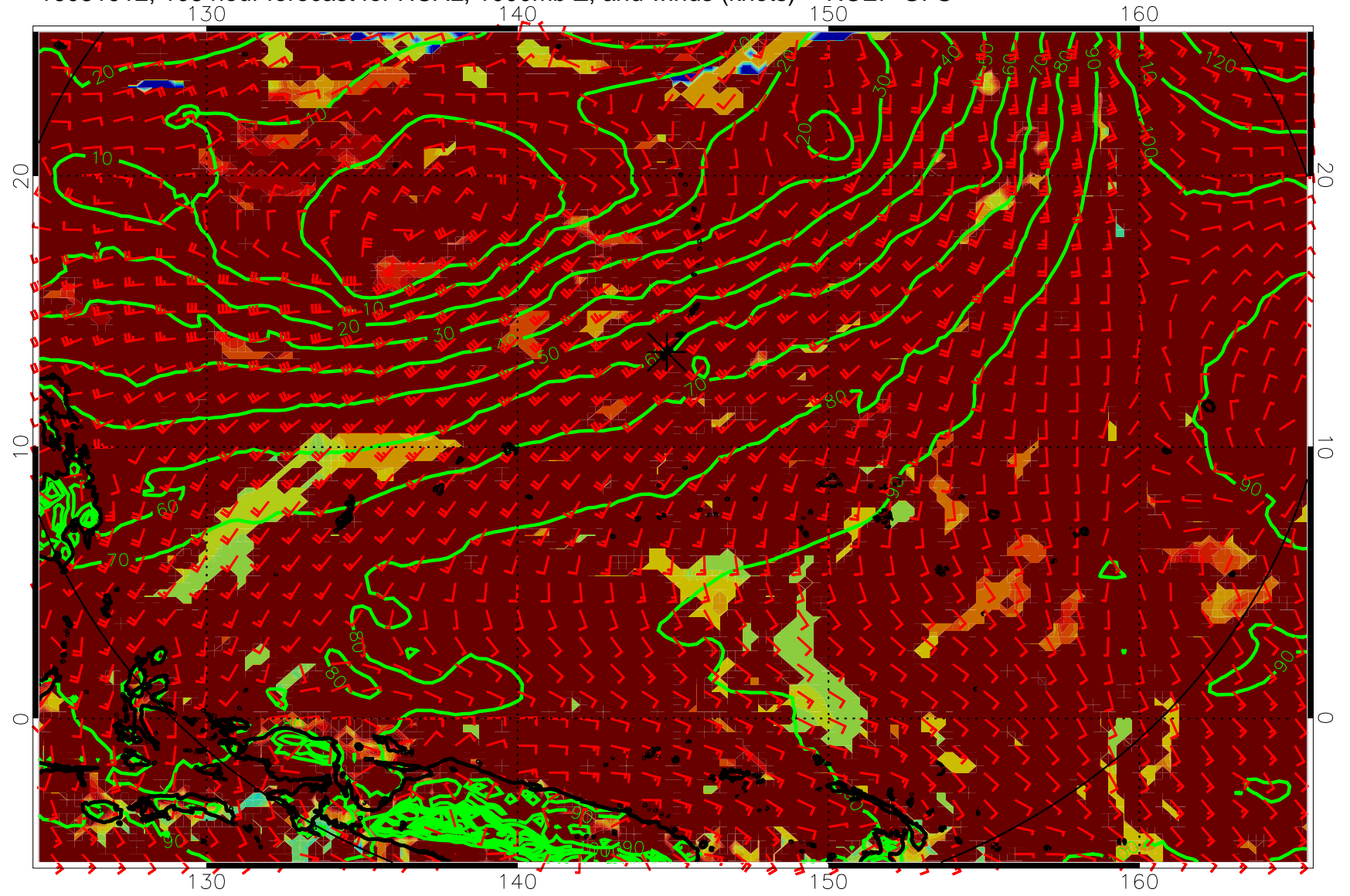
16081912, 108 hour forecast for HCAL, 1000mb Z, and winds (knots) -- NCEP GFS
