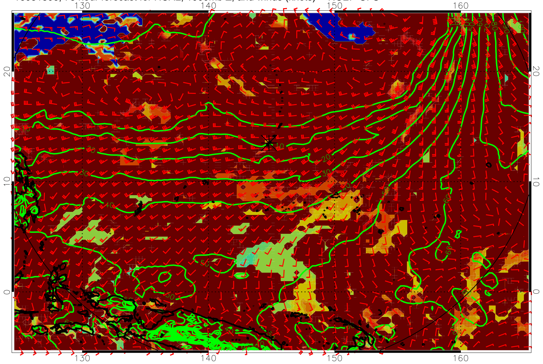
16081806, 78 hour forecast for HCAL, 1000mb Z, and winds (knots) -- NCEP GFS
