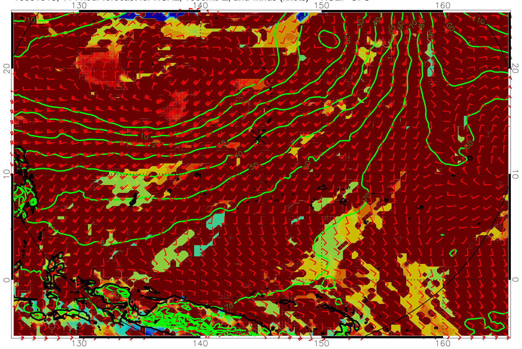
16081918, 114 hour forecast for HCAL, 1000mb Z, and winds (knots) -- NCEP GFS
