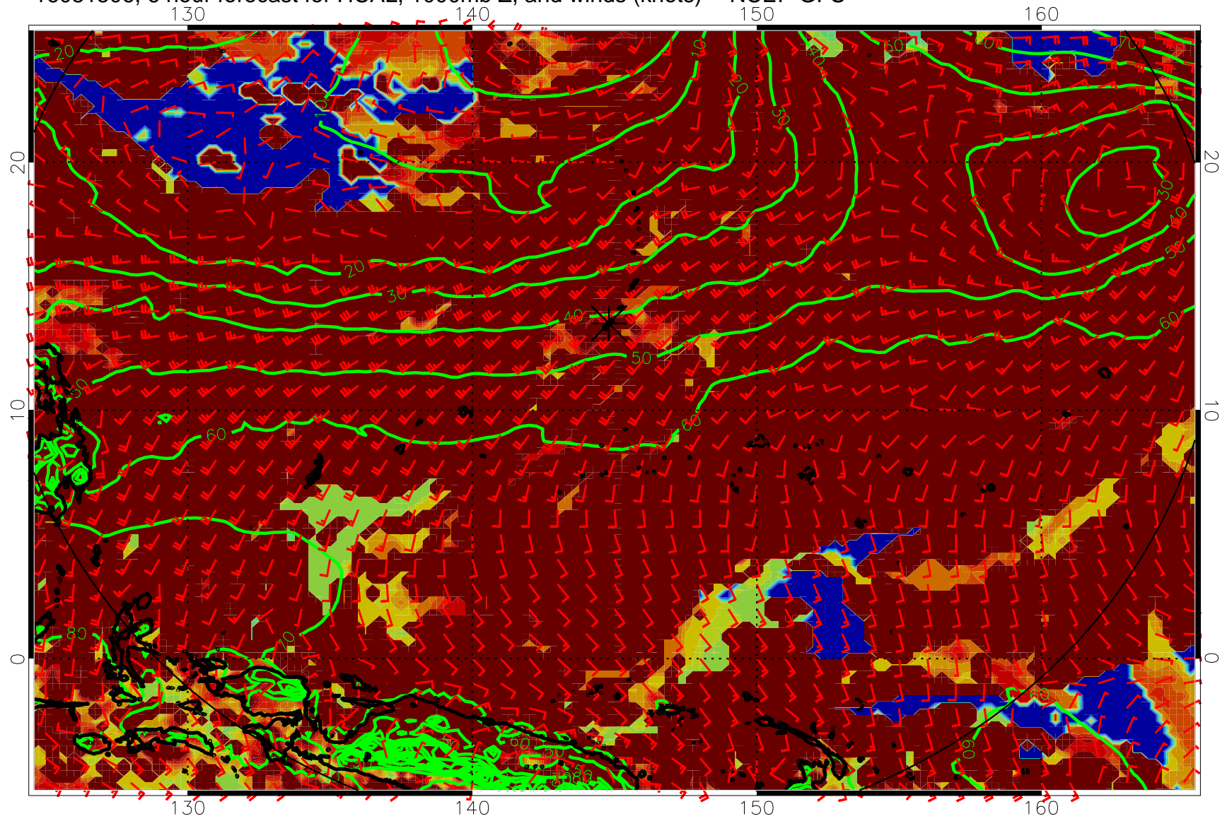
16081506, 6 hour forecast for HCAL, 1000mb Z, and winds (knots) -- NCEP GFS
