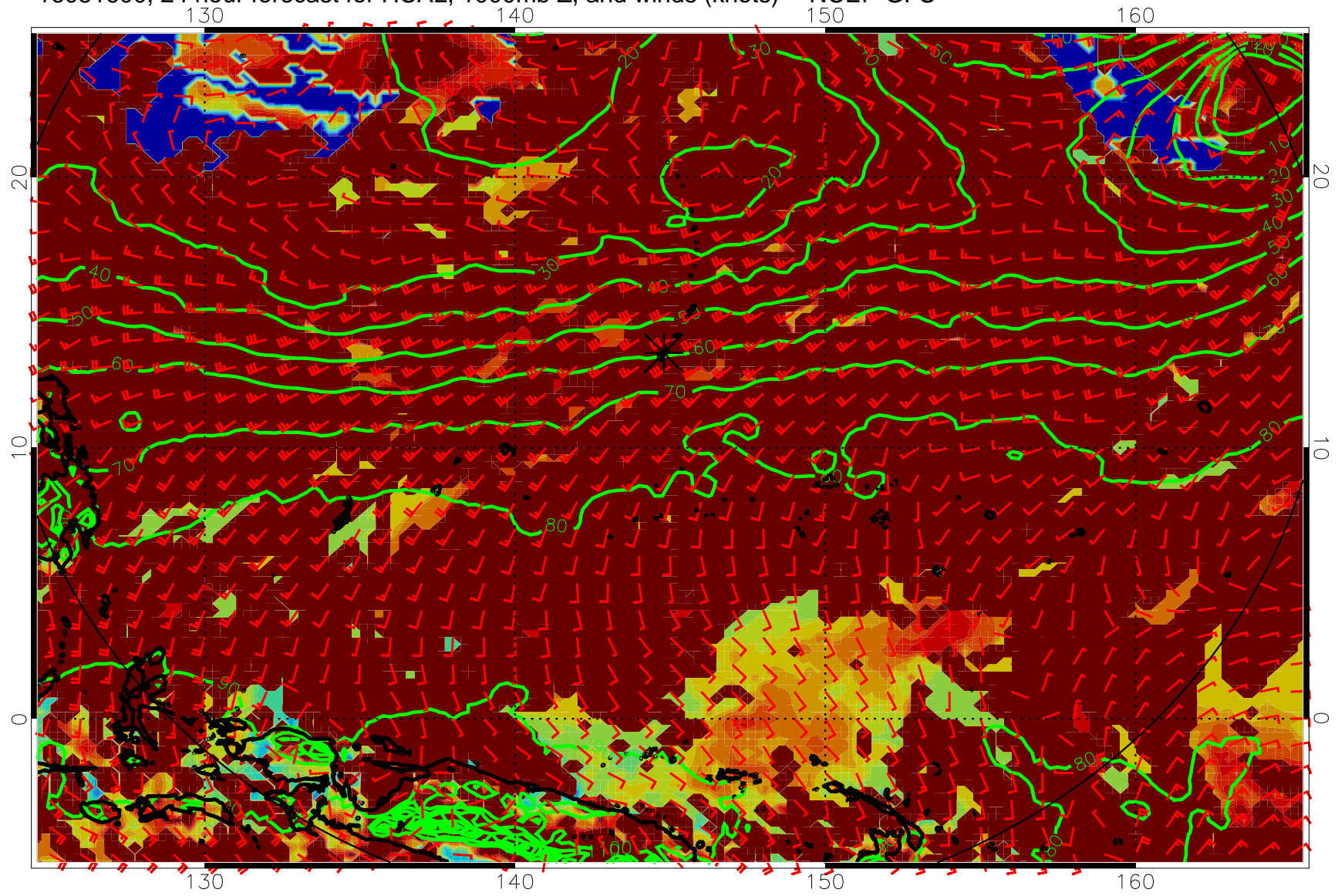
16081600, 24 hour forecast for HCAL, 1000mb Z, and winds (knots) -- NCEP GFS
