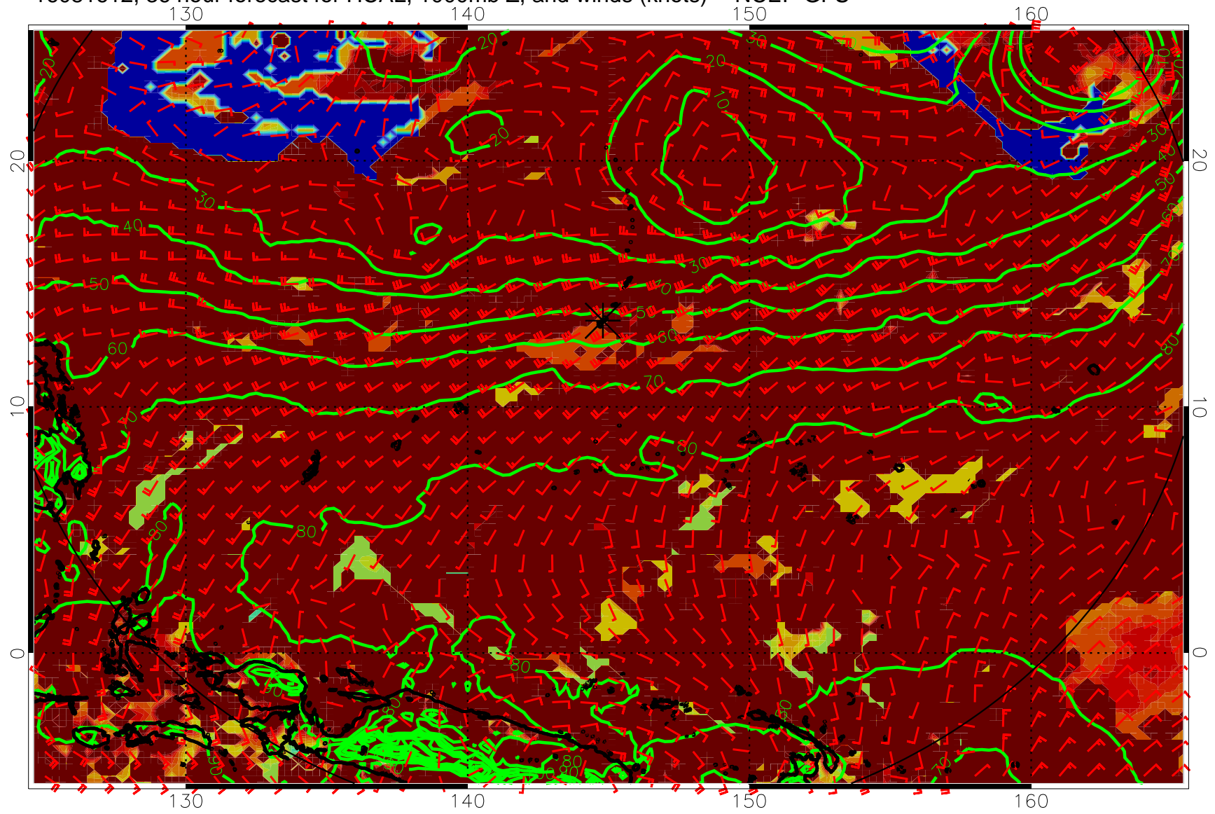
16081612, 36 hour forecast for HCAL, 1000mb Z, and winds (knots) -- NCEP GFS
