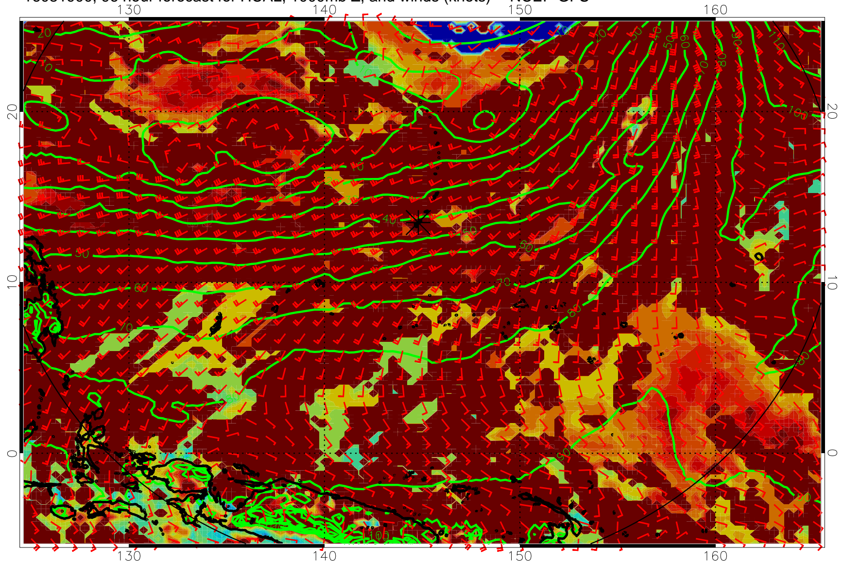
16081900, 96 hour forecast for HCAL, 1000mb Z, and winds (knots) -- NCEP GFS
