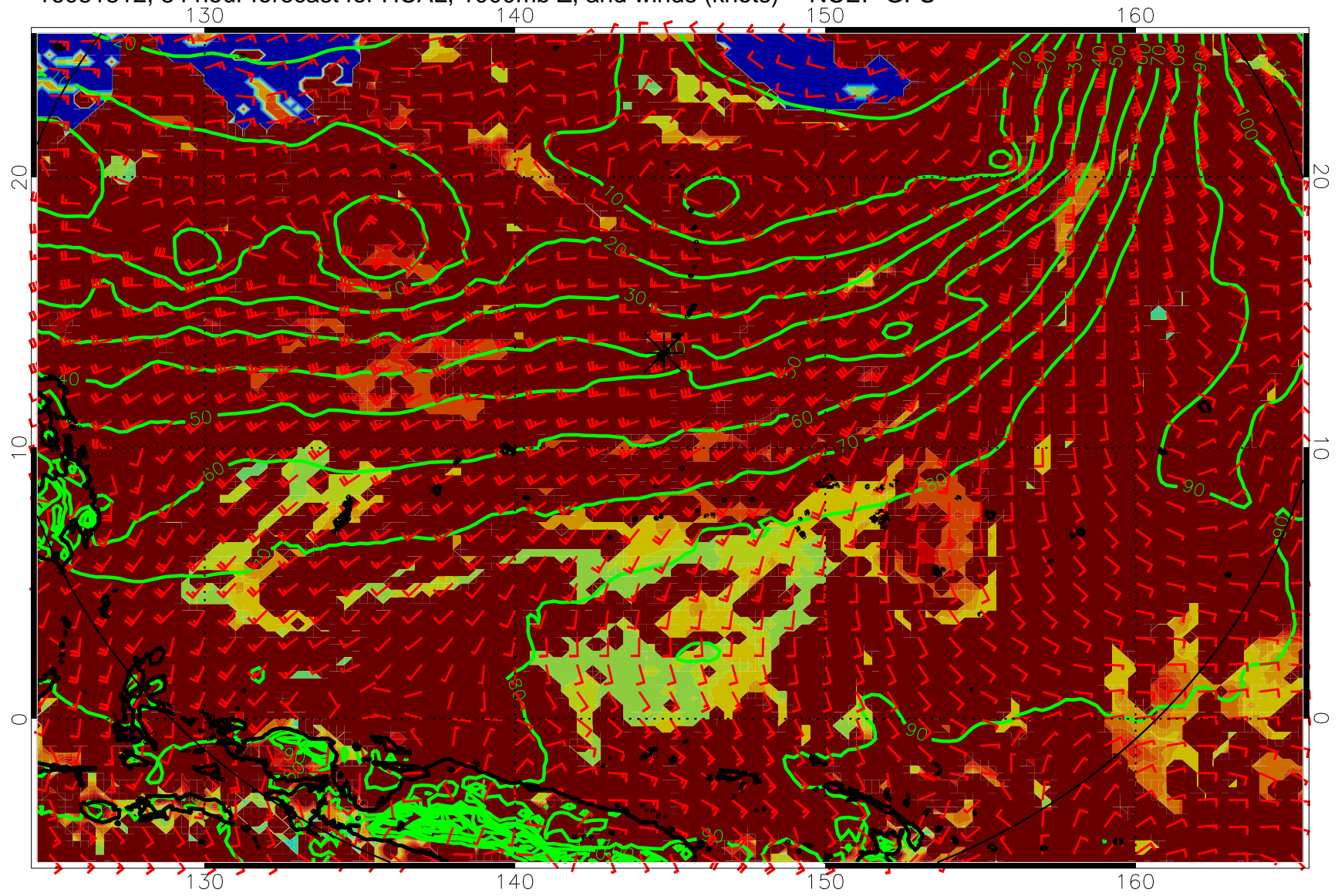
16081812, 84 hour forecast for HCAL, 1000mb Z, and winds (knots) -- NCEP GFS
