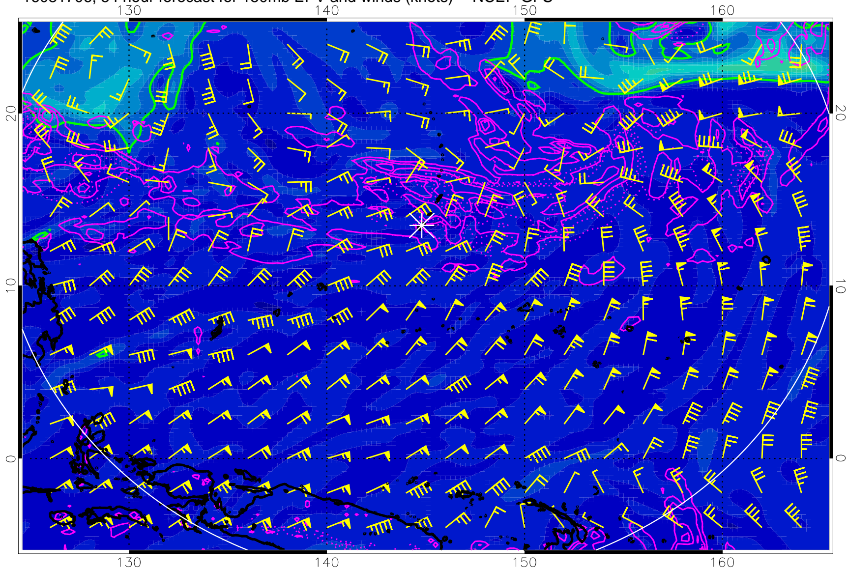
16081706, 54 hour forecast for 150mb EPV and winds (knots) -- NCEP GFS
