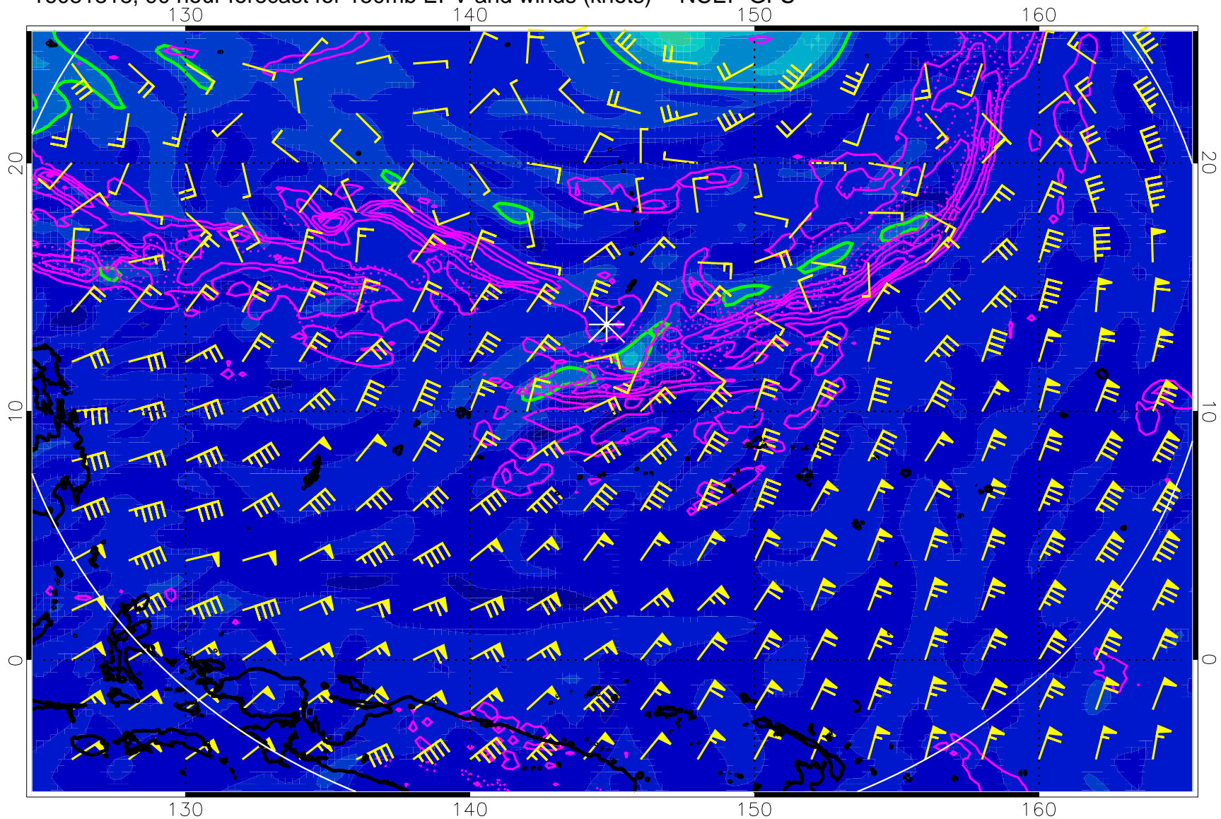
16081818, 90 hour forecast for 150mb EPV and winds (knots) -- NCEP GFS
