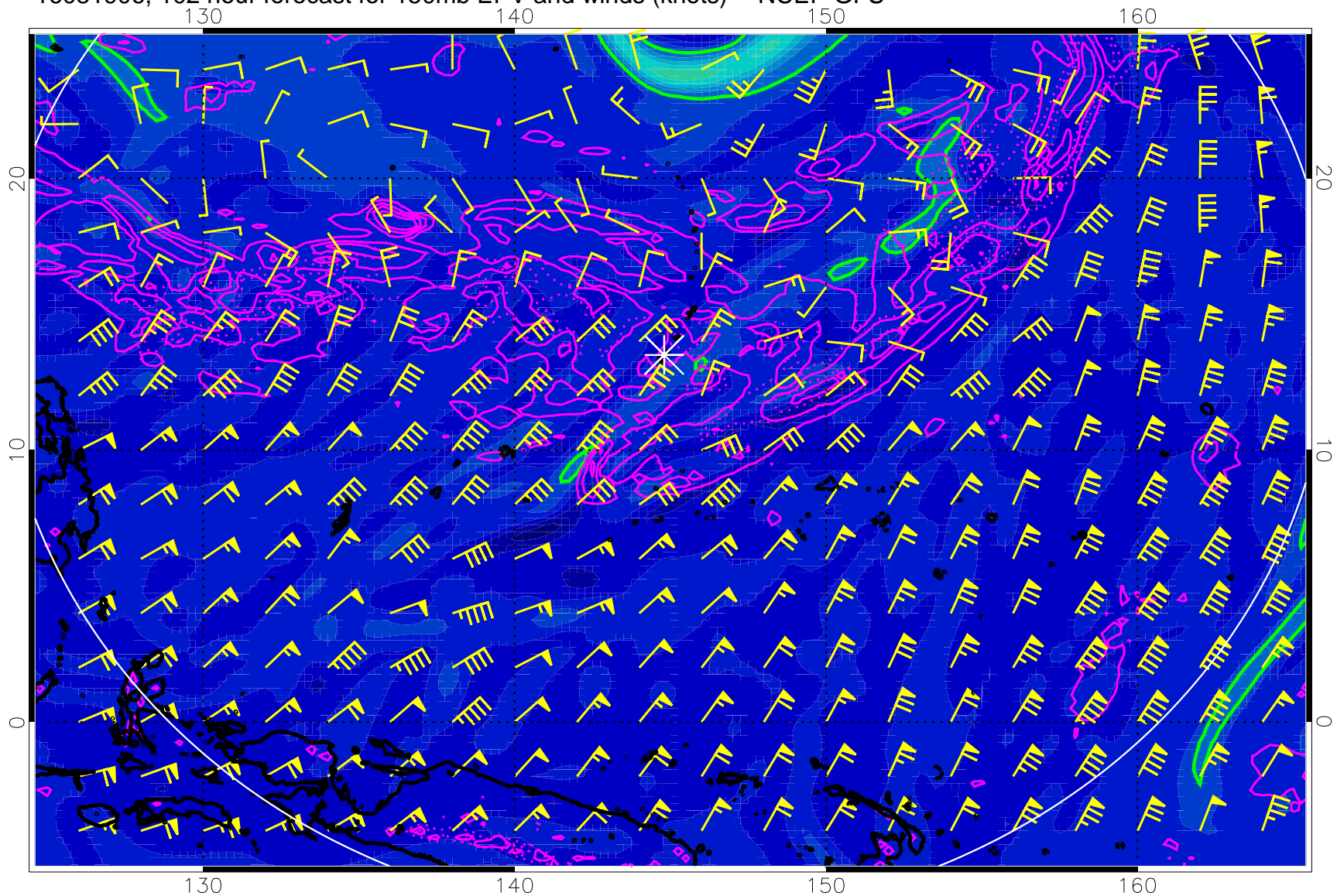
16081906, 102 hour forecast for 150mb EPV and winds (knots) -- NCEP GFS
