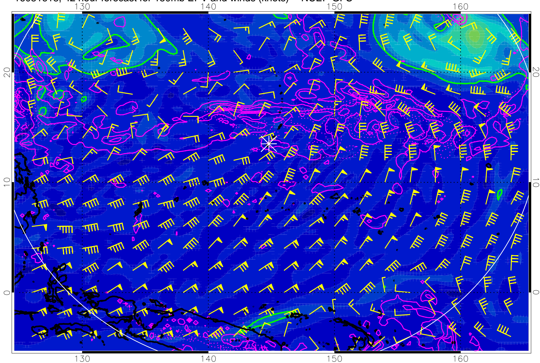
16081618, 42 hour forecast for 150mb EPV and winds (knots) -- NCEP GFS
