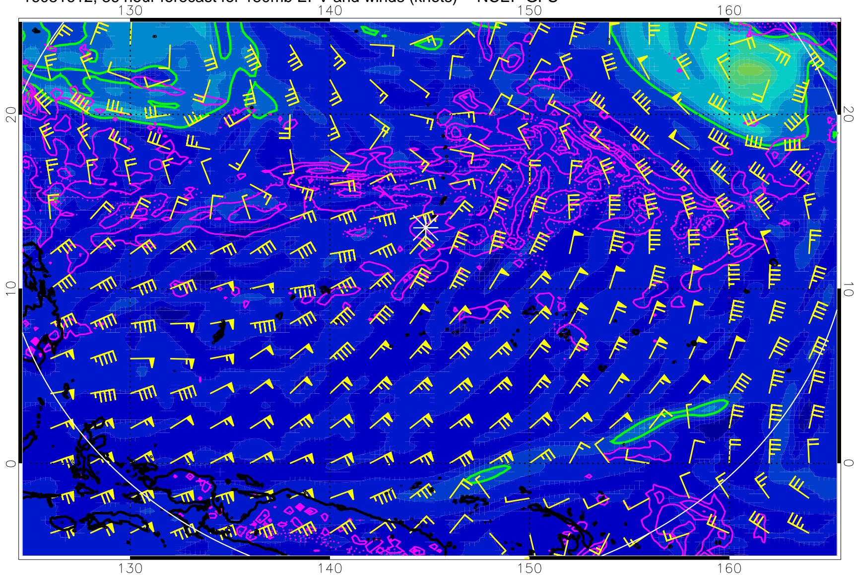
16081612, 36 hour forecast for 150mb EPV and winds (knots) -- NCEP GFS
