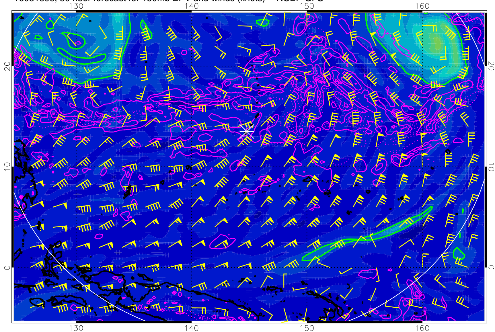
16081606, 30 hour forecast for 150mb EPV and winds (knots) -- NCEP GFS
