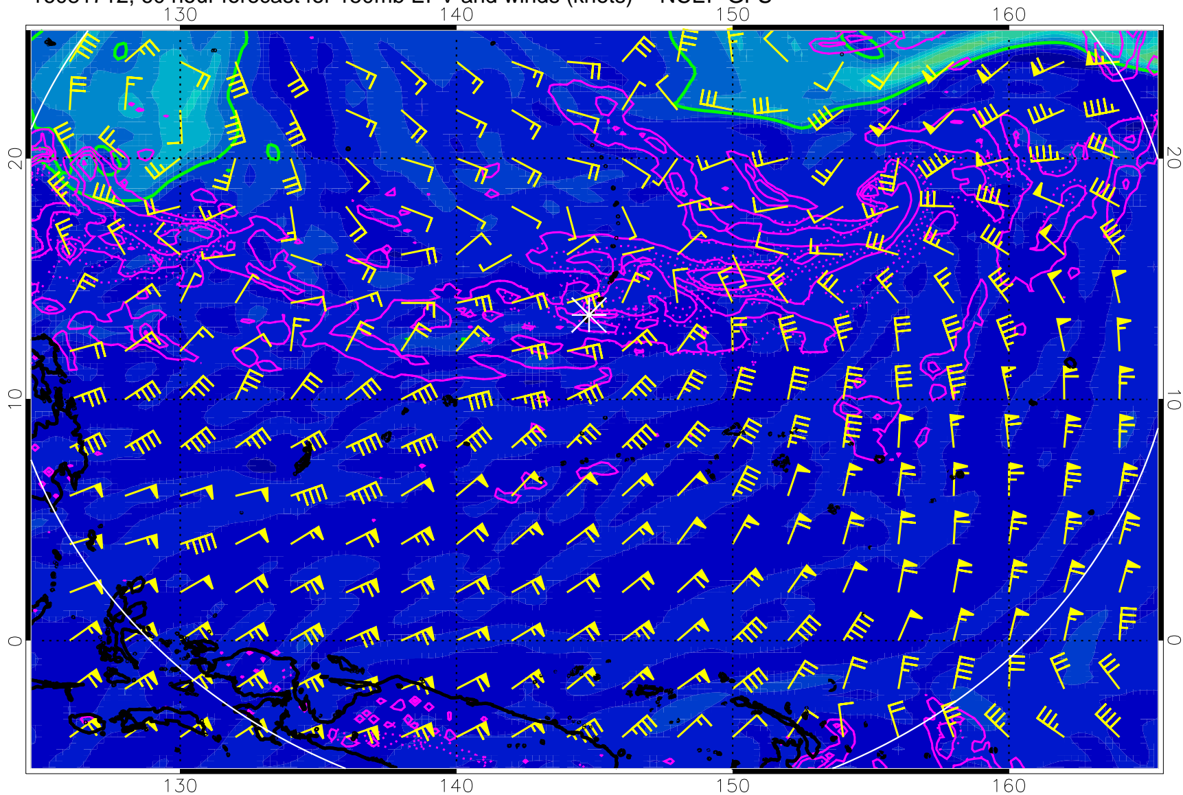
16081712, 60 hour forecast for 150mb EPV and winds (knots) -- NCEP GFS
