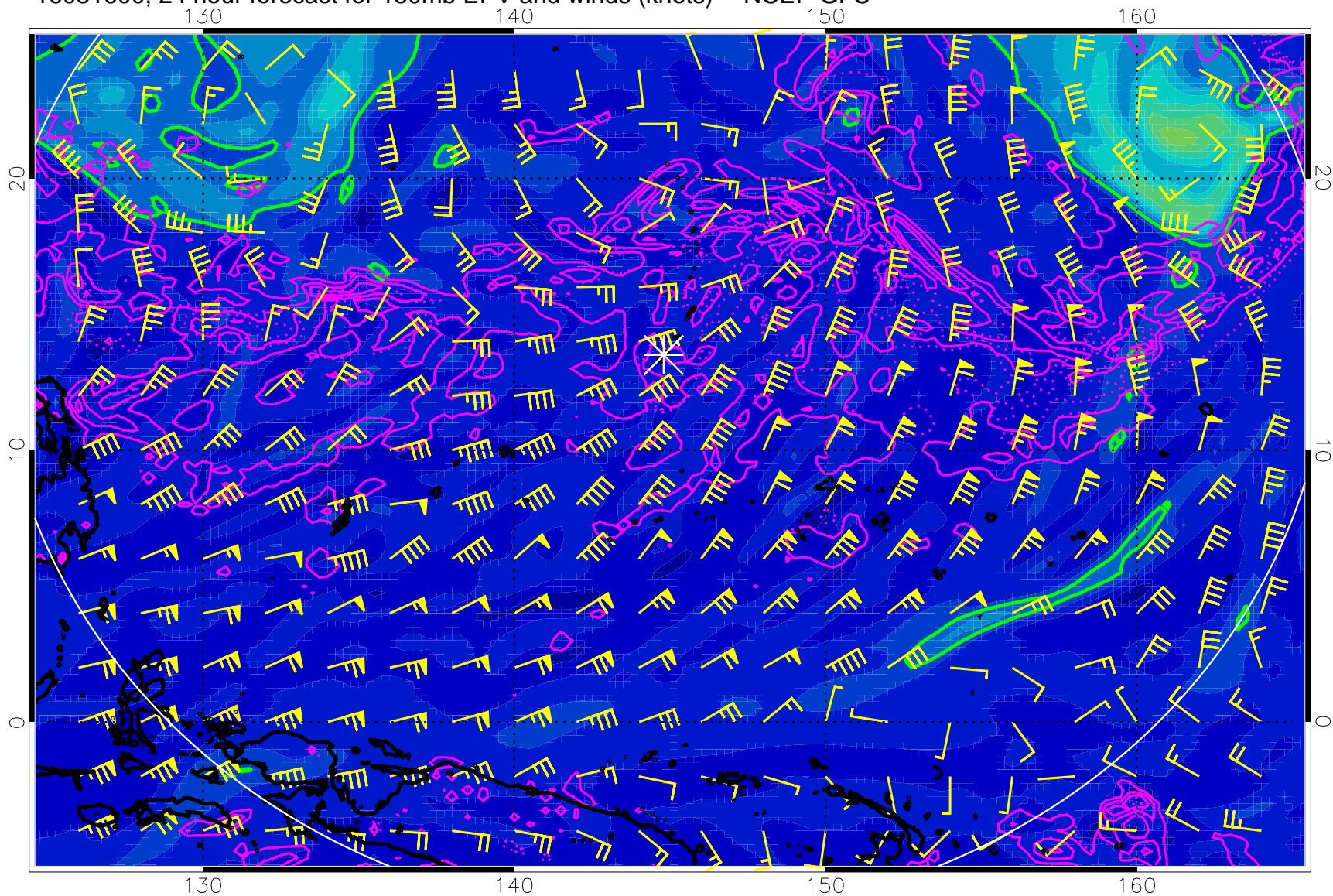
16081600, 24 hour forecast for 150mb EPV and winds (knots) -- NCEP GFS
