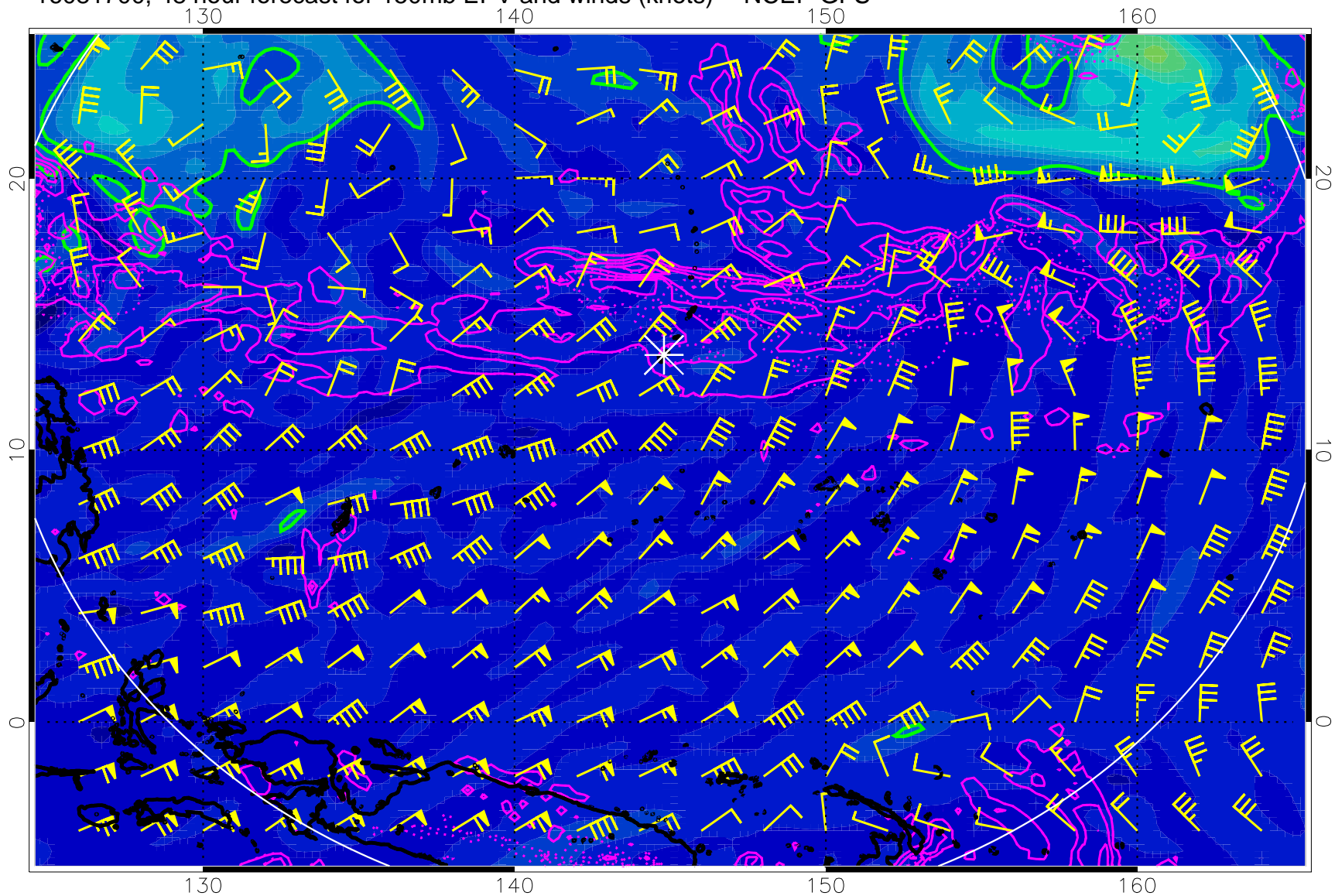
16081700, 48 hour forecast for 150mb EPV and winds (knots) -- NCEP GFS
