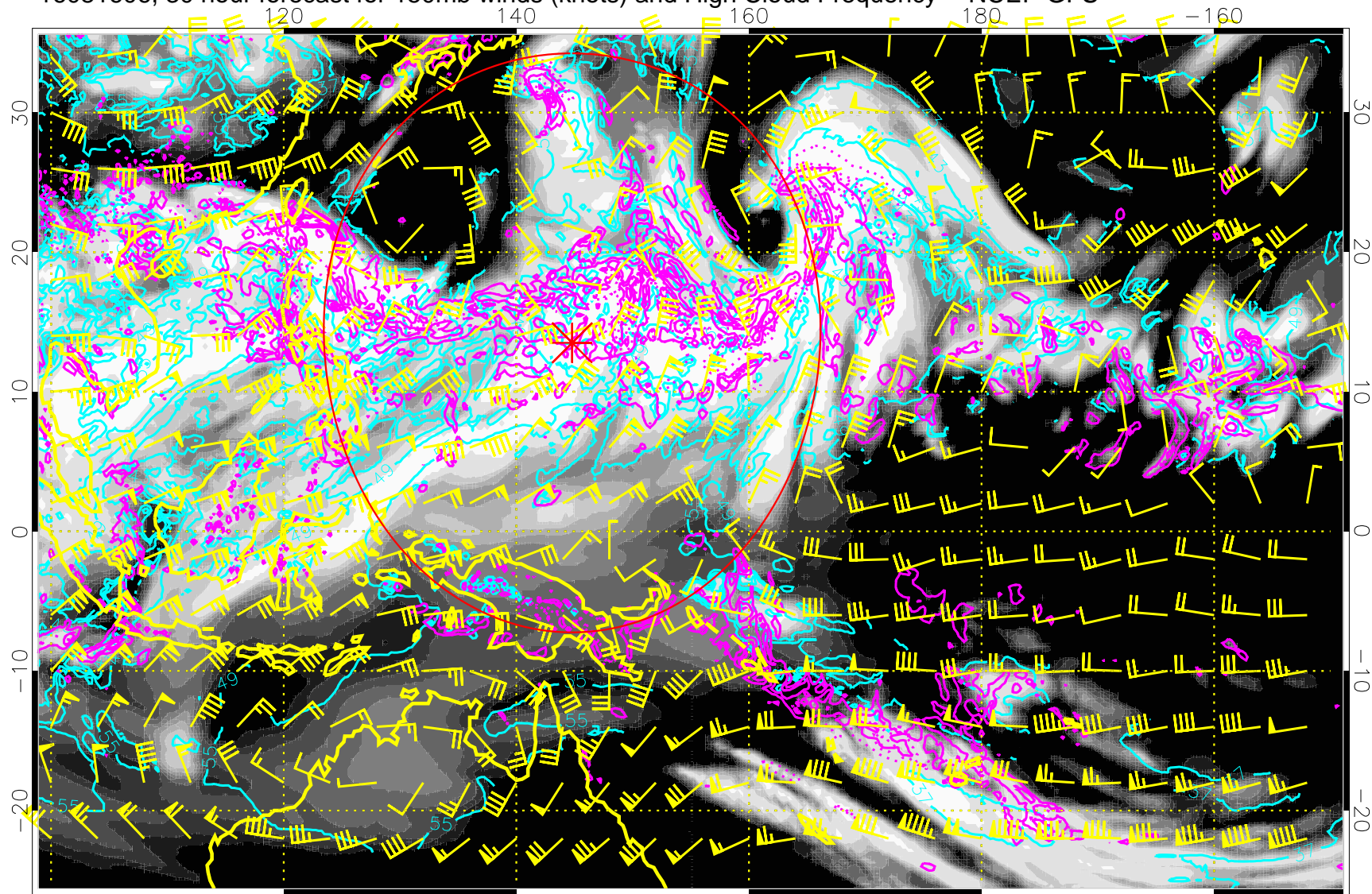
16081606, 30 hour forecast for 150mb winds (knots) and High Cloud Frequency -- NCEP GFS
