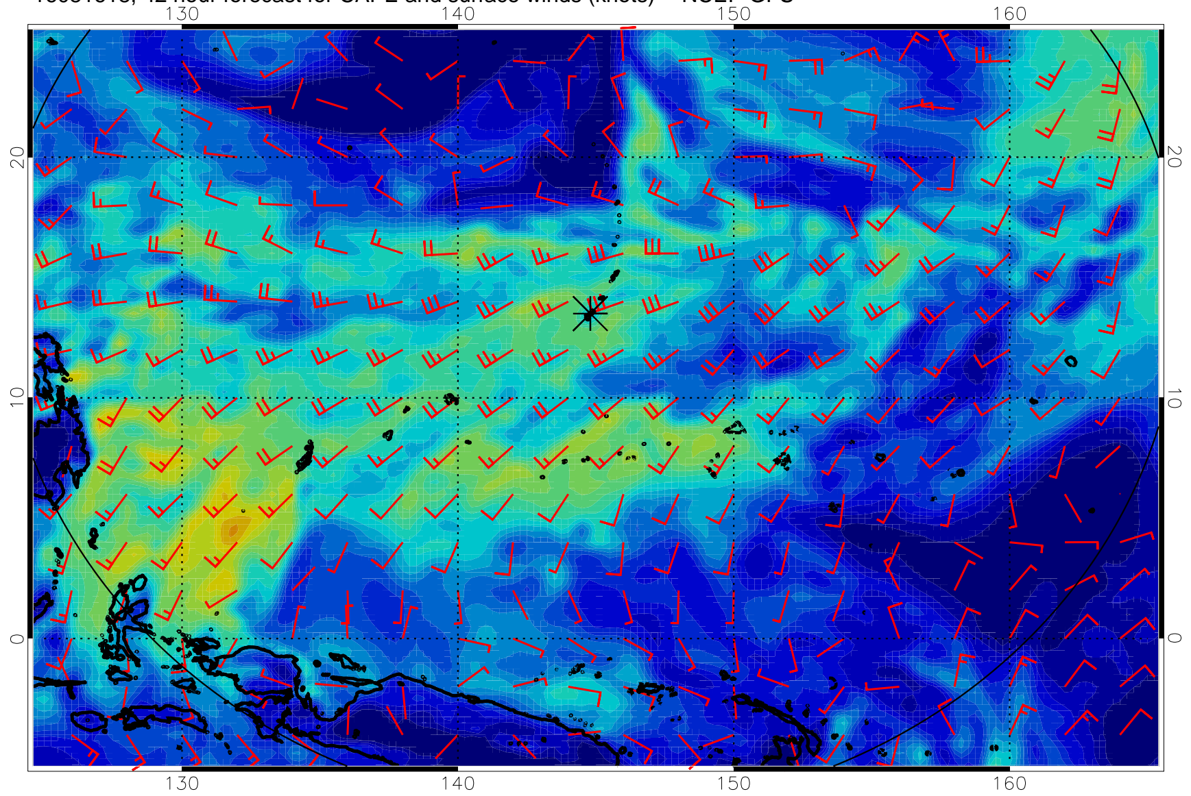
16081618, 42 hour forecast for CAPE and surface winds (knots) -- NCEP GFS
