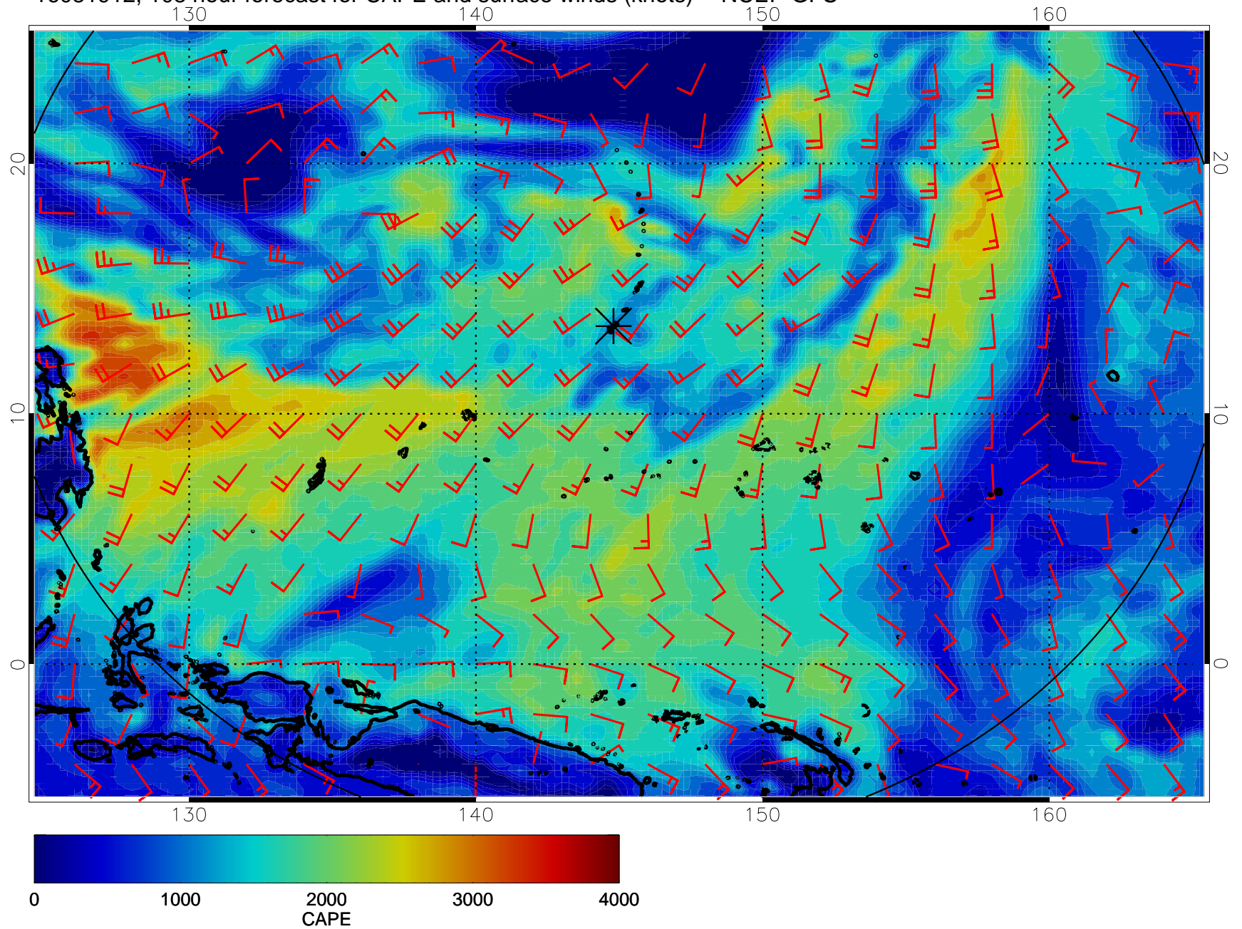
16081912, 108 hour forecast for CAPE and surface winds (knots) -- NCEP GFS
