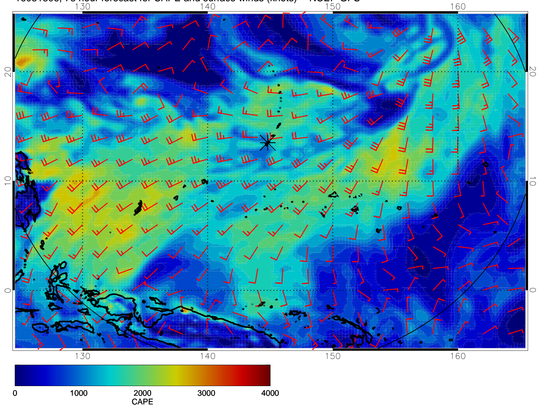
16081806, 78 hour forecast for CAPE and surface winds (knots) -- NCEP GFS
