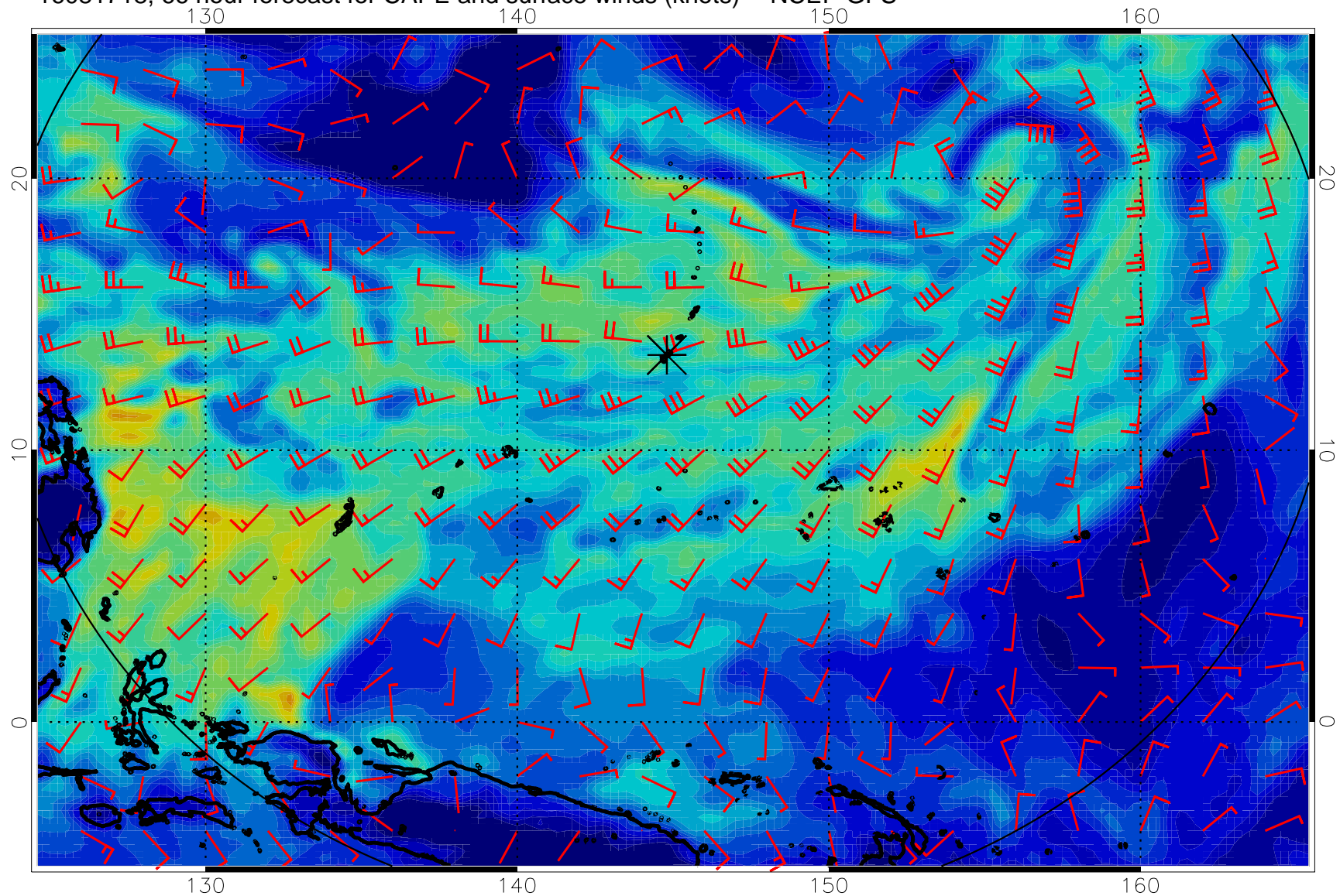
16081718, 66 hour forecast for CAPE and surface winds (knots) -- NCEP GFS
