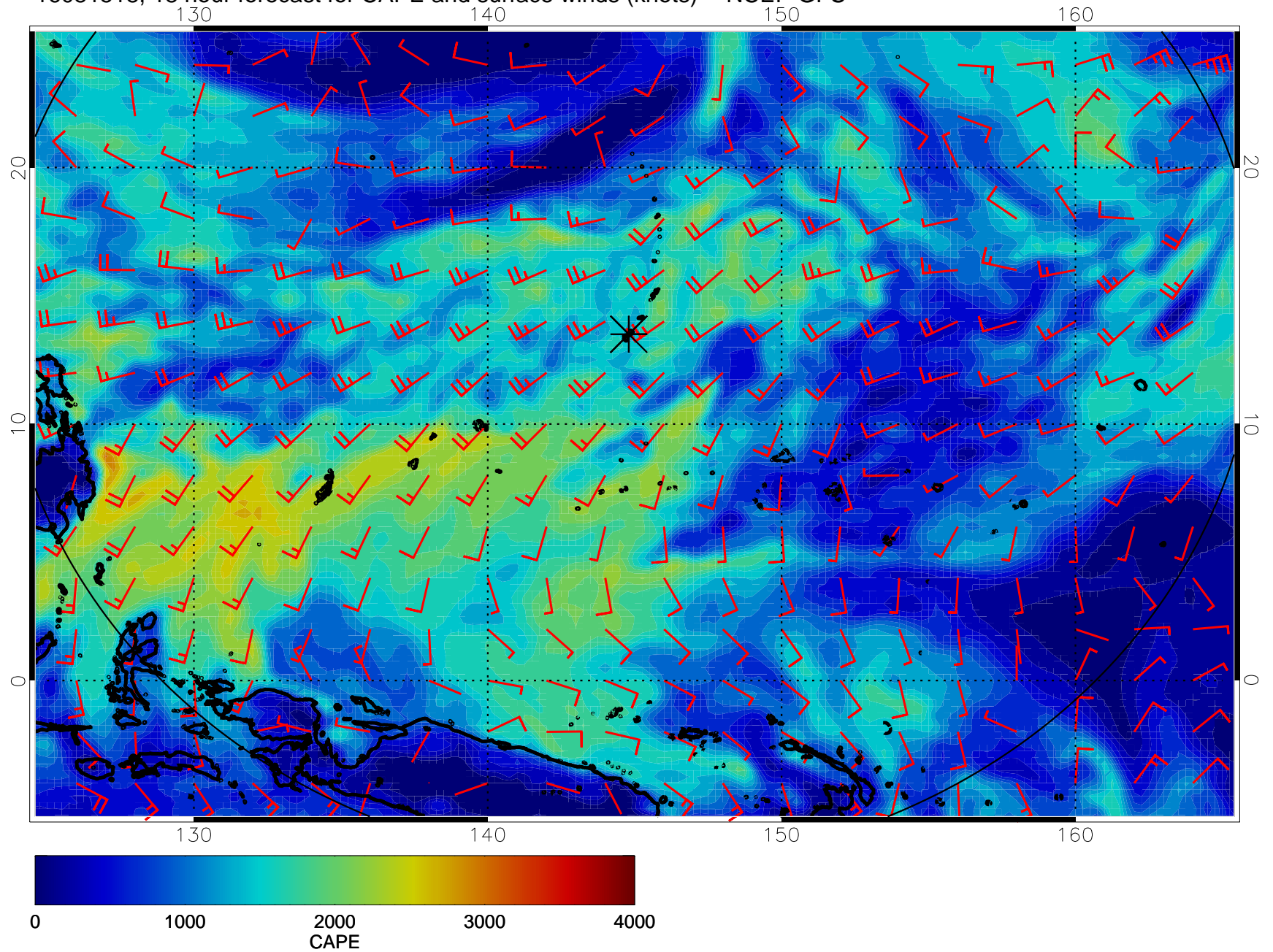
16081518, 18 hour forecast for CAPE and surface winds (knots) -- NCEP GFS
