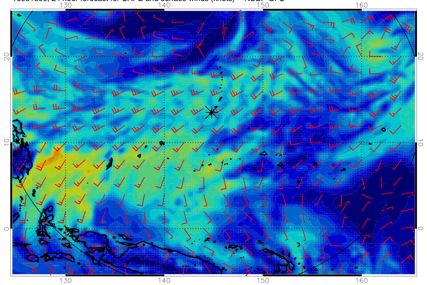
16081600, 24 hour forecast for CAPE and surface winds (knots) -- NCEP GFS
