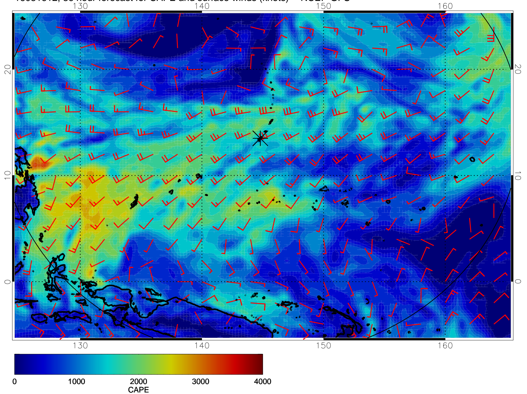
16081612, 36 hour forecast for CAPE and surface winds (knots) -- NCEP GFS
