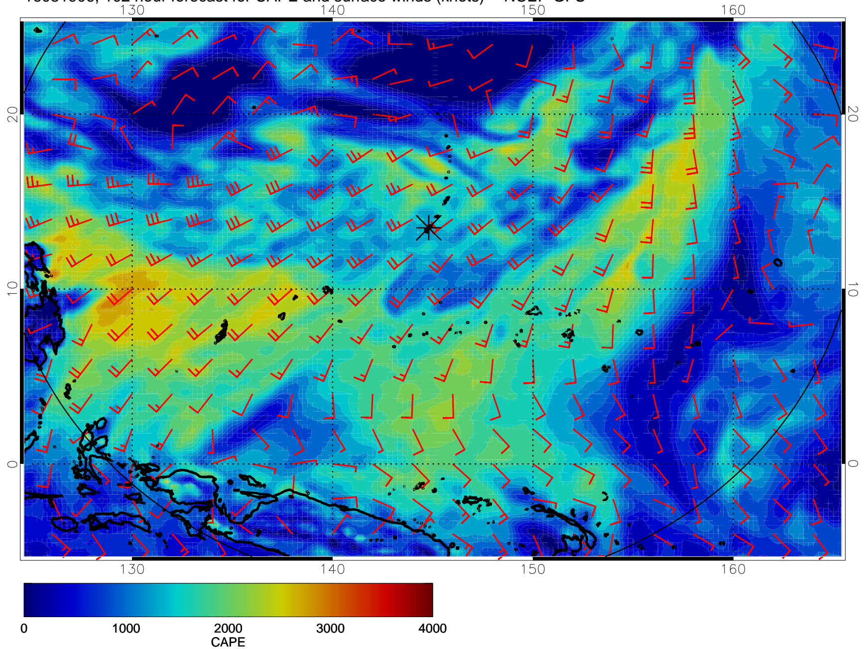
16081906, 102 hour forecast for CAPE and surface winds (knots) -- NCEP GFS
