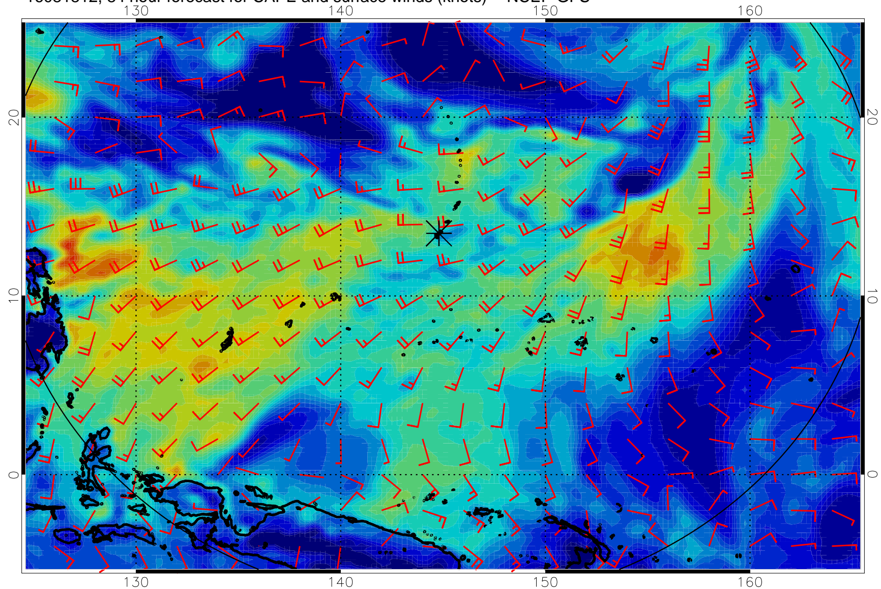
16081812, 84 hour forecast for CAPE and surface winds (knots) -- NCEP GFS
