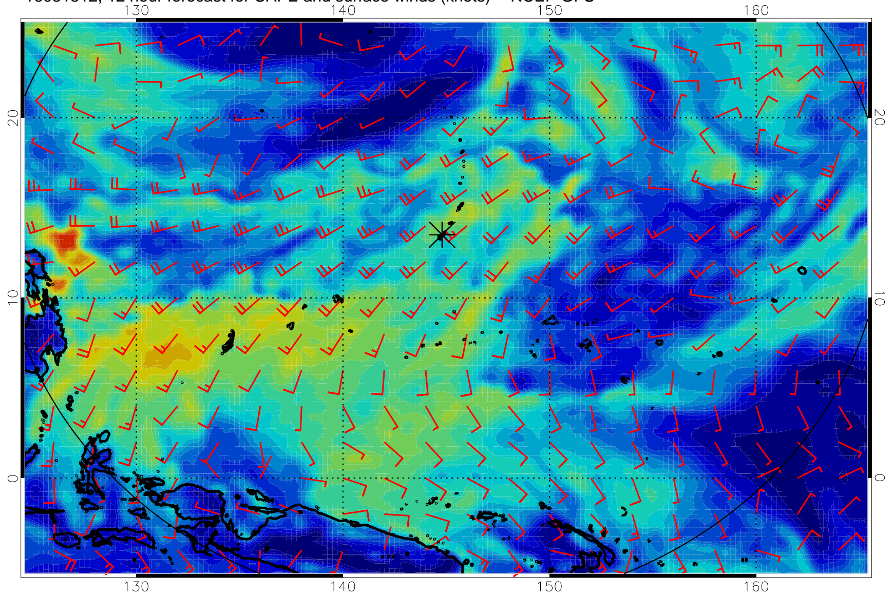
16081512, 12 hour forecast for CAPE and surface winds (knots) -- NCEP GFS
