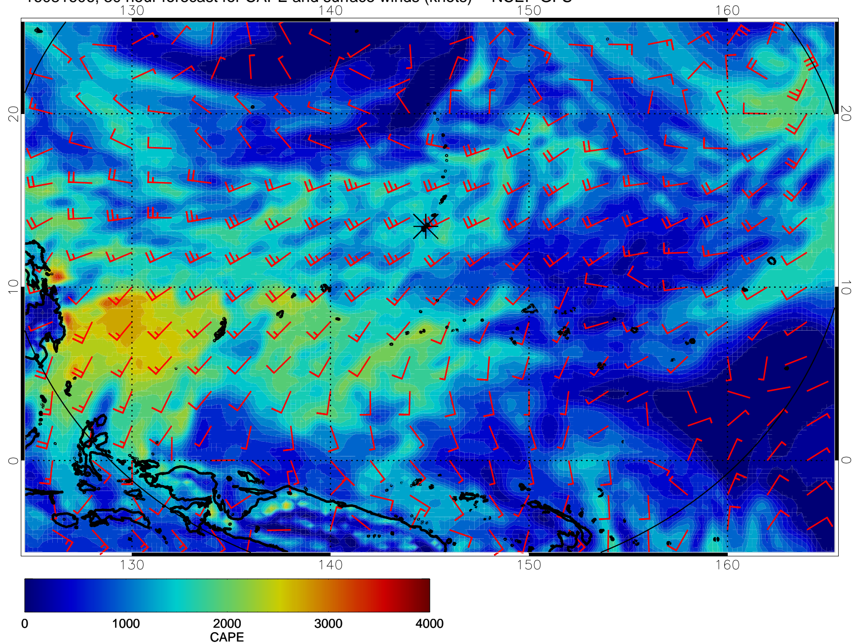
16081606, 30 hour forecast for CAPE and surface winds (knots) -- NCEP GFS
