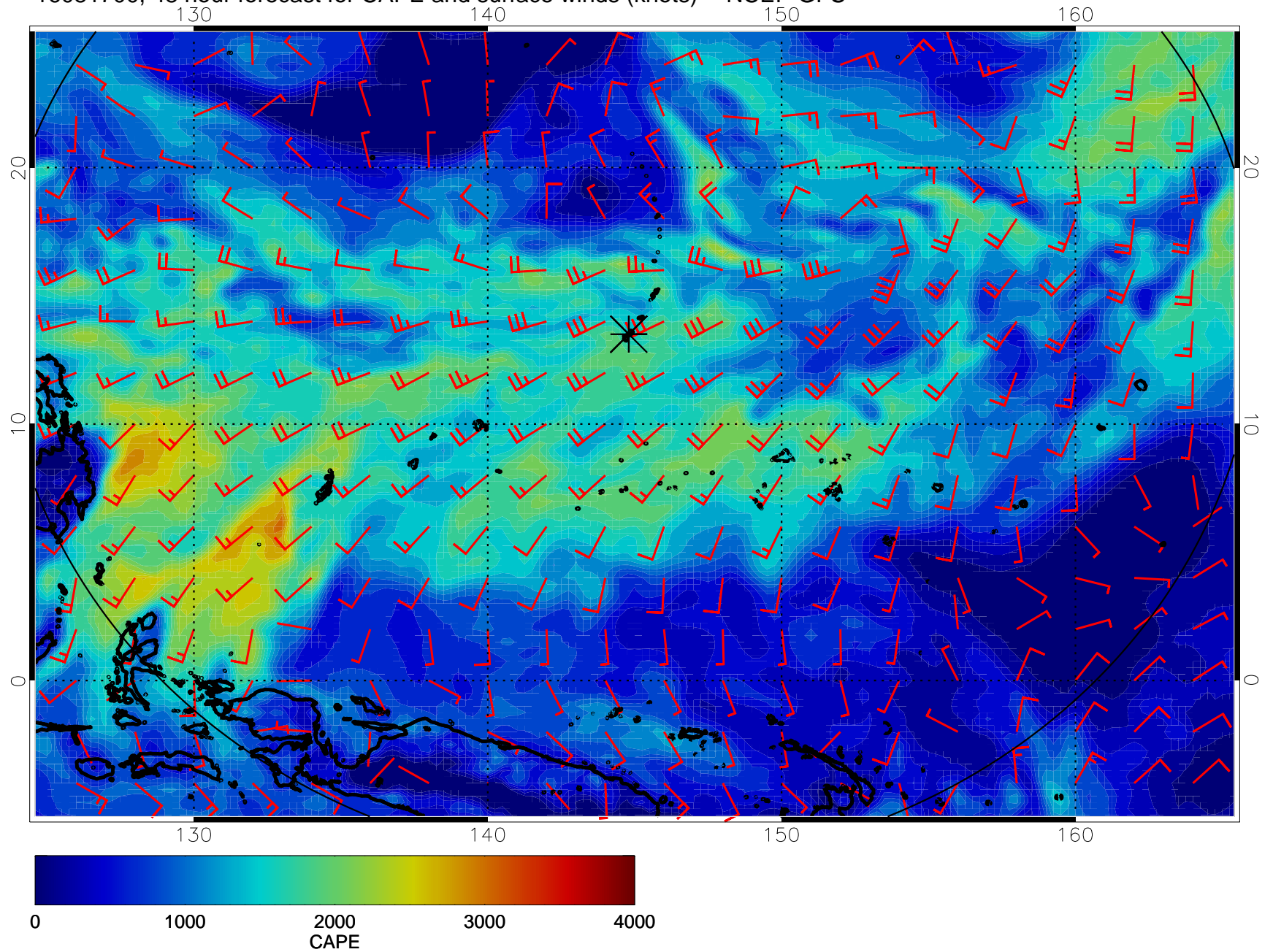
16081700, 48 hour forecast for CAPE and surface winds (knots) -- NCEP GFS
