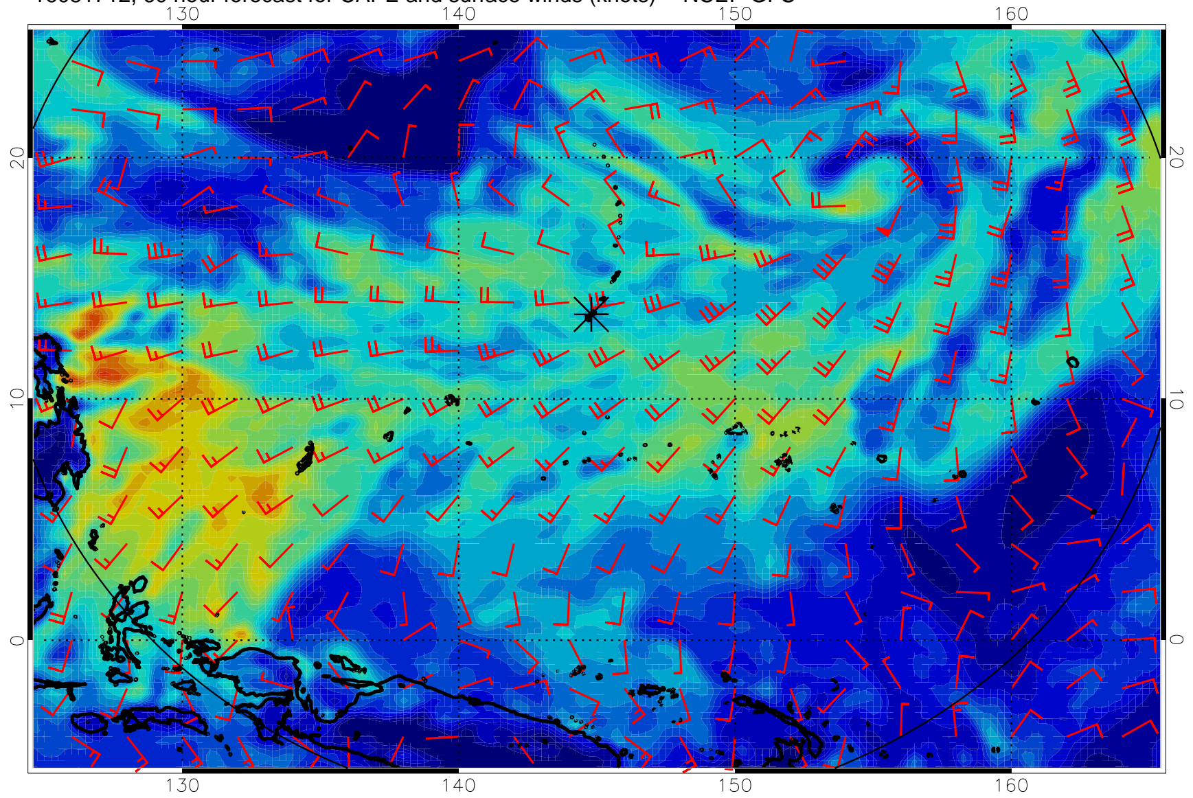
16081712, 60 hour forecast for CAPE and surface winds (knots) -- NCEP GFS
