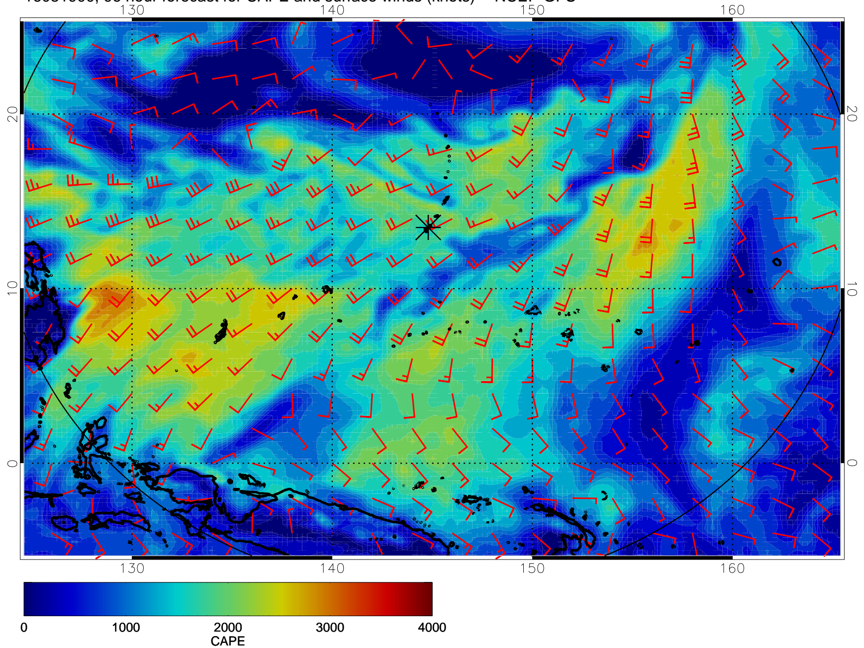
16081900, 96 hour forecast for CAPE and surface winds (knots) -- NCEP GFS
