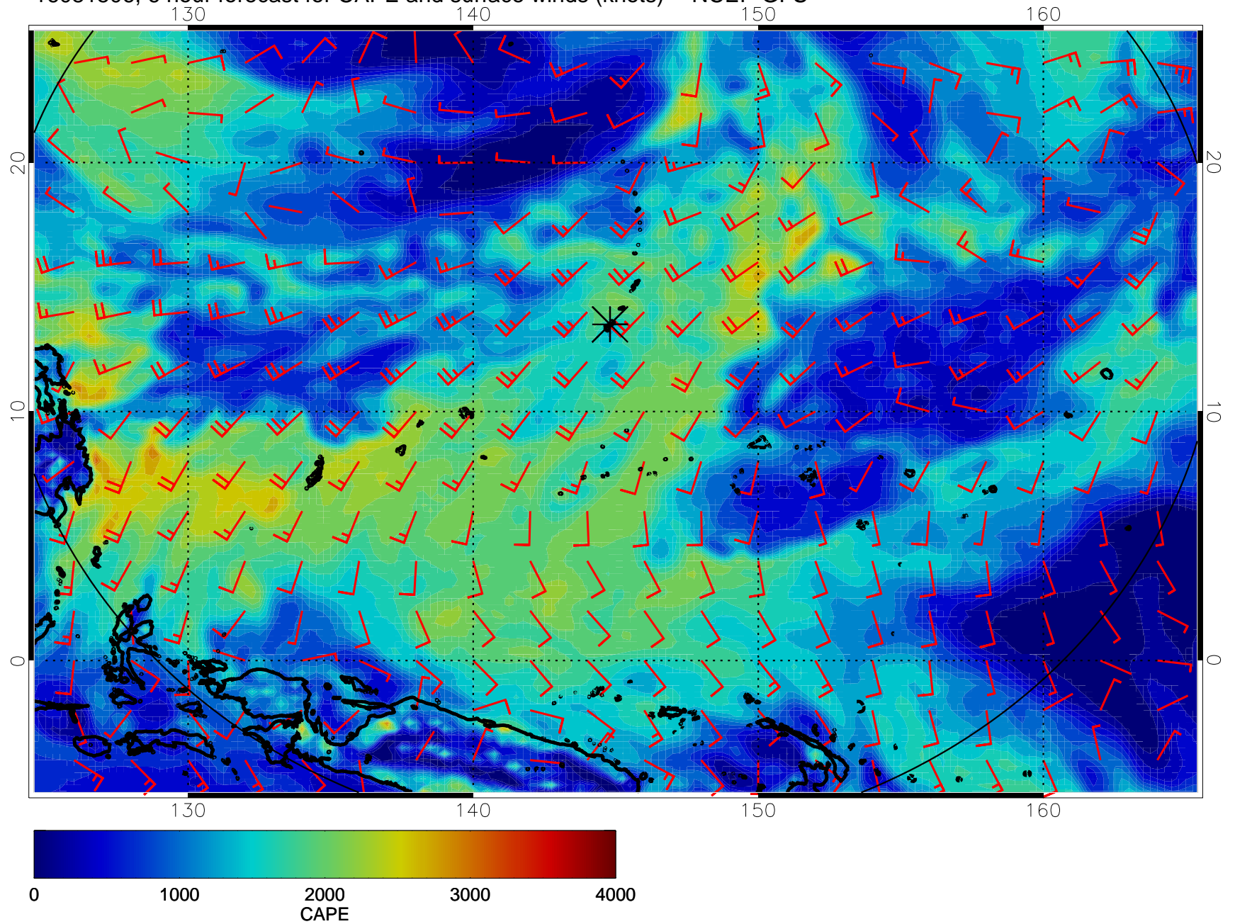
16081506, 6 hour forecast for CAPE and surface winds (knots) -- NCEP GFS
