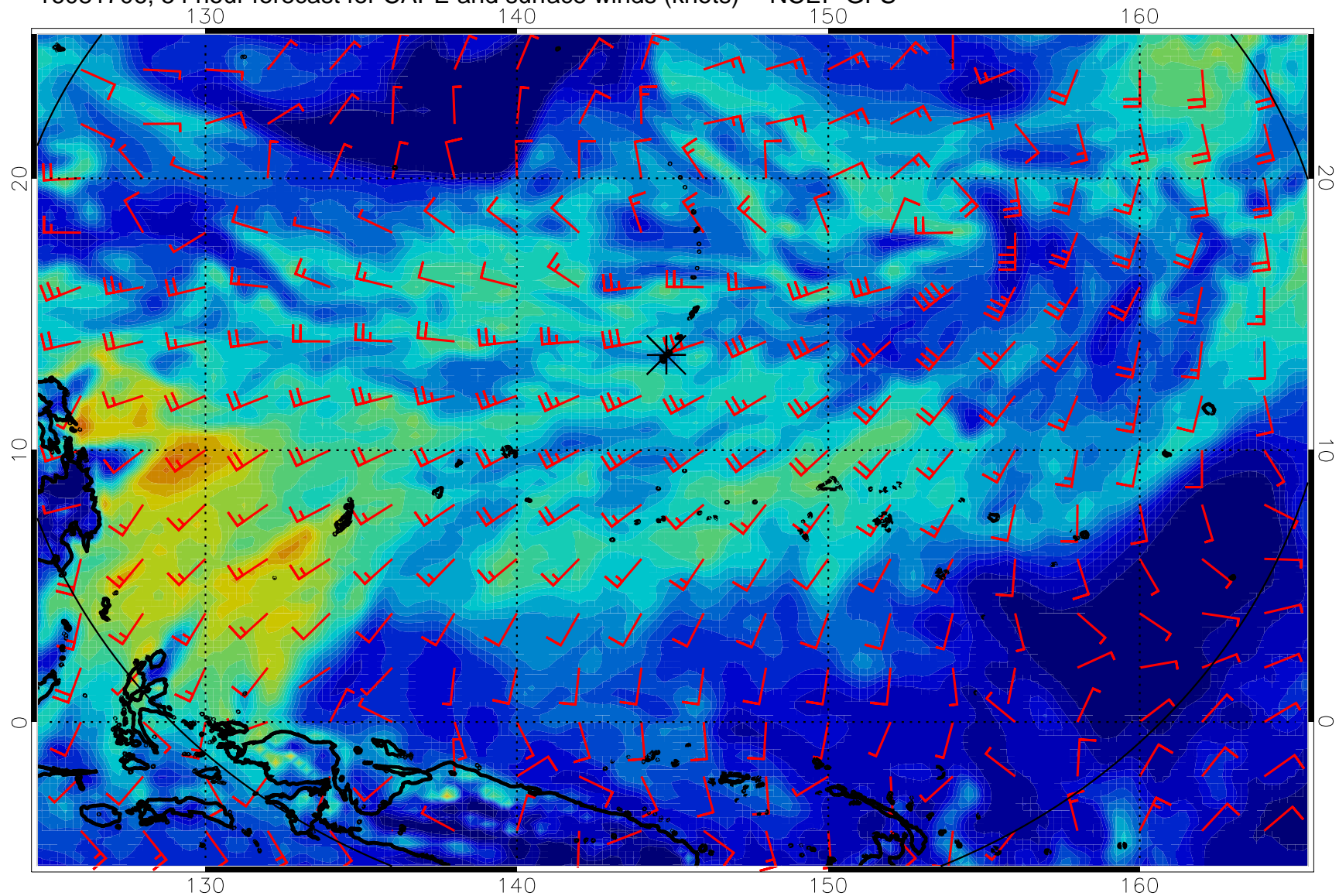
16081706, 54 hour forecast for CAPE and surface winds (knots) -- NCEP GFS
