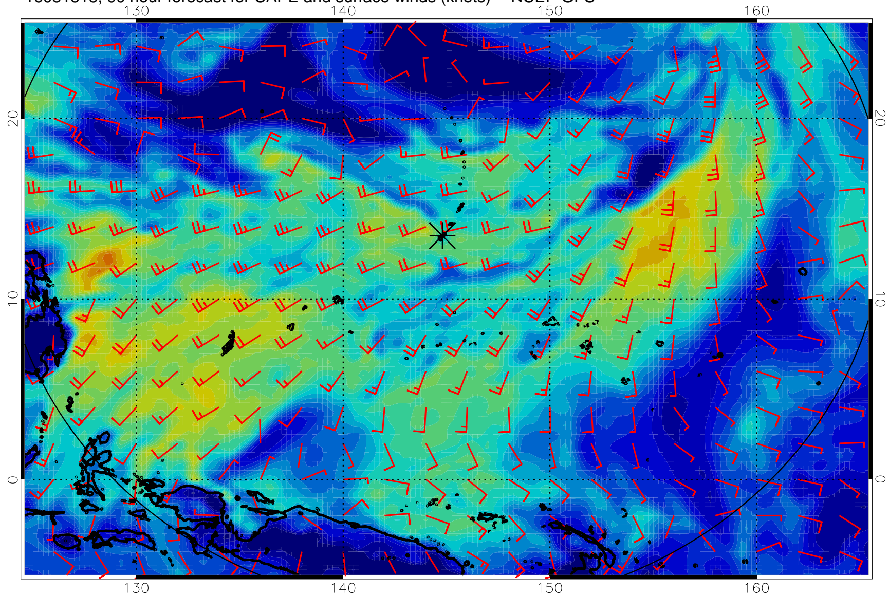
16081818, 90 hour forecast for CAPE and surface winds (knots) -- NCEP GFS
