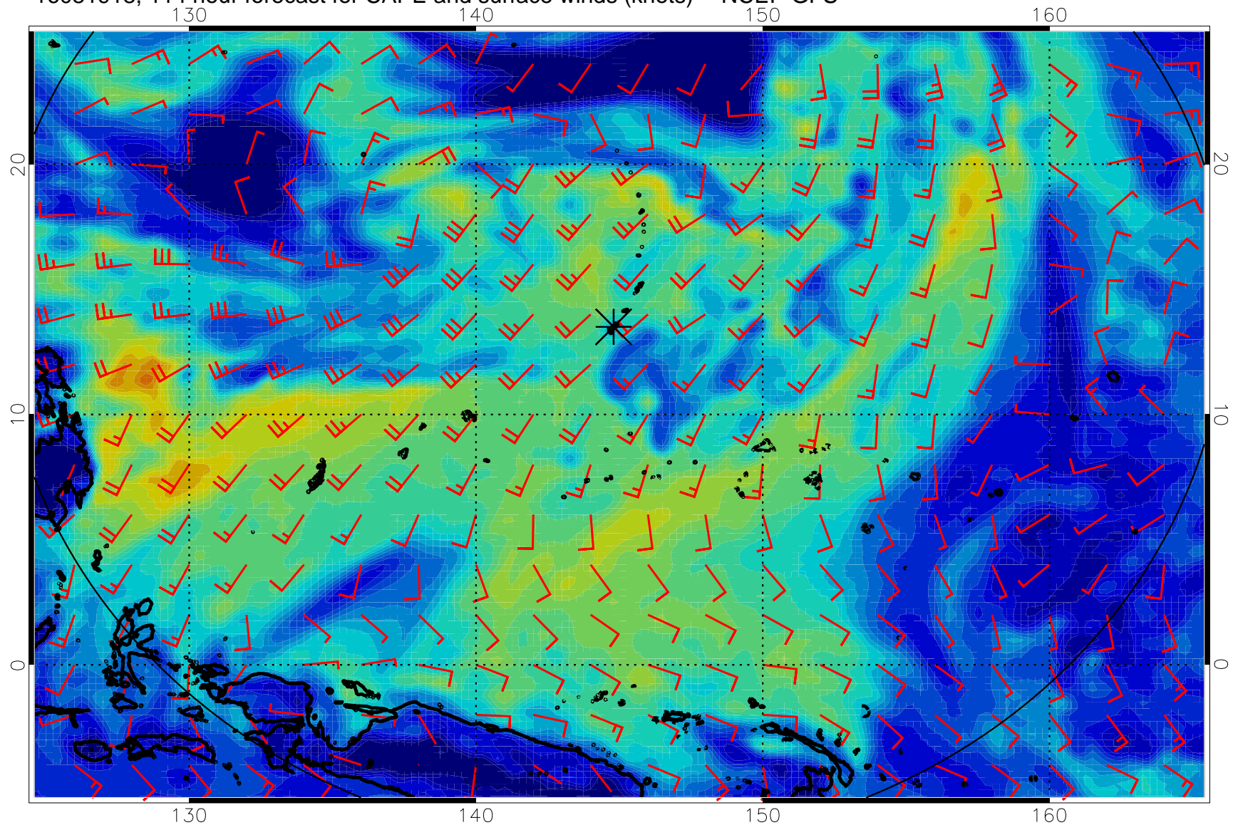
16081918, 114 hour forecast for CAPE and surface winds (knots) -- NCEP GFS
