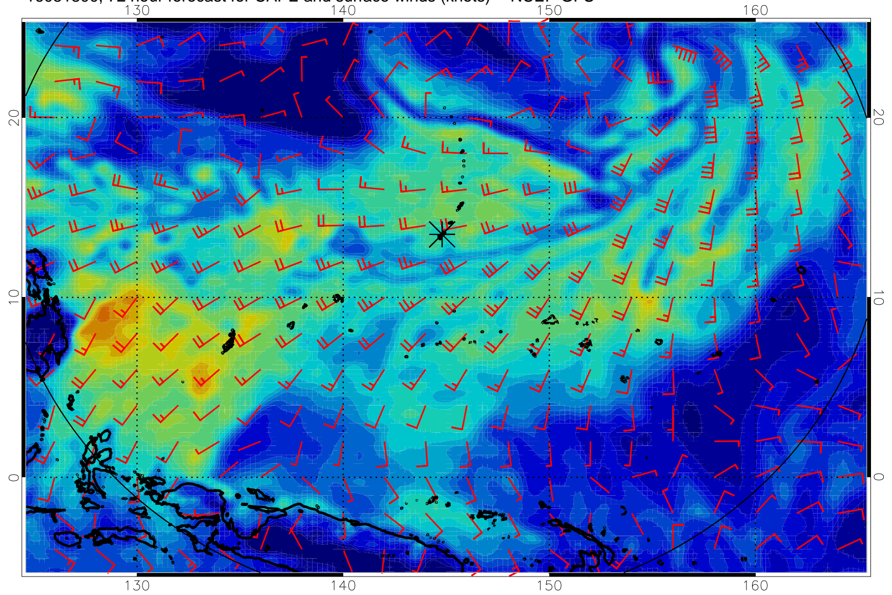
16081800, 72 hour forecast for CAPE and surface winds (knots) -- NCEP GFS
