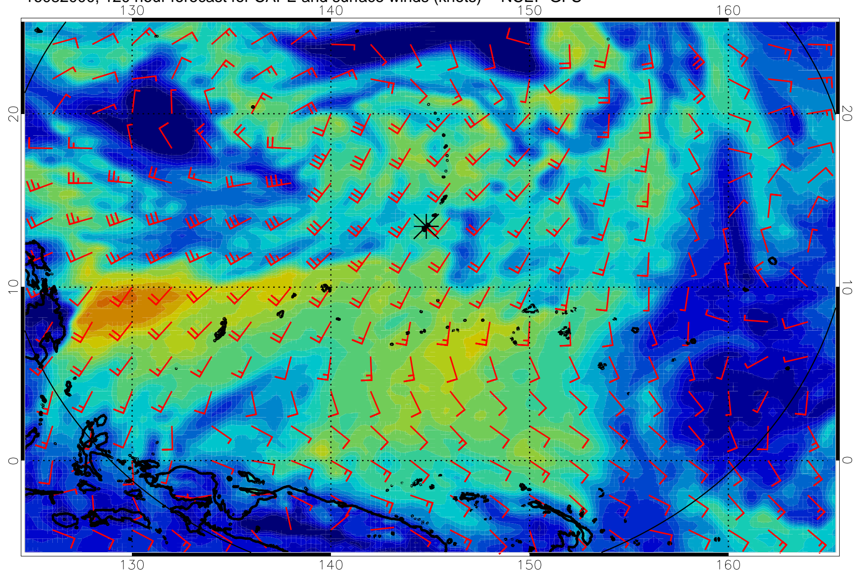
16082000, 120 hour forecast for CAPE and surface winds (knots) -- NCEP GFS
