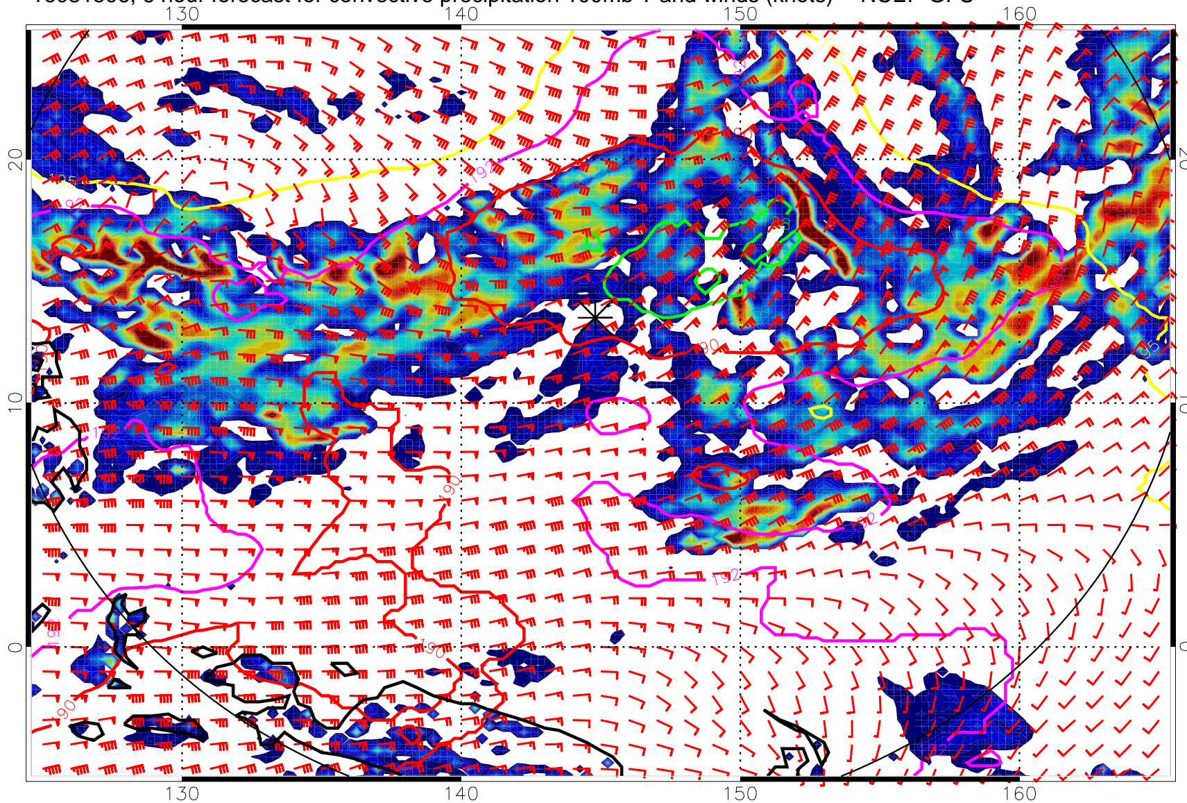
16081506, 6 hour forecast for convective precipitation 100mb T and winds (knots) -- NCEP GFS
