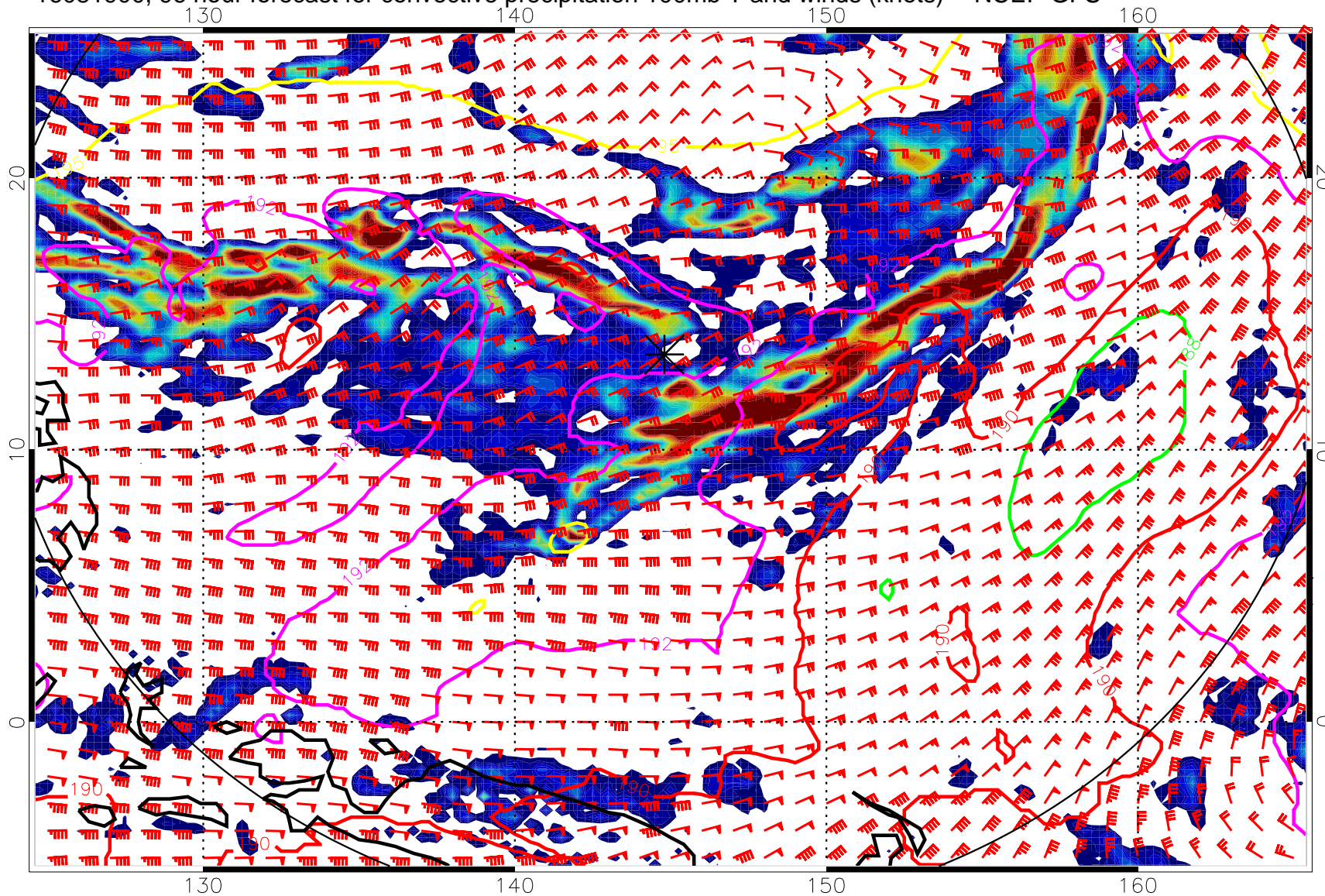
16081900, 96 hour forecast for convective precipitation 100mb T and winds (knots) -- NCEP GFS
