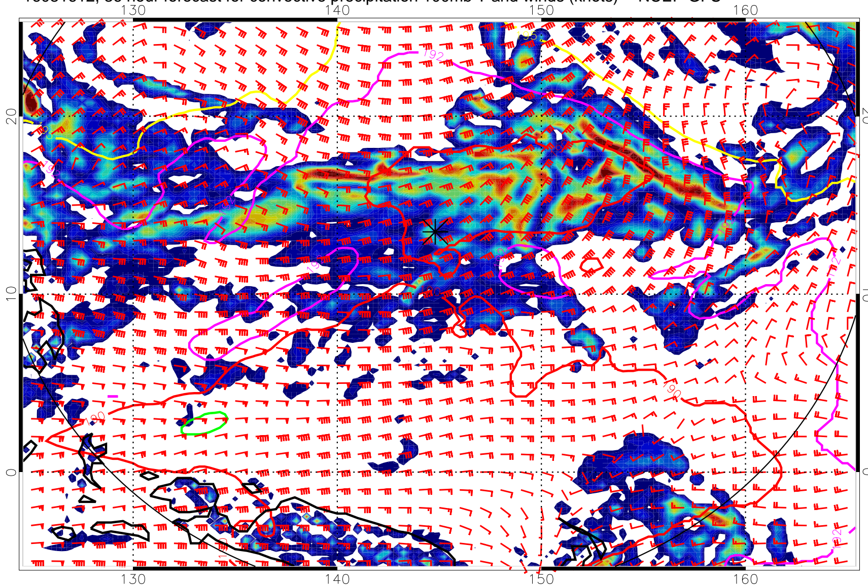
16081612, 36 hour forecast for convective precipitation 100mb T and winds (knots) -- NCEP GFS
