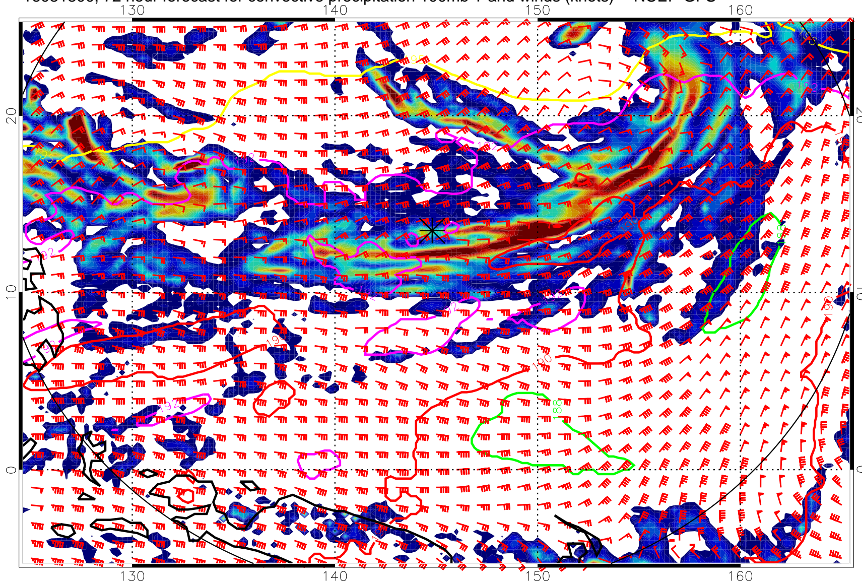
16081800, 72 hour forecast for convective precipitation 100mb T and winds (knots) -- NCEP GFS
