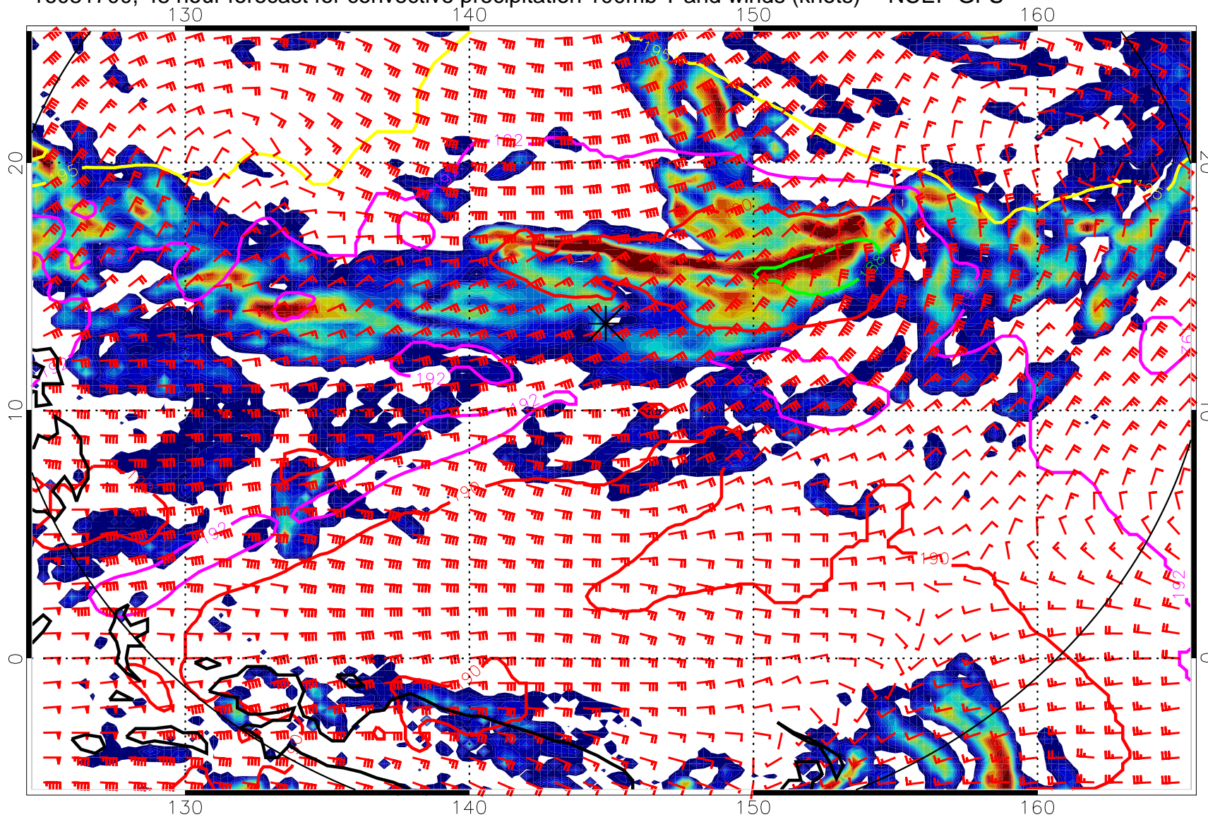
16081700, 48 hour forecast for convective precipitation 100mb T and winds (knots) -- NCEP GFS
