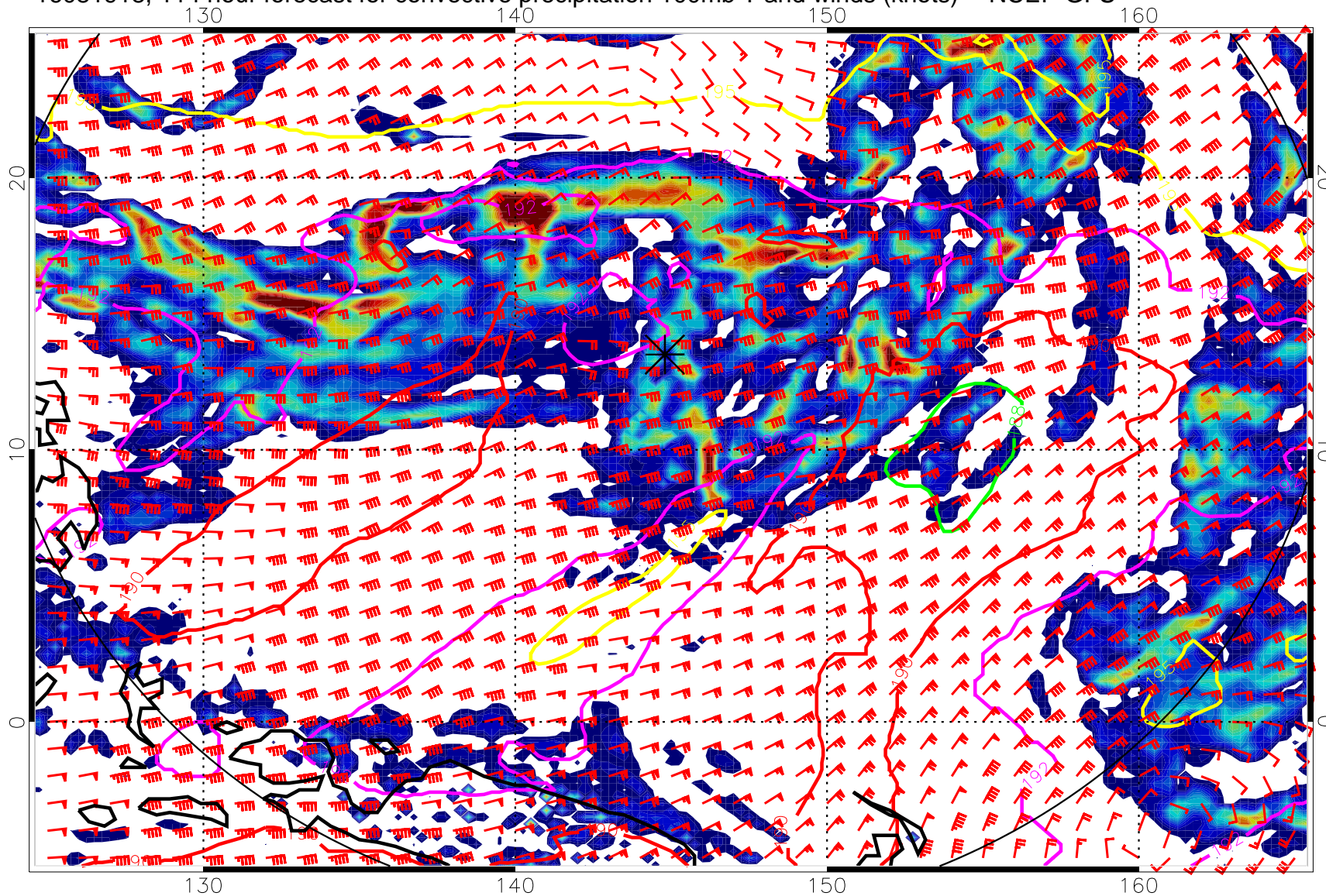
16081918, 114 hour forecast for convective precipitation 100mb T and winds (knots) -- NCEP GFS
