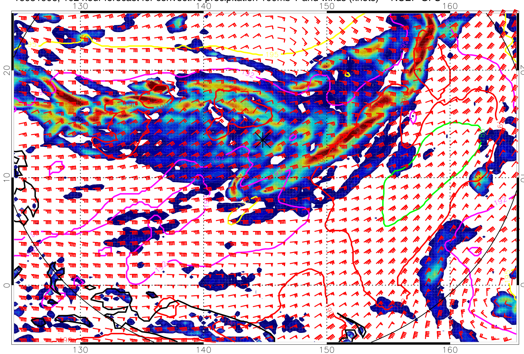
16081906, 102 hour forecast for convective precipitation 100mb T and winds (knots) -- NCEP GFS
