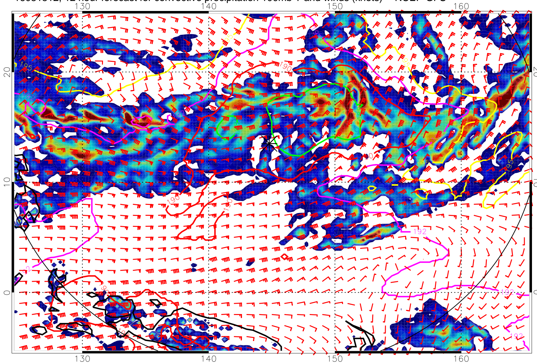
16081512, 12 hour forecast for convective precipitation 100mb T and winds (knots) -- NCEP GFS
