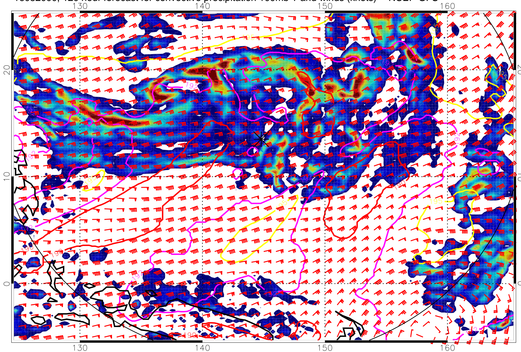
16082000, 120 hour forecast for convective precipitation 100mb T and winds (knots) -- NCEP GFS
