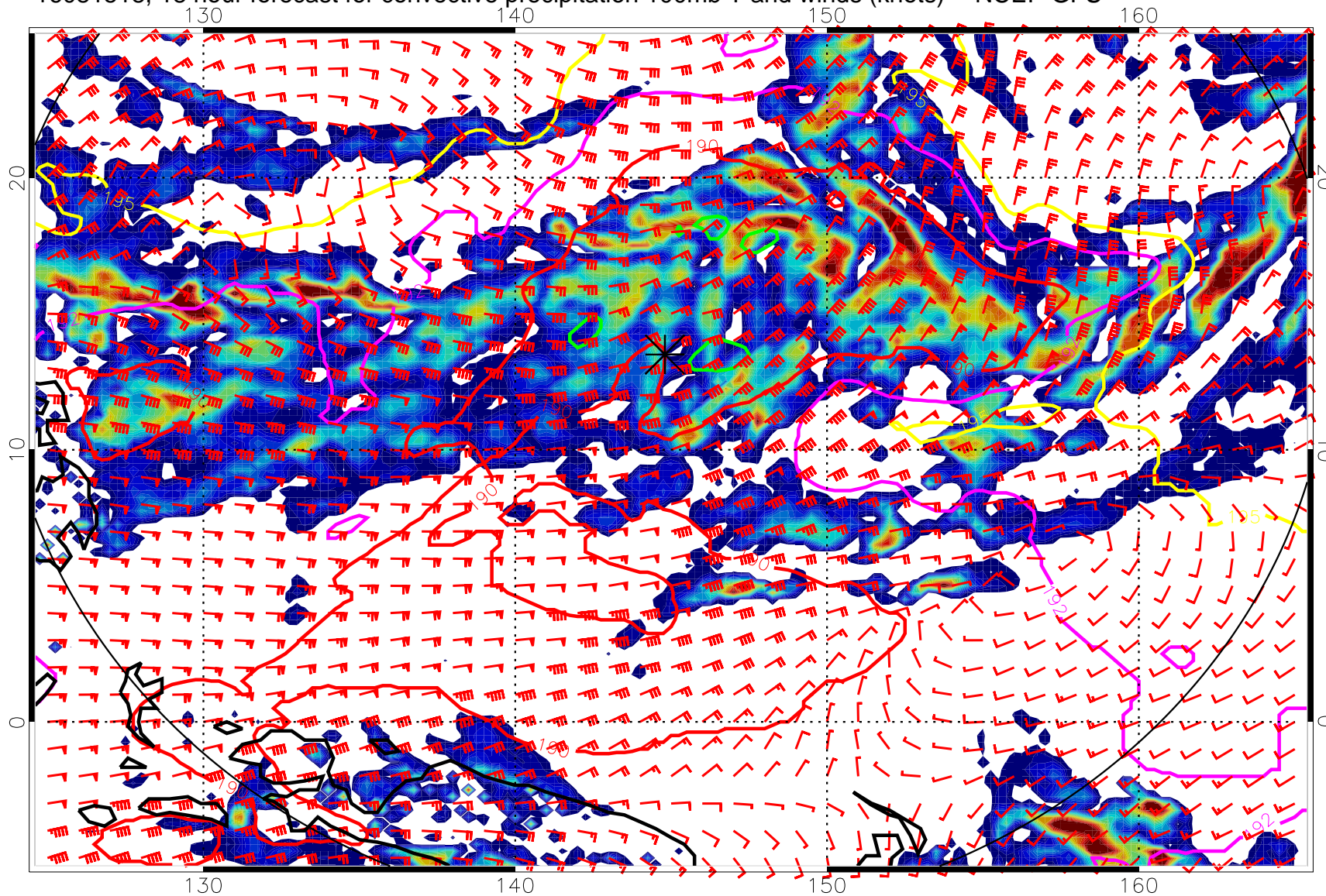
16081518, 18 hour forecast for convective precipitation 100mb T and winds (knots) -- NCEP GFS
