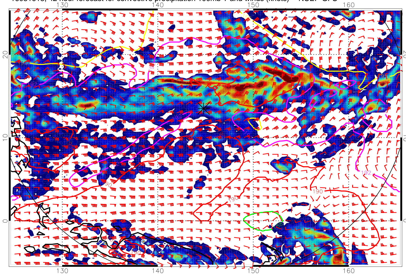
16081618, 42 hour forecast for convective precipitation 100mb T and winds (knots) -- NCEP GFS
