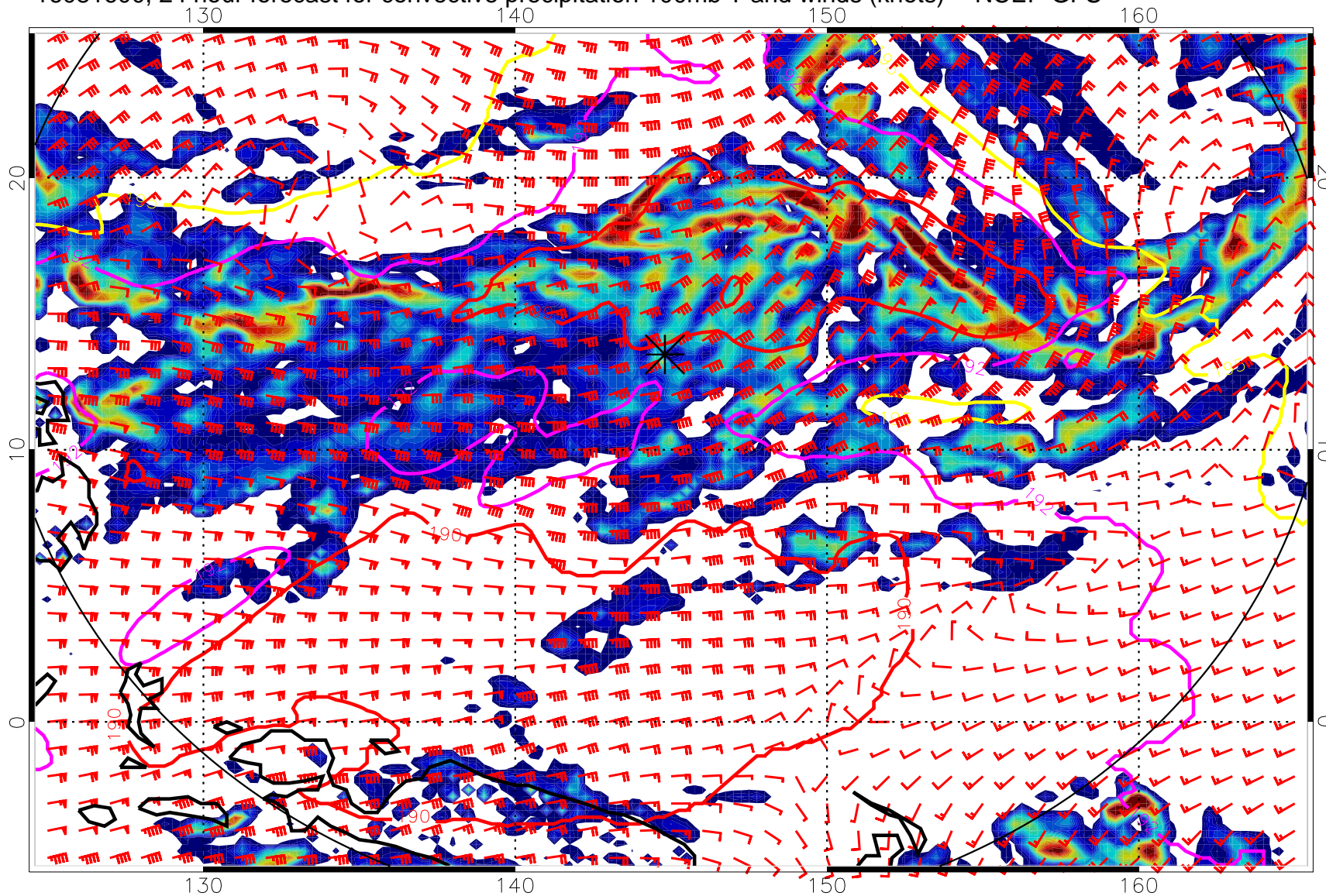
16081600, 24 hour forecast for convective precipitation 100mb T and winds (knots) -- NCEP GFS
