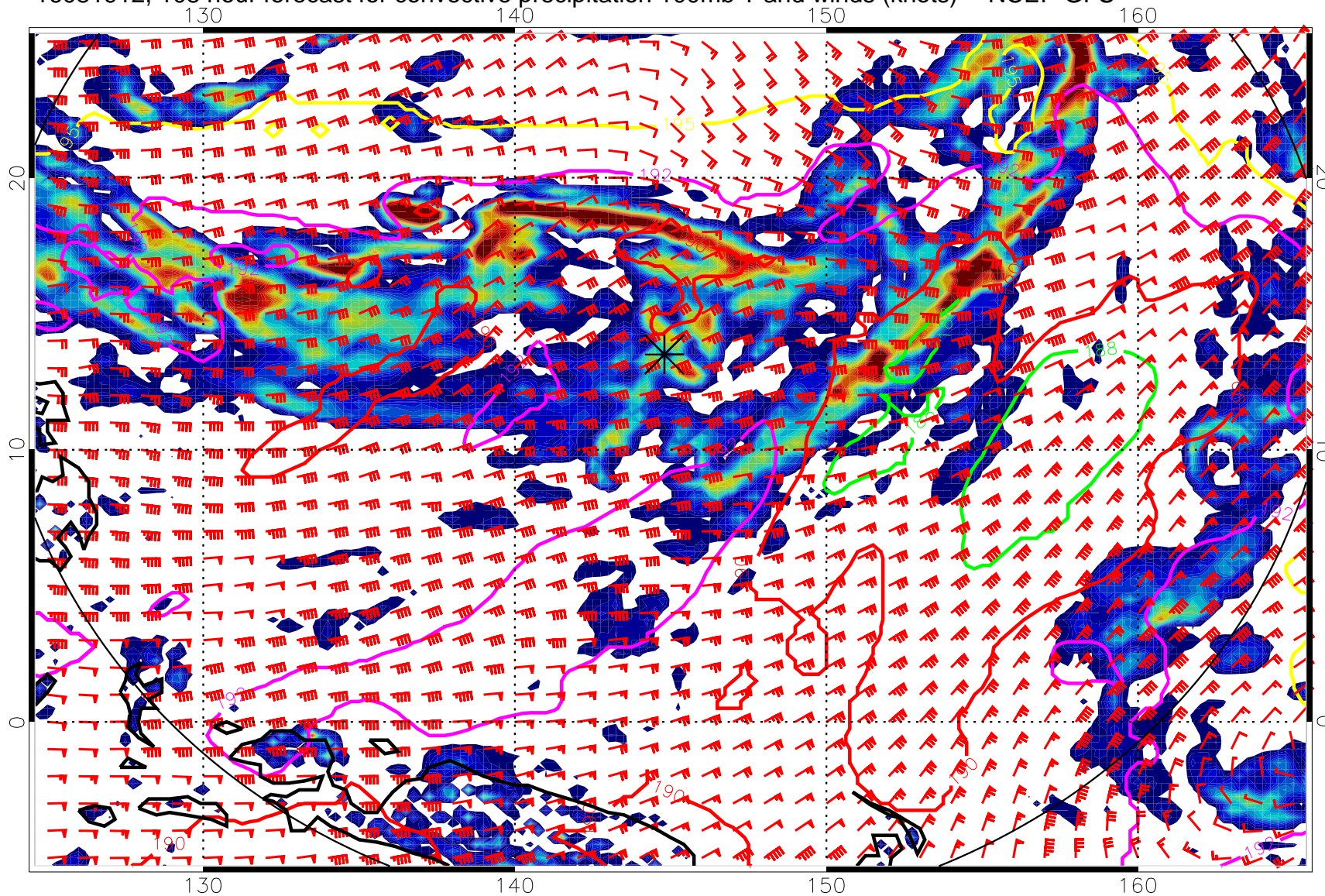
16081912, 108 hour forecast for convective precipitation 100mb T and winds (knots) -- NCEP GFS
