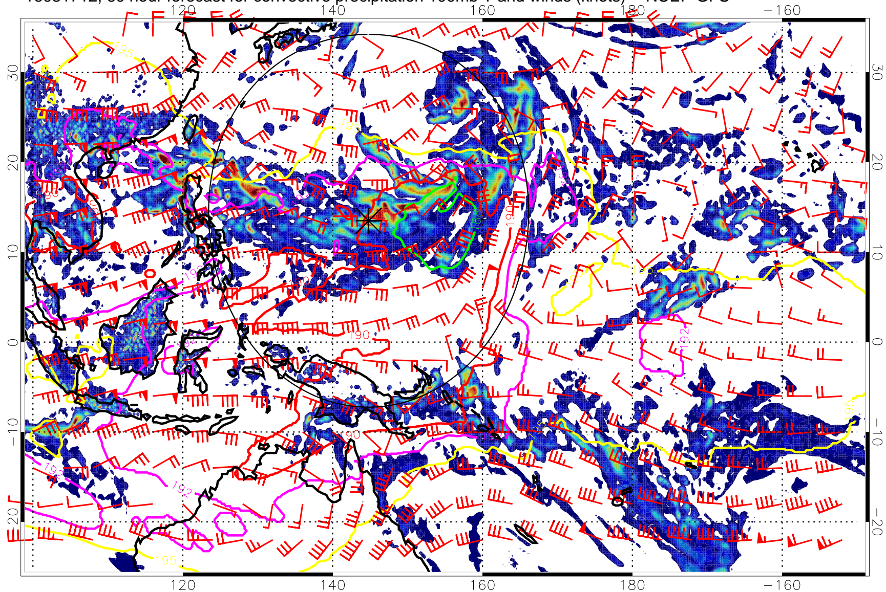
16081712, 60 hour forecast for convective precipitation 100mb T and winds (knots) -- NCEP GFS
