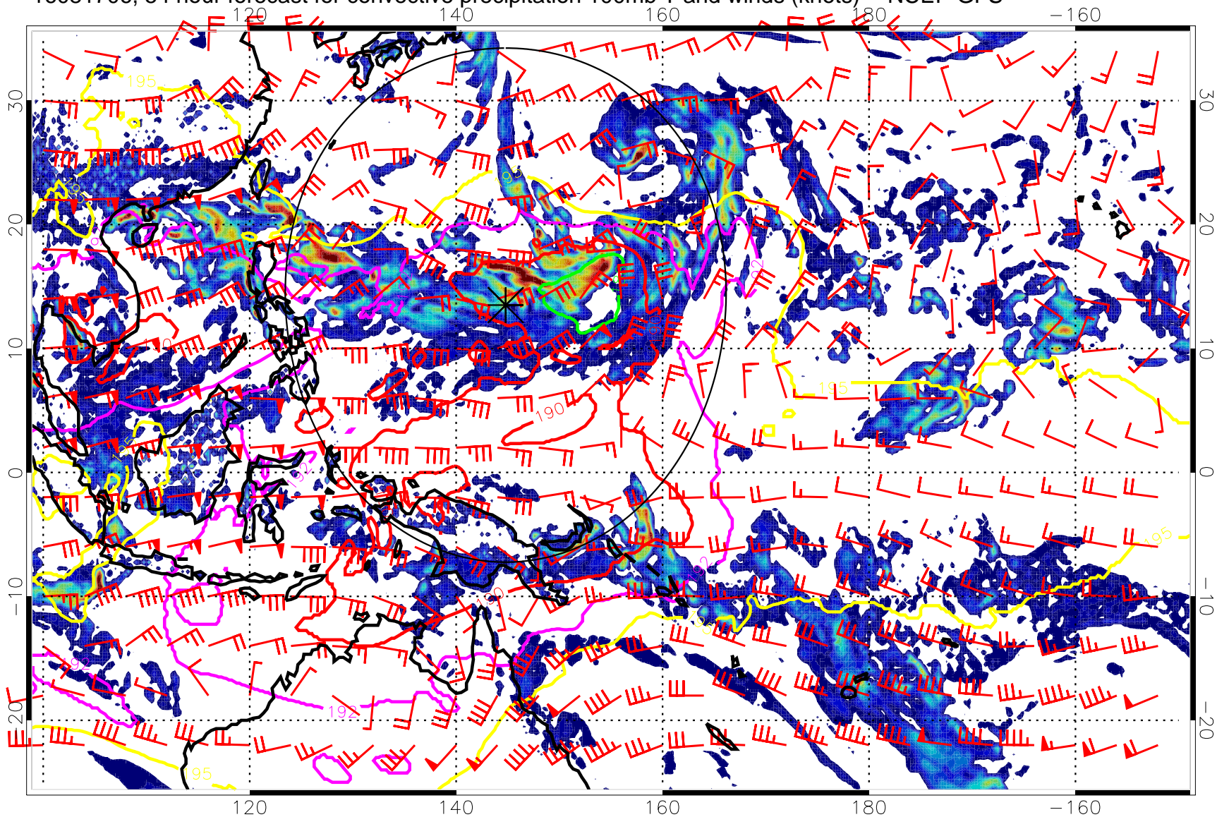
16081706, 54 hour forecast for convective precipitation 100mb T and winds (knots) -- NCEP GFS
