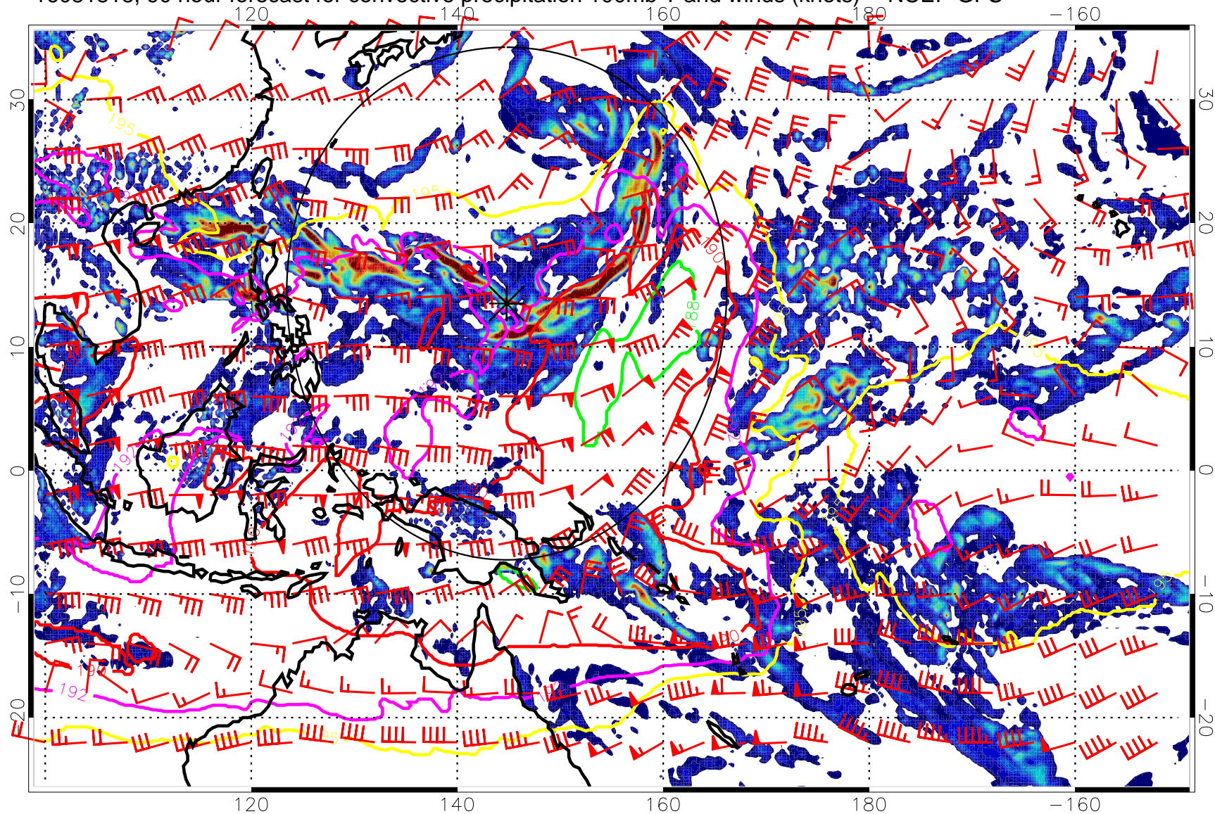
16081818, 90 hour forecast for convective precipitation 100mb T and winds (knots) -- NCEP GFS
