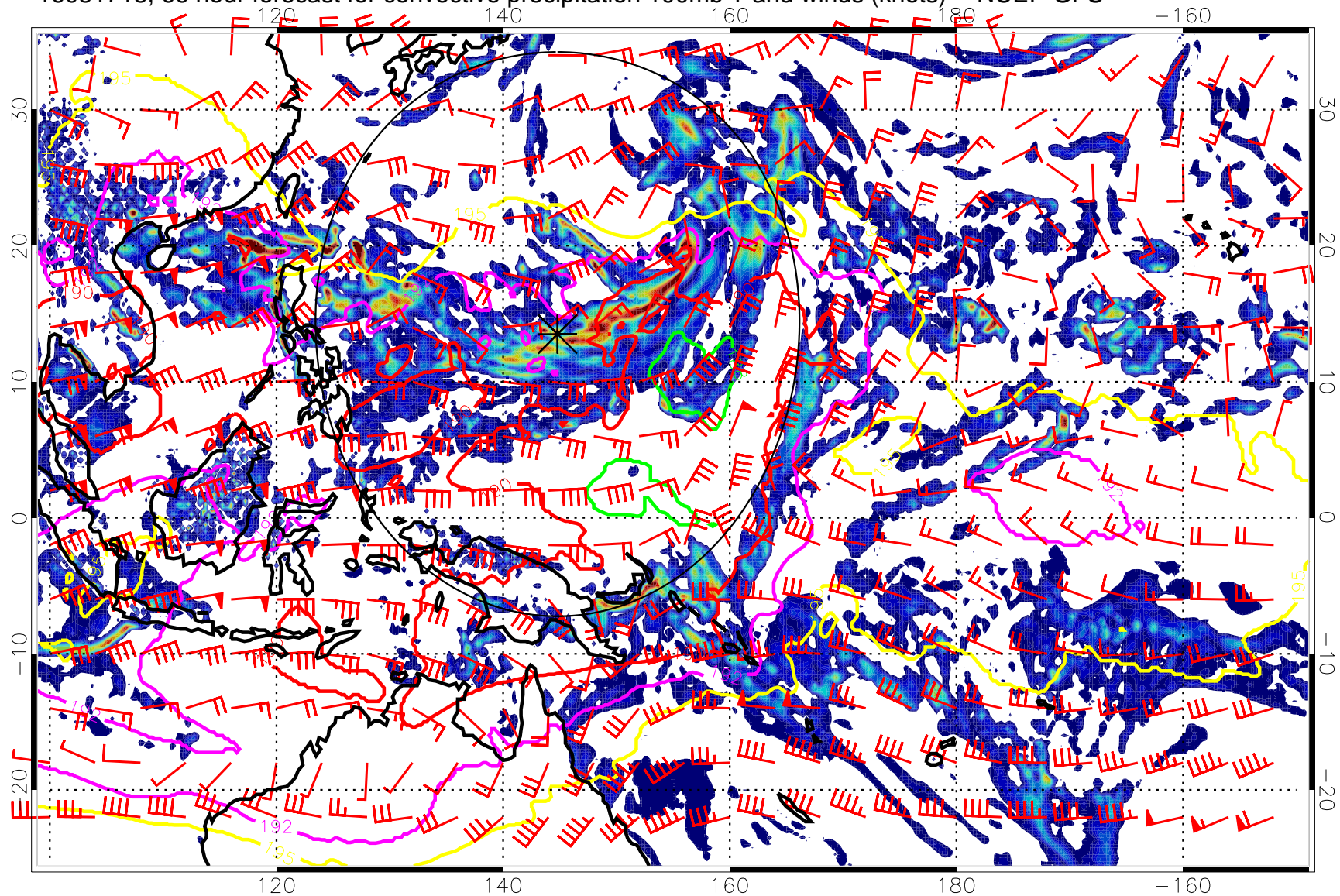
16081718, 66 hour forecast for convective precipitation 100mb T and winds (knots) -- NCEP GFS
