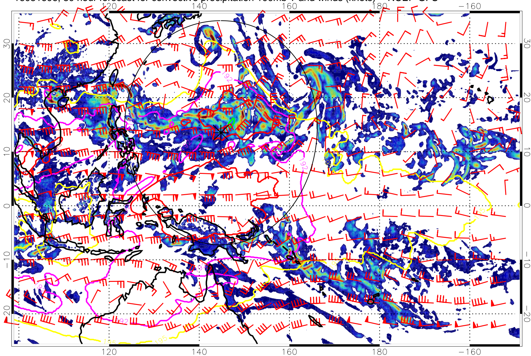
16081606, 30 hour forecast for convective precipitation 100mb T and winds (knots) -- NCEP GFS
