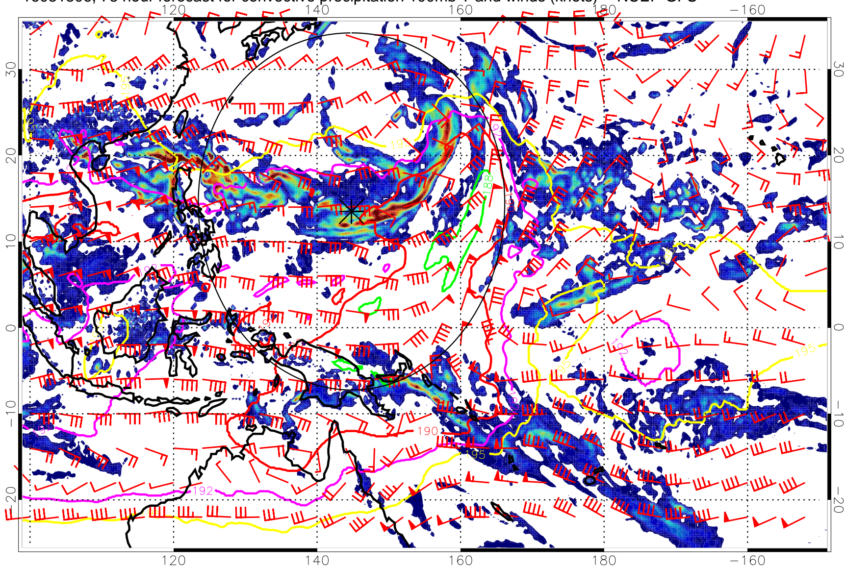
16081806, 78 hour forecast for convective precipitation 100mb T and winds (knots) -- NCEP GFS
