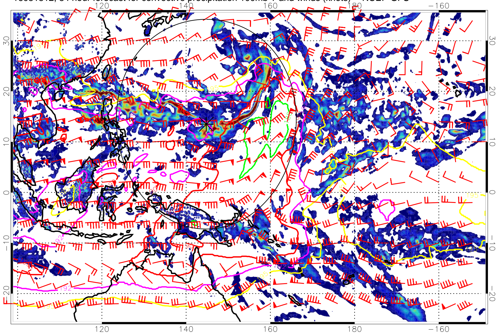
16081812, 84 hour forecast for convective precipitation 100mb T and winds (knots) -- NCEP GFS
