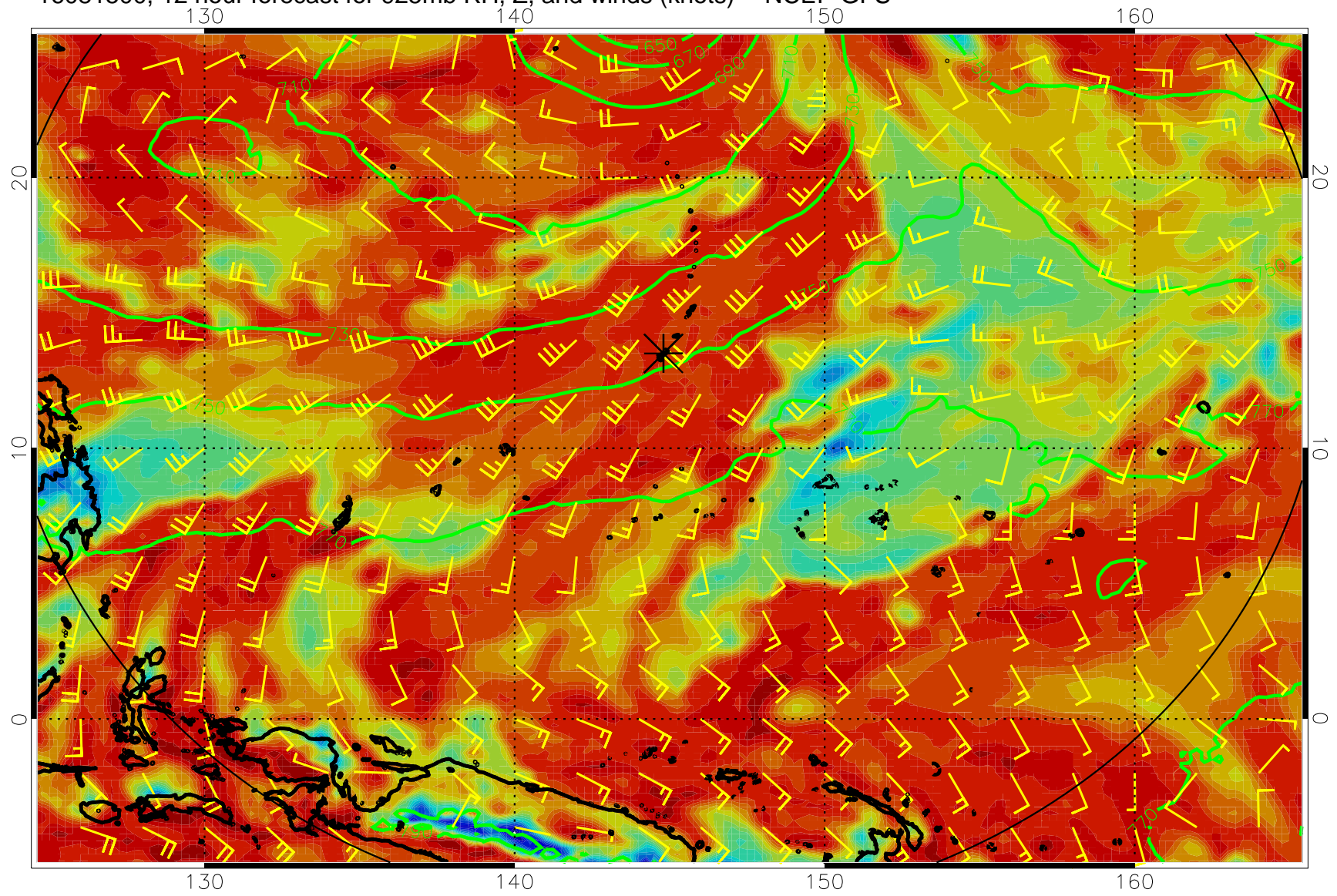
16081500, 12 hour forecast for 925mb RH, Z, and winds (knots) -- NCEP GFS
