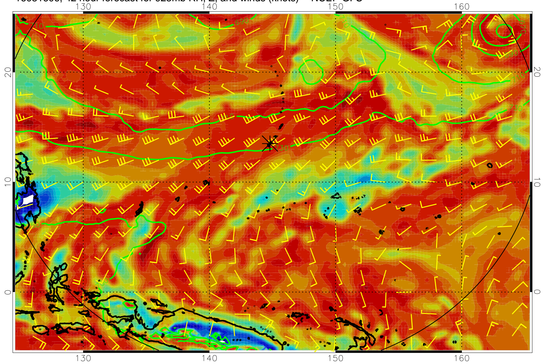
16081606, 42 hour forecast for 925mb RH, Z, and winds (knots) -- NCEP GFS
