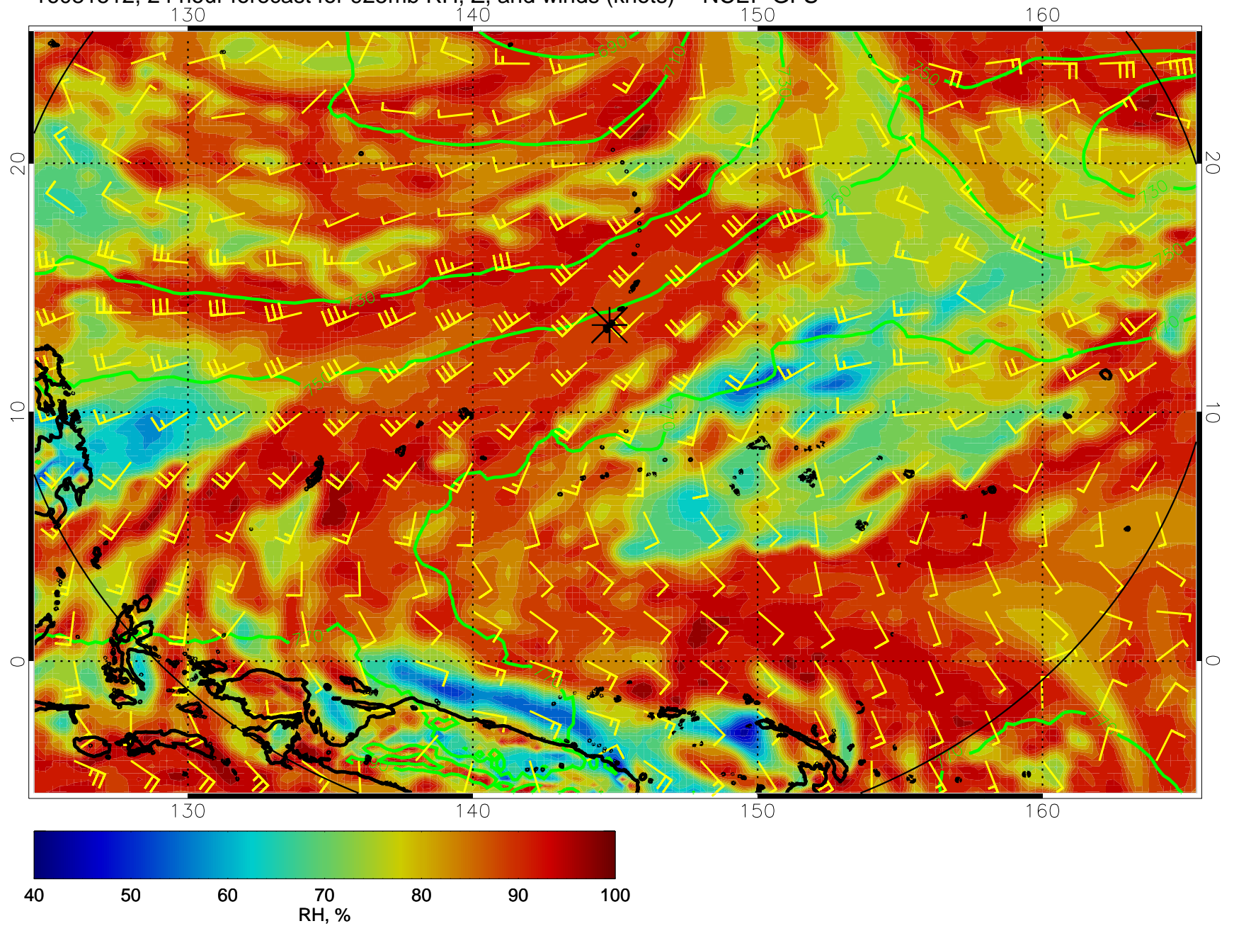
16081512, 24 hour forecast for 925mb RH, Z, and winds (knots) -- NCEP GFS
