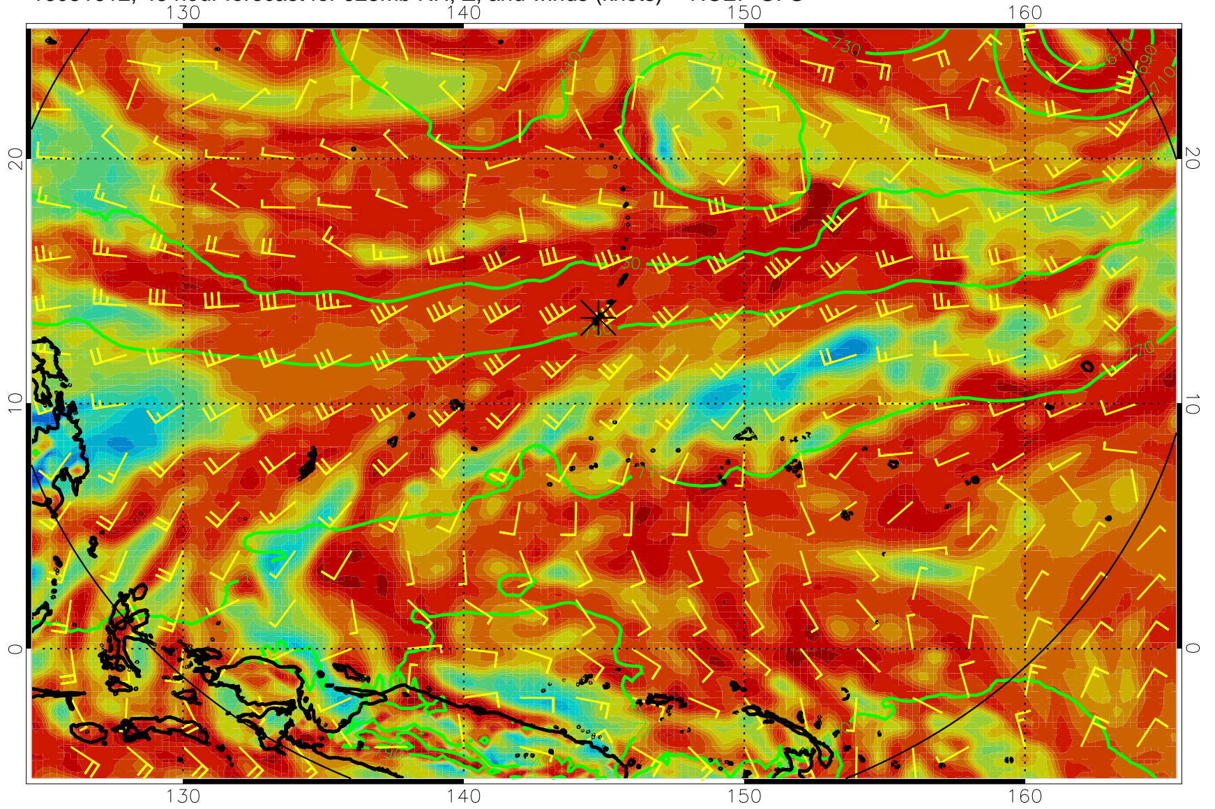
16081612, 48 hour forecast for 925mb RH, Z, and winds (knots) -- NCEP GFS
