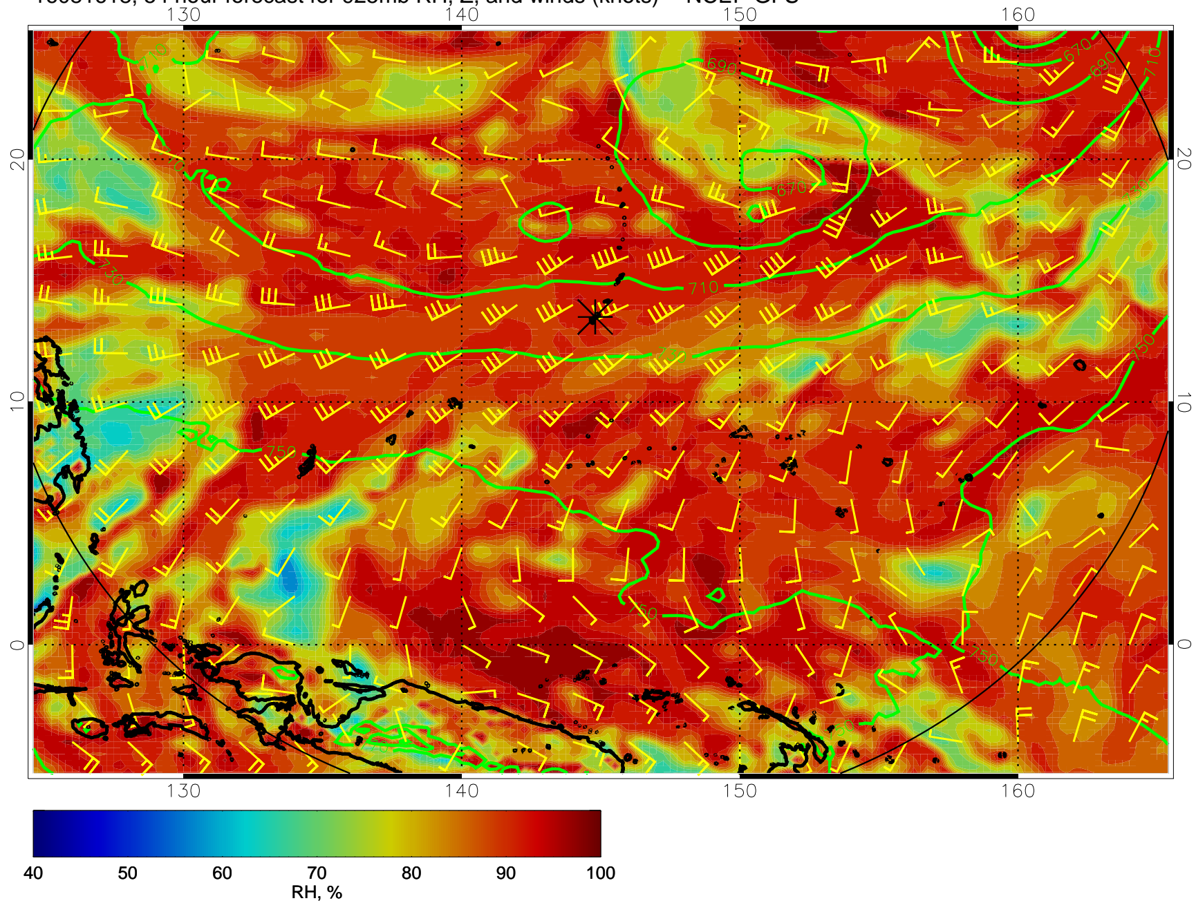
16081618, 54 hour forecast for 925mb RH, Z, and winds (knots) -- NCEP GFS
