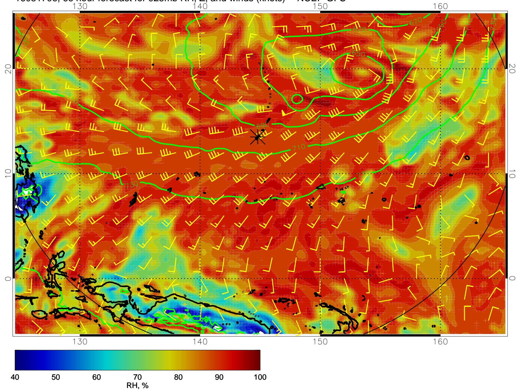
16081706, 66 hour forecast for 925mb RH, Z, and winds (knots) -- NCEP GFS
