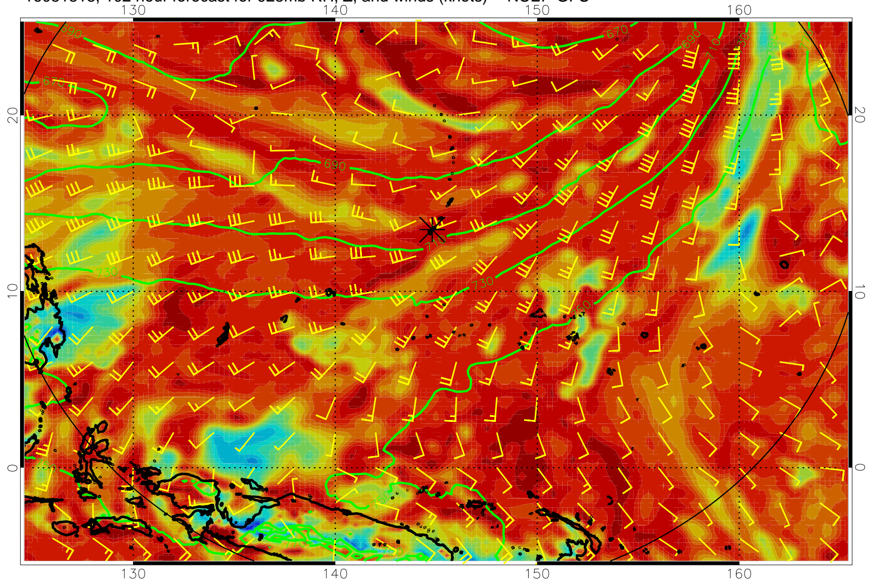
16081818, 102 hour forecast for 925mb RH, Z, and winds (knots) -- NCEP GFS
