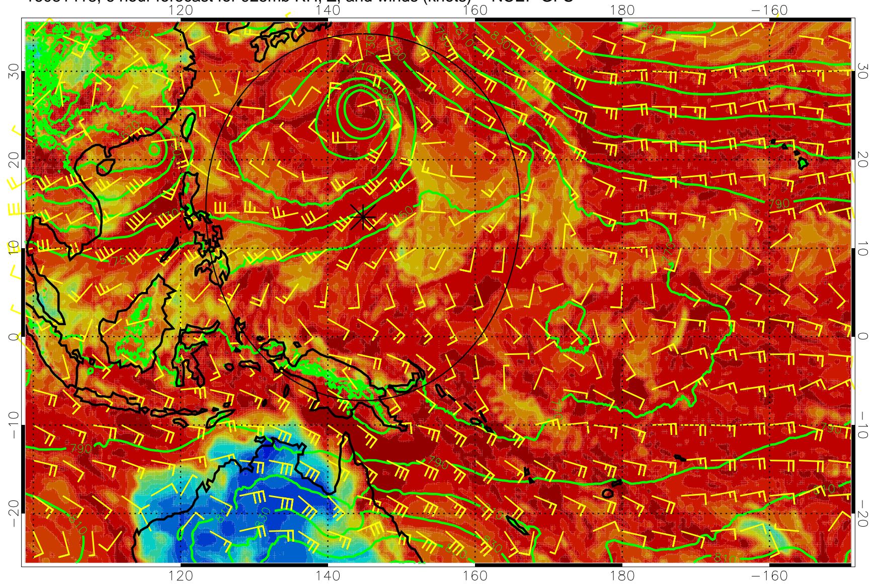
16081418, 6 hour forecast for 925mb RH, Z, and winds (knots) -- NCEP GFS
