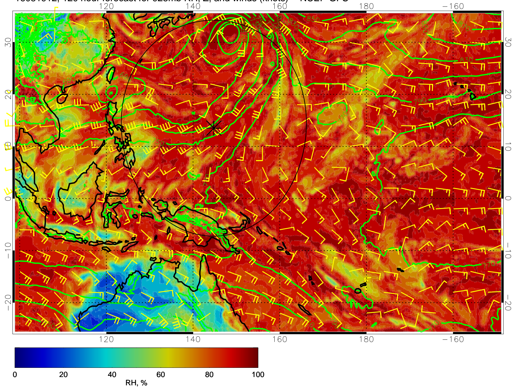
16081912, 120 hour forecast for 925mb RH, Z, and winds (knots) -- NCEP GFS
