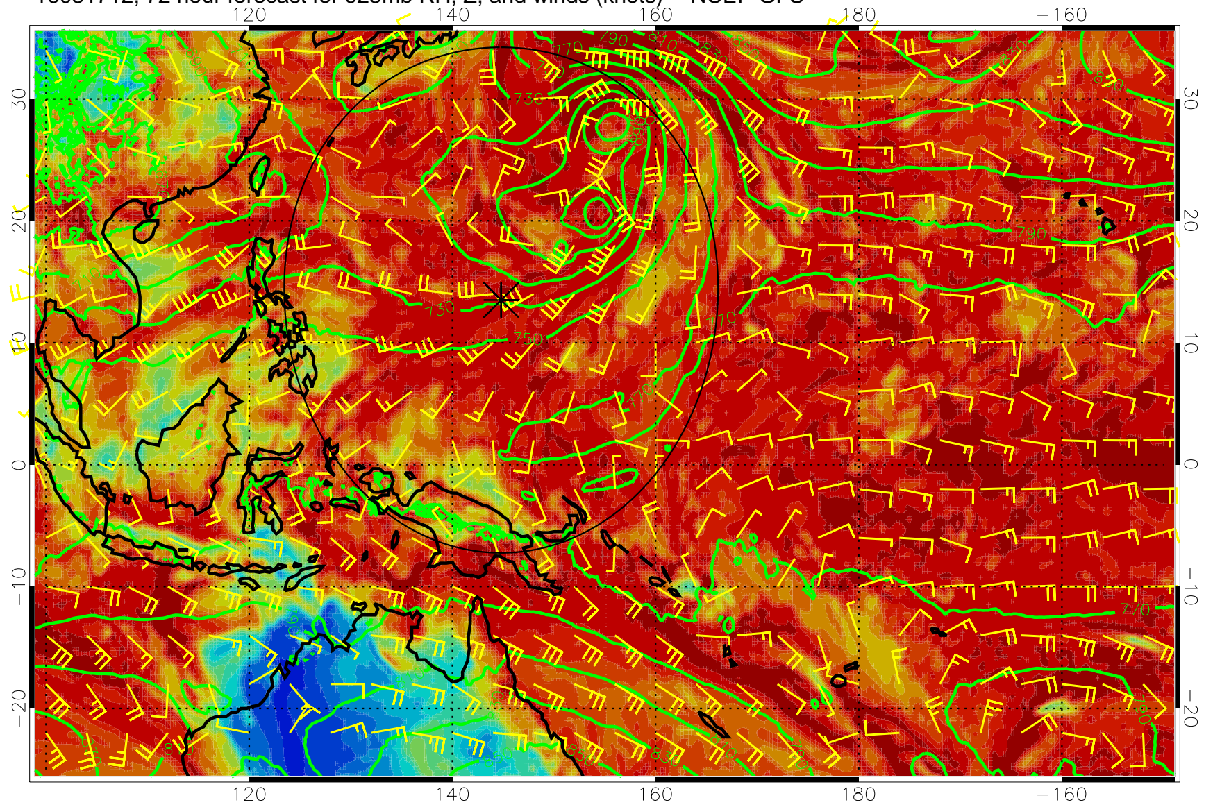
16081712, 72 hour forecast for 925mb RH, Z, and winds (knots) -- NCEP GFS
