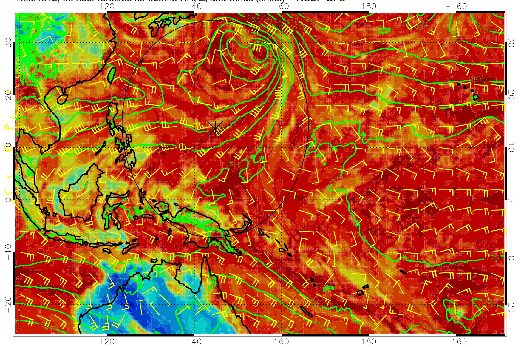
16081812, 96 hour forecast for 925mb RH, Z, and winds (knots) -- NCEP GFS
