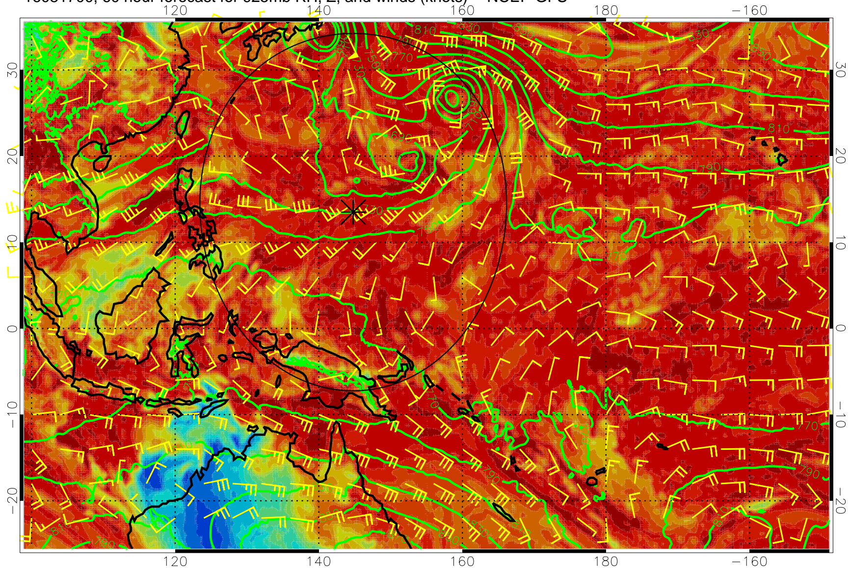
16081700, 60 hour forecast for 925mb RH, Z, and winds (knots) -- NCEP GFS
