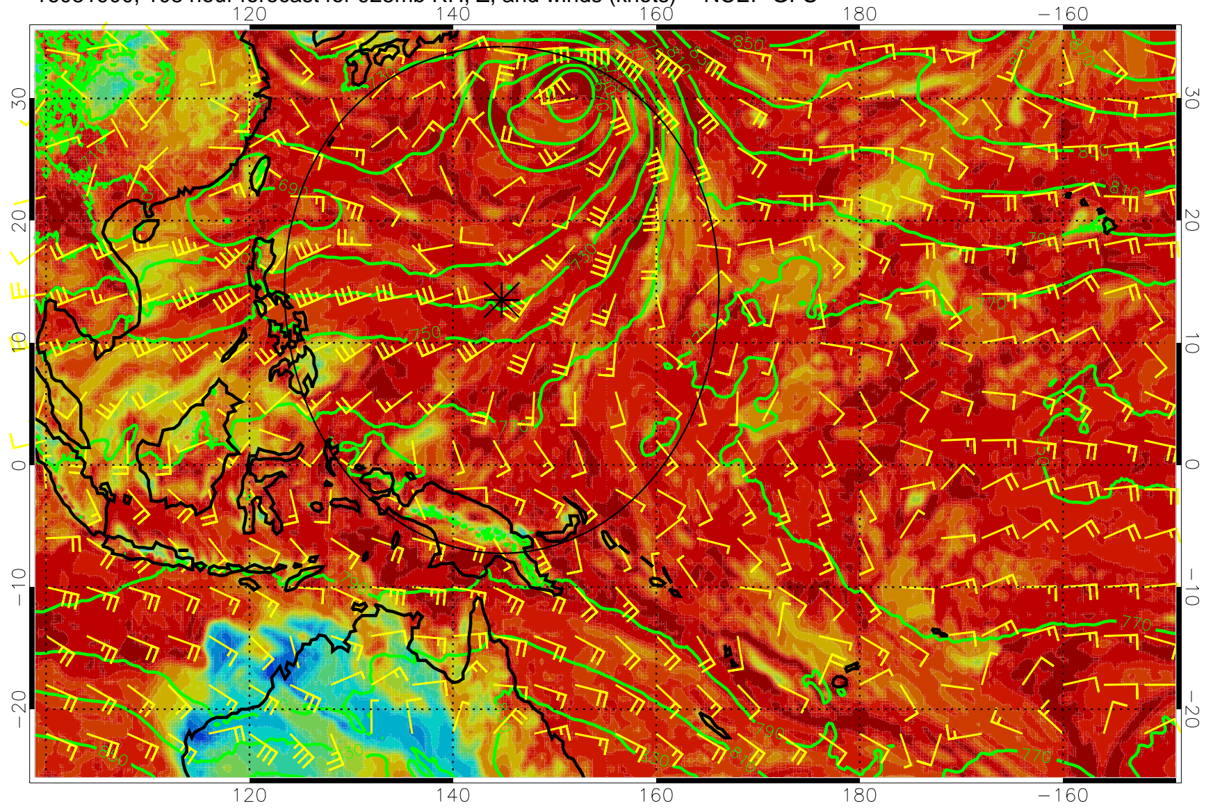
16081900, 108 hour forecast for 925mb RH, Z, and winds (knots) -- NCEP GFS
