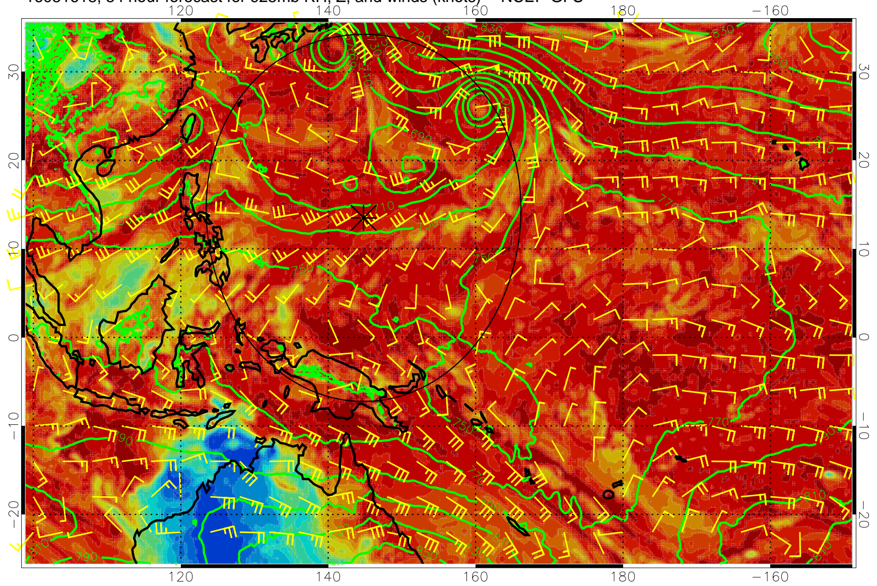
16081618, 54 hour forecast for 925mb RH, Z, and winds (knots) -- NCEP GFS
