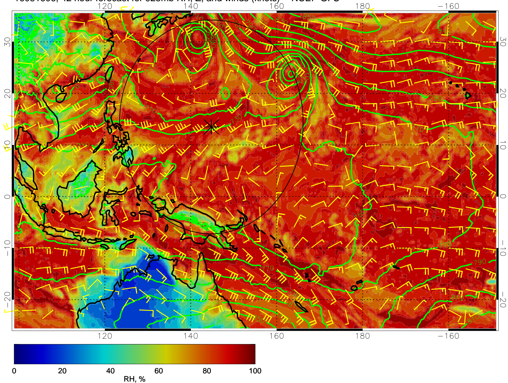
16081606, 42 hour forecast for 925mb RH, Z, and winds (knots) -- NCEP GFS
