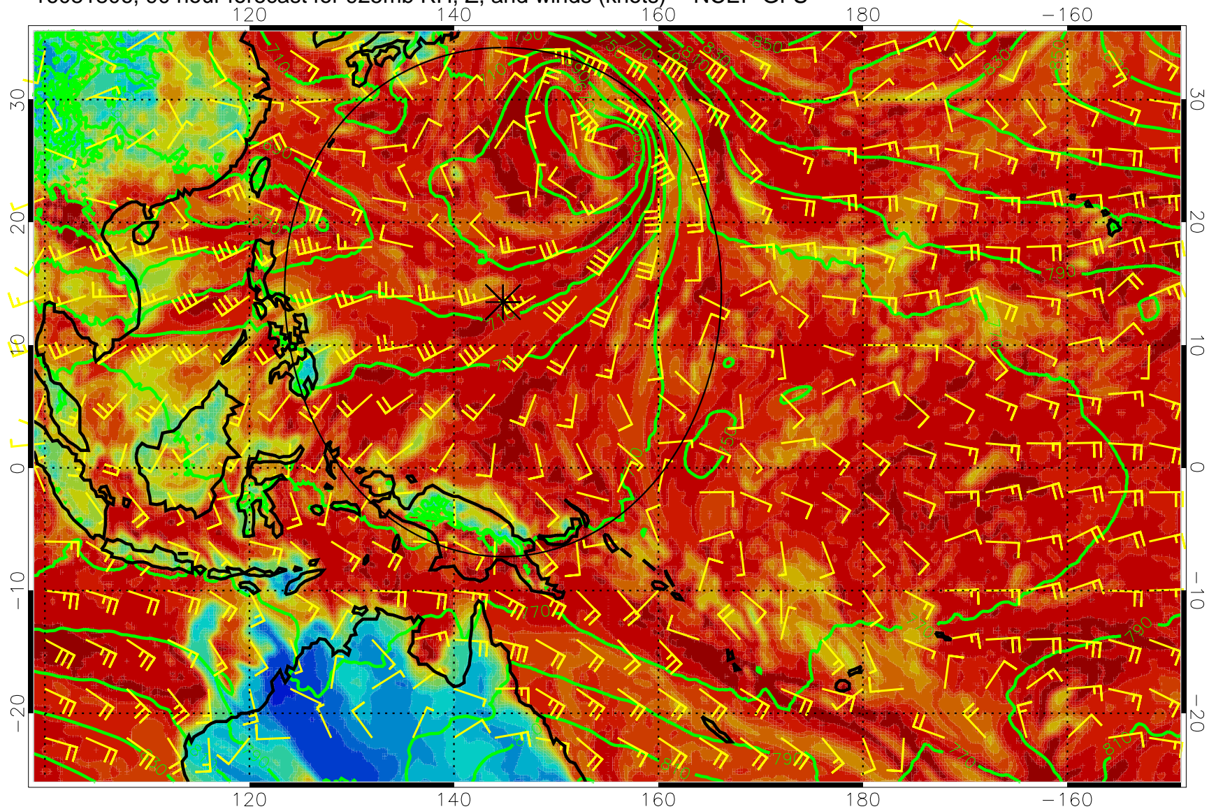
16081806, 90 hour forecast for 925mb RH, Z, and winds (knots) -- NCEP GFS
