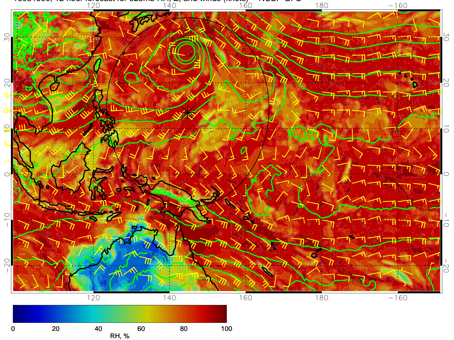
16081500, 12 hour forecast for 925mb RH, Z, and winds (knots) -- NCEP GFS
