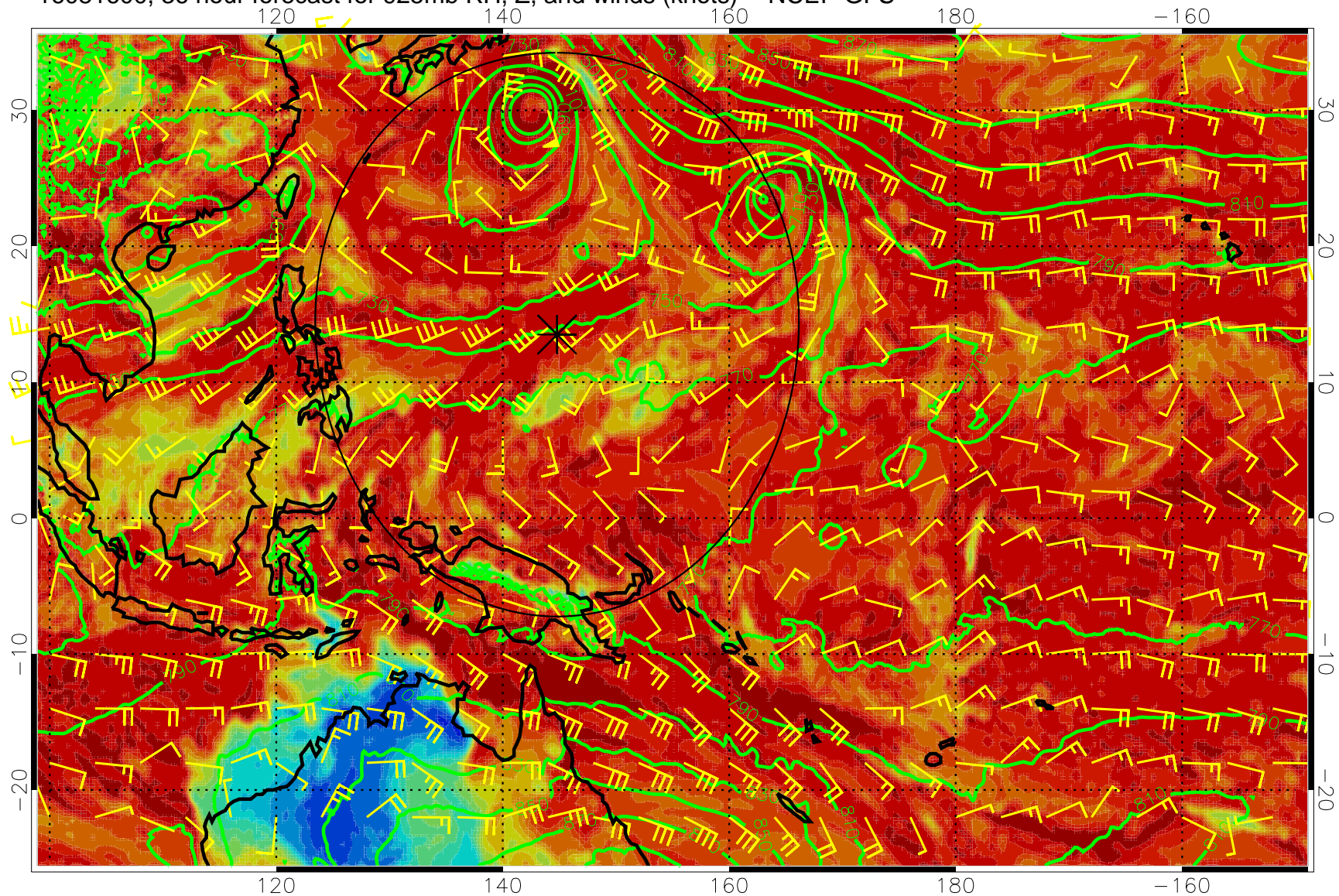
16081600, 36 hour forecast for 925mb RH, Z, and winds (knots) -- NCEP GFS
