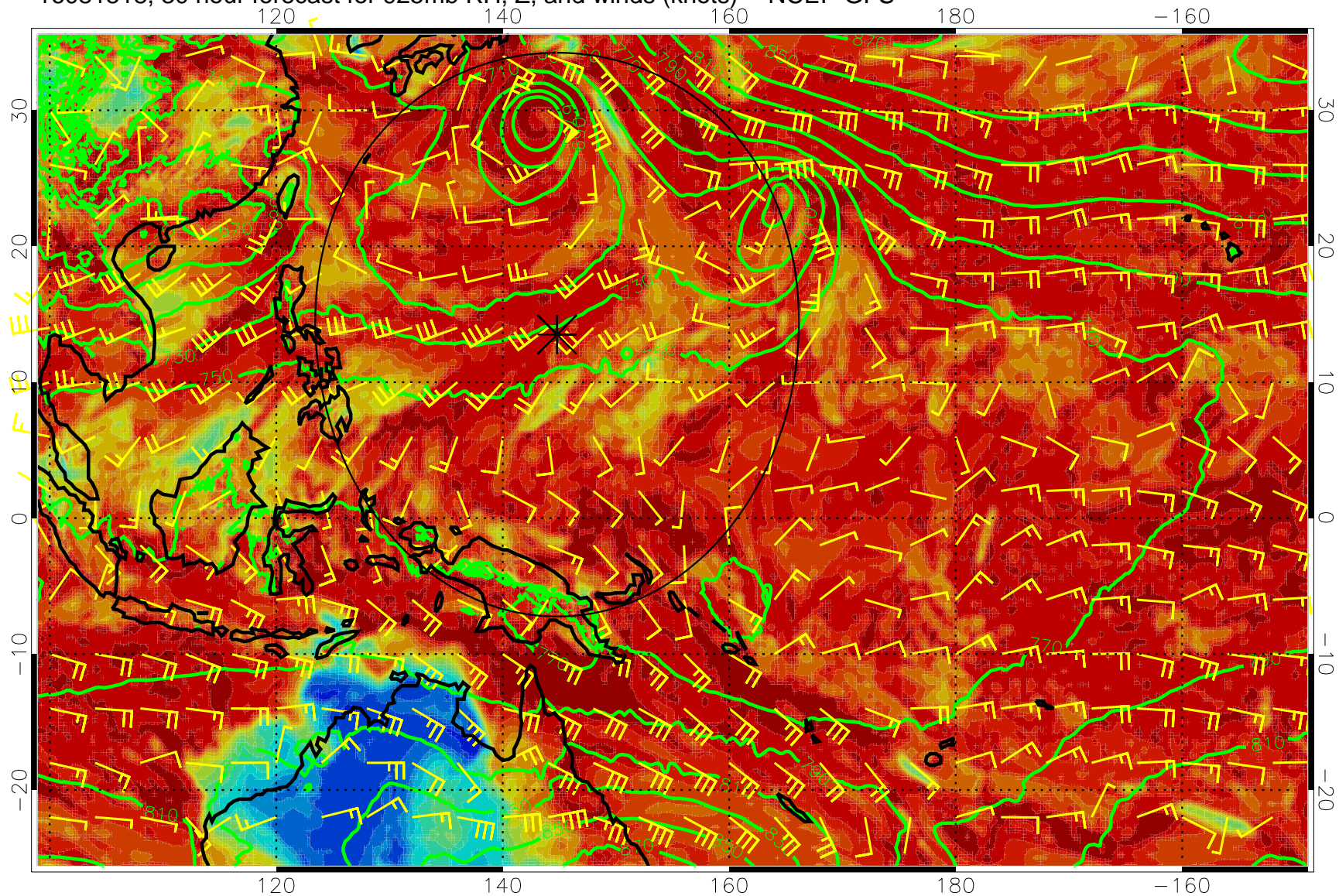
16081518, 30 hour forecast for 925mb RH, Z, and winds (knots) -- NCEP GFS
