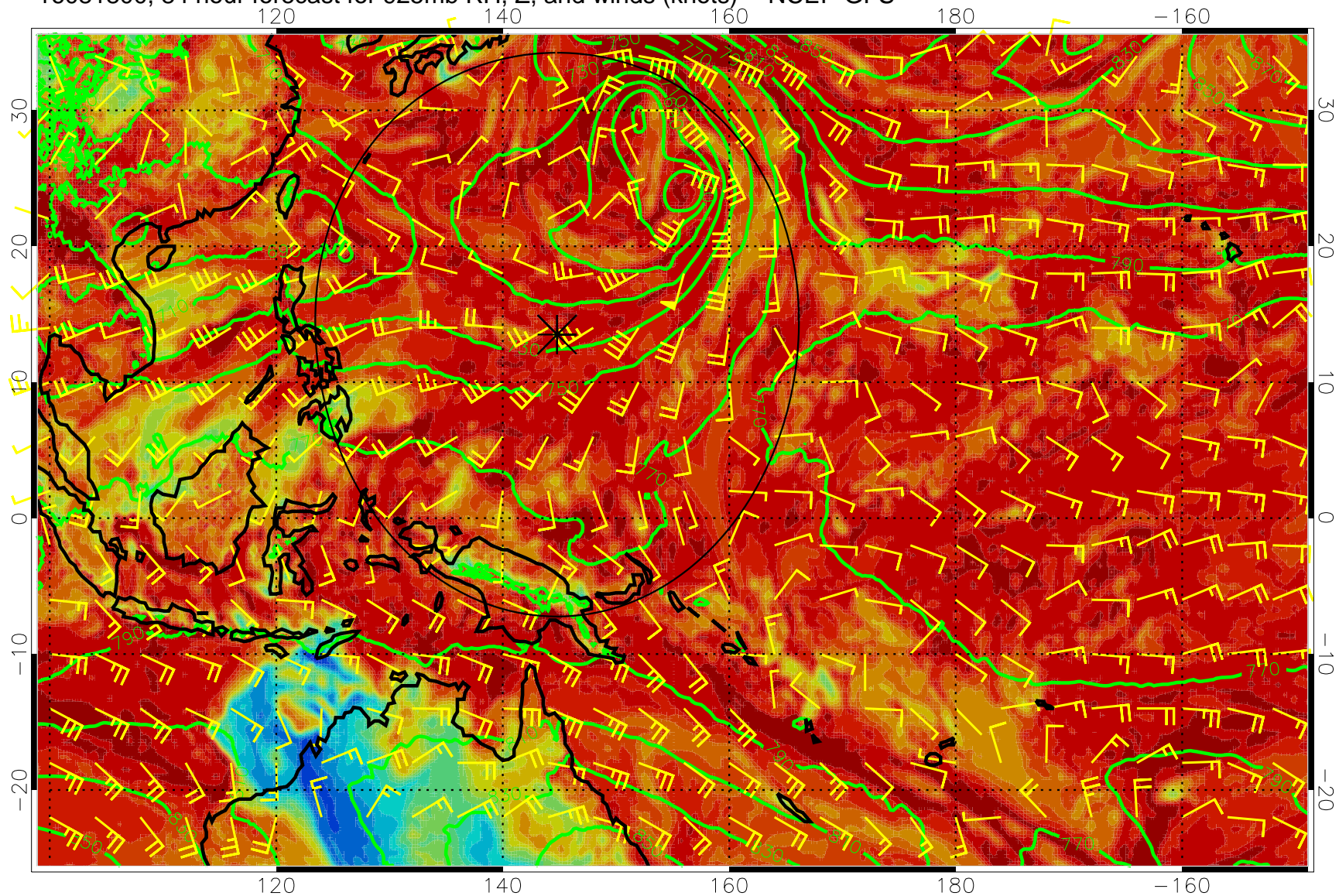
16081800, 84 hour forecast for 925mb RH, Z, and winds (knots) -- NCEP GFS
