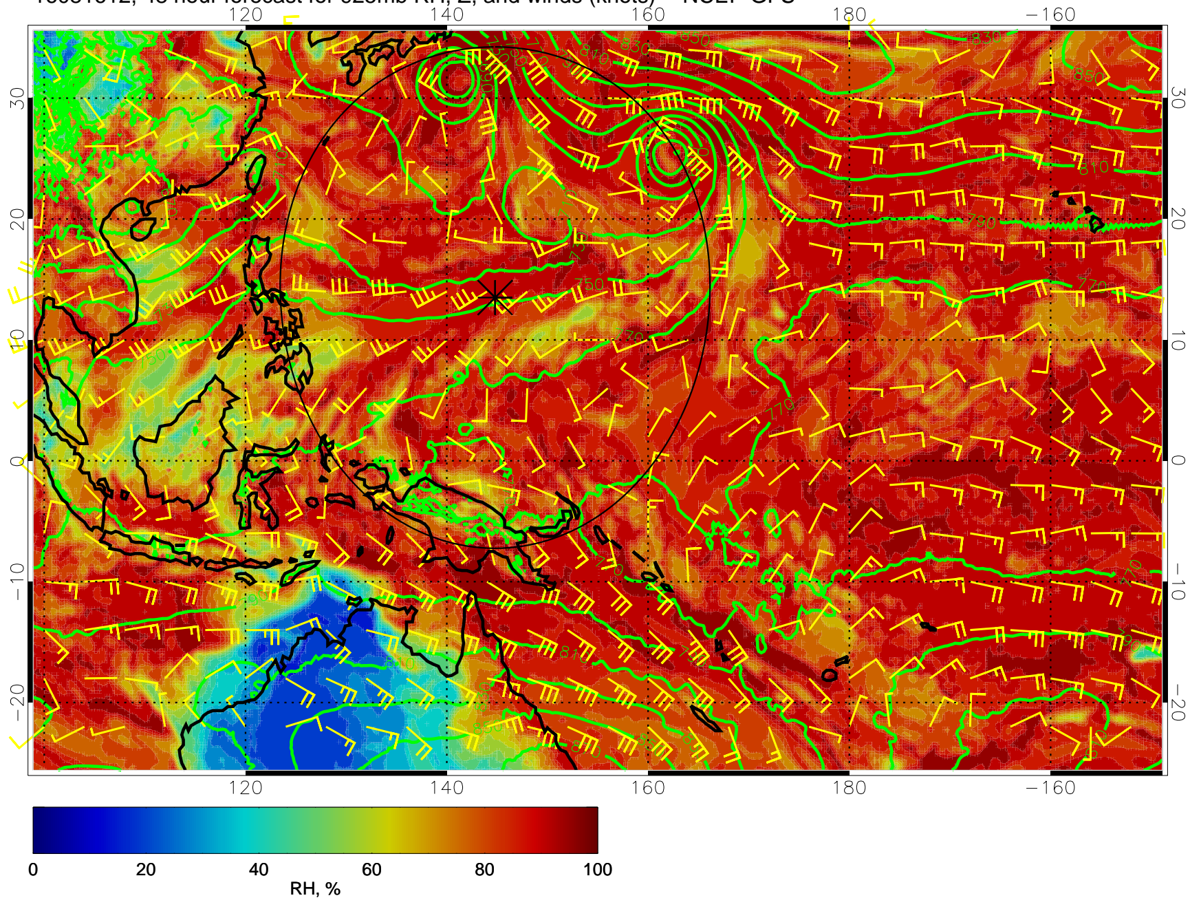
16081612, 48 hour forecast for 925mb RH, Z, and winds (knots) -- NCEP GFS
