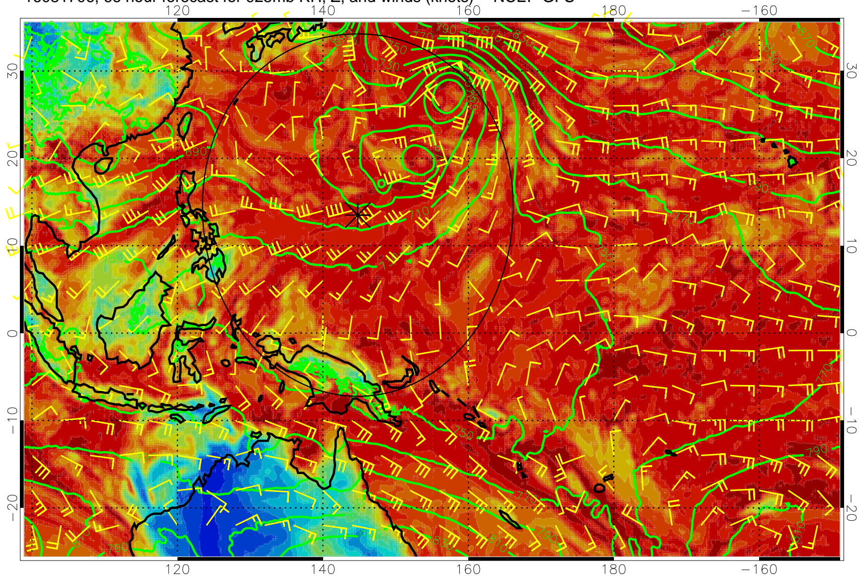
16081706, 66 hour forecast for 925mb RH, Z, and winds (knots) -- NCEP GFS
