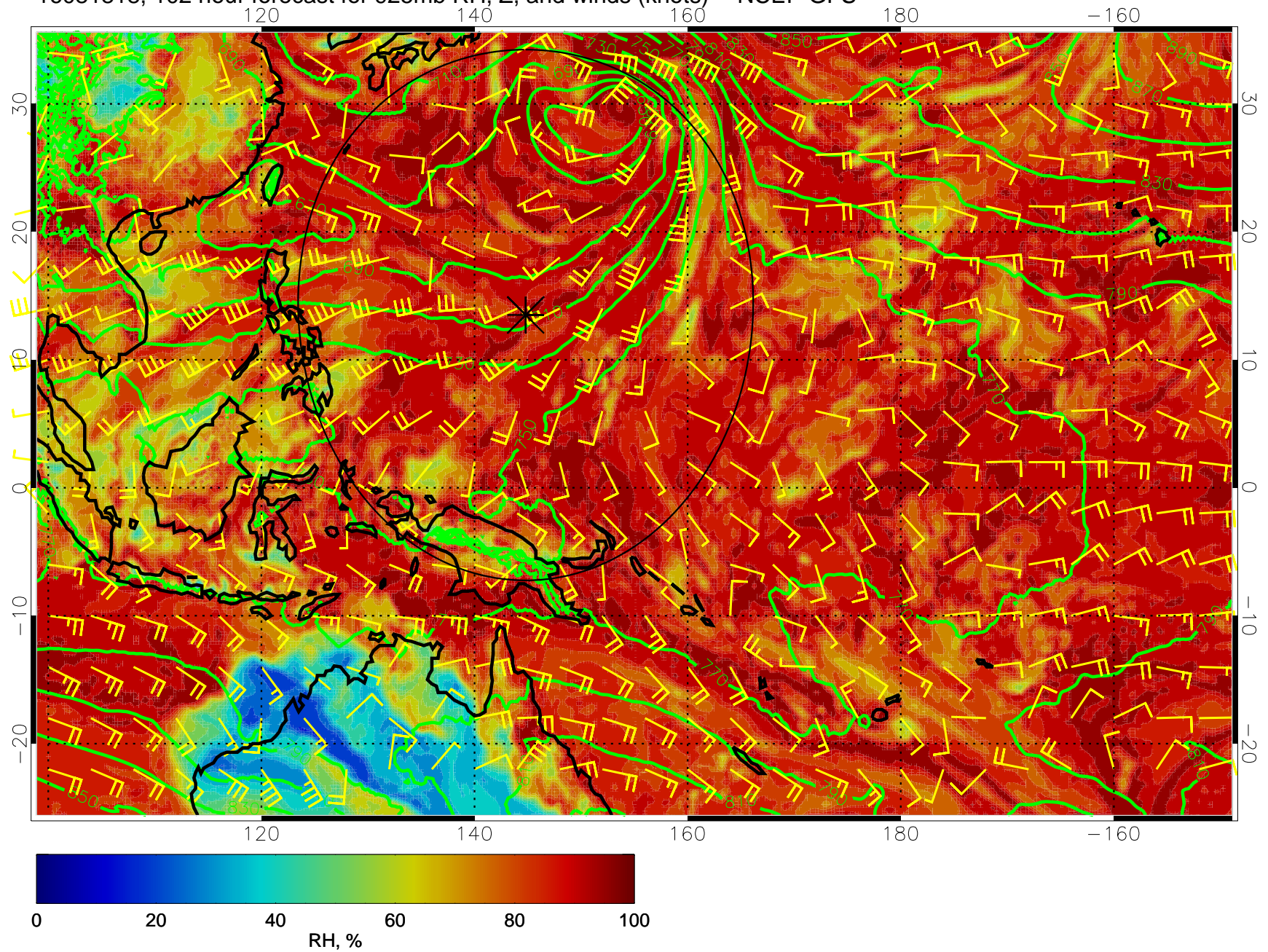
16081818, 102 hour forecast for 925mb RH, Z, and winds (knots) -- NCEP GFS
