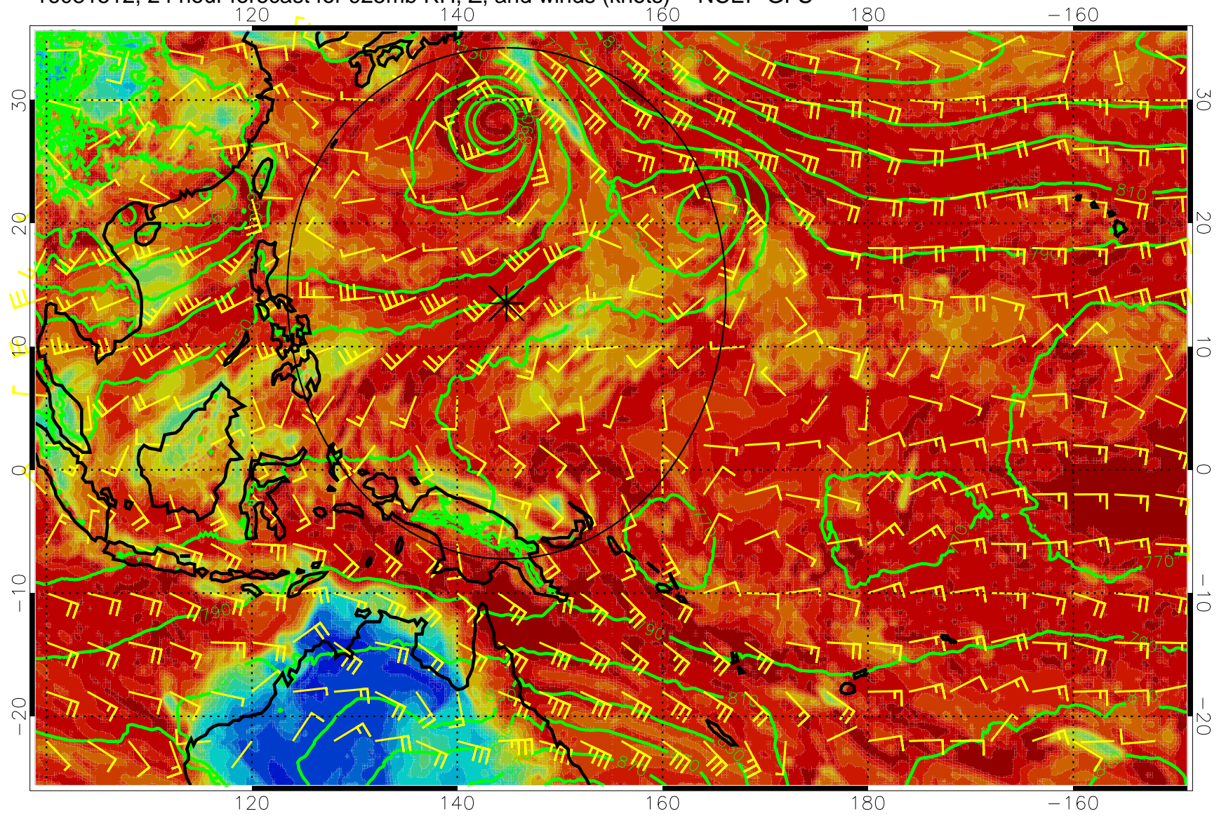
16081512, 24 hour forecast for 925mb RH, Z, and winds (knots) -- NCEP GFS
