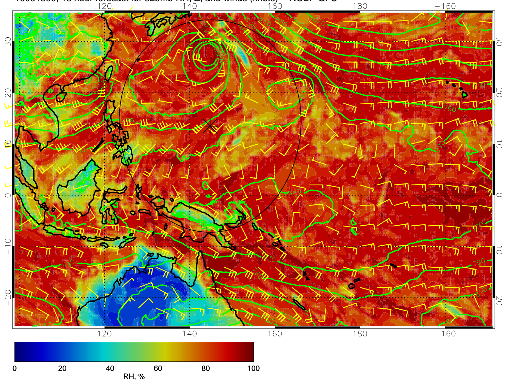
16081506, 18 hour forecast for 925mb RH, Z, and winds (knots) -- NCEP GFS
