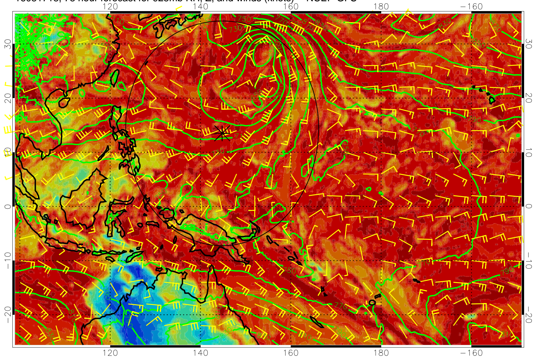
16081718, 78 hour forecast for 925mb RH, Z, and winds (knots) -- NCEP GFS
