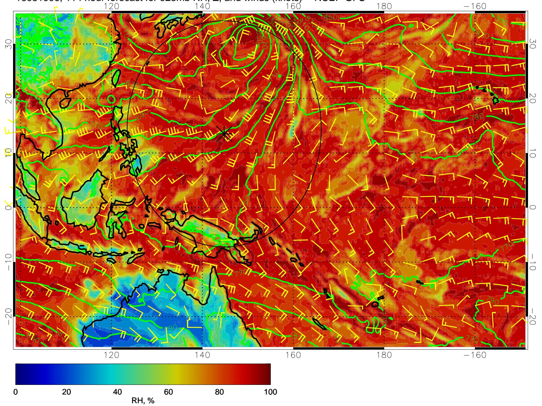
16081906, 114 hour forecast for 925mb RH, Z, and winds (knots) -- NCEP GFS
