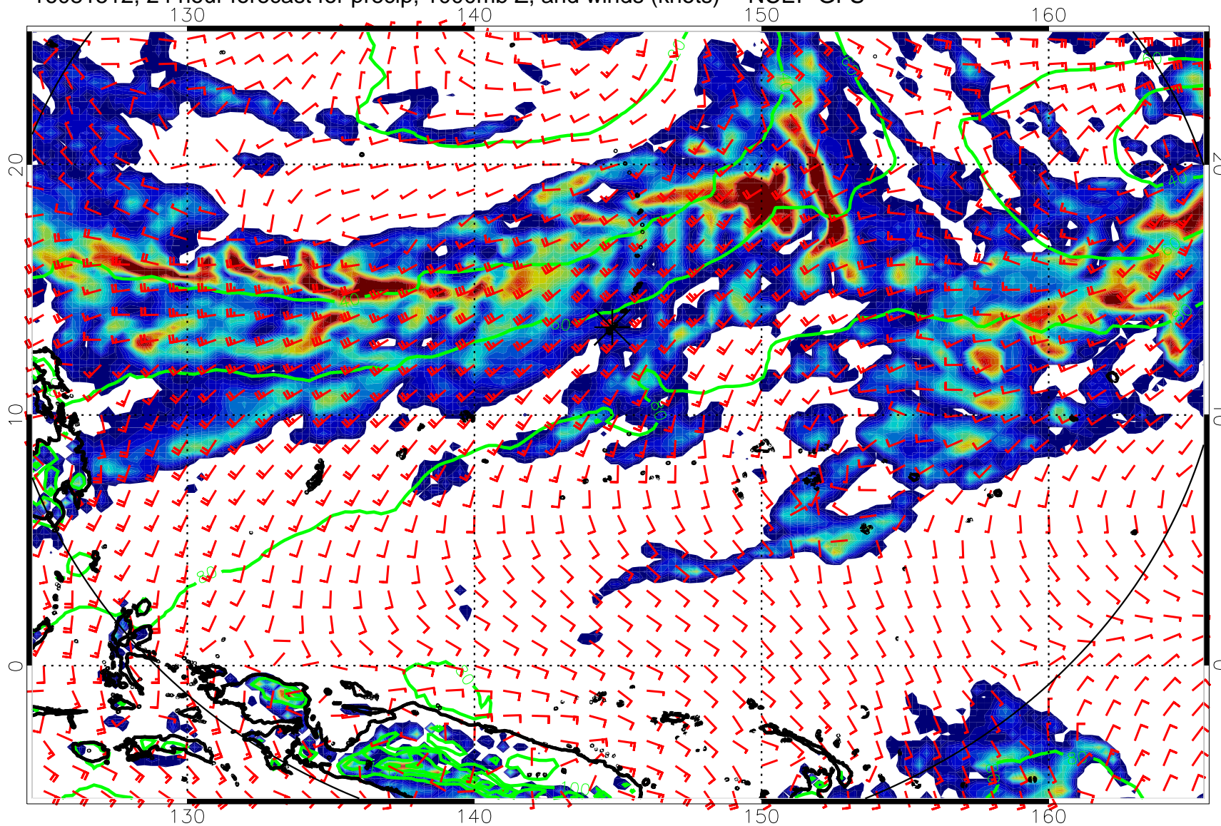
16081512, 24 hour forecast for precip, 1000mb Z, and winds (knots) -- NCEP GFS
