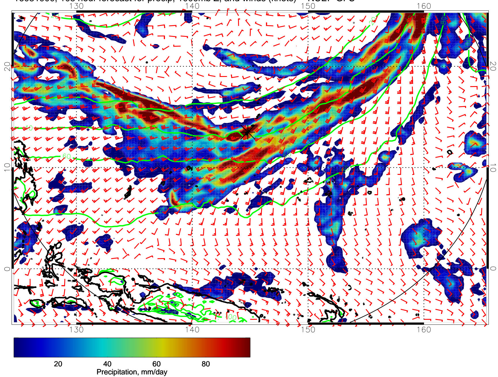
16081900, 108 hour forecast for precip, 1000mb Z, and winds (knots) -- NCEP GFS
