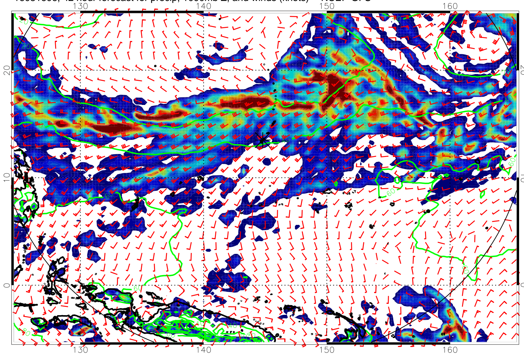
16081606, 42 hour forecast for precip, 1000mb Z, and winds (knots) -- NCEP GFS
