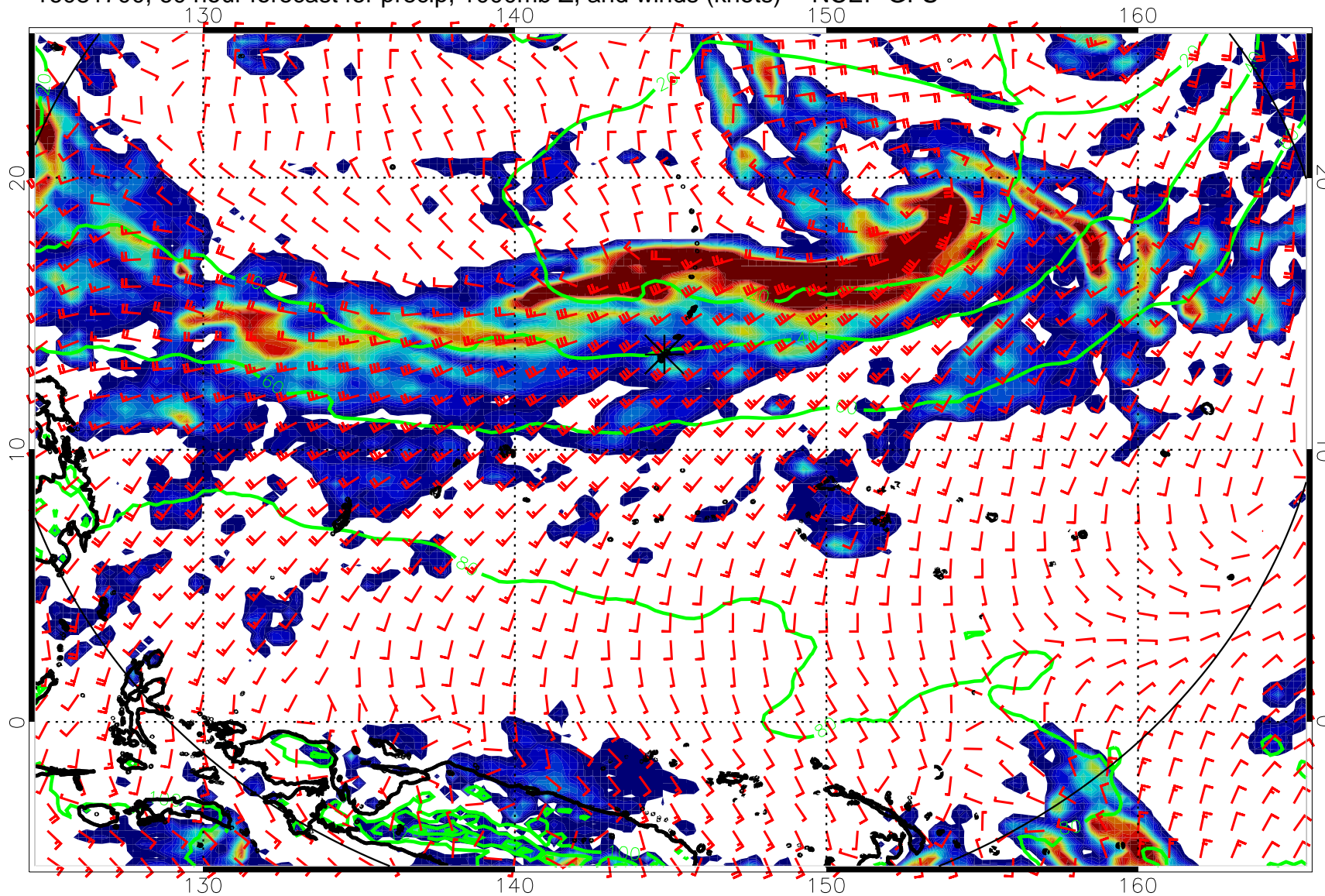
16081700, 60 hour forecast for precip, 1000mb Z, and winds (knots) -- NCEP GFS
