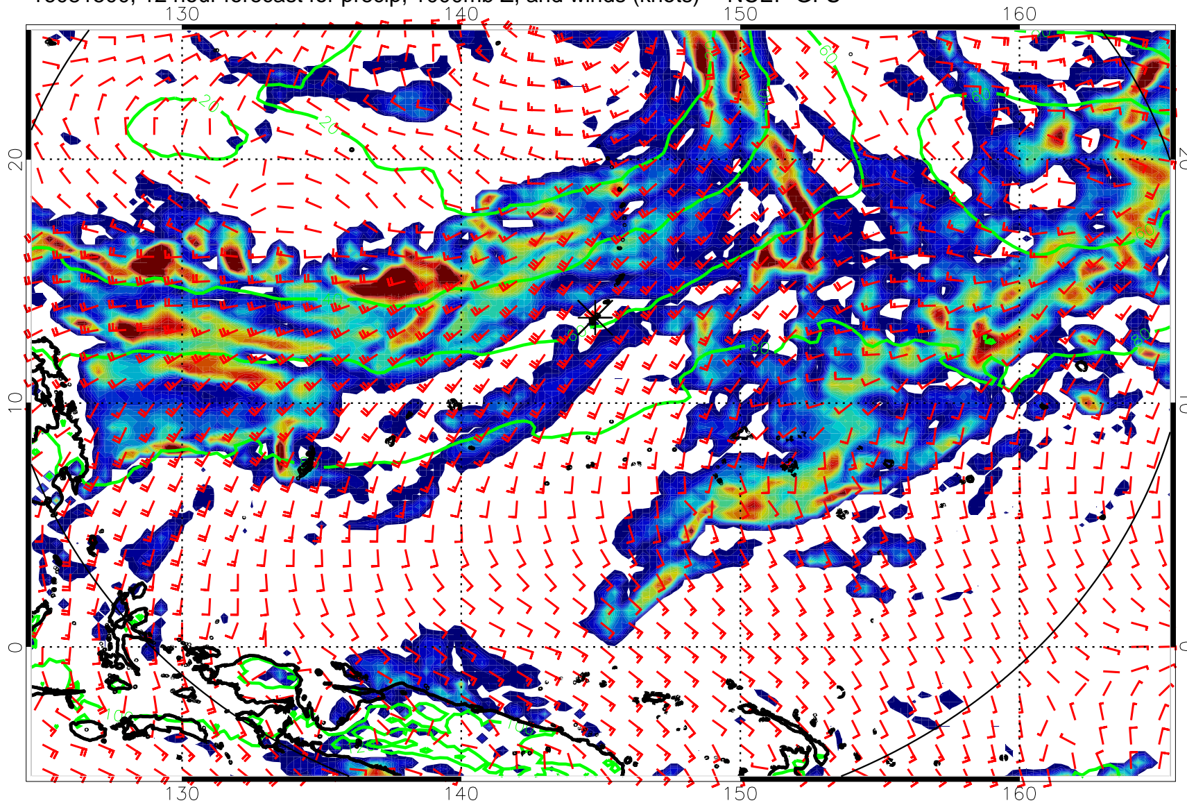
16081500, 12 hour forecast for precip, 1000mb Z, and winds (knots) -- NCEP GFS
