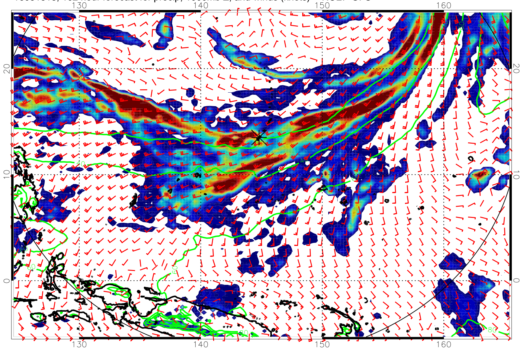
16081818, 102 hour forecast for precip, 1000mb Z, and winds (knots) -- NCEP GFS
