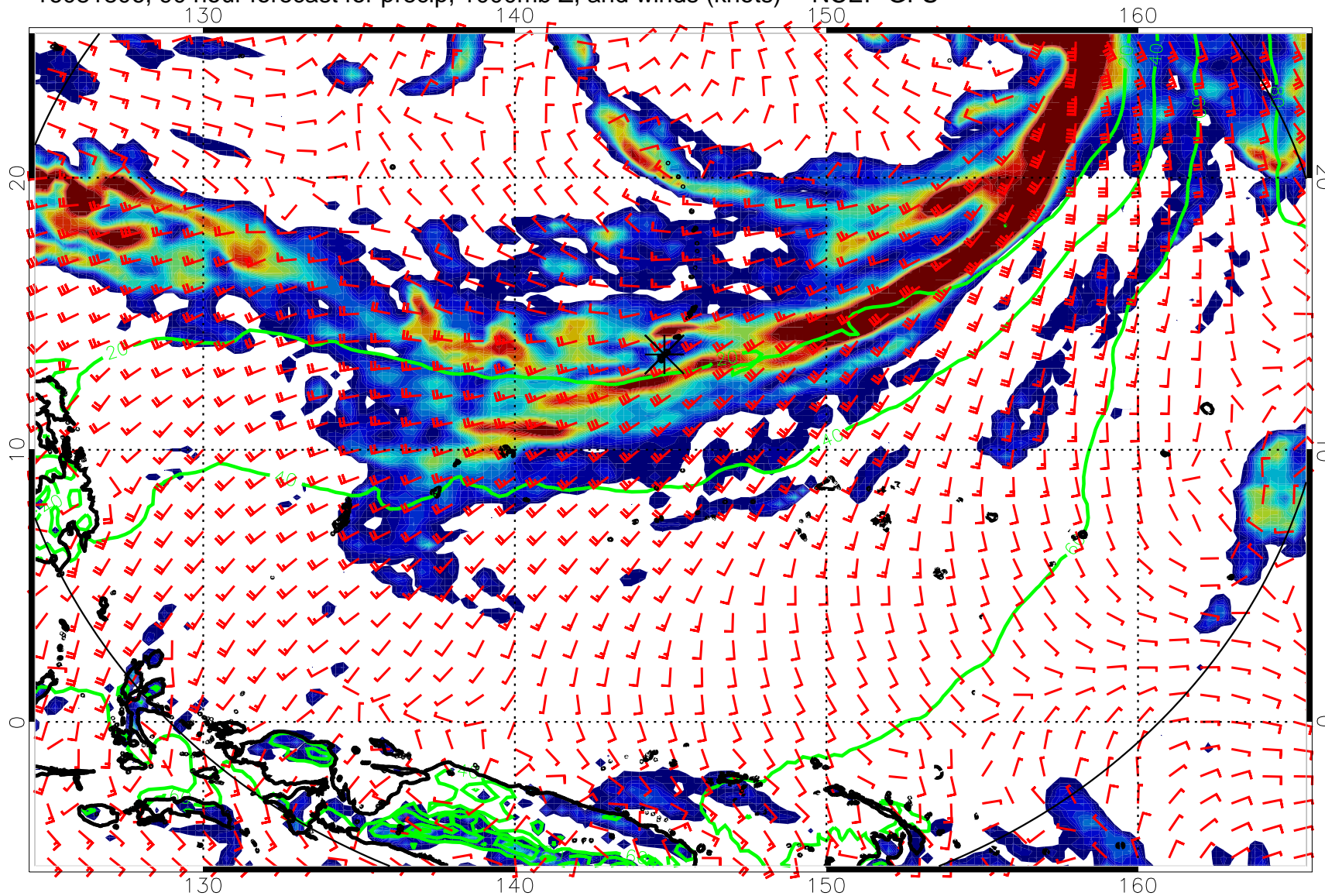
16081806, 90 hour forecast for precip, 1000mb Z, and winds (knots) -- NCEP GFS
