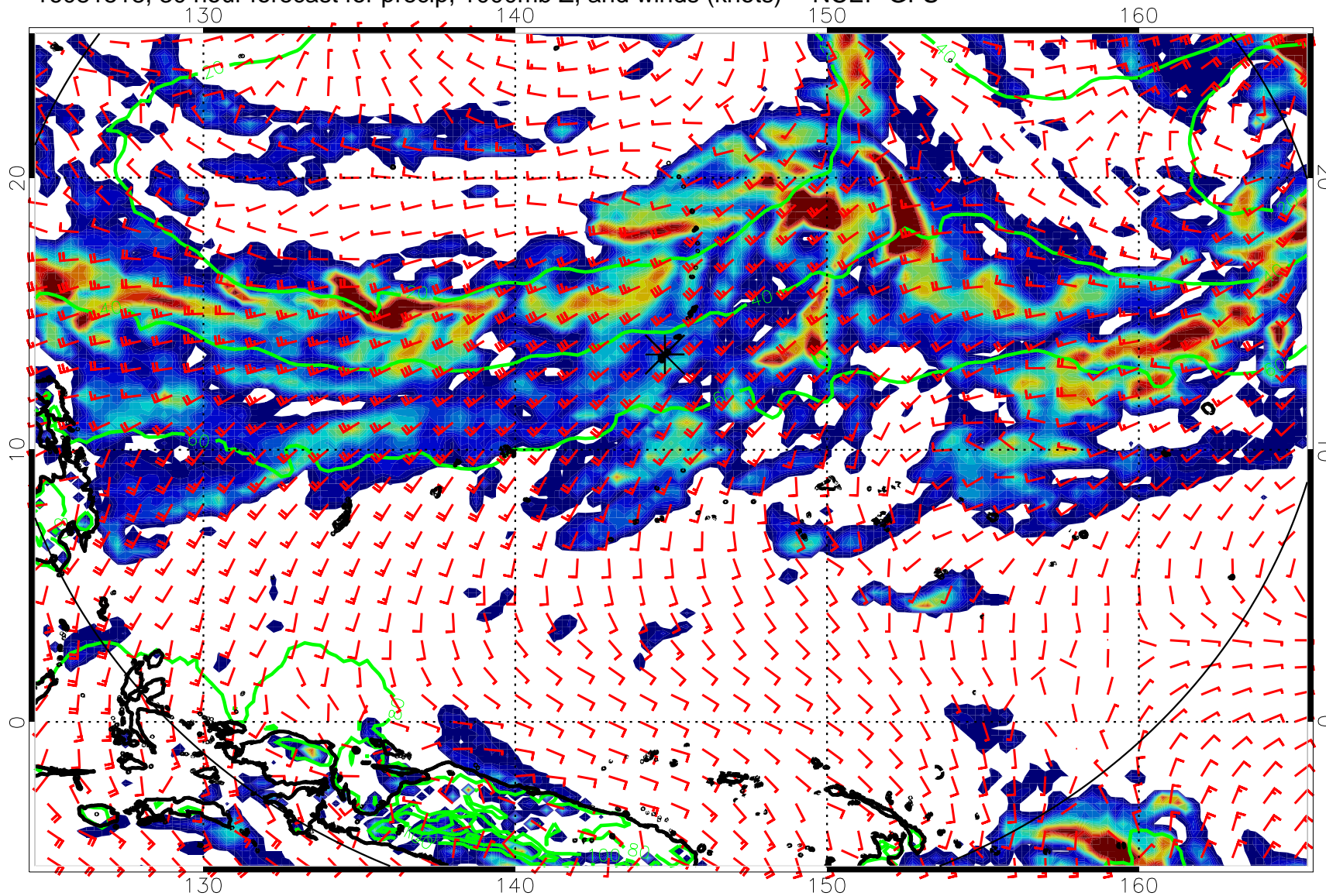
16081518, 30 hour forecast for precip, 1000mb Z, and winds (knots) -- NCEP GFS
