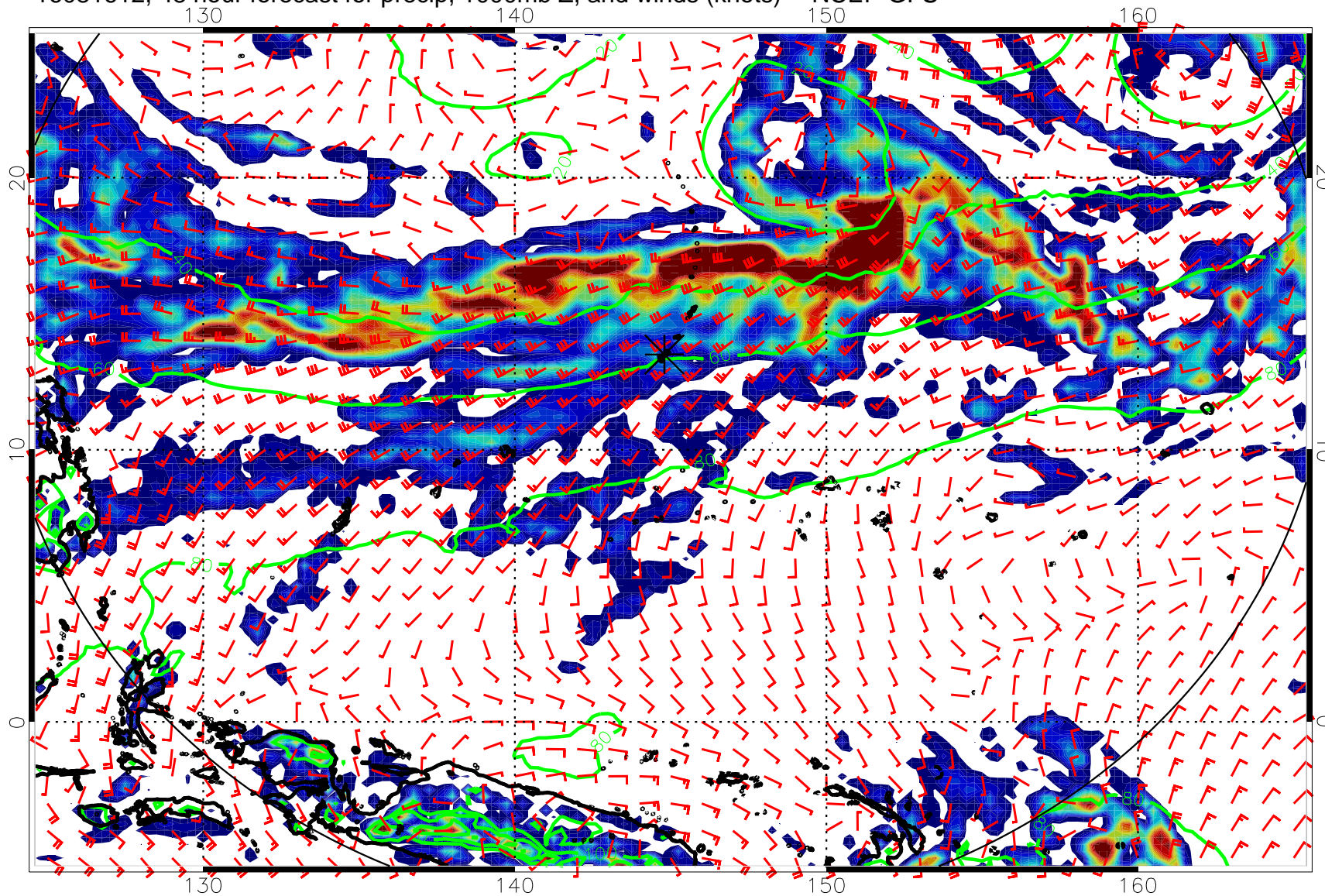
16081612, 48 hour forecast for precip, 1000mb Z, and winds (knots) -- NCEP GFS
