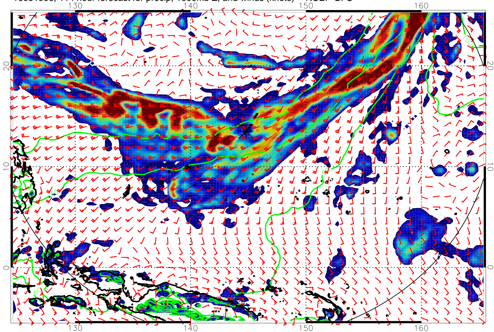
16081906, 114 hour forecast for precip, 1000mb Z, and winds (knots) -- NCEP GFS
