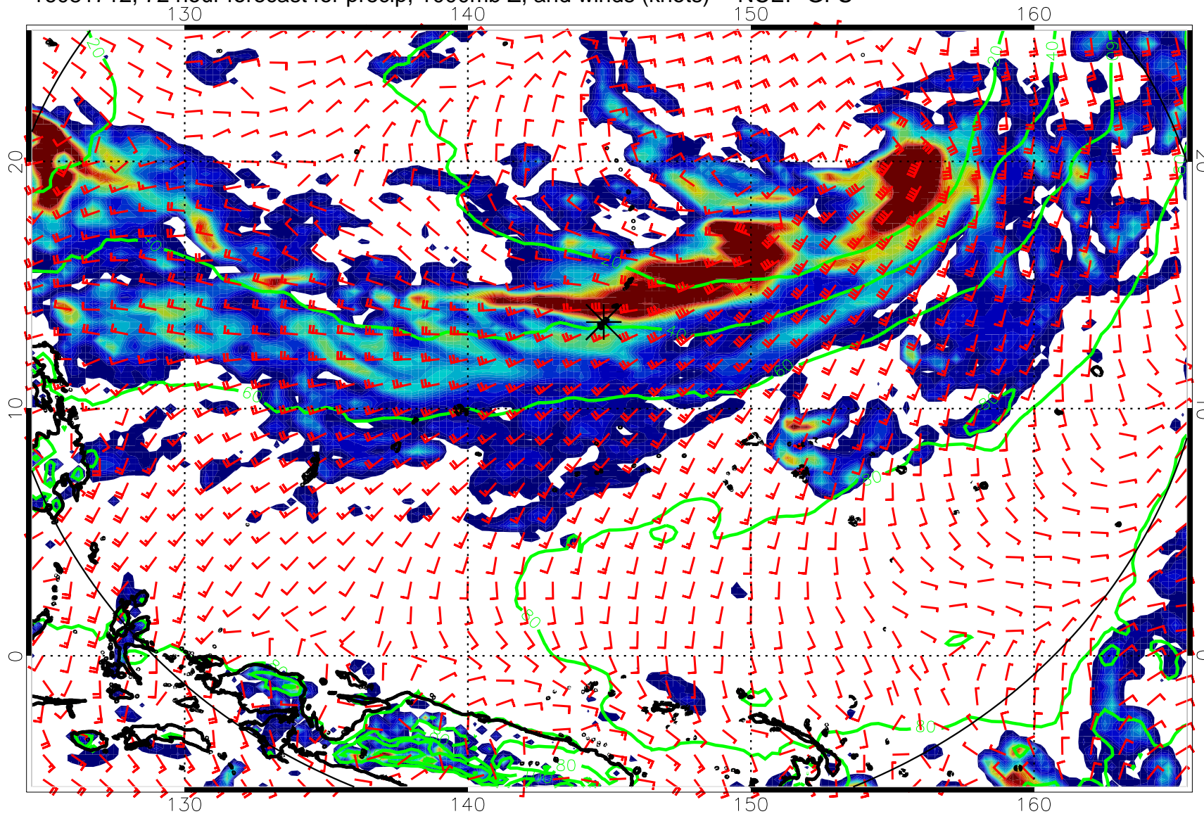
16081712, 72 hour forecast for precip, 1000mb Z, and winds (knots) -- NCEP GFS
