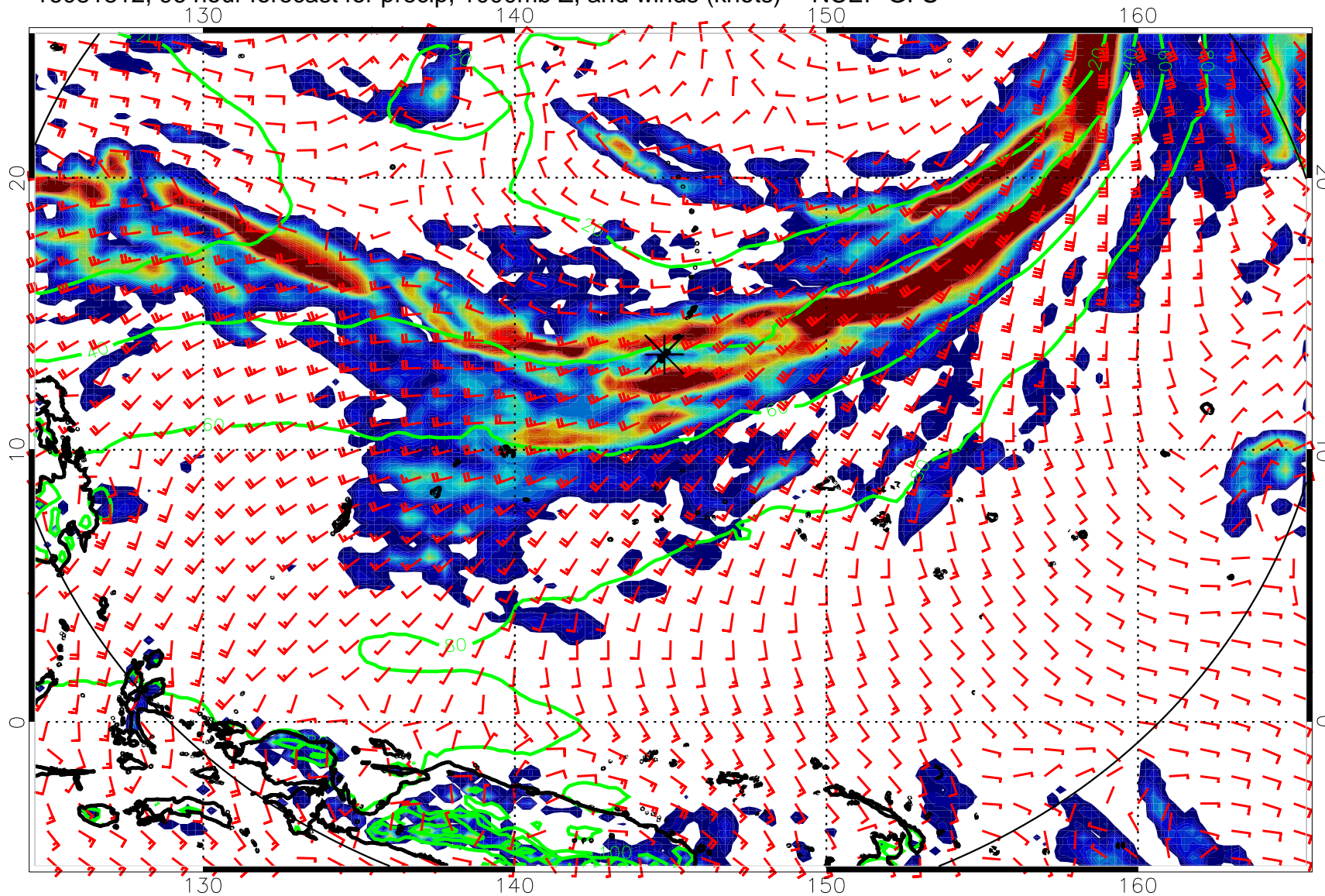
16081812, 96 hour forecast for precip, 1000mb Z, and winds (knots) -- NCEP GFS
