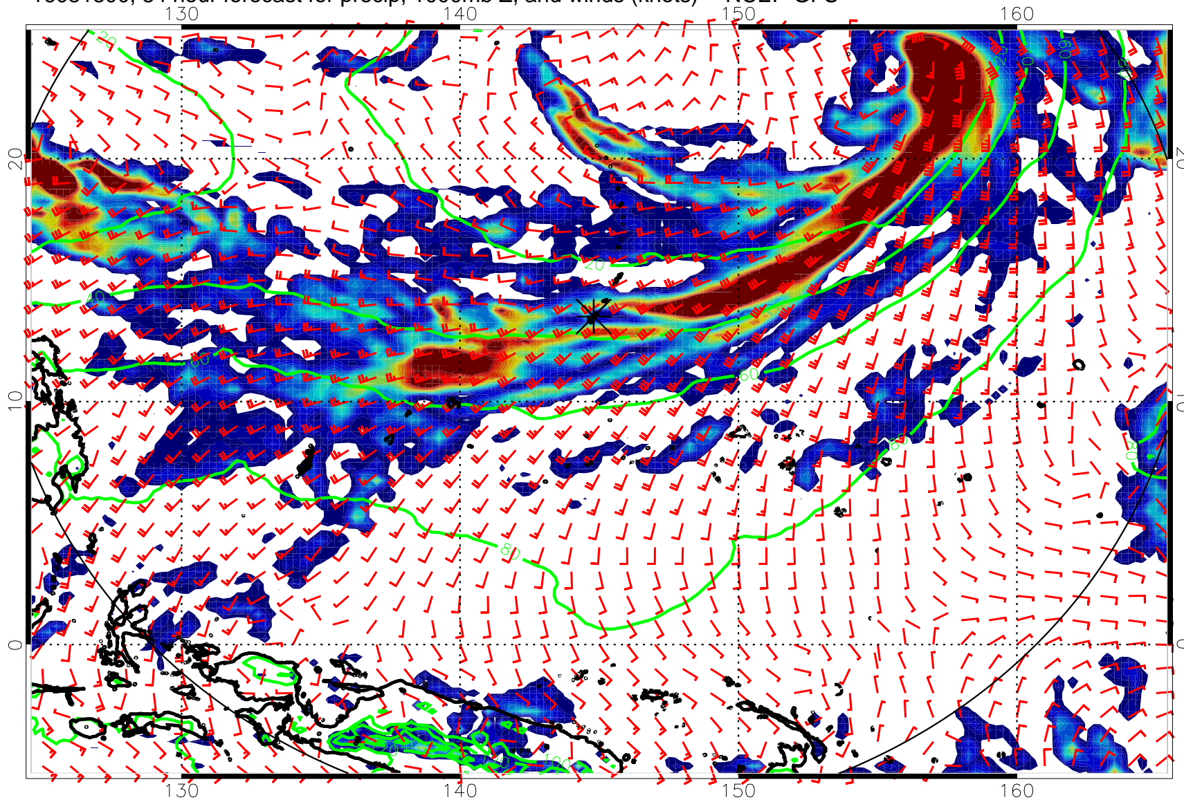
16081800, 84 hour forecast for precip, 1000mb Z, and winds (knots) -- NCEP GFS
