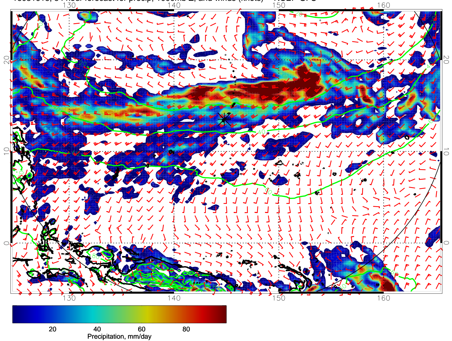
16081618, 54 hour forecast for precip, 1000mb Z, and winds (knots) -- NCEP GFS
