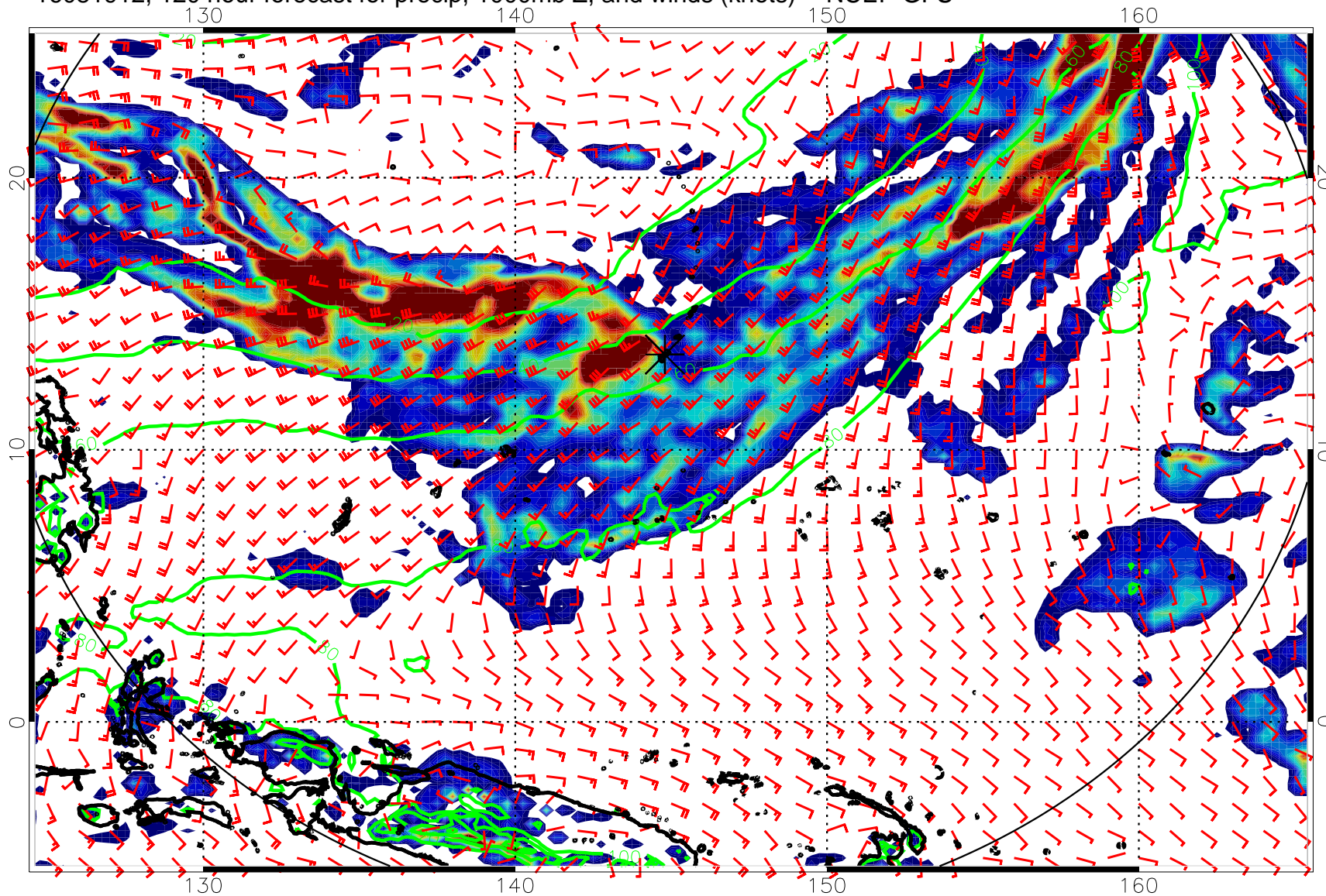
16081912, 120 hour forecast for precip, 1000mb Z, and winds (knots) -- NCEP GFS
