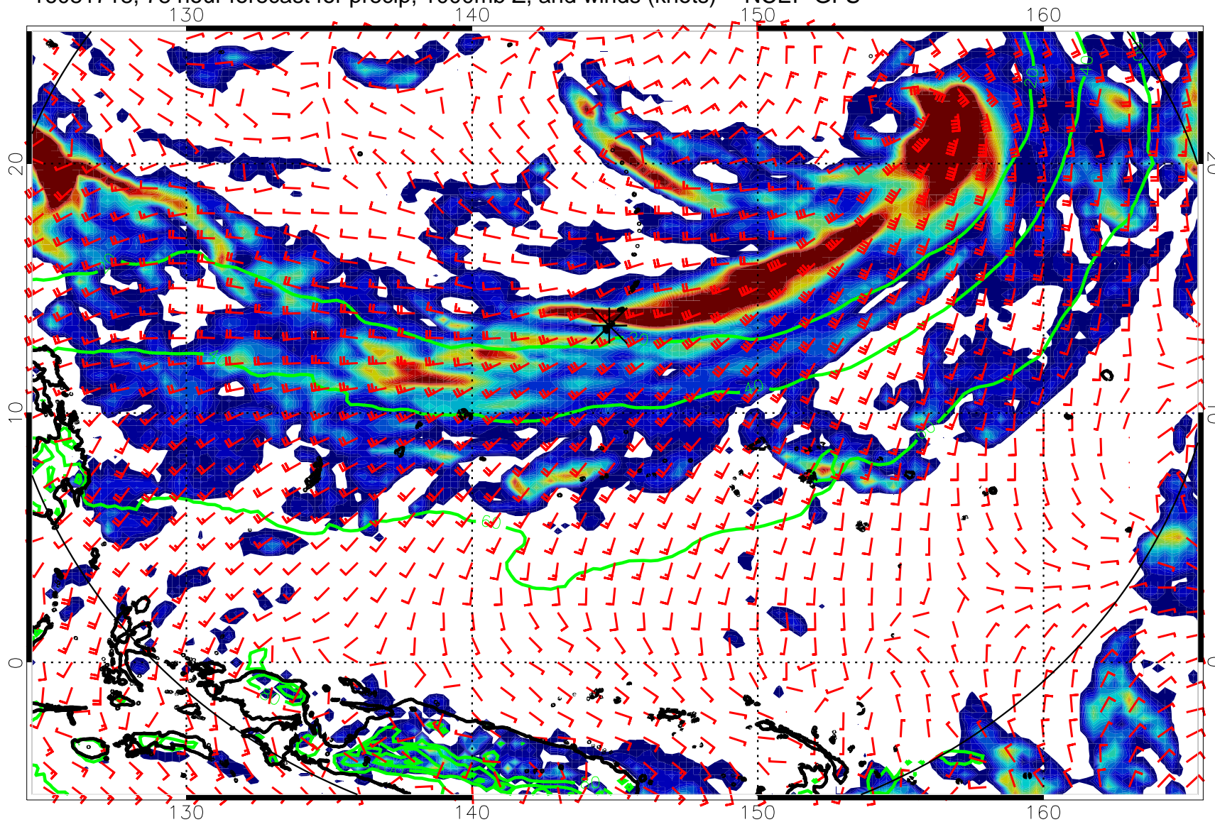
16081718, 78 hour forecast for precip, 1000mb Z, and winds (knots) -- NCEP GFS
