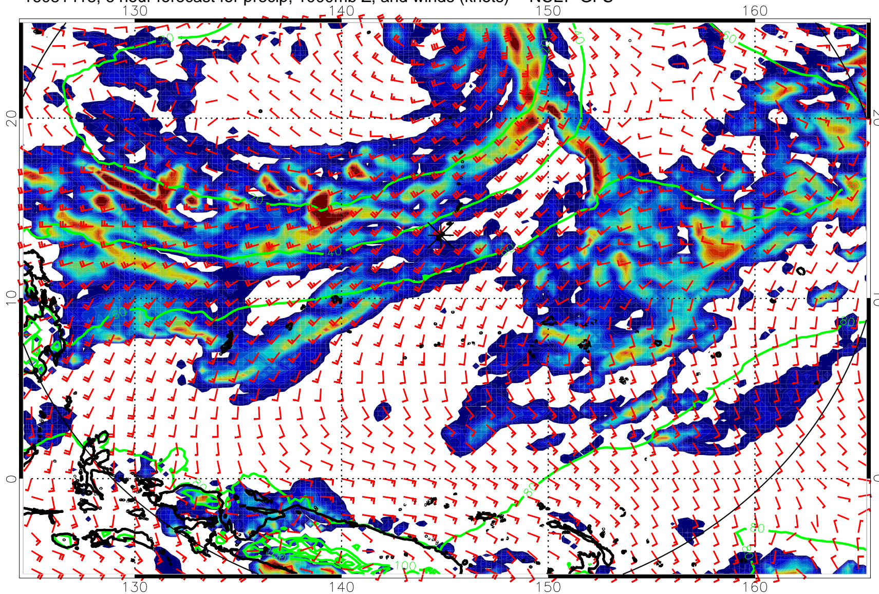
16081418, 6 hour forecast for precip, 1000mb Z, and winds (knots) -- NCEP GFS
