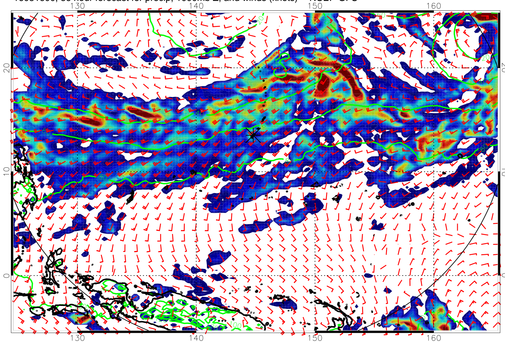
16081600, 36 hour forecast for precip, 1000mb Z, and winds (knots) -- NCEP GFS
