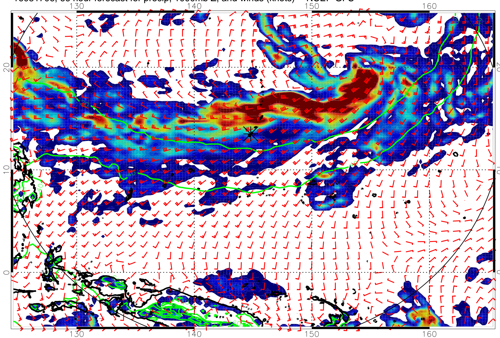
16081706, 66 hour forecast for precip, 1000mb Z, and winds (knots) -- NCEP GFS
