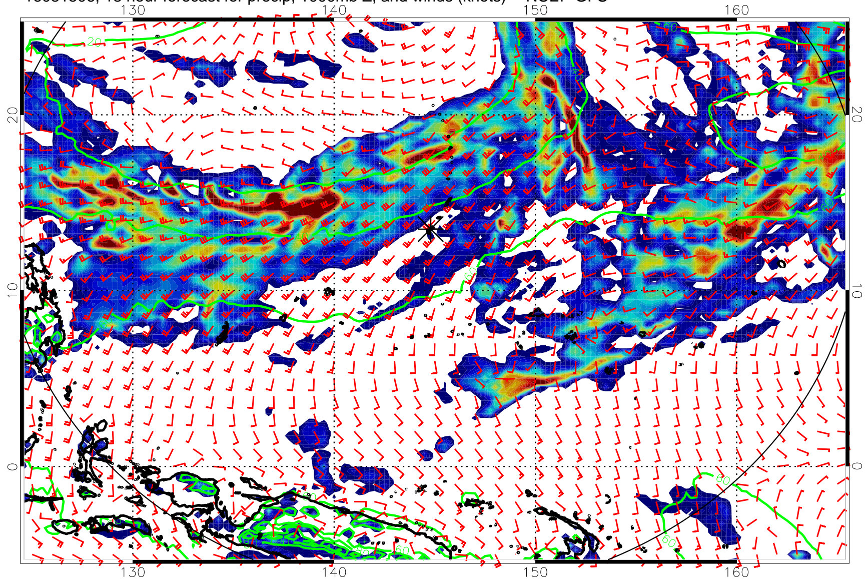
16081506, 18 hour forecast for precip, 1000mb Z, and winds (knots) -- NCEP GFS
