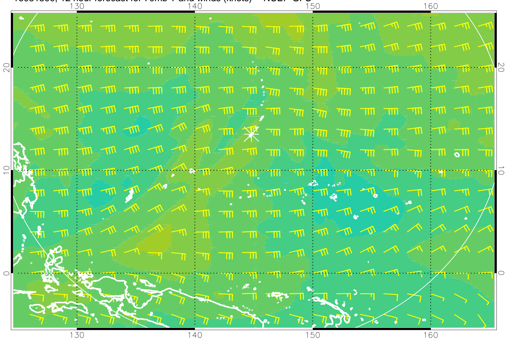
16081500, 12 hour forecast for 70mb T and winds (knots) -- NCEP GFS
