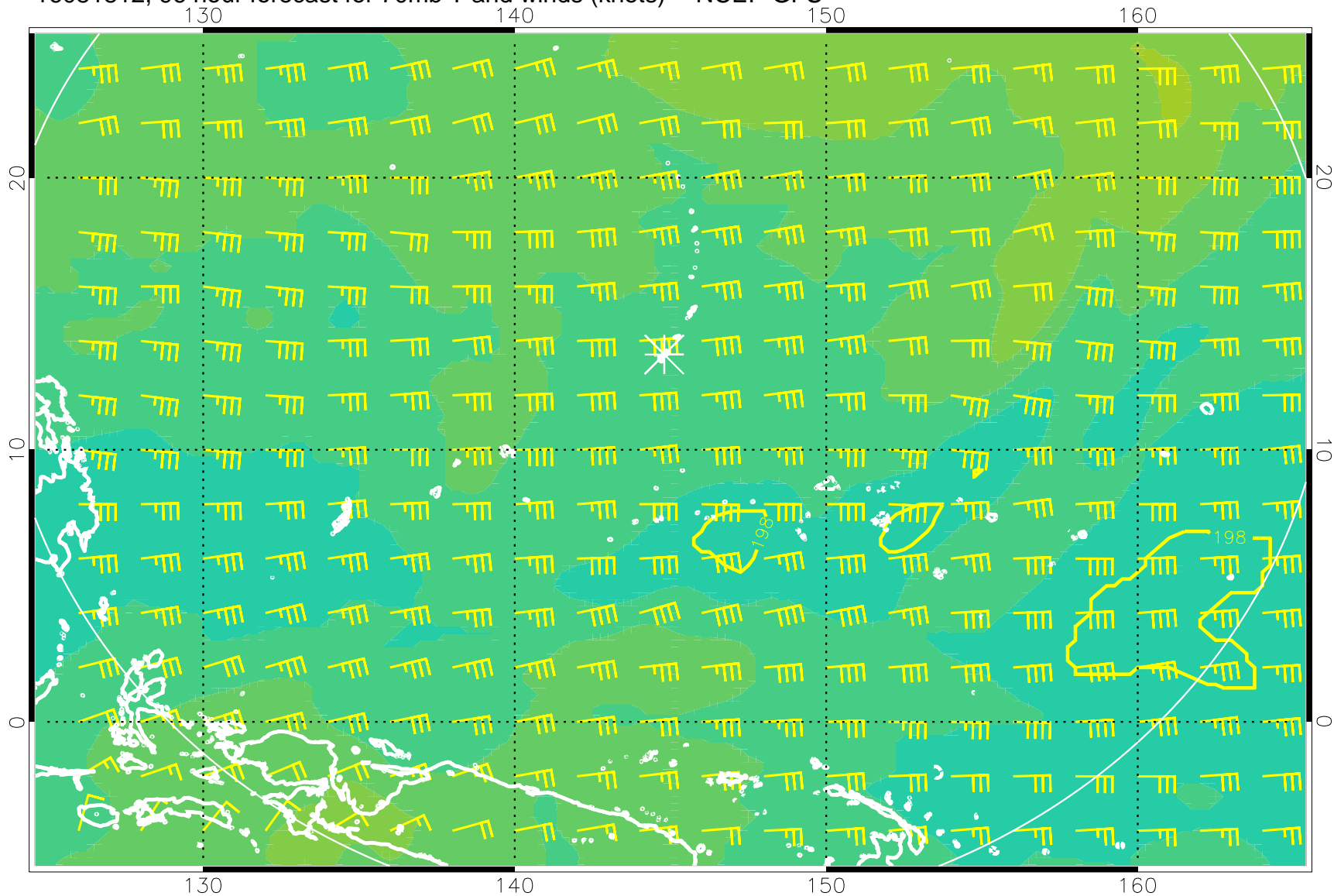
16081812, 96 hour forecast for 70mb T and winds (knots) -- NCEP GFS
