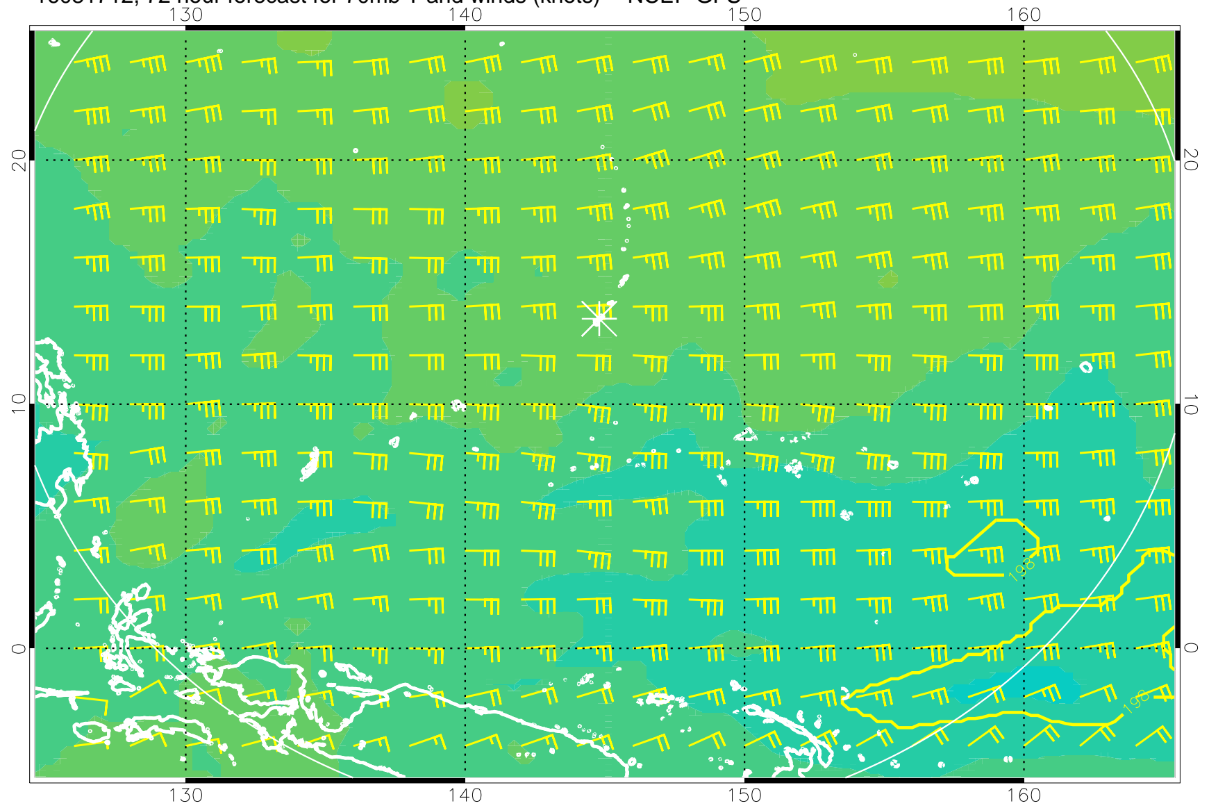
16081712, 72 hour forecast for 70mb T and winds (knots) -- NCEP GFS
