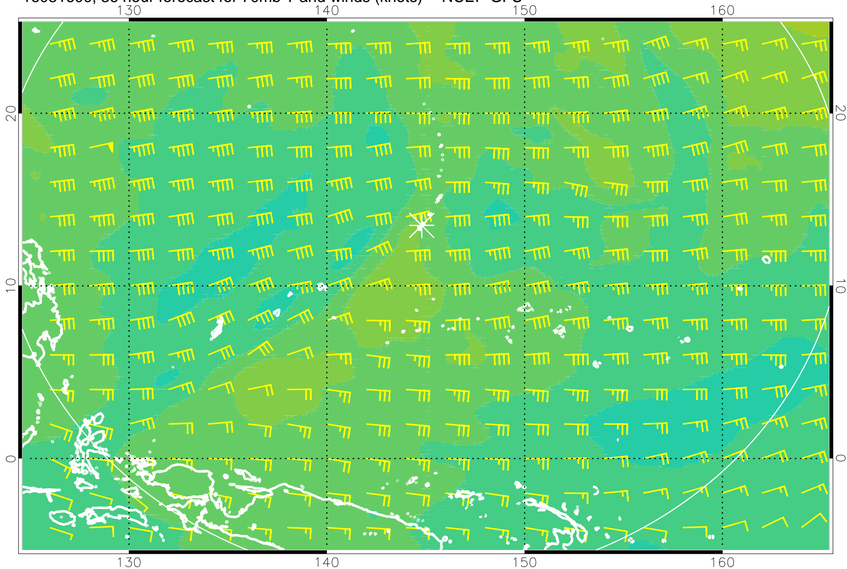
16081600, 36 hour forecast for 70mb T and winds (knots) -- NCEP GFS
