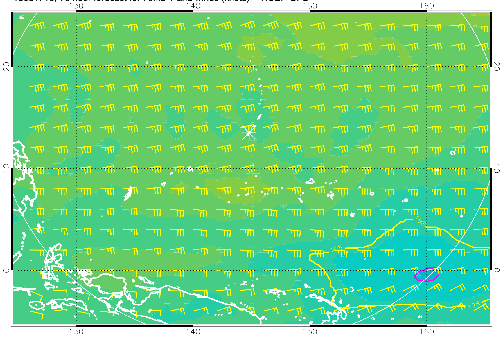
16081718, 78 hour forecast for 70mb T and winds (knots) -- NCEP GFS
