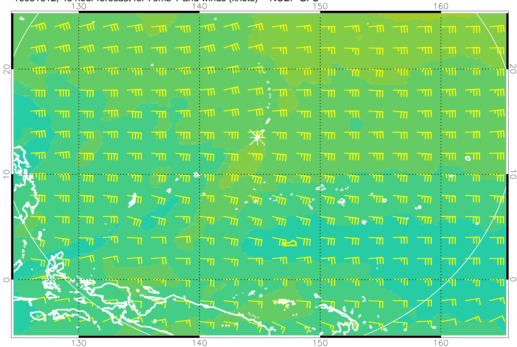
16081612, 48 hour forecast for 70mb T and winds (knots) -- NCEP GFS
