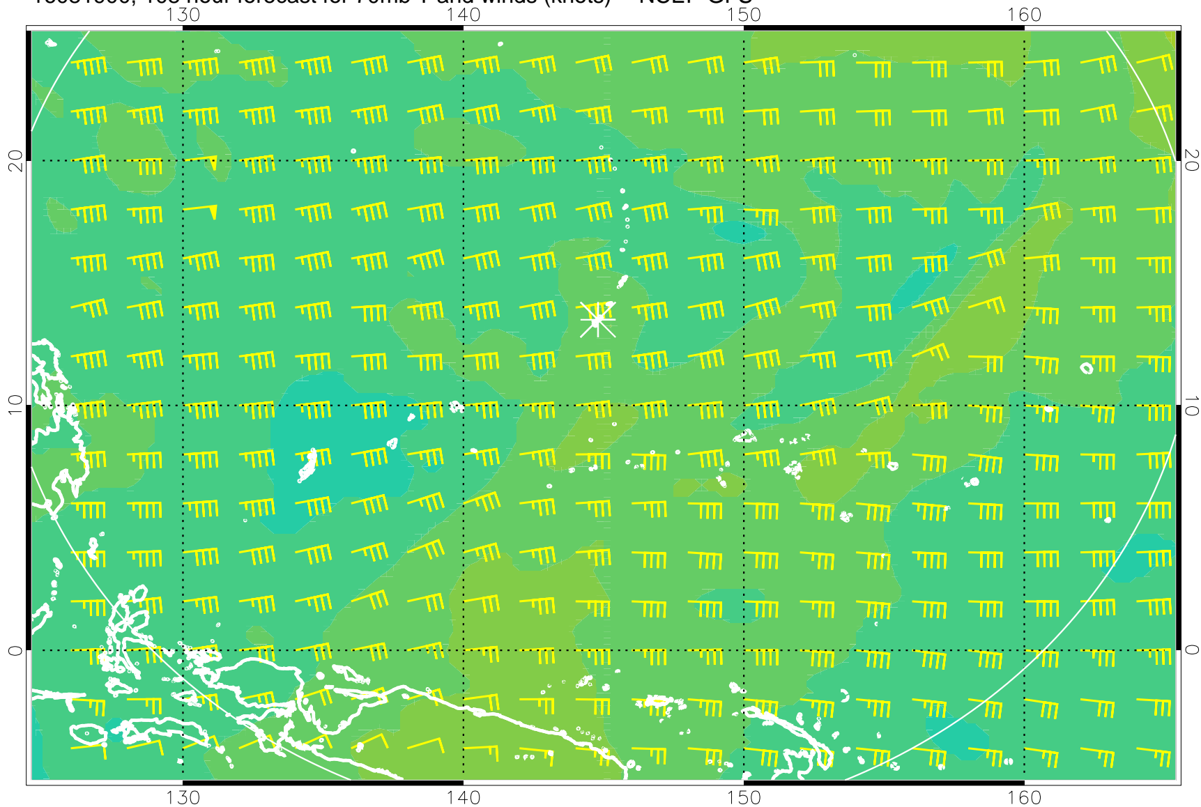
16081900, 108 hour forecast for 70mb T and winds (knots) -- NCEP GFS
