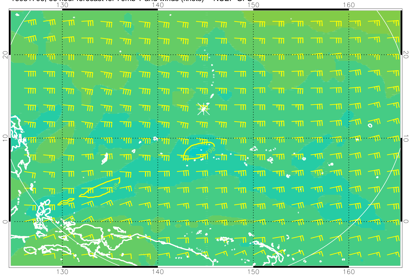
16081706, 66 hour forecast for 70mb T and winds (knots) -- NCEP GFS
