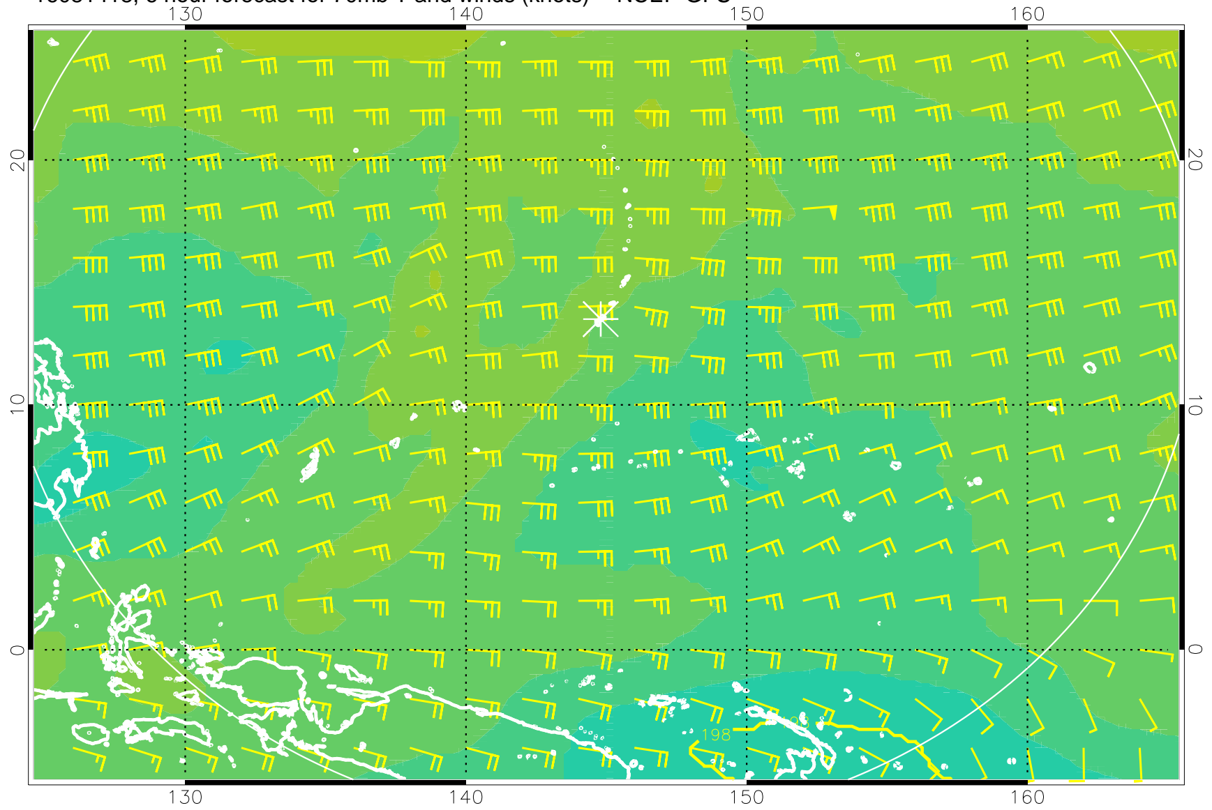
16081418, 6 hour forecast for 70mb T and winds (knots) -- NCEP GFS
