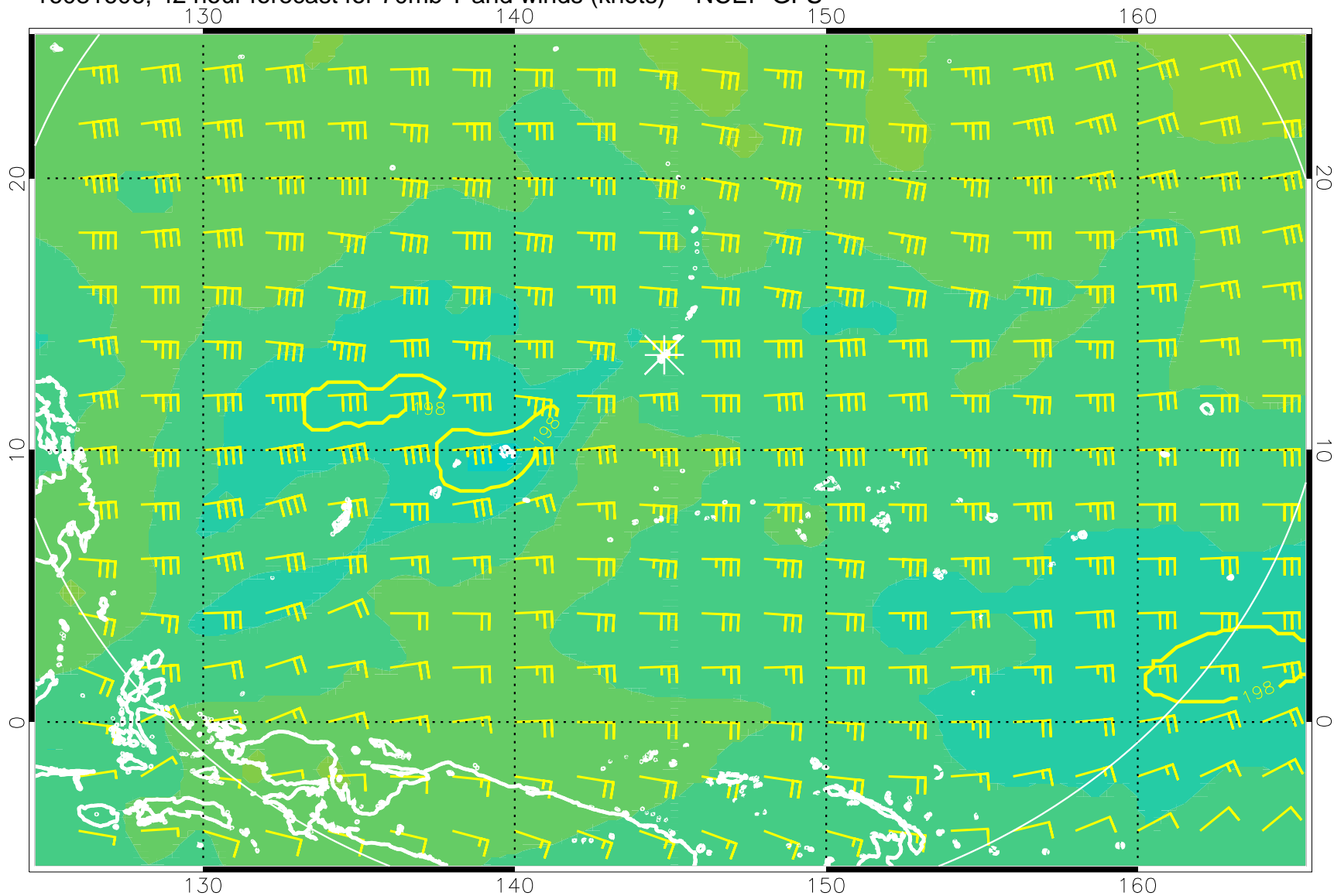
16081606, 42 hour forecast for 70mb T and winds (knots) -- NCEP GFS
