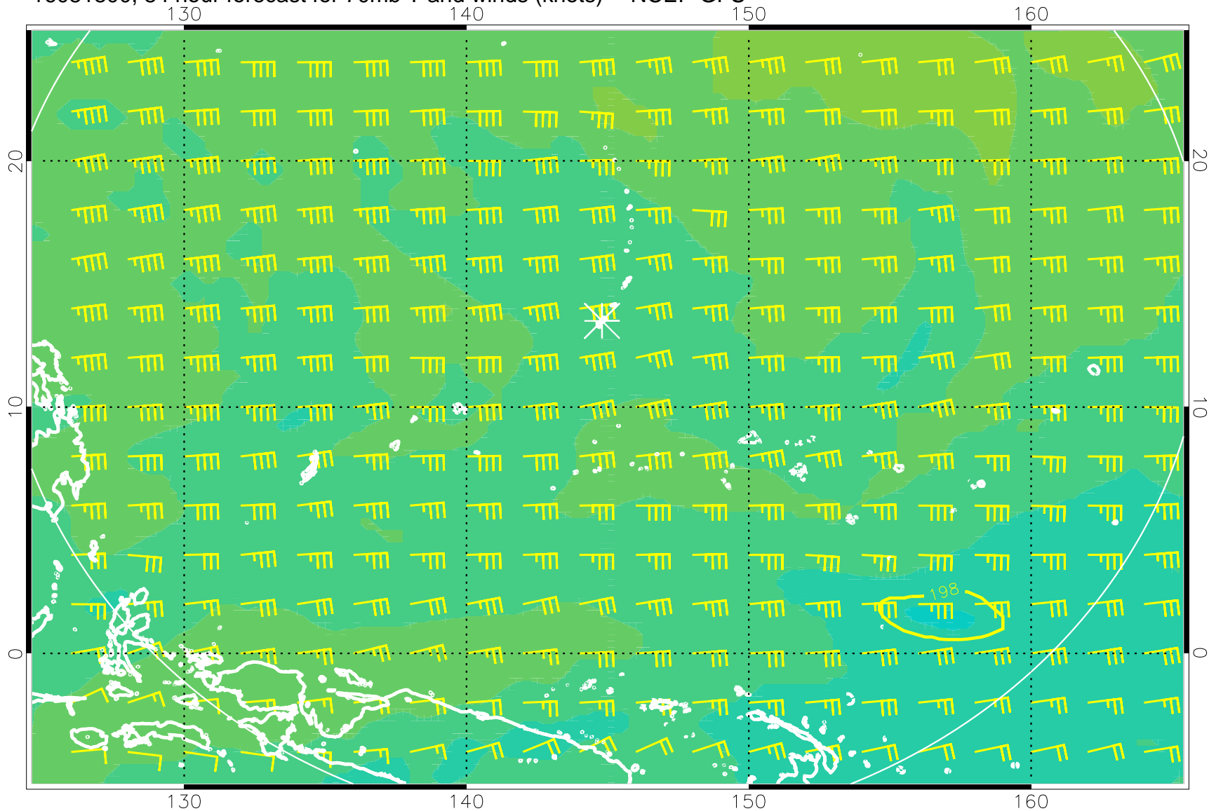
16081800, 84 hour forecast for 70mb T and winds (knots) -- NCEP GFS
