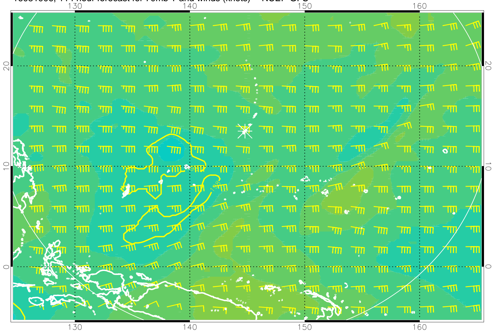
16081906, 114 hour forecast for 70mb T and winds (knots) -- NCEP GFS
