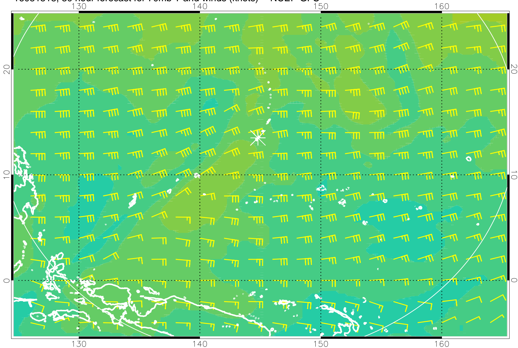
16081518, 30 hour forecast for 70mb T and winds (knots) -- NCEP GFS
