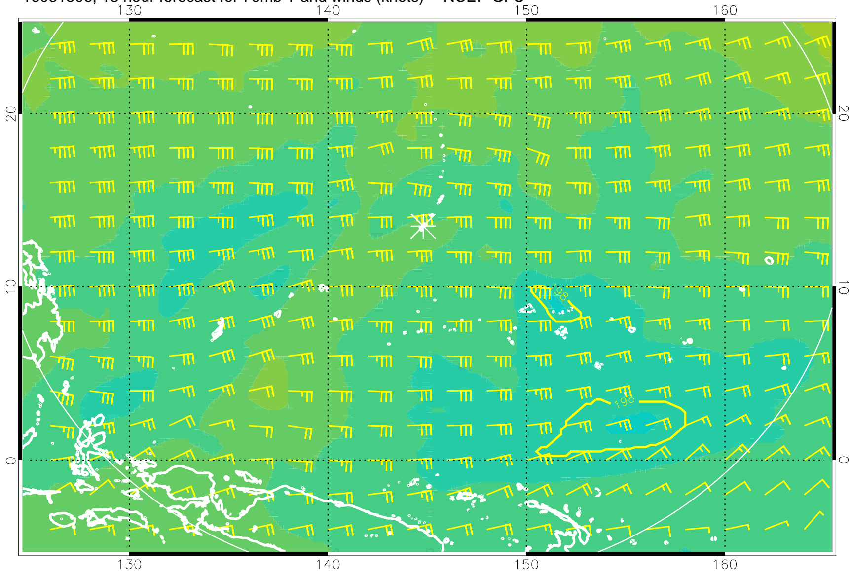
16081506, 18 hour forecast for 70mb T and winds (knots) -- NCEP GFS
