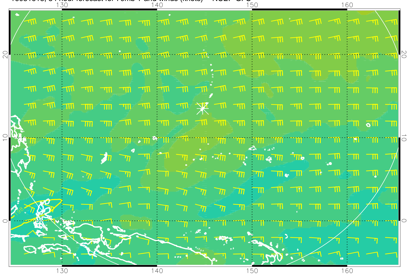
16081618, 54 hour forecast for 70mb T and winds (knots) -- NCEP GFS
