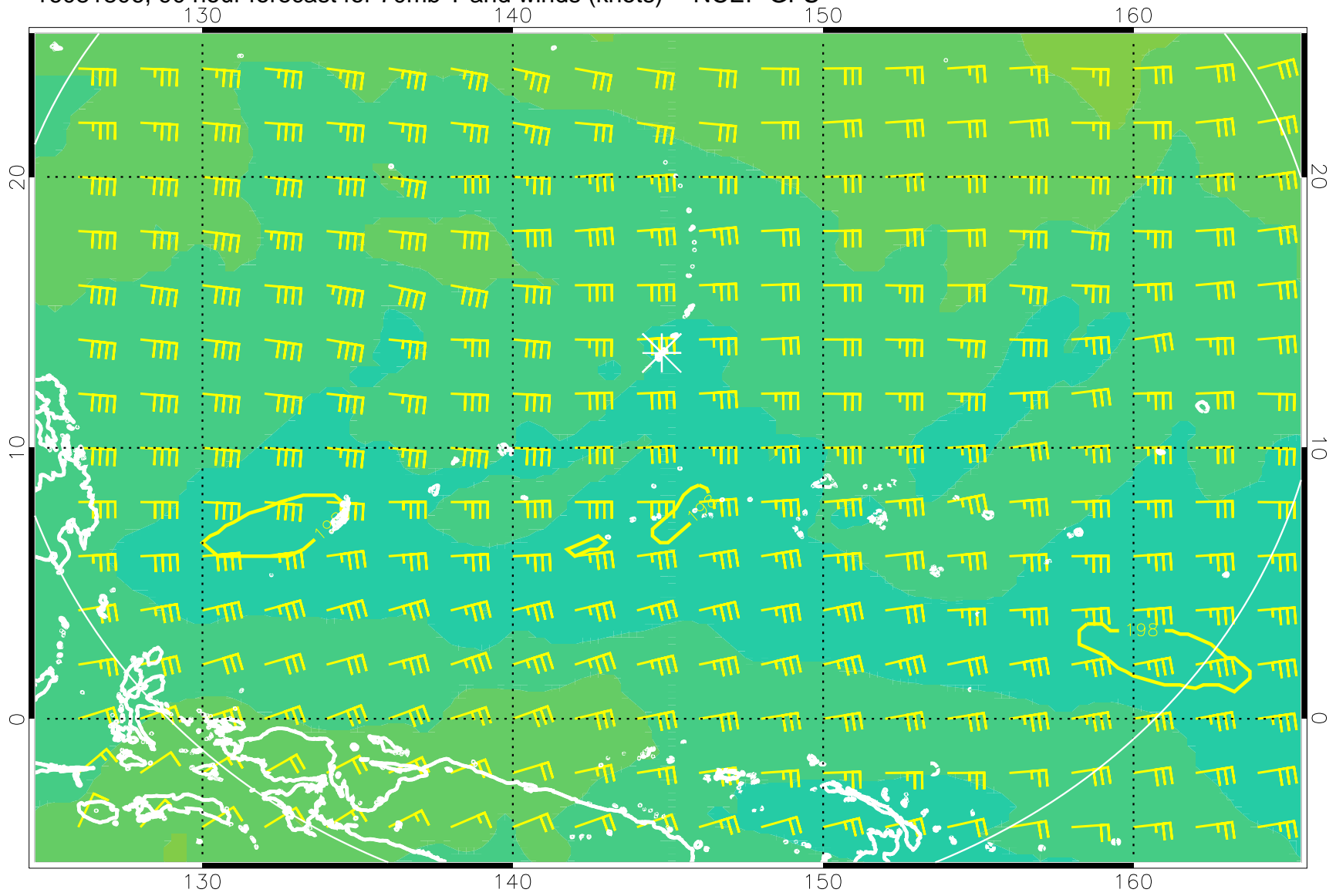
16081806, 90 hour forecast for 70mb T and winds (knots) -- NCEP GFS
