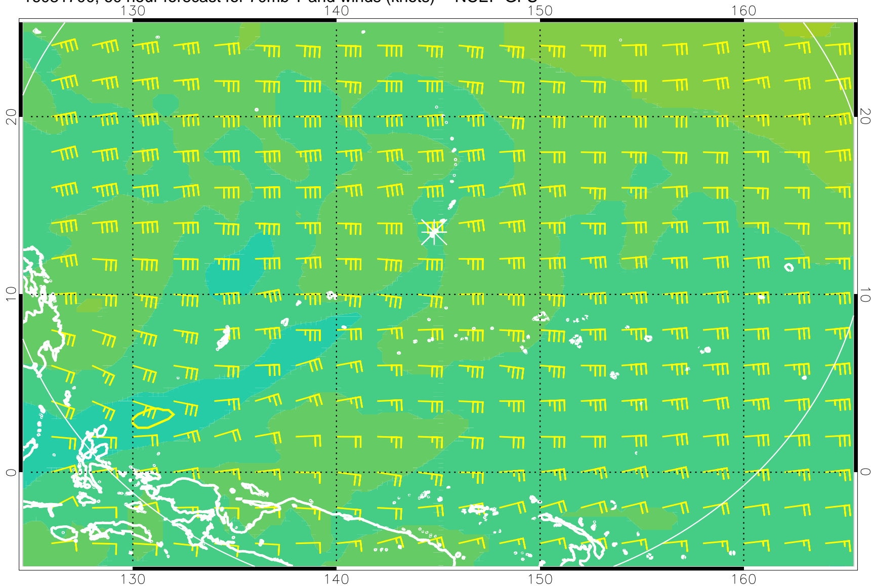
16081700, 60 hour forecast for 70mb T and winds (knots) -- NCEP GFS
