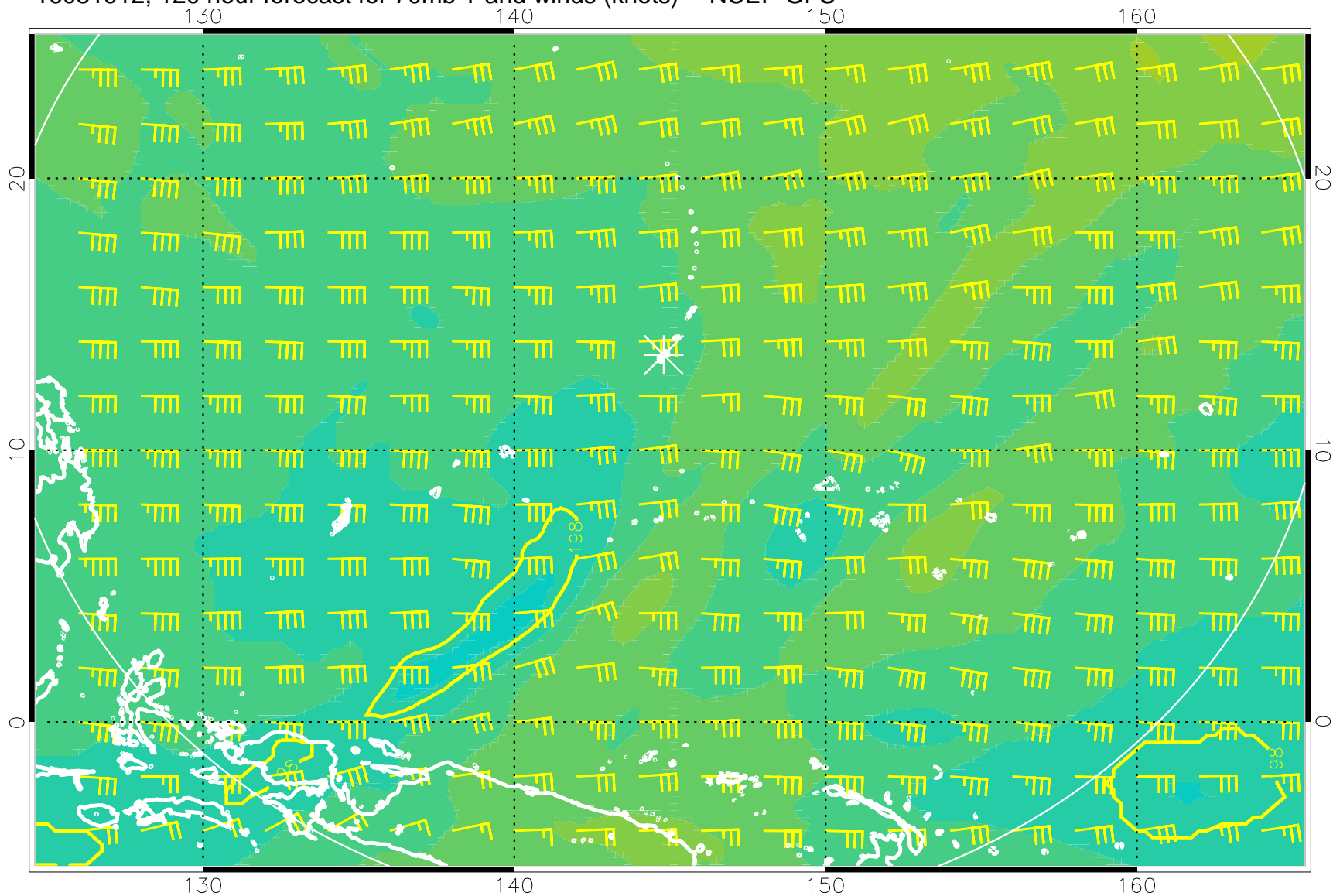
16081912, 120 hour forecast for 70mb T and winds (knots) -- NCEP GFS
