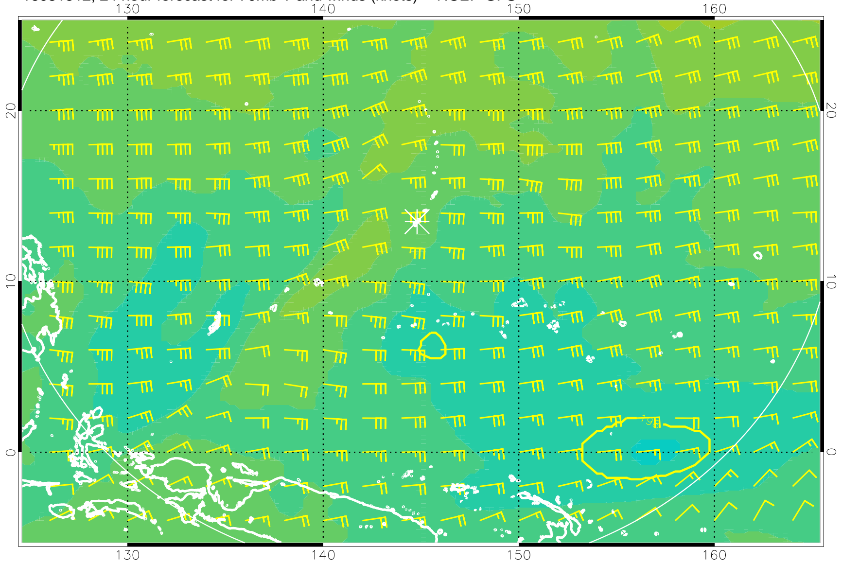
16081512, 24 hour forecast for 70mb T and winds (knots) -- NCEP GFS
