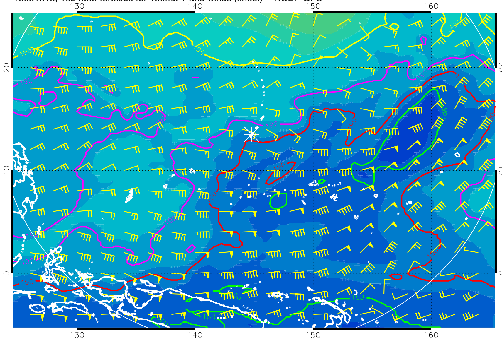
16081818, 102 hour forecast for 100mb T and winds (knots) -- NCEP GFS
