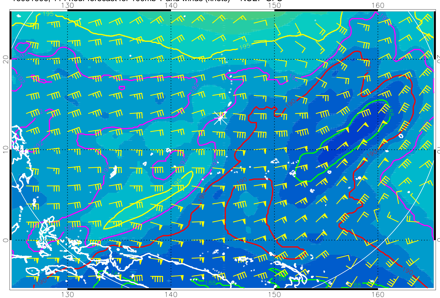
16081906, 114 hour forecast for 100mb T and winds (knots) -- NCEP GFS
