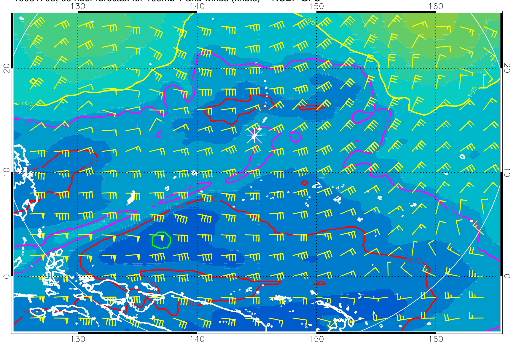
16081700, 60 hour forecast for 100mb T and winds (knots) -- NCEP GFS
