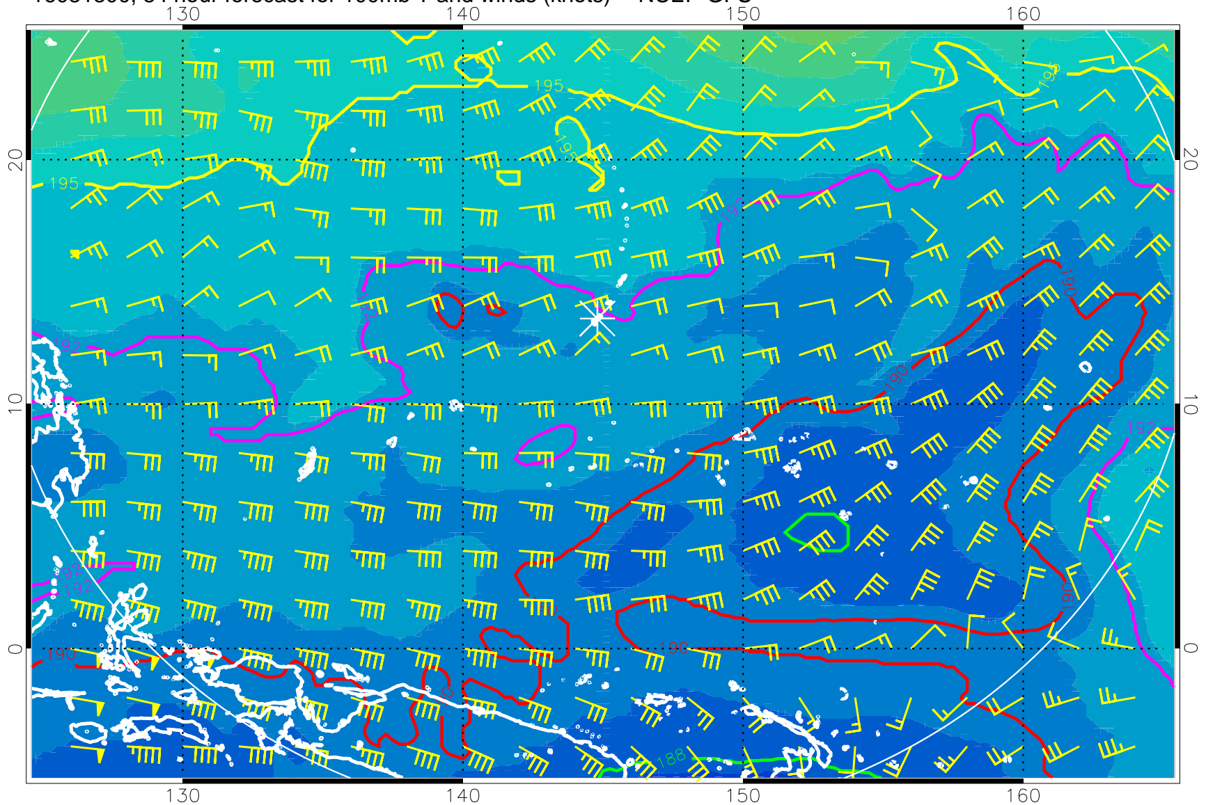
16081800, 84 hour forecast for 100mb T and winds (knots) -- NCEP GFS
