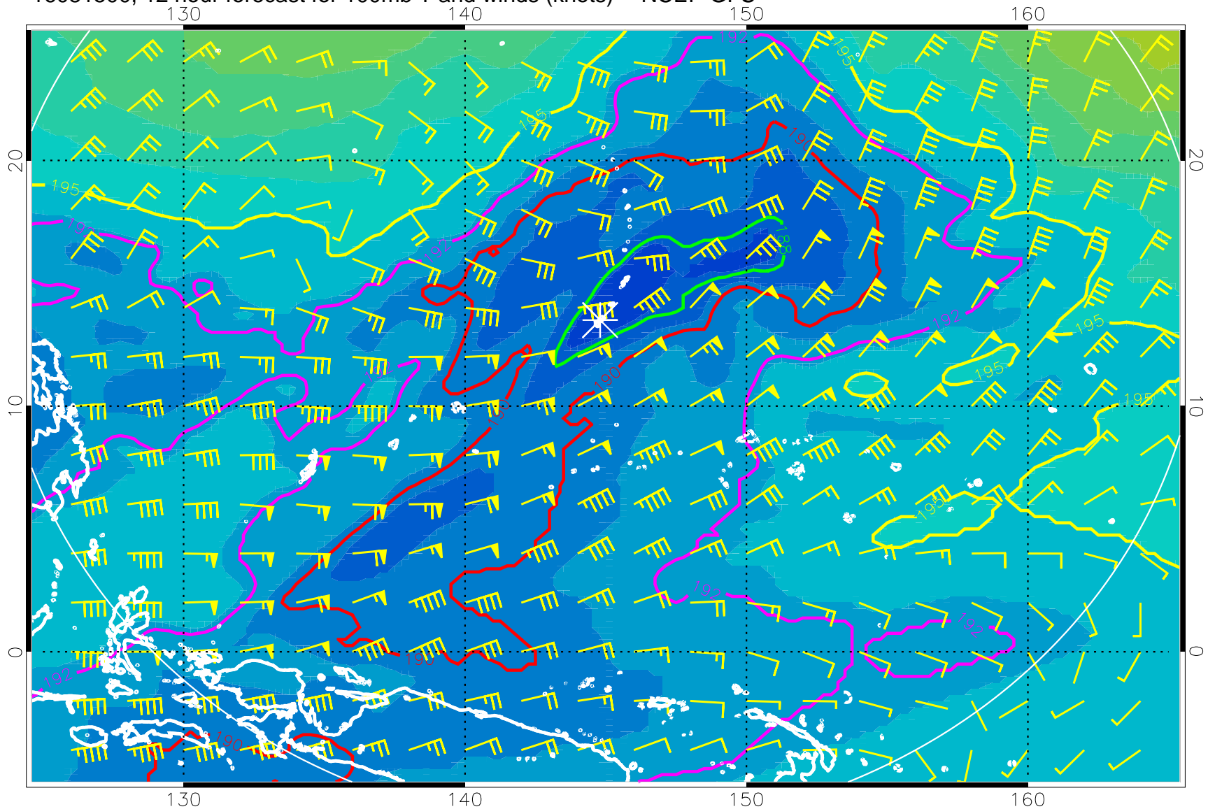
16081500, 12 hour forecast for 100mb T and winds (knots) -- NCEP GFS
