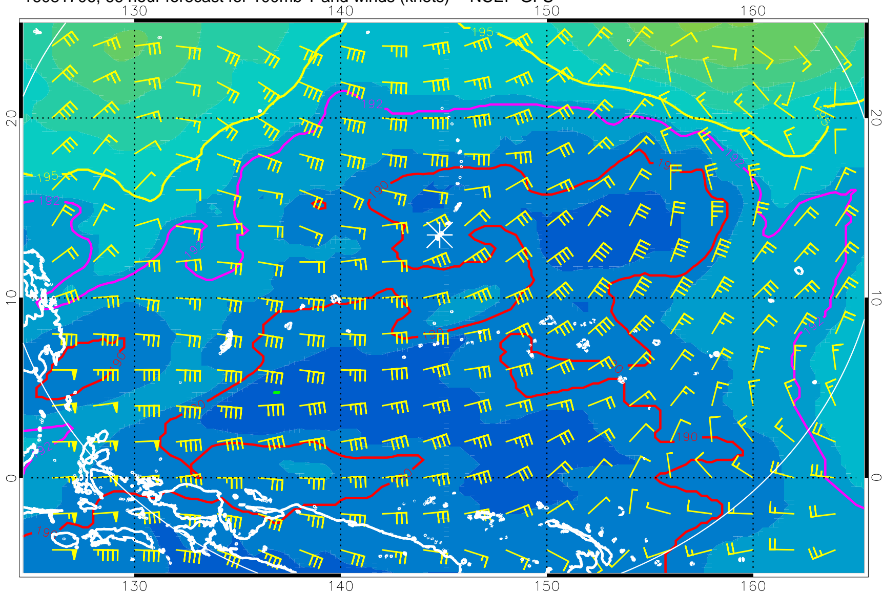
16081706, 66 hour forecast for 100mb T and winds (knots) -- NCEP GFS
