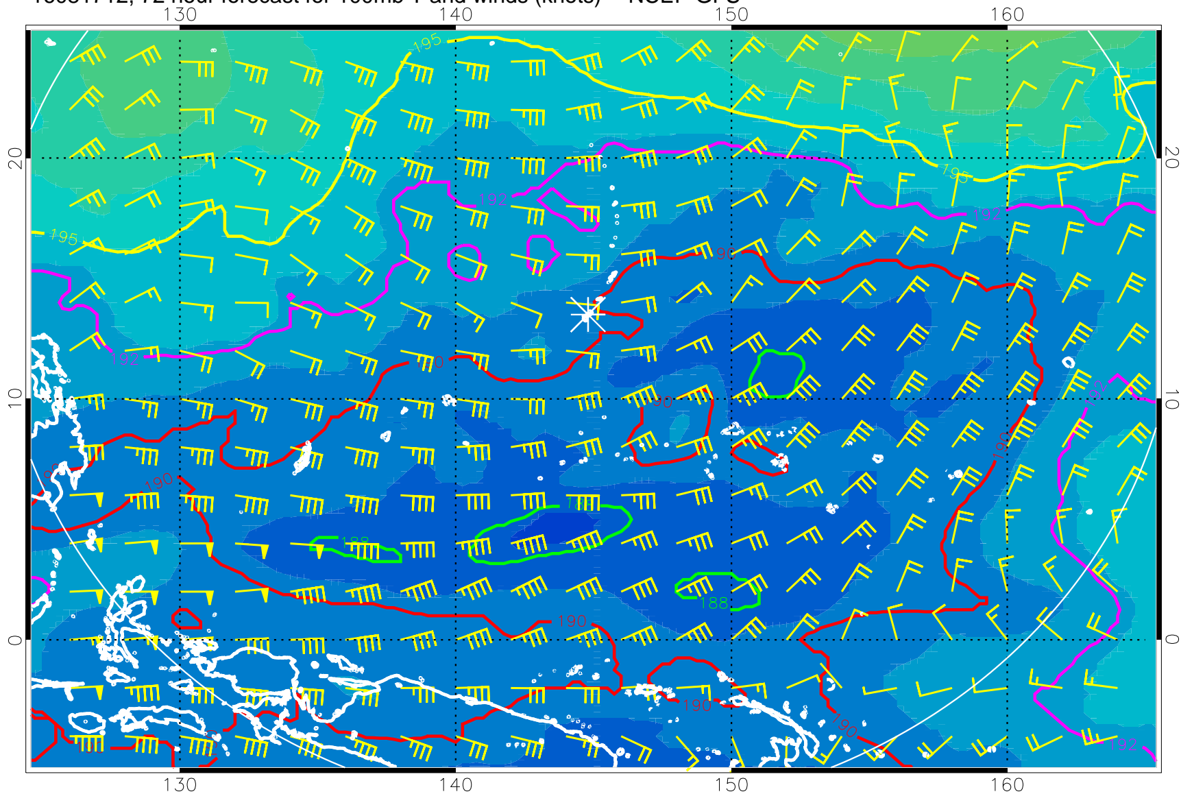
16081712, 72 hour forecast for 100mb T and winds (knots) -- NCEP GFS
