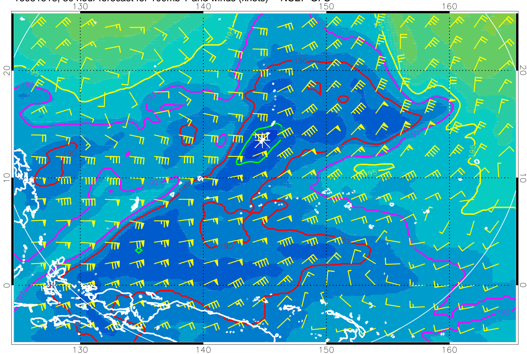
16081518, 30 hour forecast for 100mb T and winds (knots) -- NCEP GFS
