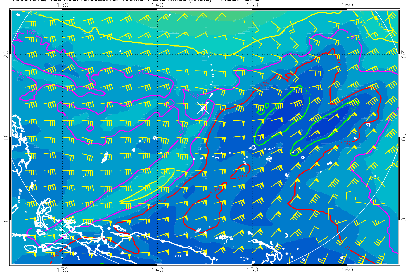
16081912, 120 hour forecast for 100mb T and winds (knots) -- NCEP GFS
