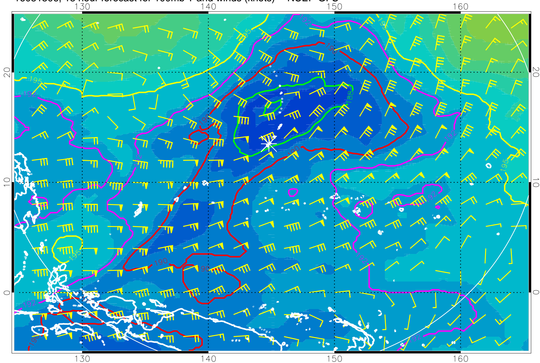
16081506, 18 hour forecast for 100mb T and winds (knots) -- NCEP GFS
