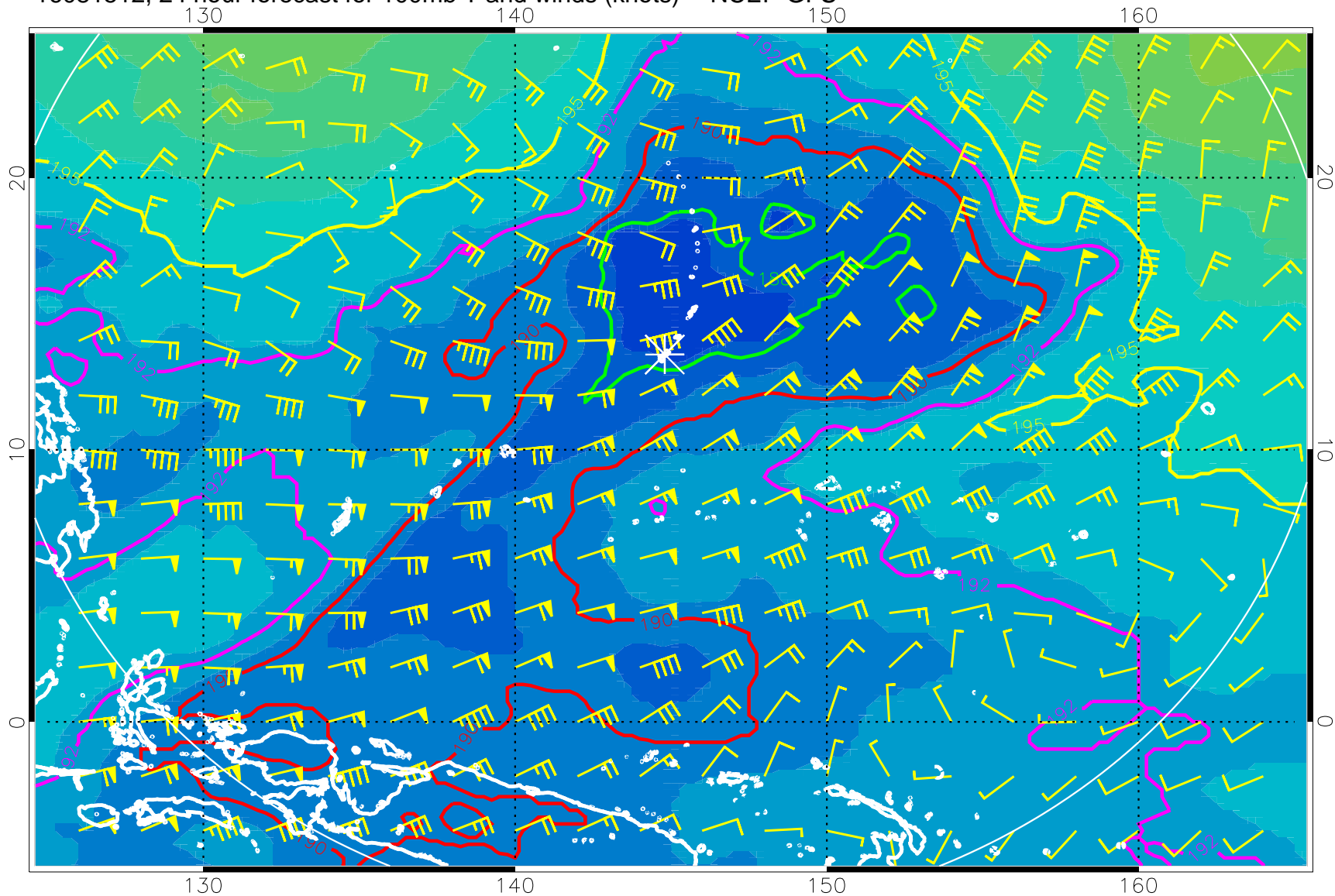
16081512, 24 hour forecast for 100mb T and winds (knots) -- NCEP GFS
