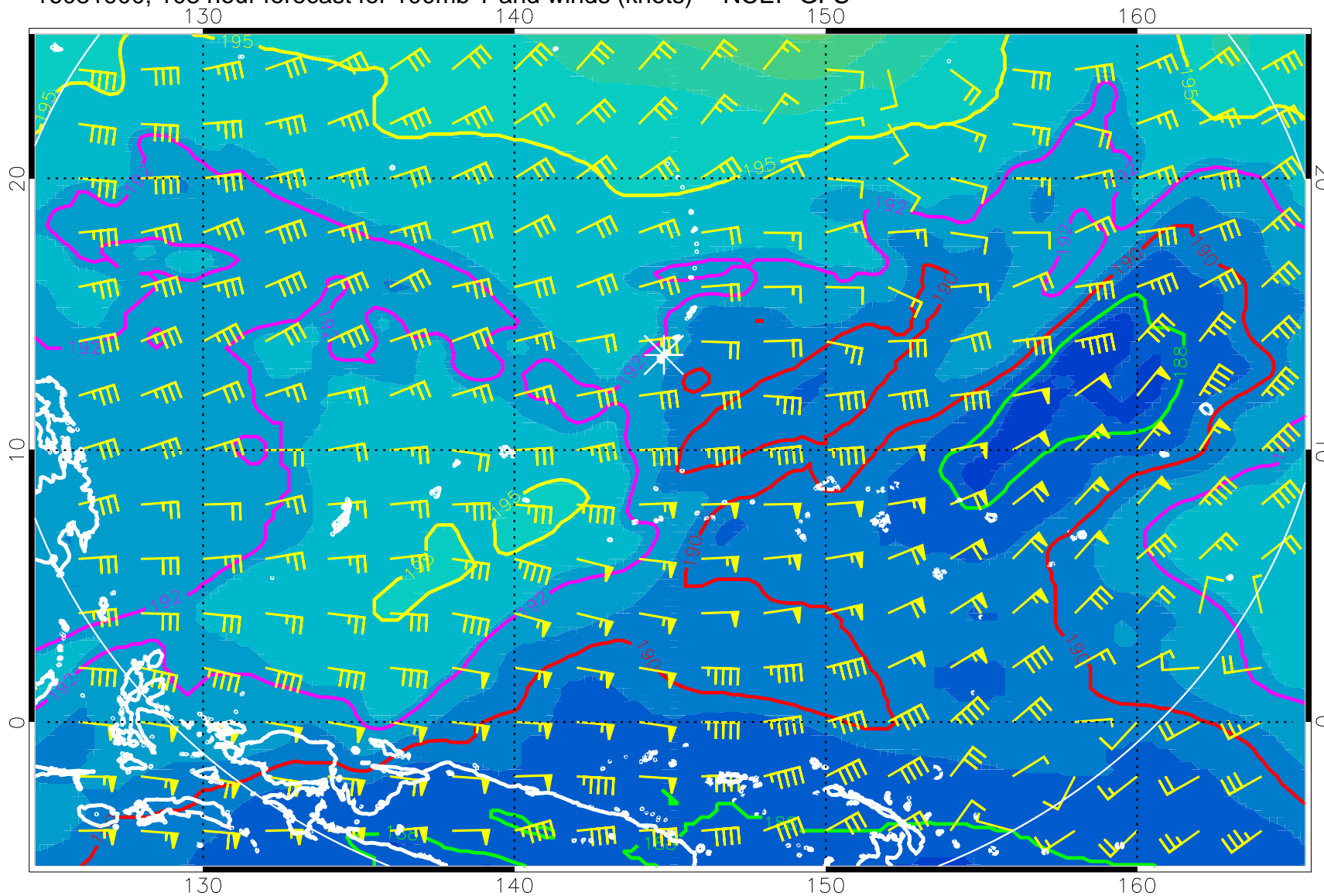
16081900, 108 hour forecast for 100mb T and winds (knots) -- NCEP GFS
