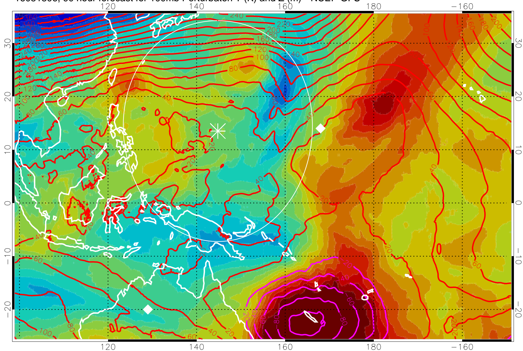
16081806, 90 hour forecast for 100mb Perturbaton T (K) and Z (m)-- NCEP GFS
