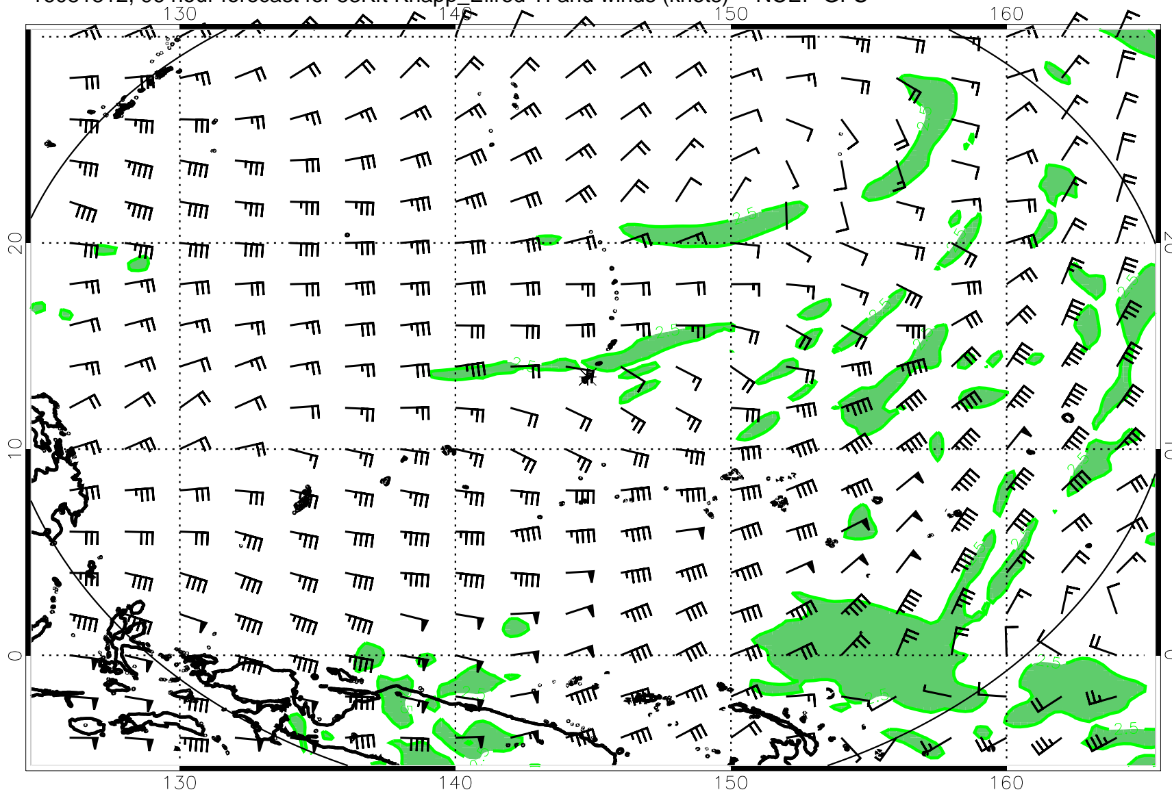
16081812, 96 hour forecast for 53Kft Knapp_Ellrod TI and winds (knots) -- NCEP GFS
