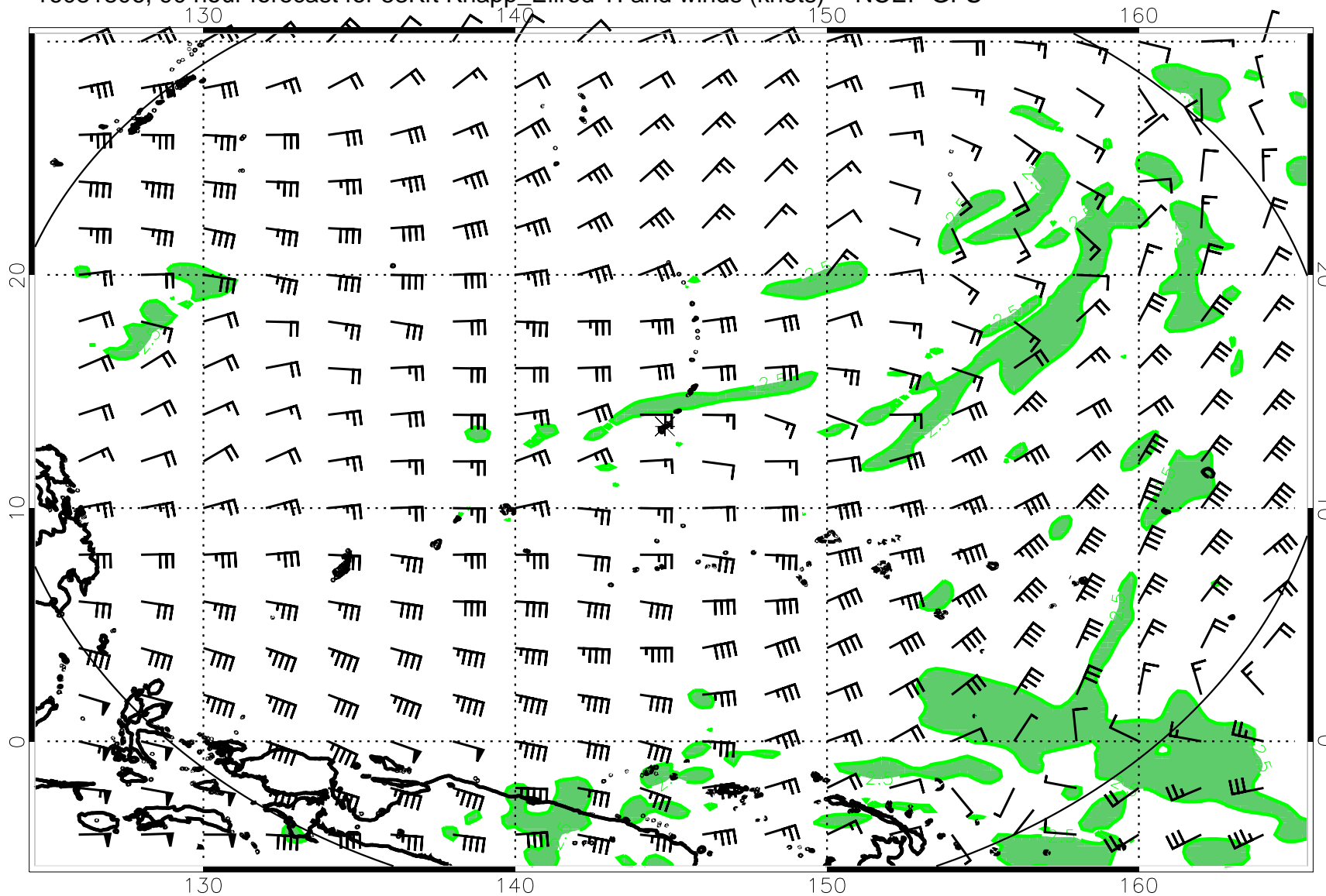
16081806, 90 hour forecast for 53Kft Knapp_Ellrod TI and winds (knots) -- NCEP GFS
