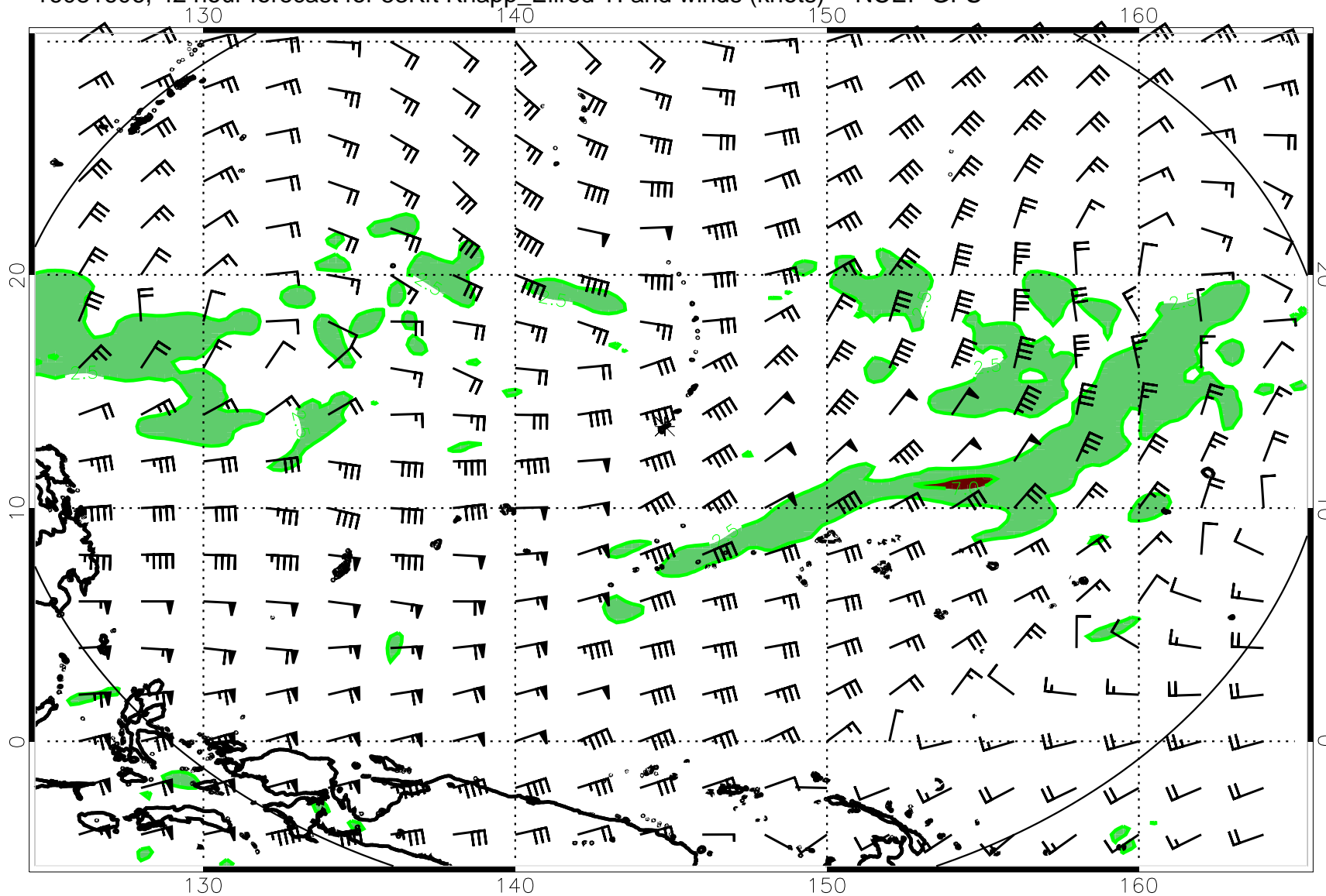
16081606, 42 hour forecast for 53Kft Knapp_Ellrod TI and winds (knots) -- NCEP GFS
