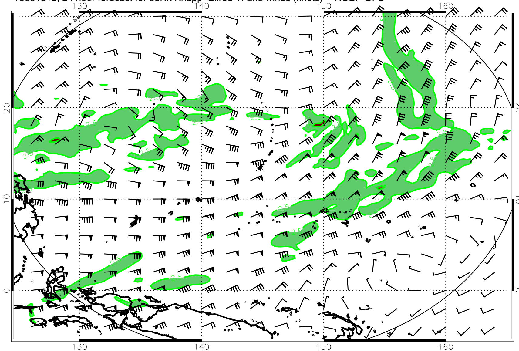
16081512, 24 hour forecast for 53Kft Knapp_Ellrod TI and winds (knots) -- NCEP GFS
