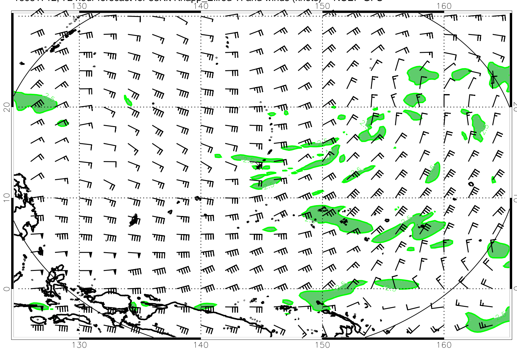
16081712, 72 hour forecast for 53Kft Knapp_Ellrod TI and winds (knots) -- NCEP GFS
