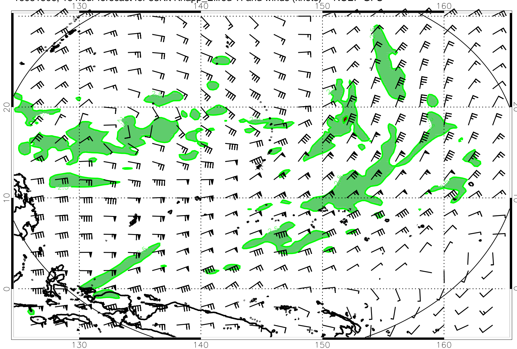
16081506, 18 hour forecast for 53Kft Knapp_Ellrod TI and winds (knots) -- NCEP GFS
