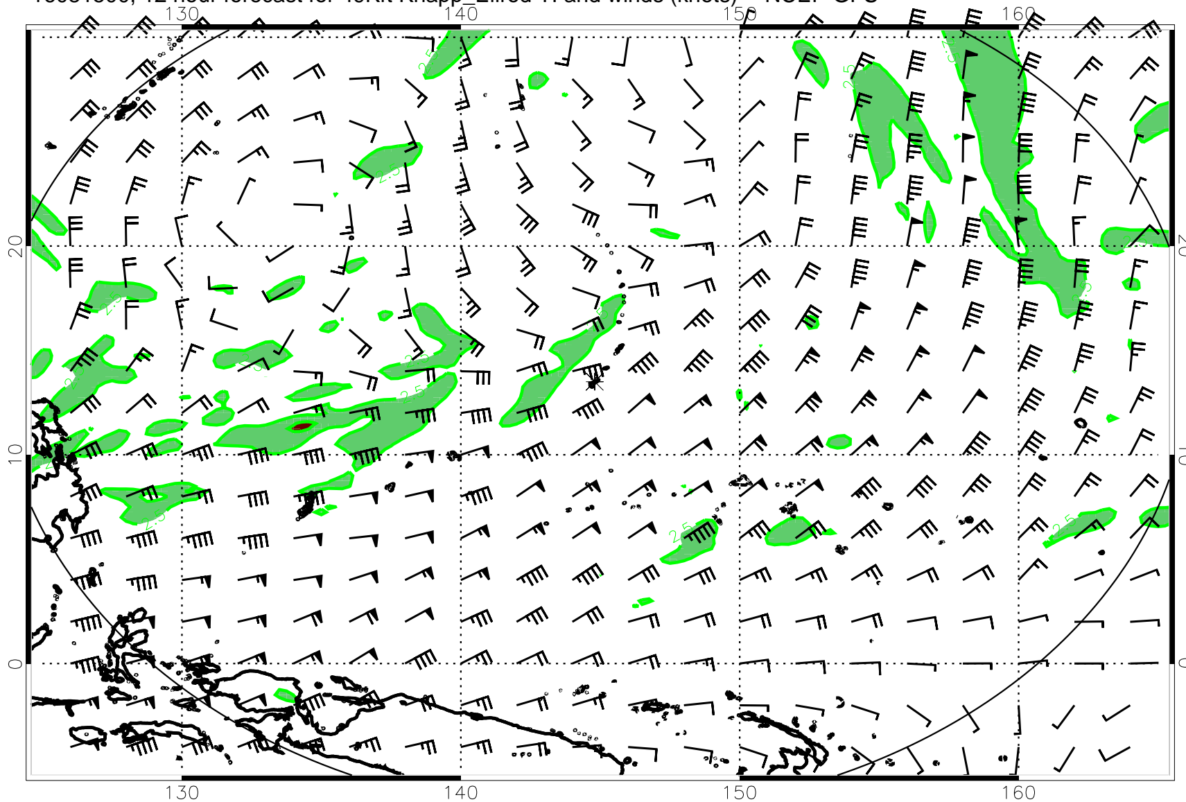
16081500, 12 hour forecast for 49Kft Knapp_Ellrod TI and winds (knots) -- NCEP GFS
