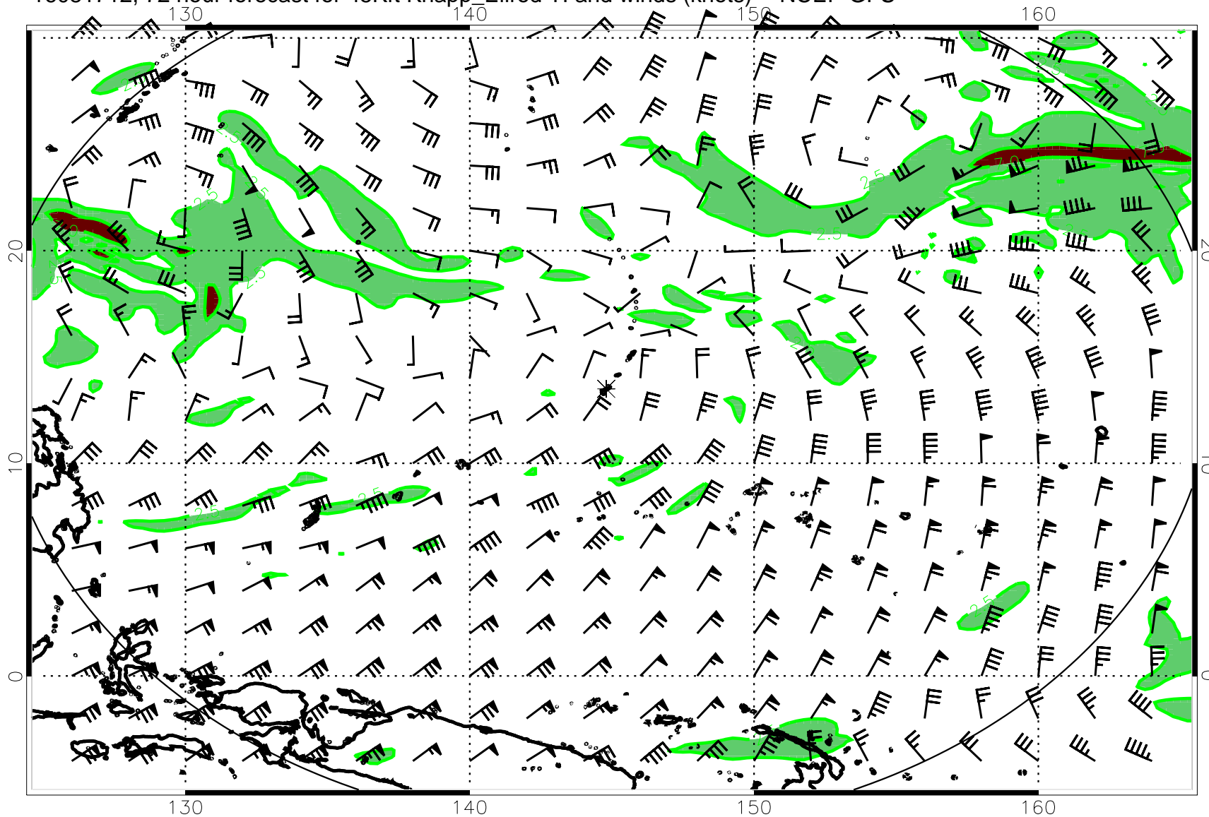
16081712, 72 hour forecast for 45Kft Knapp_Ellrod TI and winds (knots) -- NCEP GFS
