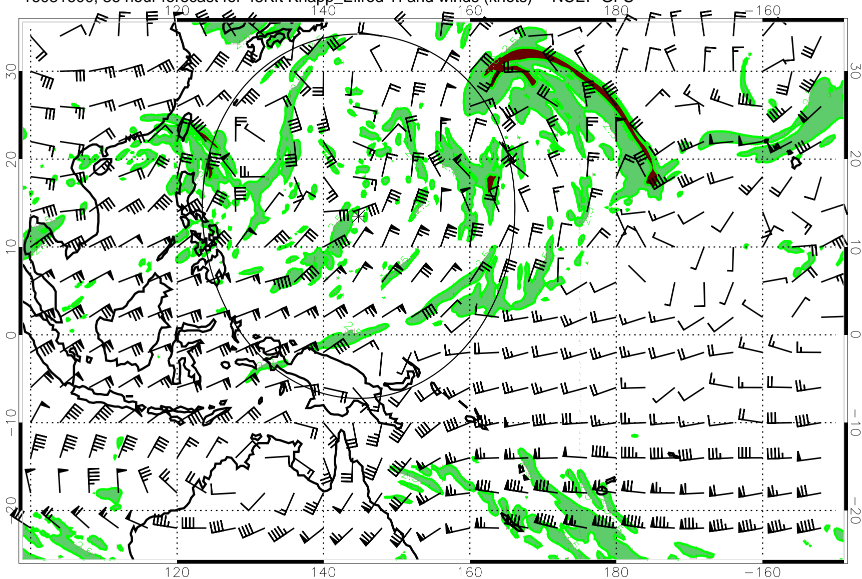
16081600, 36 hour forecast for 45Kft Knapp_Ellrod TI and winds (knots) -- NCEP GFS
