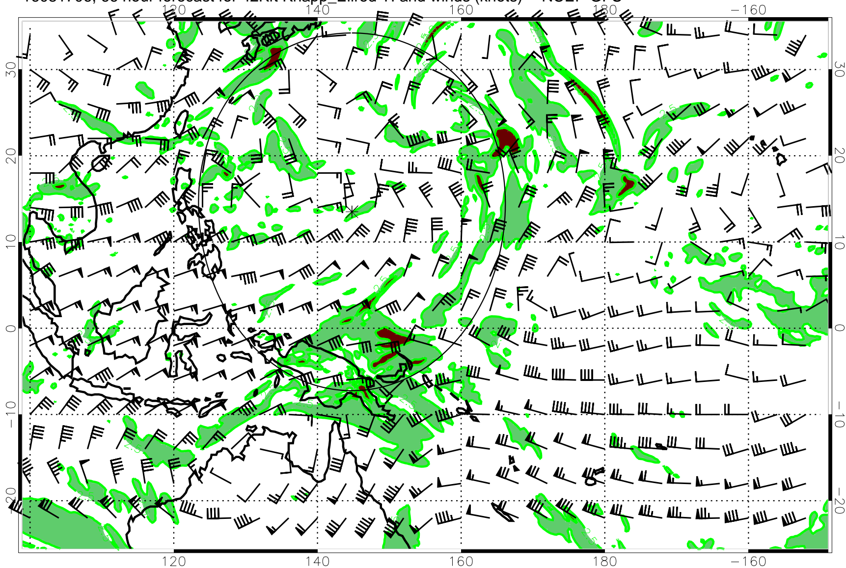
16081706, 66 hour forecast for 42Kft Knapp_Ellrod TI and winds (knots) -- NCEP GFS
