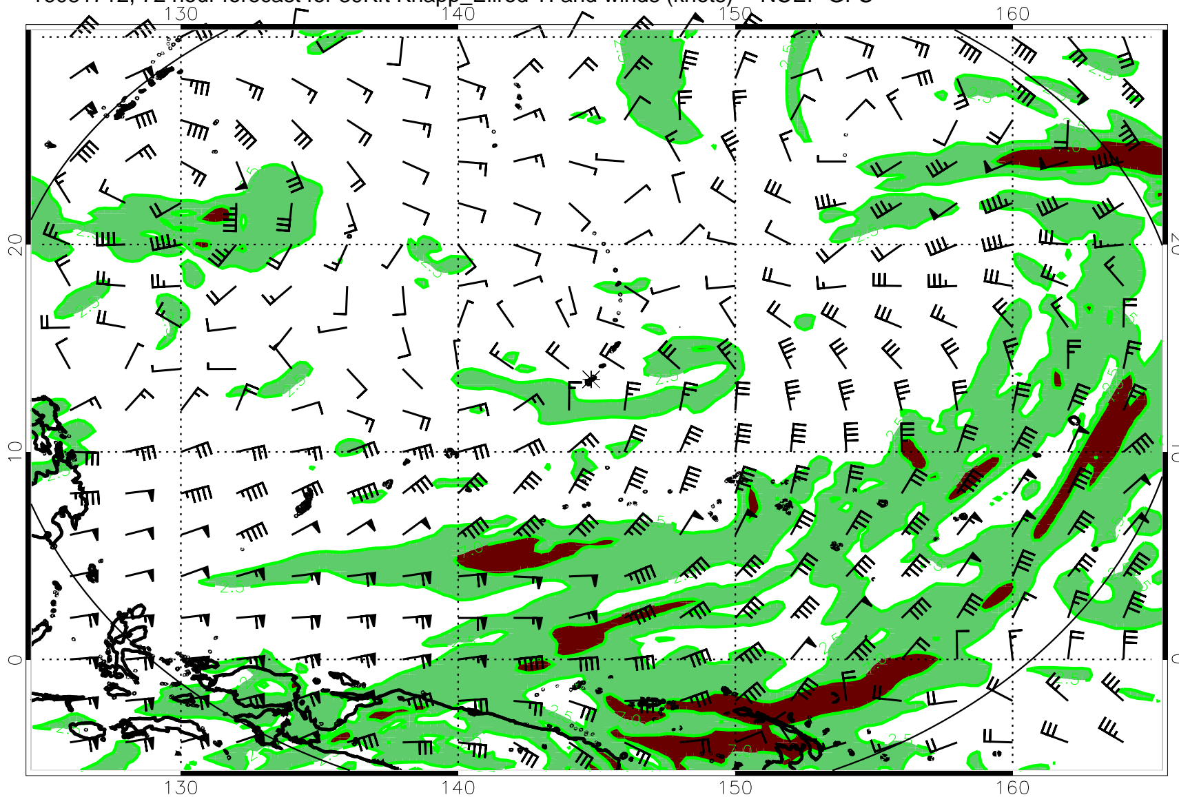
16081712, 72 hour forecast for 39Kft Knapp_Ellrod TI and winds (knots) -- NCEP GFS
