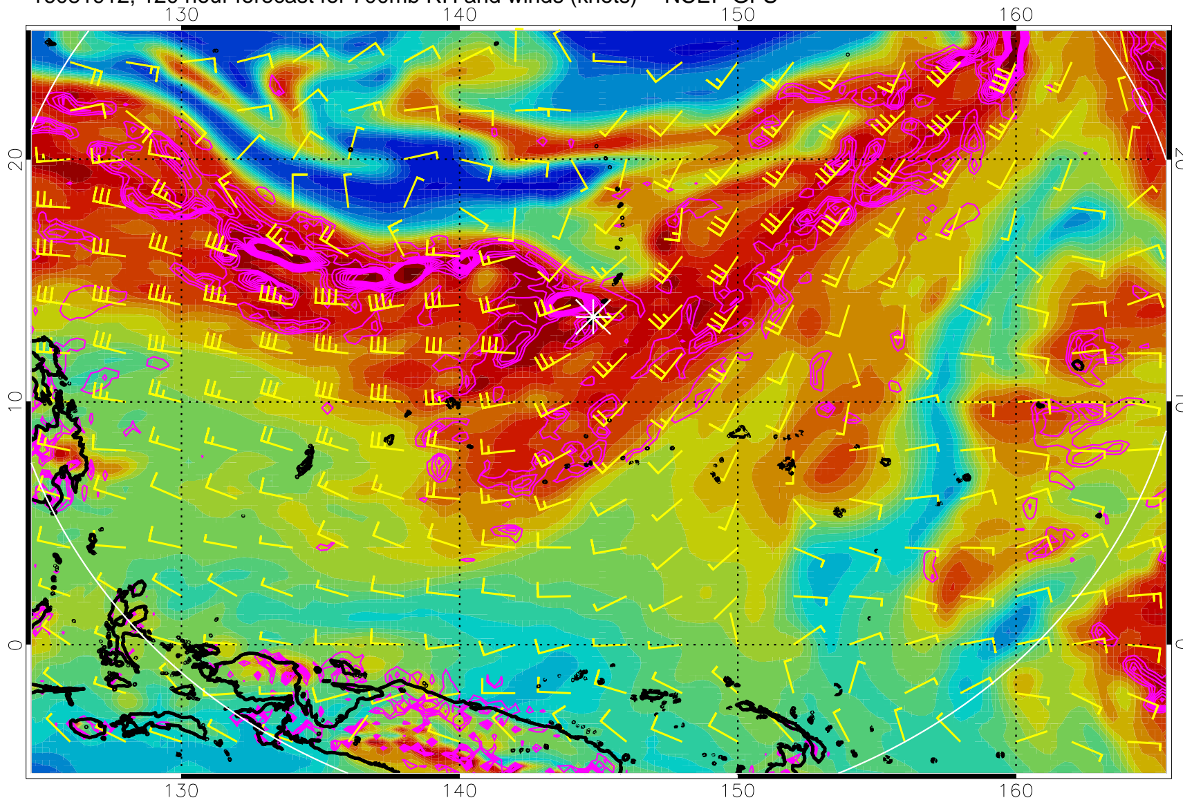
16081912, 120 hour forecast for 700mb RH and winds (knots) -- NCEP GFS
