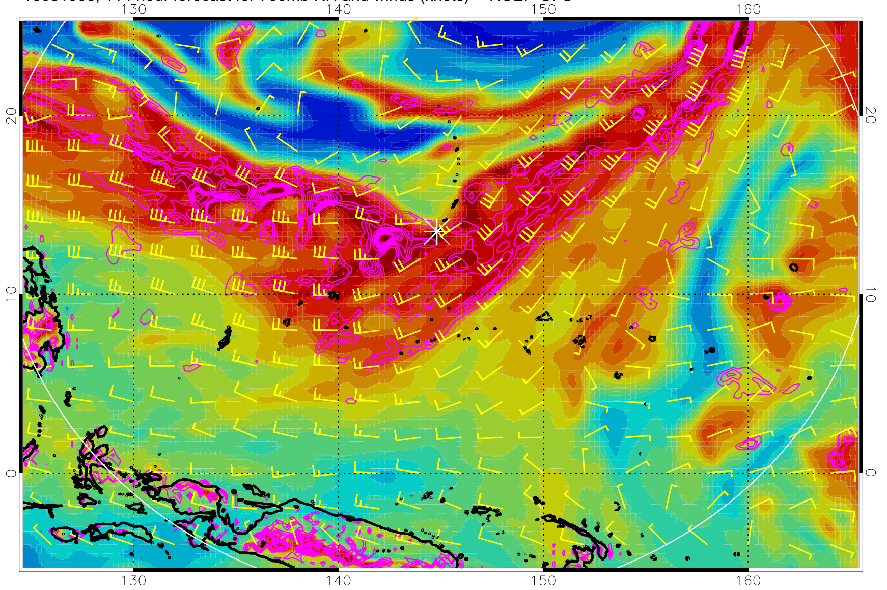
16081906, 114 hour forecast for 700mb RH and winds (knots) -- NCEP GFS
