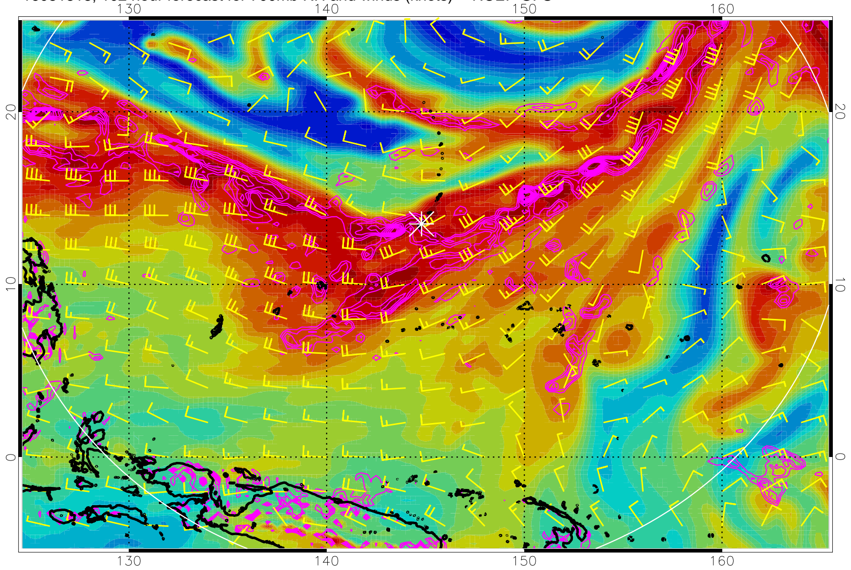
16081818, 102 hour forecast for 700mb RH and winds (knots) -- NCEP GFS
